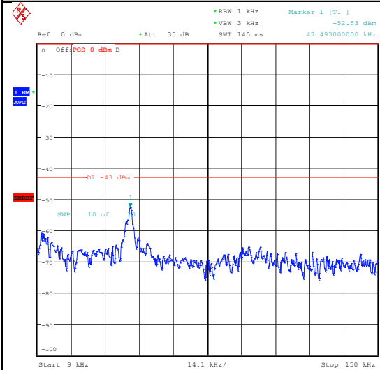
Band4_10MHz_16QAM_20000_1RB#0_1000~3000_00_1000~3000
