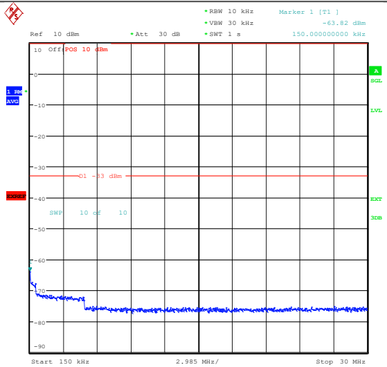
Band4_20MHz_16QAM_20050_1RB#0_3000~20000_00_3000~20000
