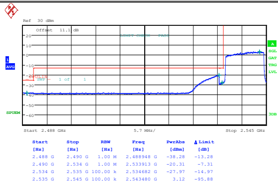
Band41_10MHz_16QAM_40090_1RB#49
