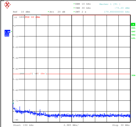
Band41_10MHz_QPSK_40090_50RB#0_20000~ 27000_20000~27000
