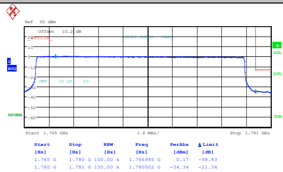
Band66_15MHz_16QAM_132597_1RB#74
