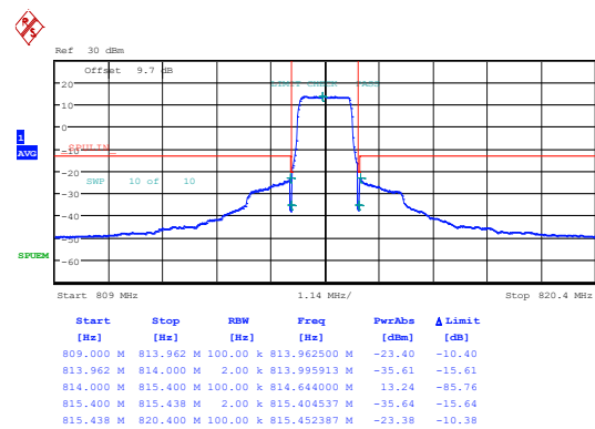
Band26_1.4MHz_QPSK_26697_1RB#5
