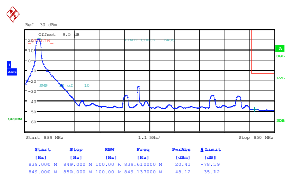
Band26_10MHz_16QAM_26840_50RB#0
