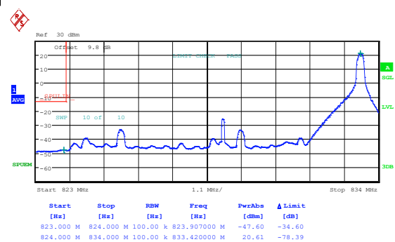
Band26_10MHz_16QAM_26840_1RB#0
