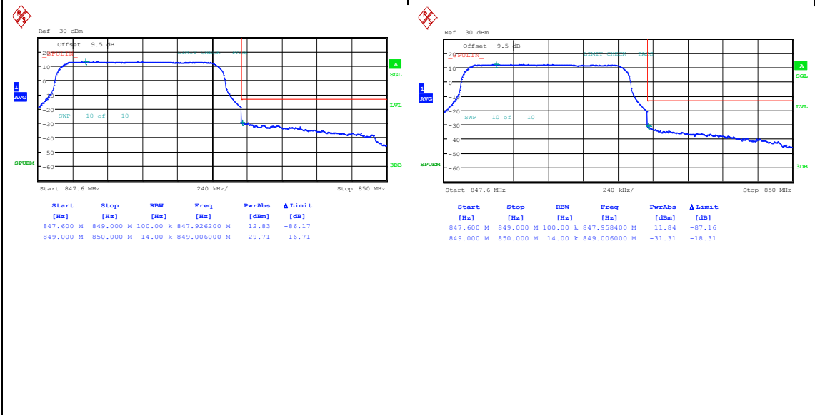
Band26_1.4MHz_QPSK_27033_6RB#0
