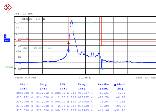
Band26_1.4MHz_QPSK_26783_6RB#0
