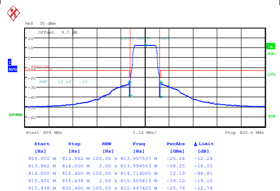
Band26_1.4MHz_16QAM_26697_1RB#5
