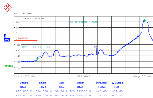
Band26_5MHz_QPSK_26815_1RB#0
