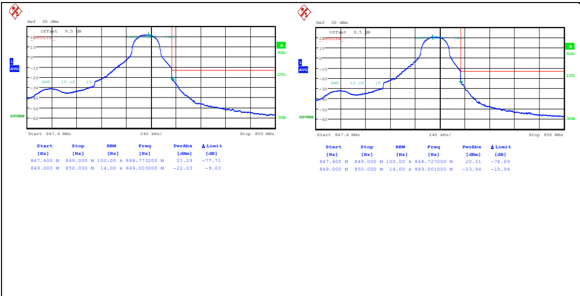
Band26_1.4MHz_QPSK_27033_1RB#5
