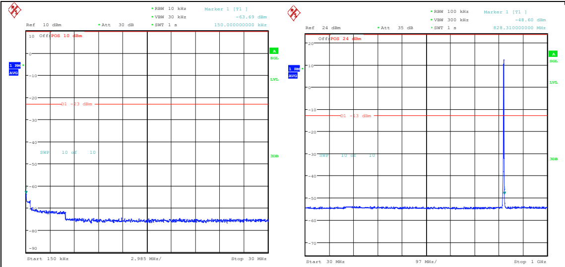
Band26_1.4MHz_16QAM_26797_6RB#0_0.15~30 0_0.15~30 Band26_1.4MHz_16QAM_26797_6RB#0_30~100 0_30~1000
