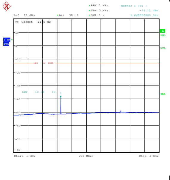
Band26_3MHz_QPSK_26805_1RB#0_1000~3000_1000~3000
