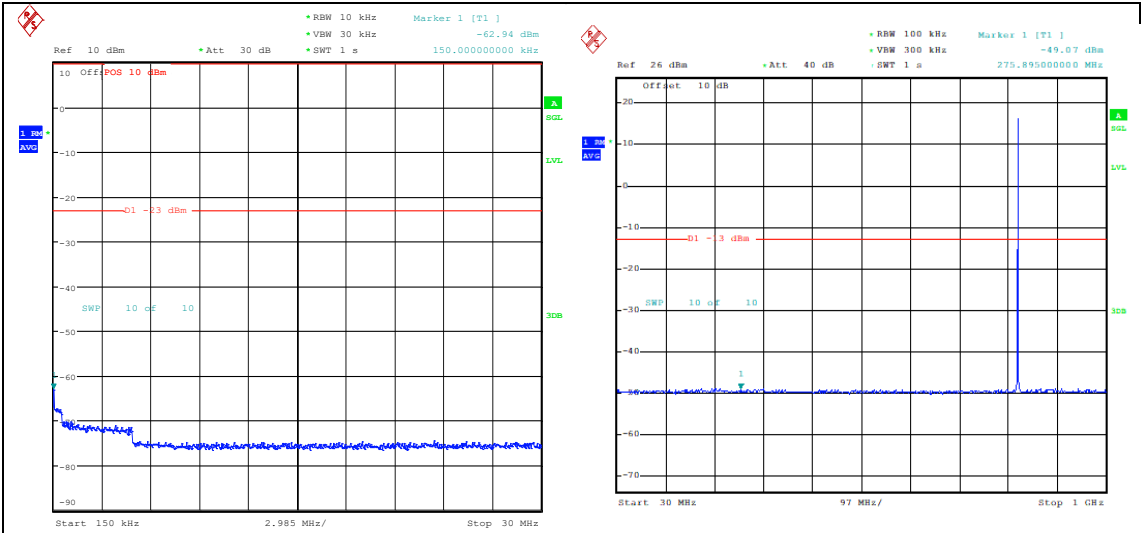
Band26_1.4MHz_16QAM_26797_1RB#0_0.15~3 0_0.15~30
