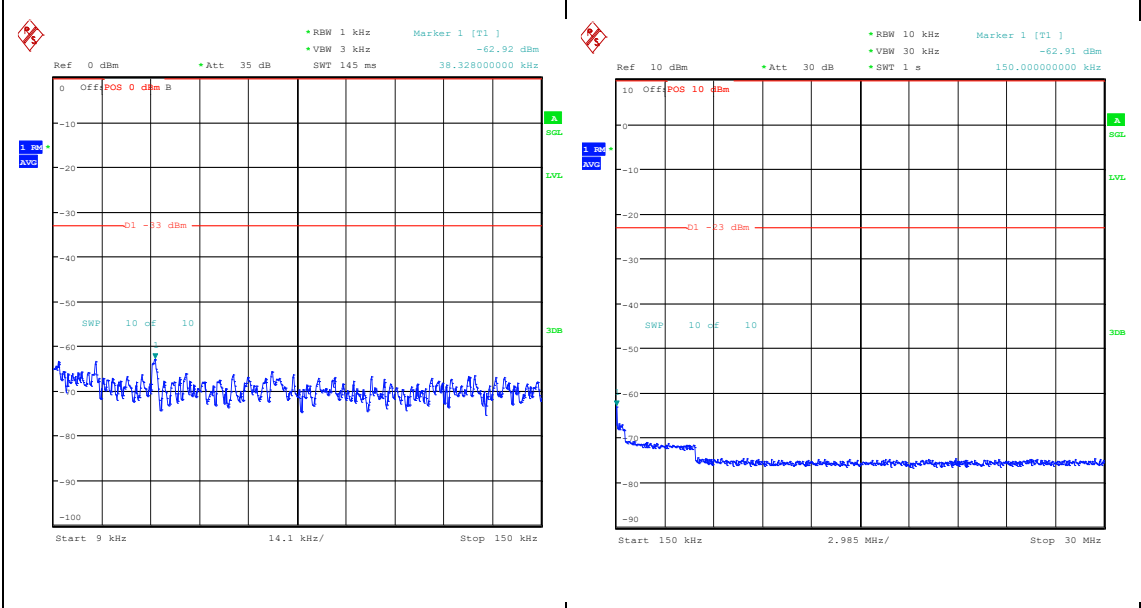
Band26_3MHz_QPSK_26805_1RB#14_0.009~0.15_0.009~0.15 Band26_3MHz_QPSK_26805_1RB#14_0.15~30_0.15~30
