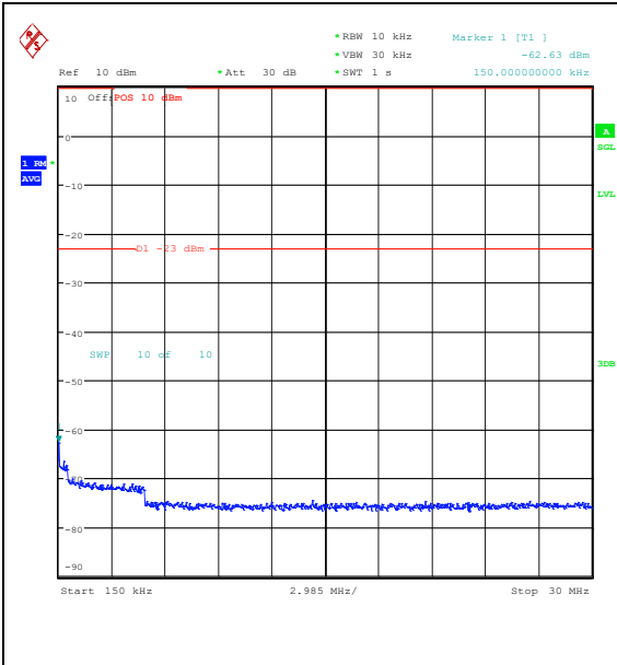
Band26_5MHz_16QAM_26915_1RB#24_0.15~3 0_0.15~30
