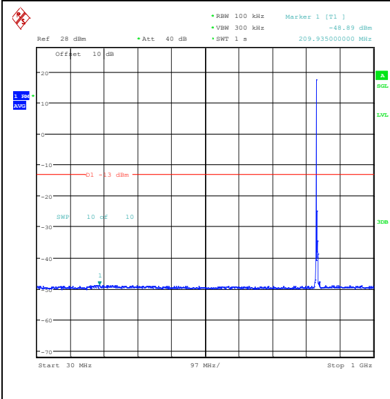
Band26_5MHz_QPSK_26915_1RB#0_30~1000_ 30~1000
