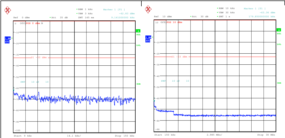
Band26_10MHz_QPSK_26740_50RB#0_0.009~0.15 _15_0.009~0.15 Band26_10MHz_QPSK_26740_50RB#0_0.15~30 _0.15~30
