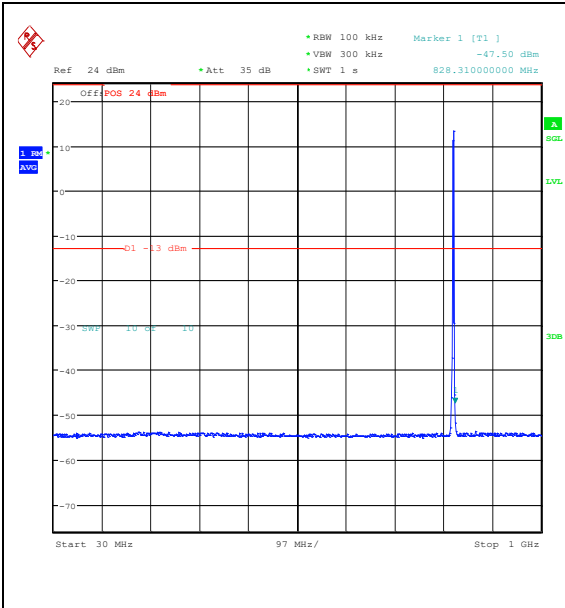
Band26_1.4MHz_QPSK_26797_6RB#0_30~1000_30~1000
