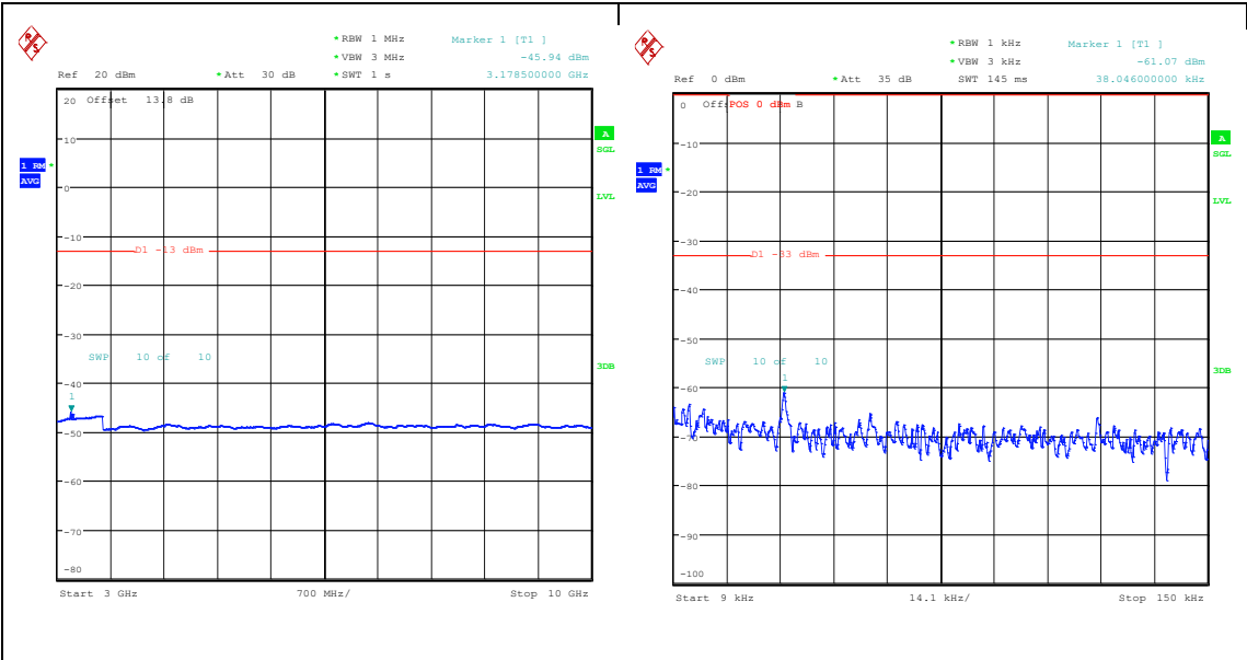
Band26_3MHz_QPSK_27025_1RB#0_3000~10000_3000~10000 Band26_3MHz_16QAM_27025_1RB#0_0.009~0.15_5_0.009~0.15
