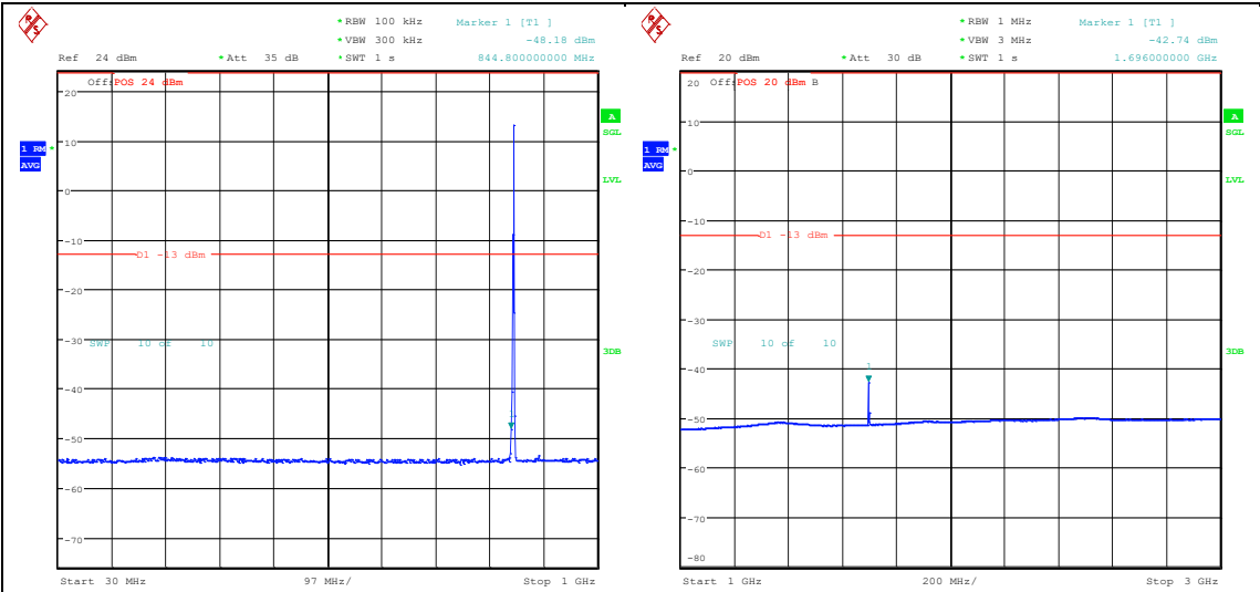
Band26_1.4MHz_QPSK_27033_6RB#0_30~1000_30~1000 Band26_1.4MHz_QPSK_27033_6RB#0_1000~3000_1000~3000
