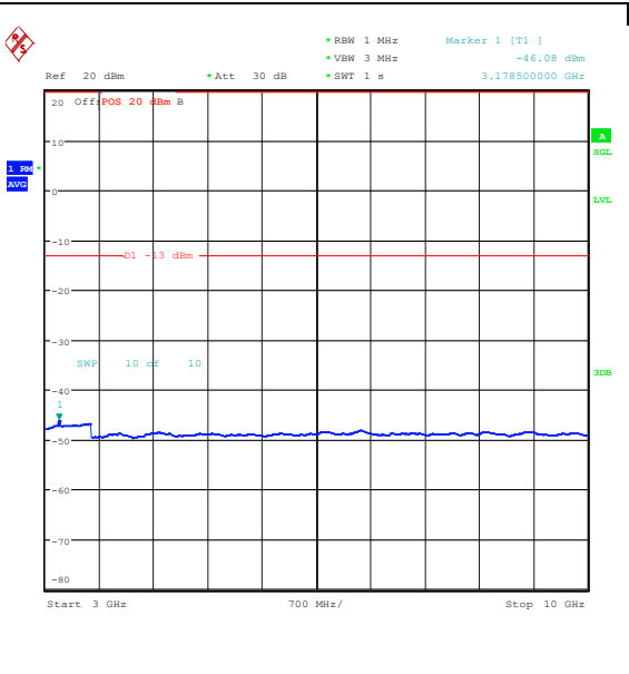
Band26_10MHz_16QAM_26740_50RB#0_3000~10000_3000~10000
