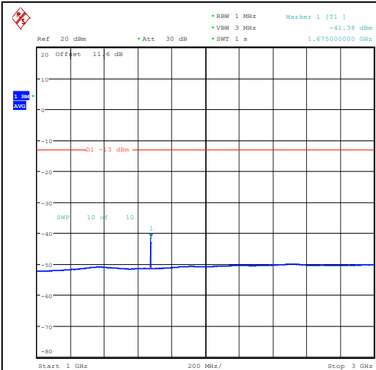
Band26_3MHz_16QAM_26915_1RB#14_1000~3000_1000~3000
