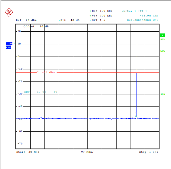
Band26_1.4MHz_QPSK_27033_1RB#5_30~1000_30~1000
