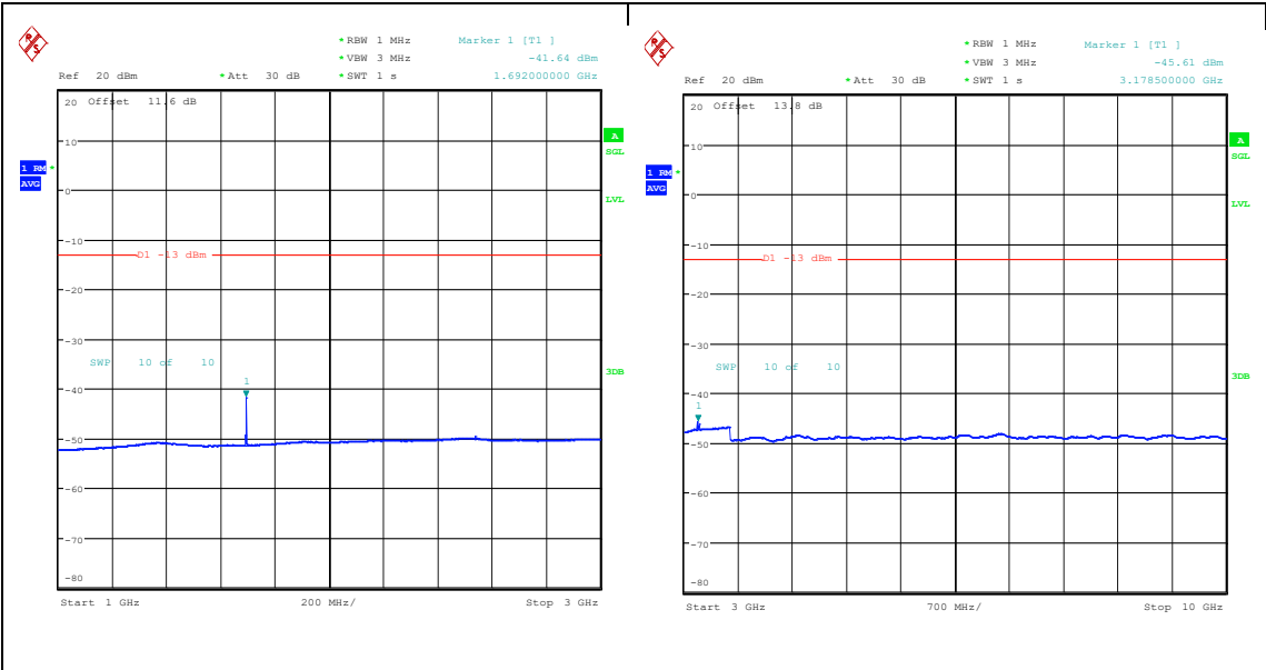
Band26_3MHz_16QAM_27025_1RB#0_1000~3000_00_1000~3000 Band26_3MHz_16QAM_27025_1RB#0_3000~10000_00_3000~10000
