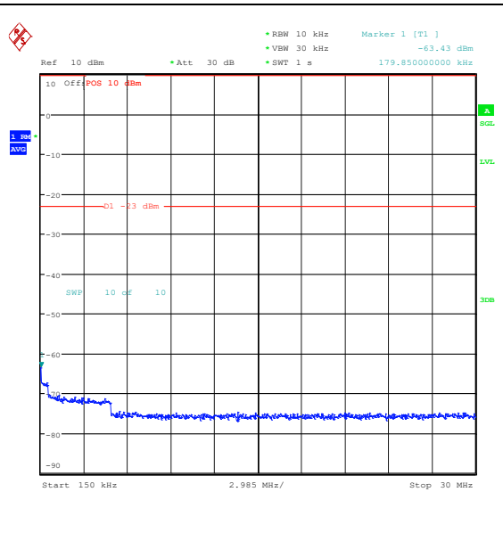
Band26_10MHz_QPSK_26740_1RB#0_0.15~30_0.15~30
