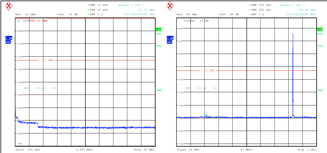
Band26_3MHz_16QAM_26915_1RB#0_0.15~30 _0.15~30
