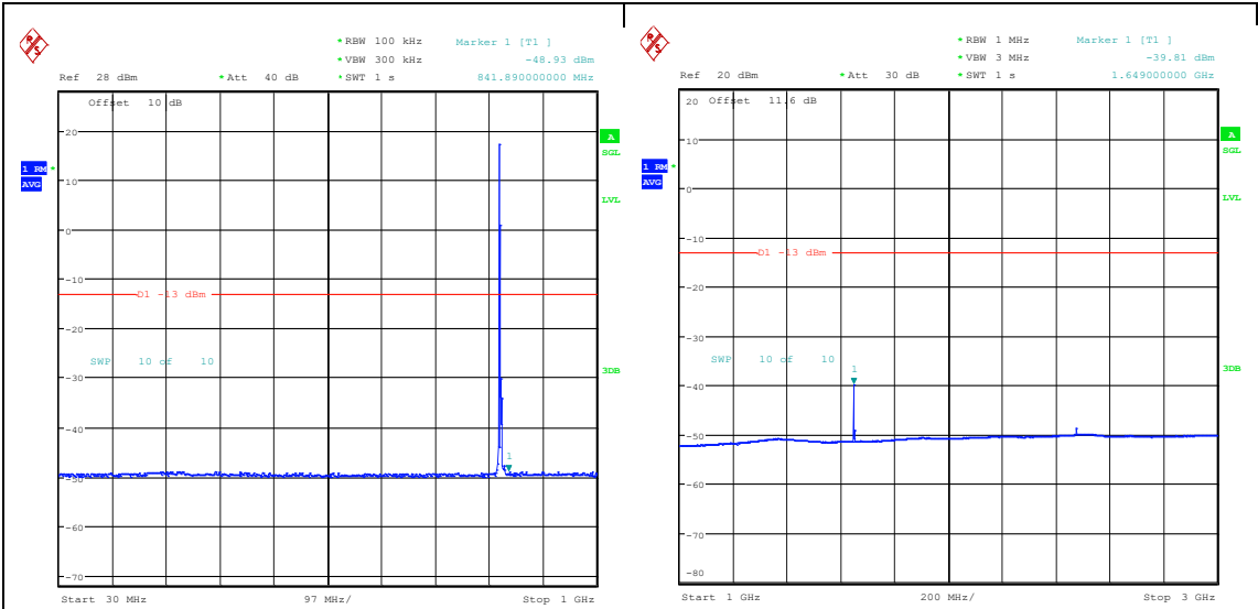
Band26_5MHz_QPSK_26815_1RB#0_30~1000_30~1000 Band26_5MHz_QPSK_26815_1RB#0_1000~3000_1000~3000
