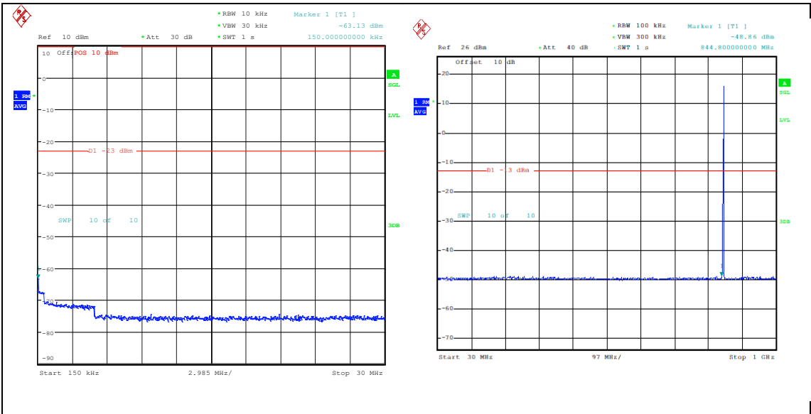
Band26_1.4MHz_16QAM_27033_1RB#0_0.15~30_0.15~30 Band26_1.4MHz_16QAM_27033_1RB#0_30~1000_30~1000
