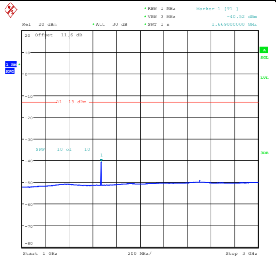
Band26_5MHz_QPSK_26915_1RB#0_1000~3000_ _1000~3000
