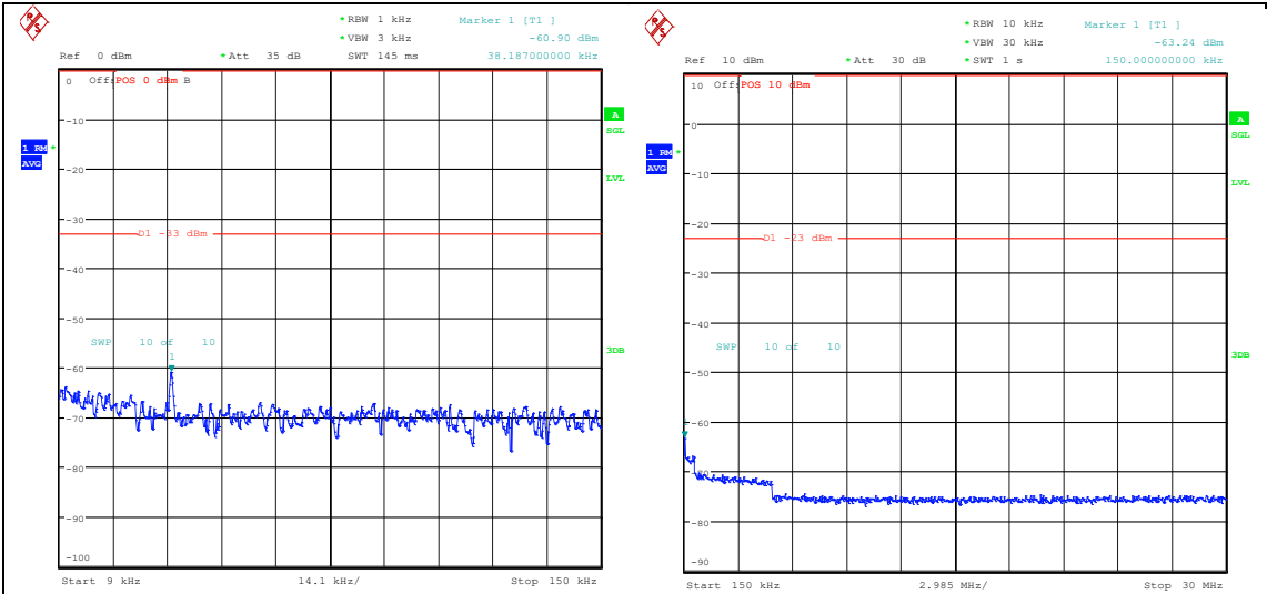
Band26_5MHz_QPSK_26915_25RB#0_0.009~0.15_0.009~0.15 Band26_5MHz_QPSK_26915_25RB#0_0.15~30_0.15~30
