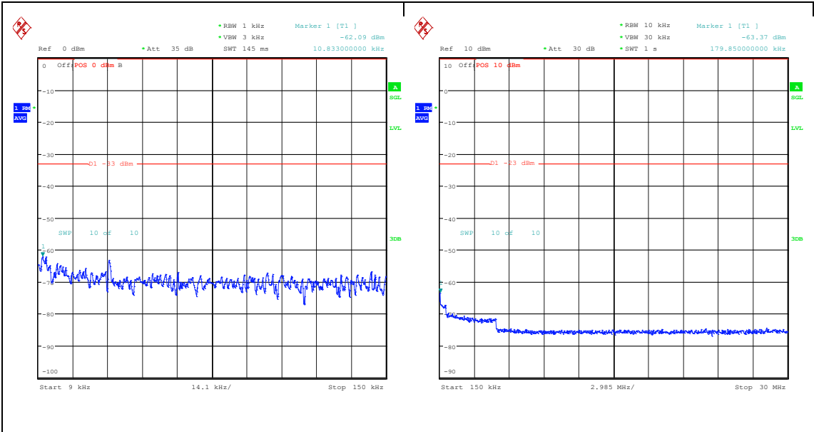
Band26_3MHz_QPSK_26805_15RB#0_0.009~0.15_0.009~0.15 Band26_3MHz_QPSK_26805_15RB#0_0.15~30_0.15~30
