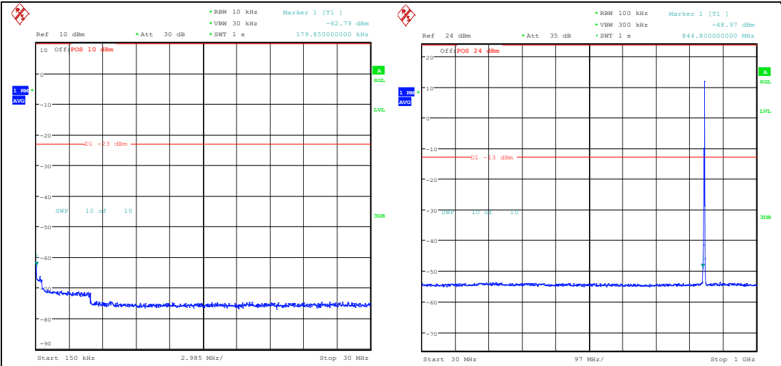
Band26_1.4MHz_16QAM_27033_6RB#0_0.15~30 0_0.15~30 Band26_1.4MHz_16QAM_27033_6RB#0_30~100 0_30~1000
