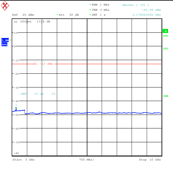
Band26_5MHz_16QAM_26915_1RB#24_3000~10 000_3000~10000
