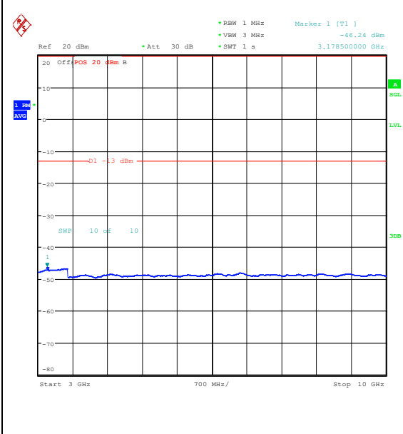
Band26_1.4MHz_QPSK_26797_6RB#0_3000~10_000_3000~10000
