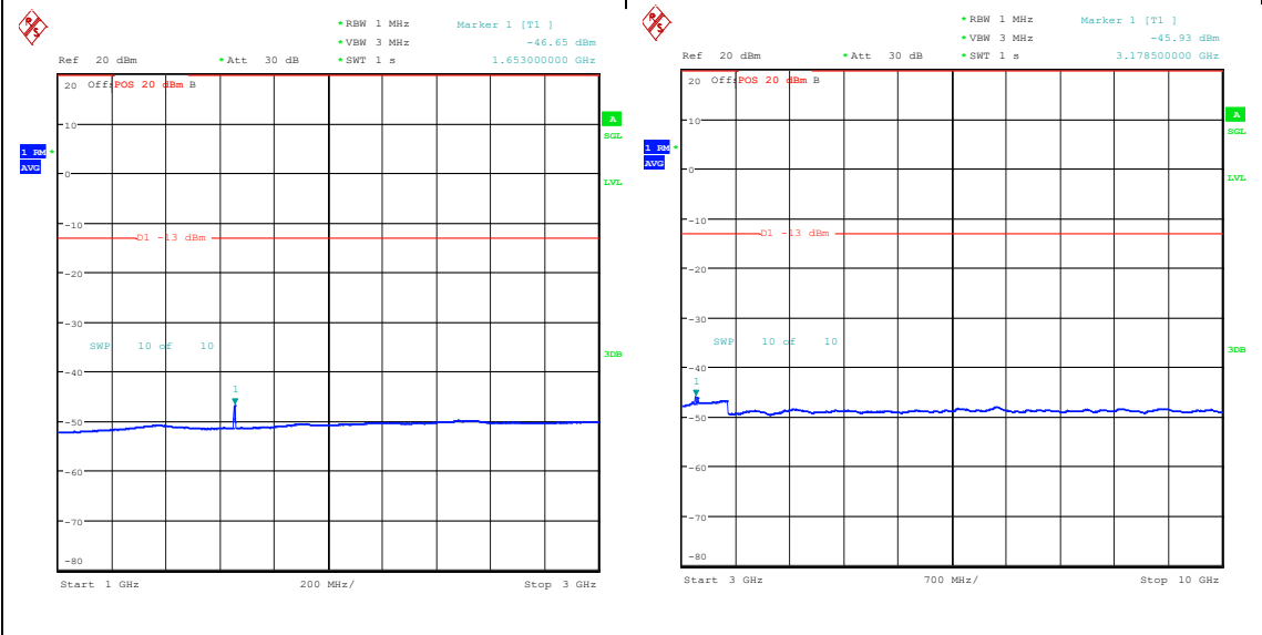
Band26_5MHz_16QAM_26815_25RB#0_1000~3 000_1000~3000 Band26_5MHz_16QAM_26815_25RB#0_3000~10 000_3000~10000
