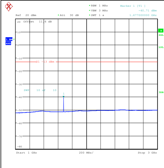
Band26_5MHz_16QAM_26915_1RB#24_1000~3 000_1000~3000
