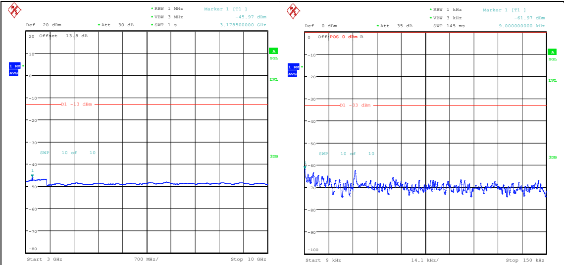
Band26_1.4MHz_QPSK_27033_1RB#5_3000~10000_3000~10000 Band26_1.4MHz_16QAM_27033_1RB#5_0.009~0.15_0.009~0.15
