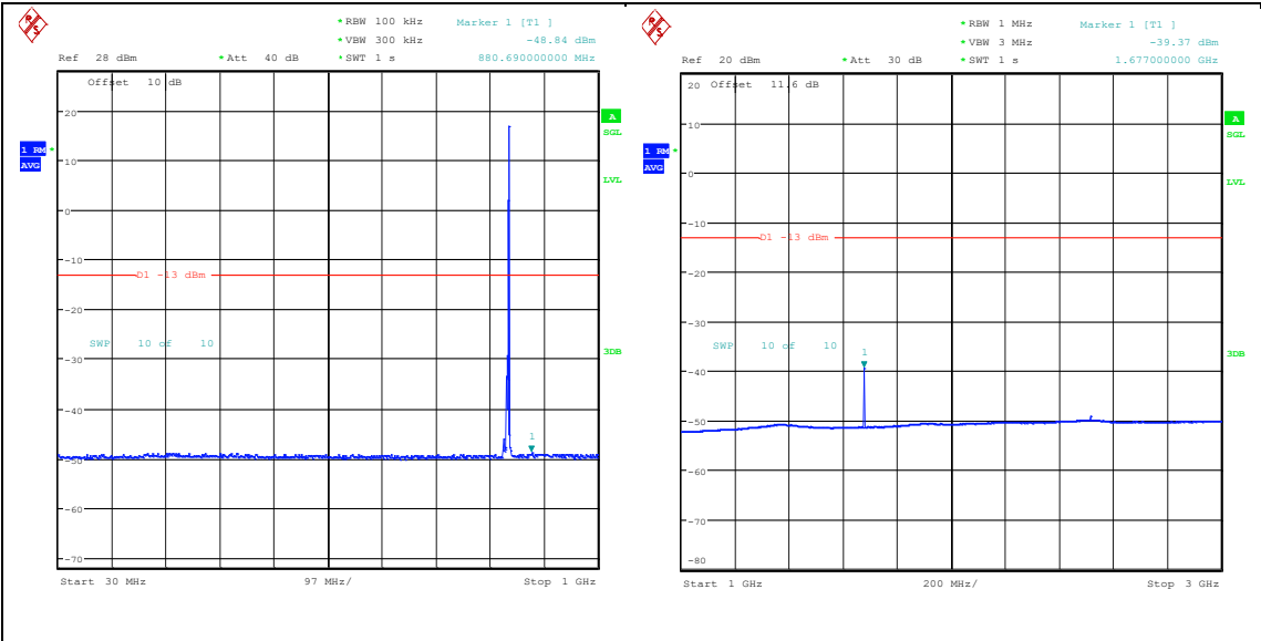
Band26_5MHz_QPSK_26915_1RB#24_30~1000_30~1000 Band26_5MHz_QPSK_26915_1RB#24_1000~3000_0_1000~3000
