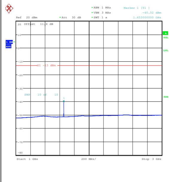
Band26_3MHz_16QAM_26805_1RB#14_1000~3000 000_1000~3000
