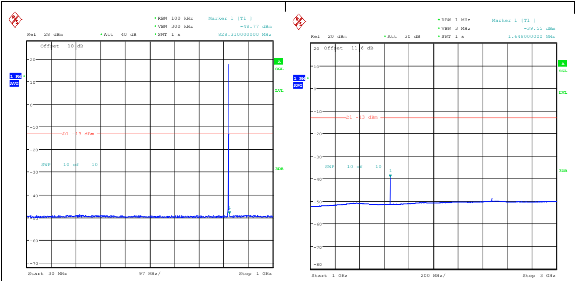
Band26_1.4MHz_QPSK_26797_1RB#0_30~1000_30~1000 Band26_1.4MHz_QPSK_26797_1RB#0_1000~3000_00_1000~3000
