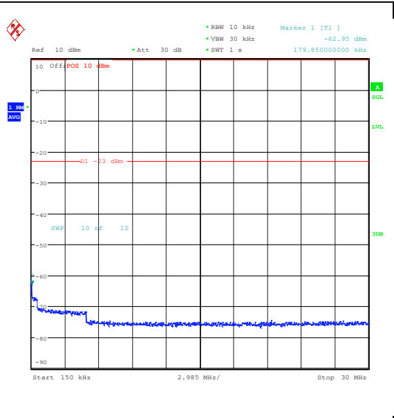
Band26_5MHz_QPSK_26915_1RB#0_0.15~30_0. 15~30
