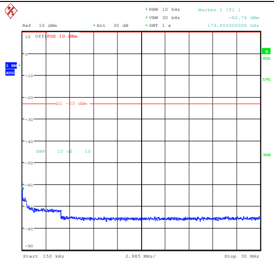
Band26_1.4MHz_QPSK_26915_6RB#0_0.15~30_0.15~30
