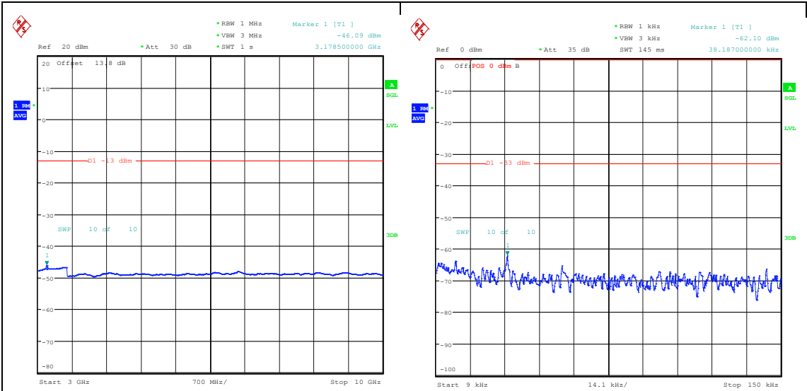
Band26_5MHz_QPSK_26915_1RB#0_3000~10000_3000~10000 Band26_5MHz_16QAM_26915_1RB#0_0.009~0.15_0.009~0.15
