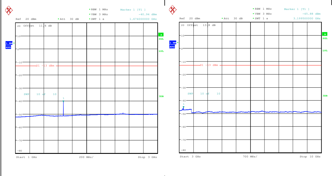
Band26_1.4MHz_16QAM_26915_1RB#5_1000~3000 3000_1000~3000 Band26_1.4MHz_16QAM_26915_1RB#5_3000~10000 0000_3000~10000
