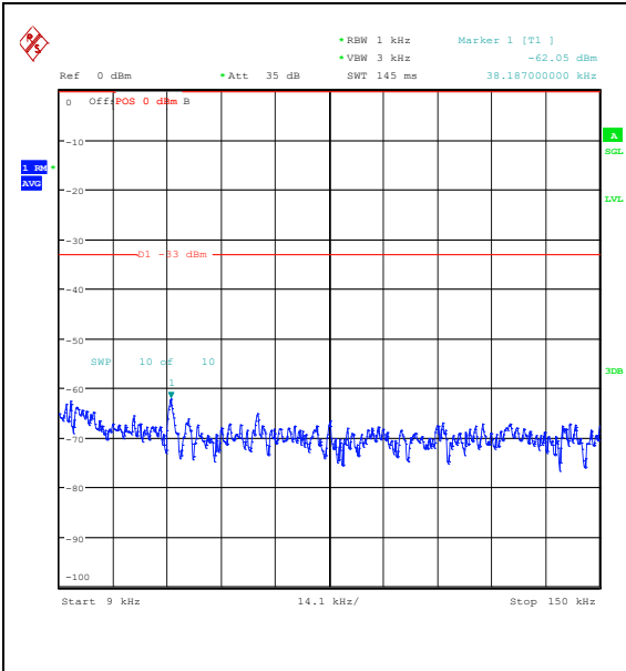
Band26_1.4MHz_QPSK_27033_1RB#5_0.009~0.15_0.009~0.15
