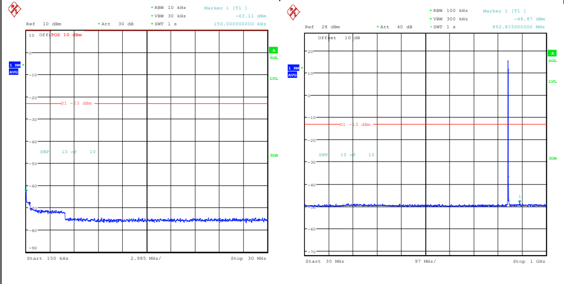
Band26_3MHz_16QAM_27025_1RB#0_0.15~30_0.15~30 Band26_3MHz_16QAM_27025_1RB#0_30~1000_30~1000
