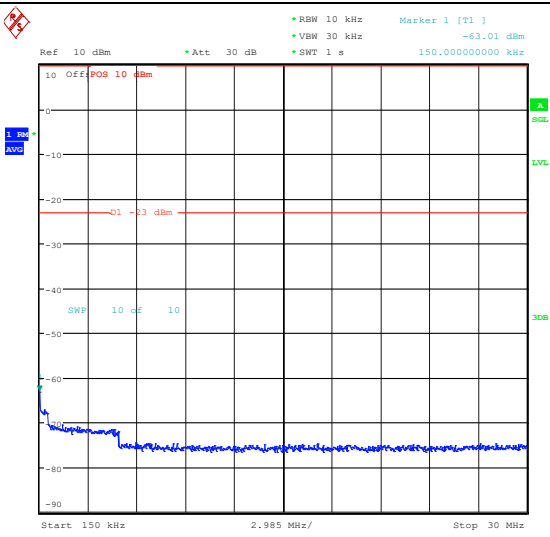
Band26_1.4MHz_QPSK_26915_1RB#0_0.15~30_0.15~30
