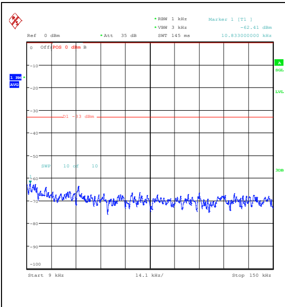
Band26_10MHz_QPSK_26740_1RB#0_0.009~0.15_15_0.009~0.15
