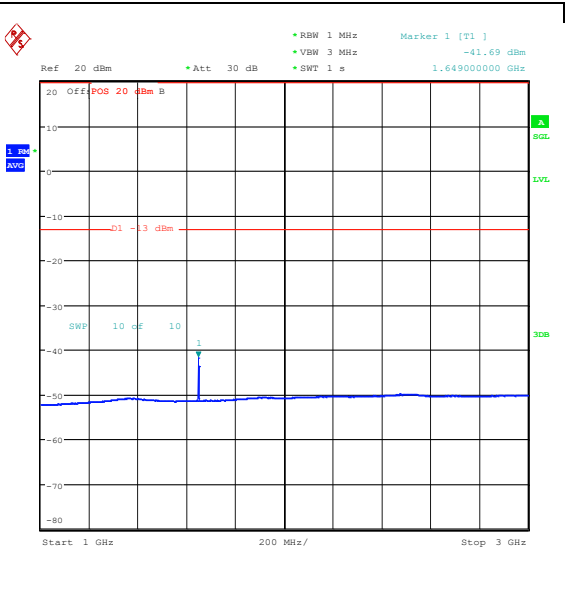
Band26_1.4MHz_QPSK_26797_6RB#0_1000~30_00_1000~3000
