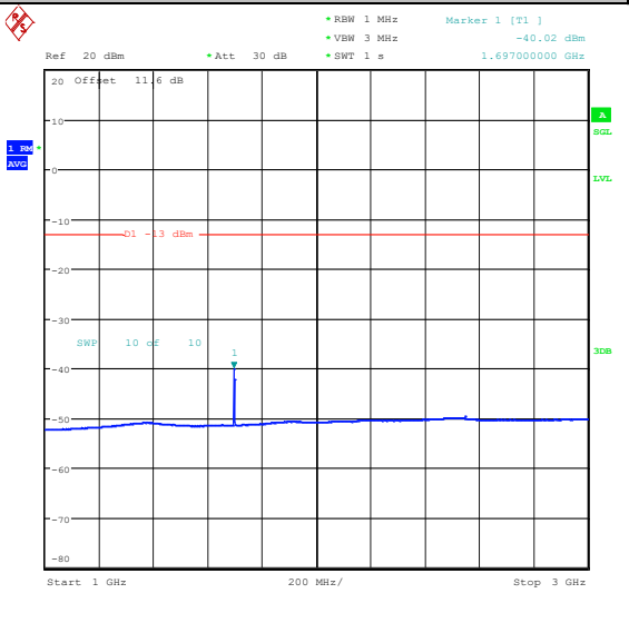
Band26_1.4MHz_QPSK_27033_1RB#5_1000~30_1000~3000
