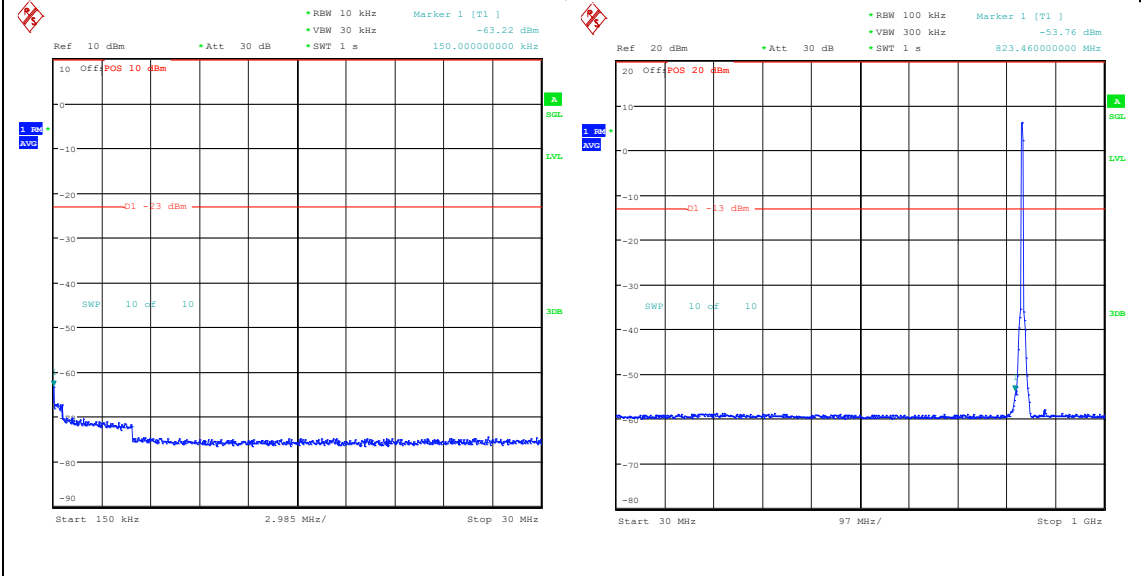
Band26_5MHz_16QAM_26915_25RB#0_0.15~30_0.15~30 Band26_5MHz_16QAM_26915_25RB#0_30~1000_30~1000
