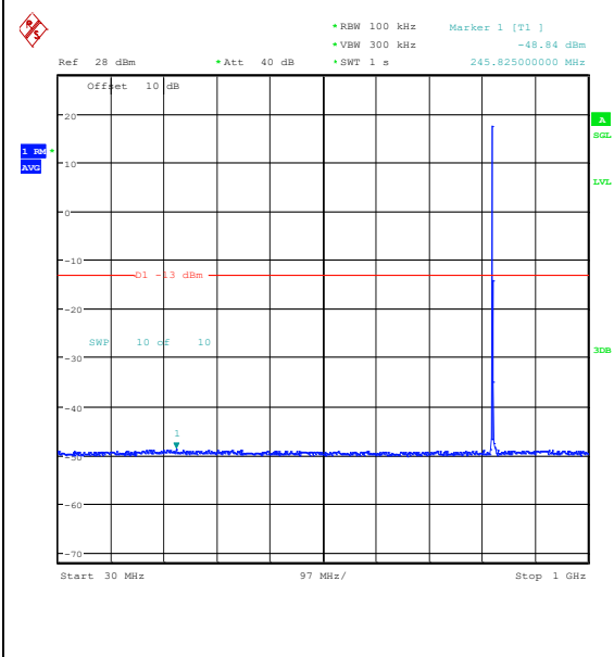
Band26_3MHz_QPSK_26805_1RB#0_30~1000_30~1000
