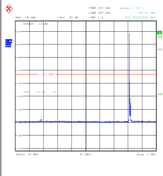
Band26_10MHz_QPSK_26740_1RB#0_30~1000_30~1000
