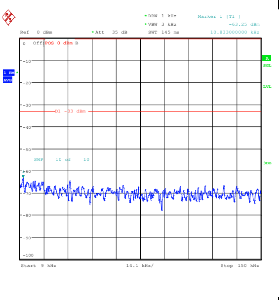
Band26_1.4MHz_16QAM_26797_6RB#0_0.009~0.15_0.009~0.15
