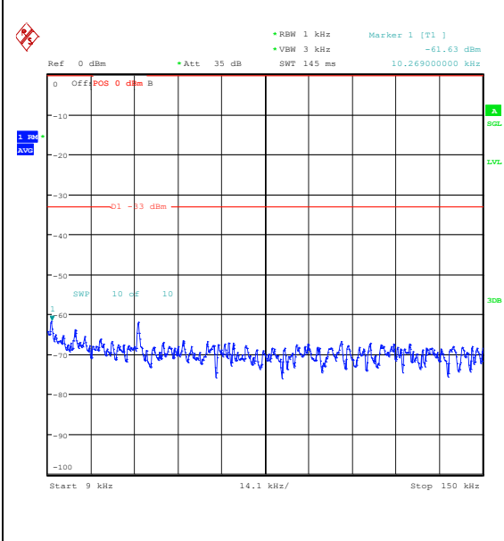
Band26_1.4MHz_QPSK_26797_1RB#0_0.009~0.15_0.009~0.15
