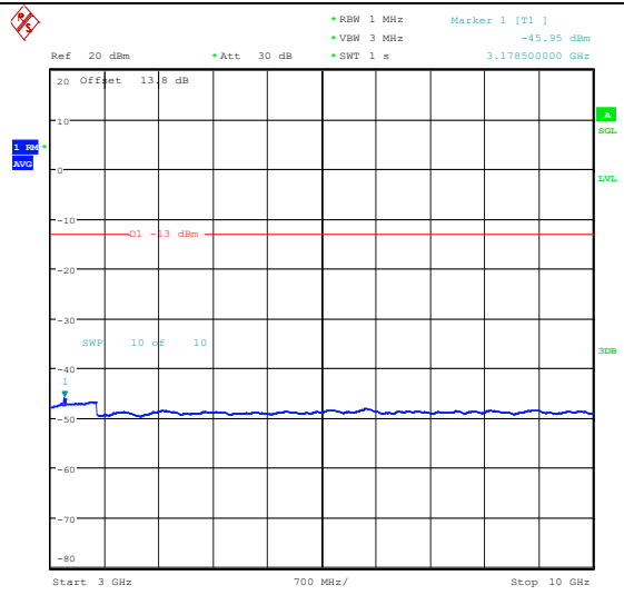
Band26_3MHz_16QAM_26915_1RB#14_3000~10000_3000~10000
