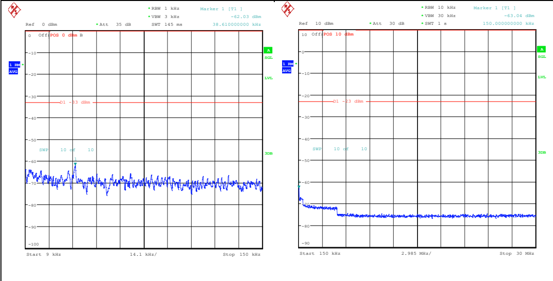
Band26_3MHz_QPSK_27025_1RB#14_0.009~0.15_0.009~0.15 Band26_3MHz_QPSK_27025_1RB#14_0.15~30_0.15~30
