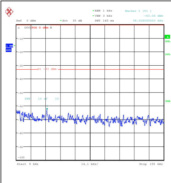
Band26_3MHz_QPSK_26805_1RB#0_0.009~0.15_5_0.009~0.15
