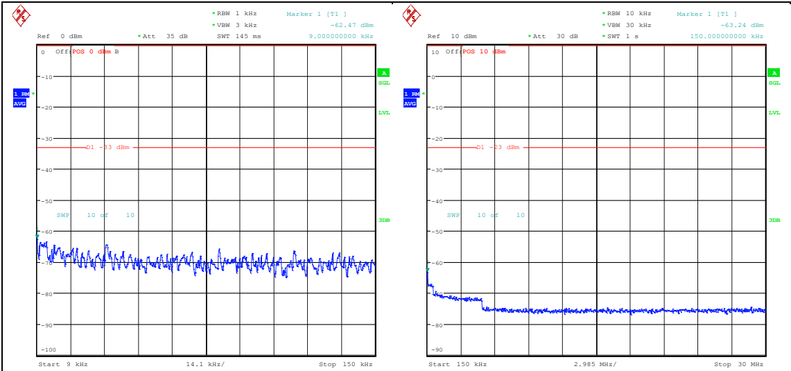
Band26_3MHz_QPSK_27025_15RB#0_0.009~0.15_0.009~0.15 Band26_3MHz_QPSK_27025_15RB#0_0.15~30_0.15~30
