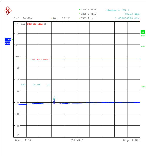
Band26_10MHz_16QAM_26740_50RB#0_1000~3000_1000~3000
