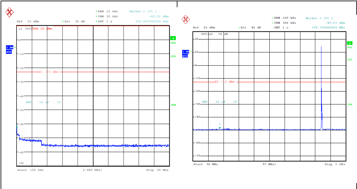
Band26_5MHz_16QAM_27015_1RB#0_0.15~30_0.15~30 Band26_5MHz_16QAM_27015_1RB#0_30~1000_30~1000
