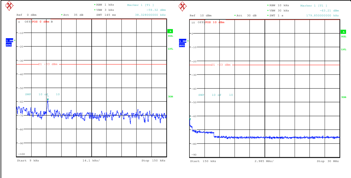
Band26_10MHz_QPSK_26740_1RB#49_0.009~0.15_0.009~0.15 Band26_10MHz_QPSK_26740_1RB#49_0.15~30_0.15~30
