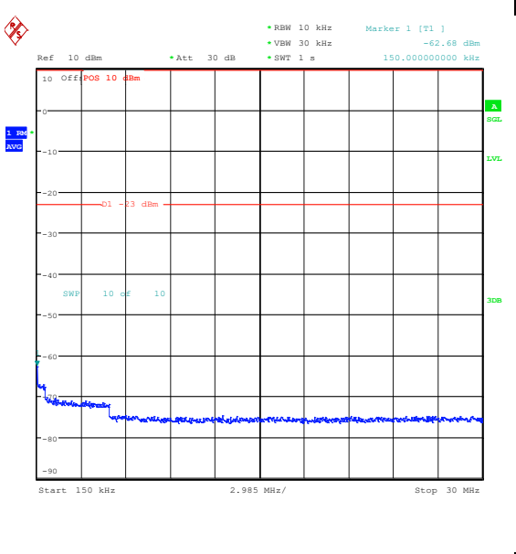
Band26_1.4MHz_QPSK_26797_1RB#0_0.15~30_0.15~30
