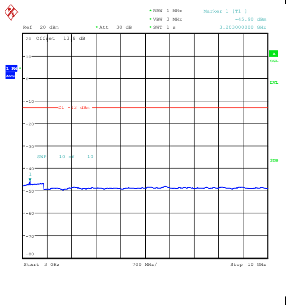
Band26_3MHz_16QAM_26805_1RB#14_3000~10000 000_3000~10000
