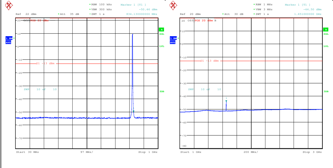
Band26_3MHz_QPSK_26805_15RB#0_30~1000_30~1000 Band26_3MHz_QPSK_26805_15RB#0_1000~3000_0_1000~3000
