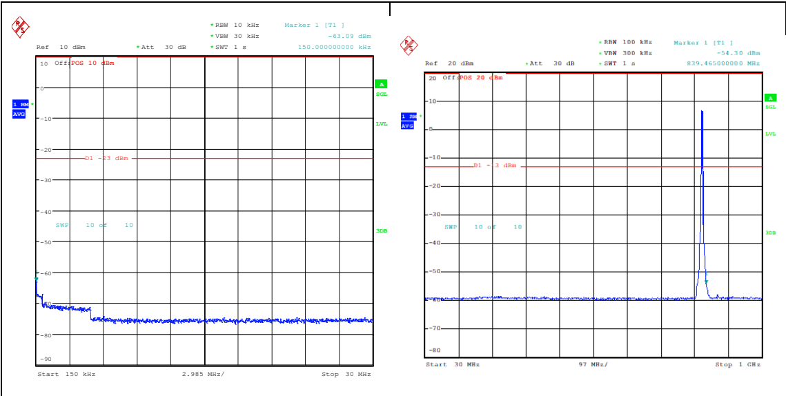
Band26_5MHz_16QAM_26815_25RB#0_0.15~3 0_0.15~30 Band26_5MHz_16QAM_26815_25RB#0_30~1000 _30~1000
