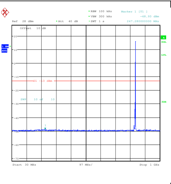
Band26_5MHz_16QAM_26915_1RB#24_30~1000 _30~1000
