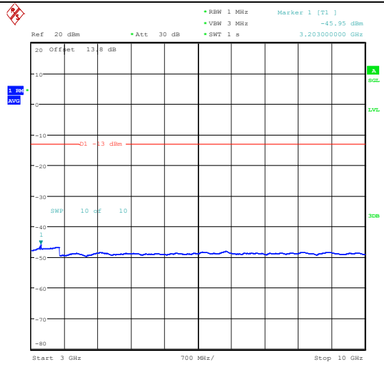
Band26_5MHz_16QAM_26815_1RB#24_3000~10000_3000~10000
