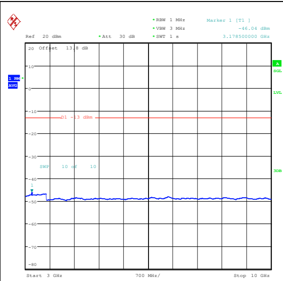
Band26_1.4MHz_QPSK_26915_1RB#0_3000~10000_3000~10000
