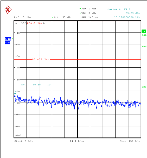
Band26_5MHz_QPSK_26915_1RB#0_0.009~0.15 5_0.009~0.15
