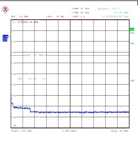
Band26_3MHz_QPSK_26805_1RB#0_0.15~30_0.15~30
