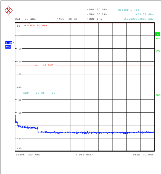
Band26_3MHz_16QAM_26805_1RB#14_0.15~30 0_0.15~30
