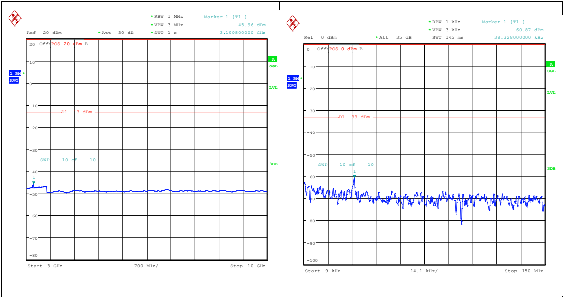
Band26_5MHz_QPSK_26915_25RB#0_3000~10000_3000~10000 Band26_5MHz_16QAM_26915_25RB#0_0.009~0.15_0.009~0.15
