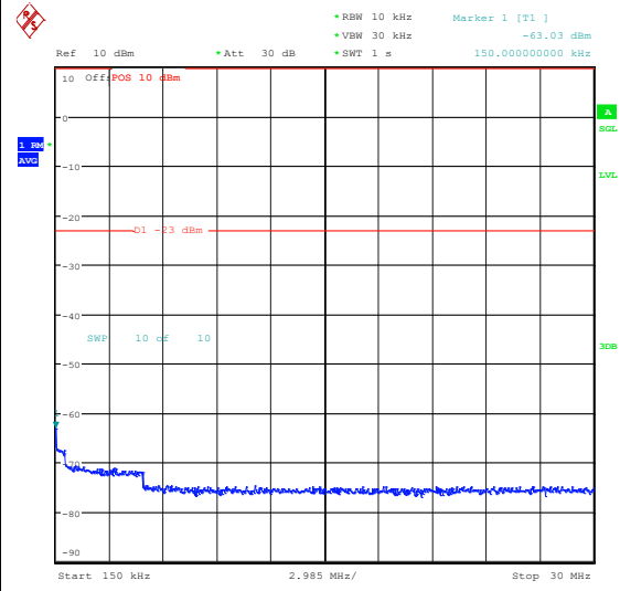
Band26_1.4MHz_16QAM_26915_1RB#0_0.15~30_0.15~30
