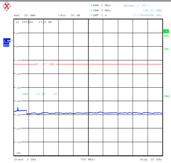
Band26_1.4MHz_16QAM_26797_1RB#5_3000~10000_3000~10000
