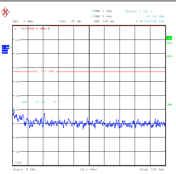
Band26_1.4MHz_16QAM_26915_1RB#0_0.009~0.15_0.009~0.15
