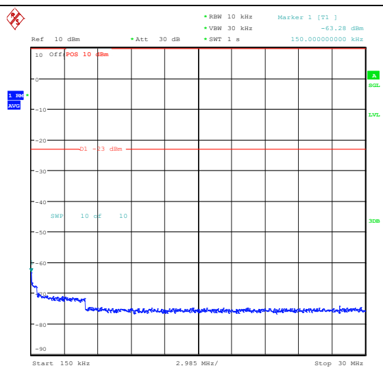
Band26_3MHz_QPSK_26915_1RB#14_0.15~30_0.15~30
