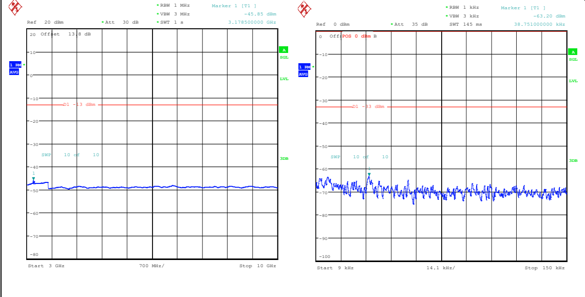
Band26_5MHz_QPSK_26915_1RB#24_3000~10000_000_3000~10000 Band26_5MHz_16QAM_26915_1RB#24_0.009~0.15_0.009~0.15
