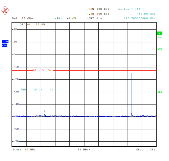
Band26_1.4MHz_16QAM_26915_1RB#0_30~1000_30~1000
