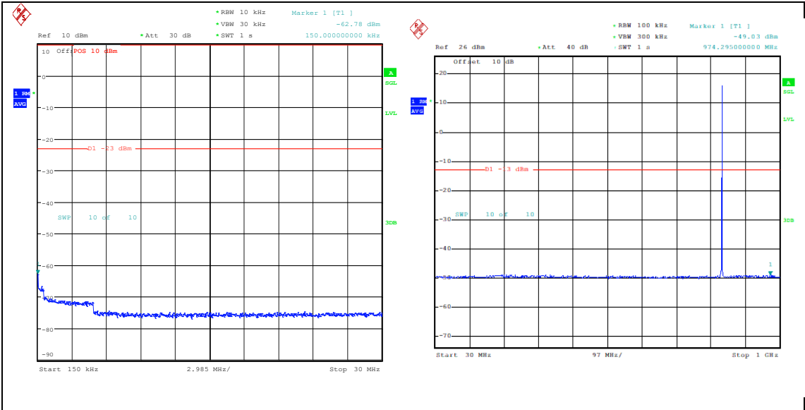
Band26_1.4MHz_16QAM_26915_1RB#5_0.15~30 0_0.15~30 Band26_1.4MHz_16QAM_26915_1RB#5_30~100 0_30~1000
