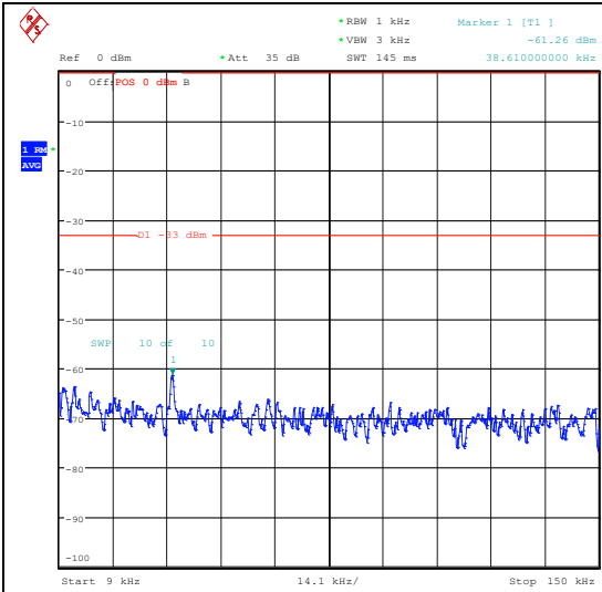
Band26_1.4MHz_QPSK_26915_6RB#0_0.009~0.15_0.009~0.15
