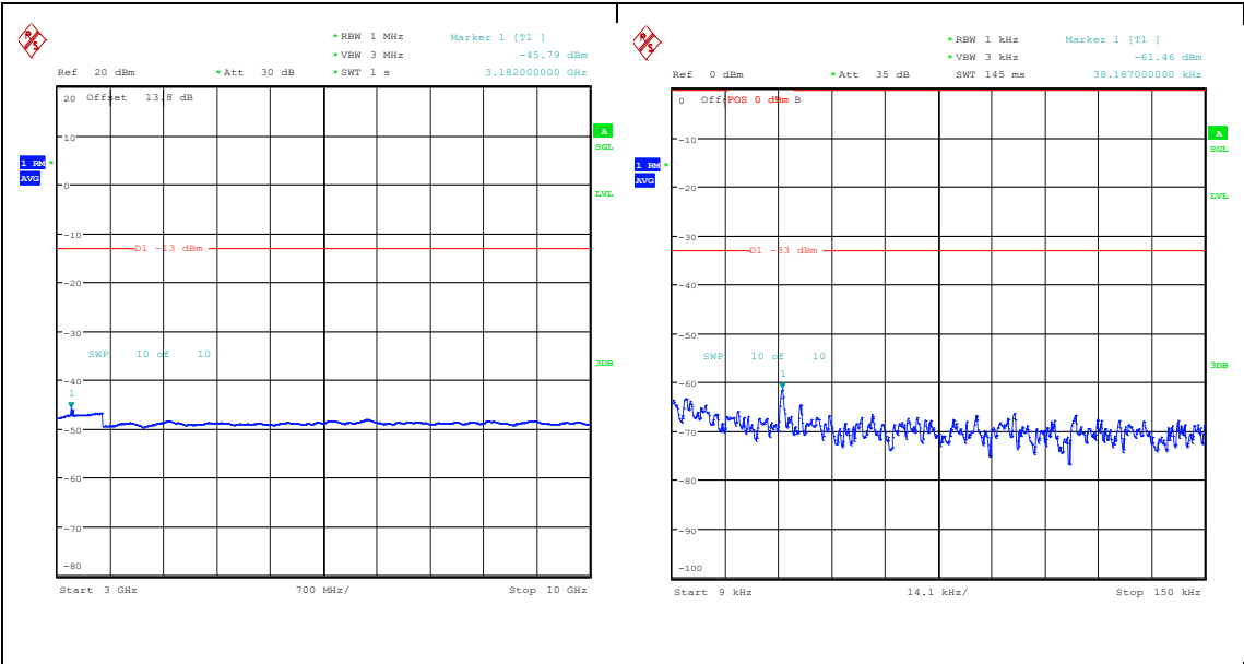
Band26_10MHz_QPSK_26740_1RB#0_3000~10000_3000~10000 Band26_10MHz_16QAM_26740_1RB#0_0.009~0.15_0.009~0.15
