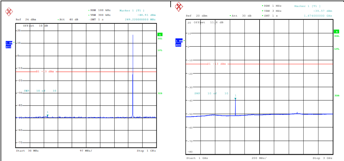
Band26_1.4MHz_QPSK_26915_1RB#5_30~1000_30~1000 Band26_1.4MHz_QPSK_26915_1RB#5_1000~3000_1000~3000
