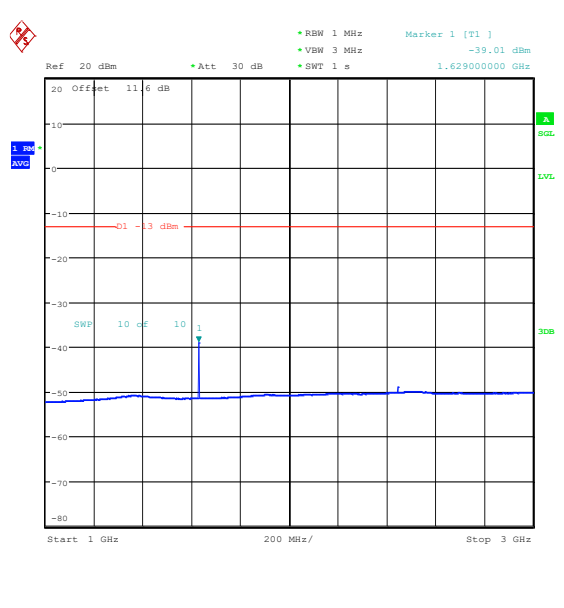
Band26_10MHz_QPSK_26740_1RB#0_1000~3000_0_1000~3000
