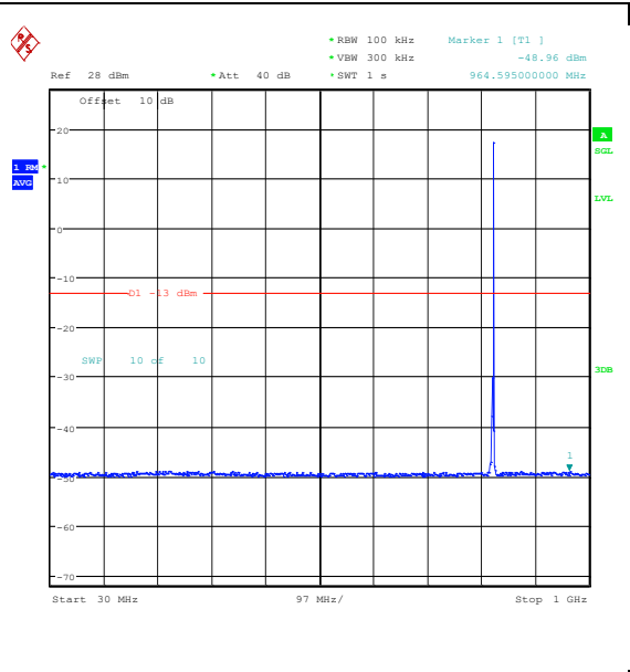
Band26_3MHz_16QAM_26805_1RB#14_30~1000 _30~1000
