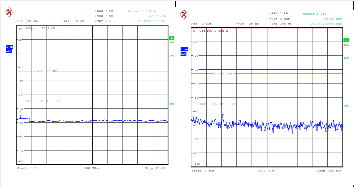
Band26_15MHz_QPSK_26865_1RB#74_3000~10000_3000~10000 Band26_15MHz_16QAM_26865_1RB#74_0.009~0.15_0.009~0.15
