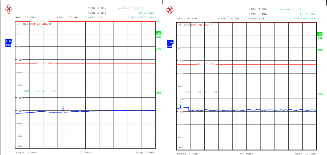
Band26_15MHz_16QAM_26965_75RB#0_0.15~30_0.15~30
