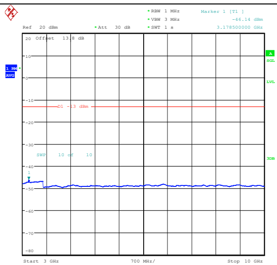
Band26_10MHz_16QAM_26990_1RB#0_3000~10000_3000~10000
