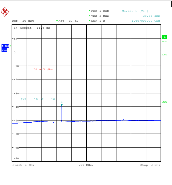
Band26_10MHz_QPSK_26840_1RB#49_1000~30 00_1000~3000
