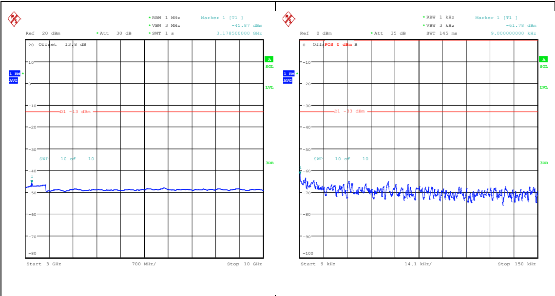
Band26_15MHz_QPSK_26965_1RB#74_3000~10000_3000~10000 Band26_15MHz_16QAM_26965_1RB#74_0.009~0.15_0.009~0.15
