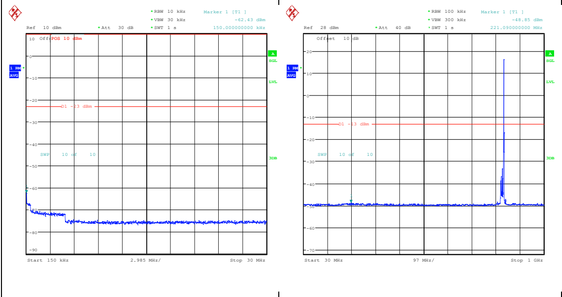
Band26_15MHz_16QAM_26865_1RB#74_0.15~30_0.15~30 Band26_15MHz_16QAM_26865_1RB#74_30~1000_30~1000
