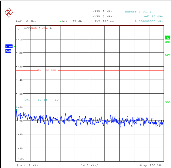
Band26_10MHz_QPSK_26915_1RB#49_0.009~0.15_0.009~0.15
