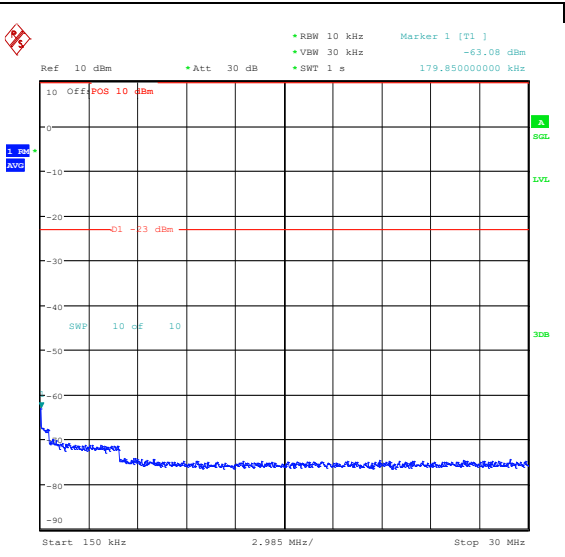
Band26_10MHz_QPSK_26840_50RB#0_0.15~30_0.15~30
