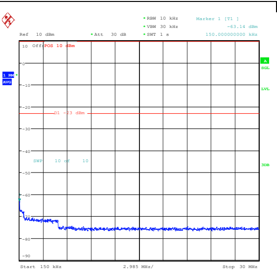
Band26_15MHz_QPSK_26965_1RB#74_0.15~30_0.15~30
