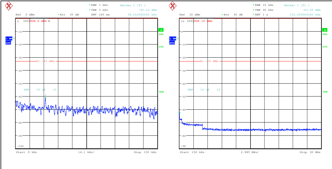
Band26_10MHz_QPSK_26990_50RB#0_0.009~0.15_0.009~0.15 Band26_10MHz_QPSK_26990_50RB#0_0.15~30_0.15~30
