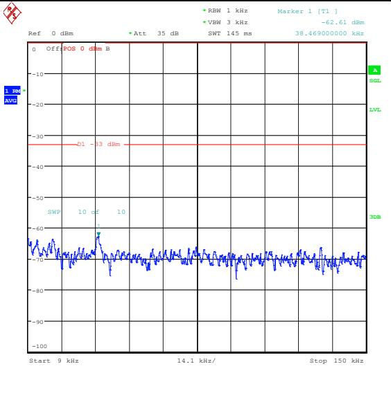
Band26_10MHz_16QAM_26915_1RB#0_0.009~0.15_0.009~0.15
