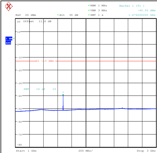
Band26_15MHz_16QAM_26865_1RB#74_1000~3000_1000~3000
