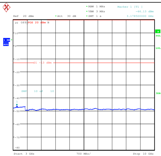
Band26_10MHz_16QAM_26840_50RB#0_1000~3000_1000~3000 Band26_10MHz_16QAM_26840_50RB#0_3000~10000_0000_3000~10000
