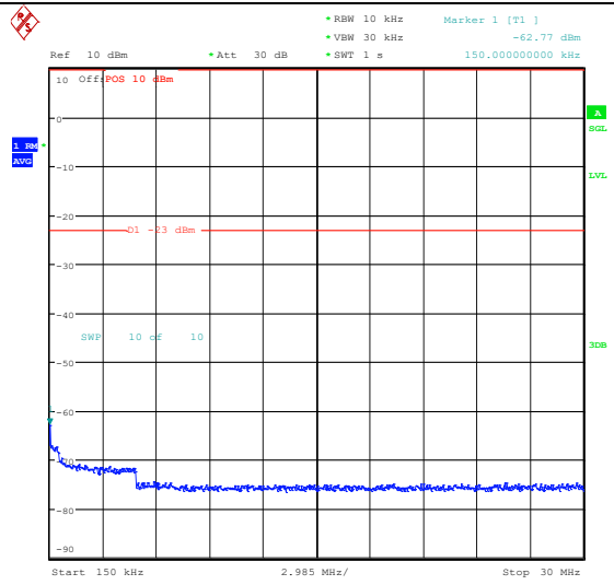
Band26_10MHz_QPSK_26990_1RB#0_0.15~30_0.15~30
