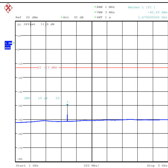
Band26_10MHz_16QAM_26990_1RB#0_1000~3000_1000~3000
