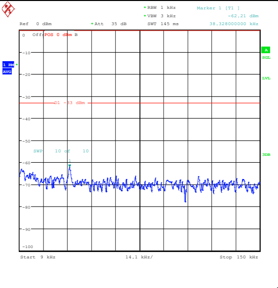
Band26_10MHz_16QAM_26840_1RB#49_0.009~ 0.15_0.009~0.15
