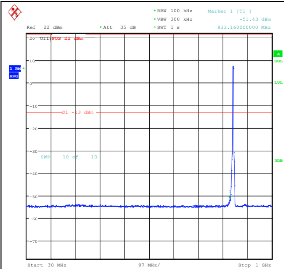
Band26_5MHz_QPSK_27015_25RB#0_30~1000_30~1000
