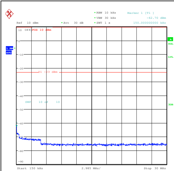
Band26_10MHz_16QAM_26840_1RB#49_0.15~30_0.15~30
