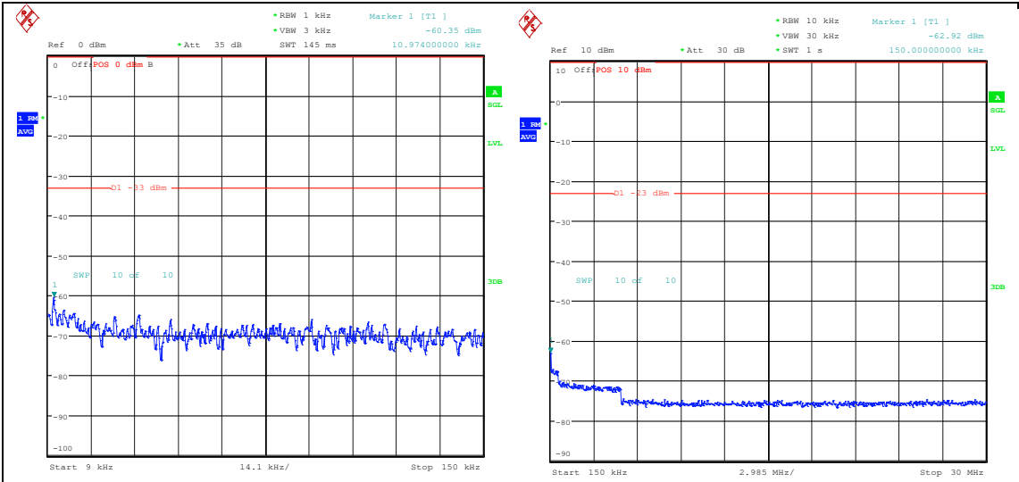
Band26_15MHz_QPSK_26915_1RB#0_0.009~0.15_0.009~0.15 Band26_15MHz_QPSK_26915_1RB#0_0.15~30_0.15~30
