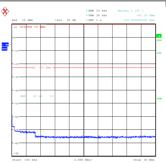
Band26_10MHz_QPSK_26915_1RB#49_0.15~30_0.15~30
