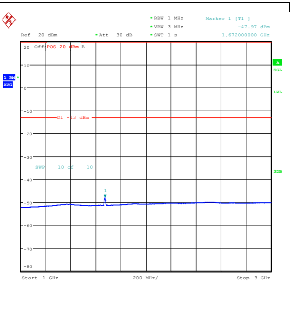
Band26_10MHz_QPSK_26915_50RB#0_1000~3000 00_1000~3000
