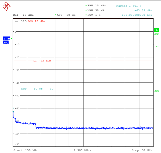
Band26_10MHz_QPSK_26840_1RB#0_0.15~30_0.15~30
