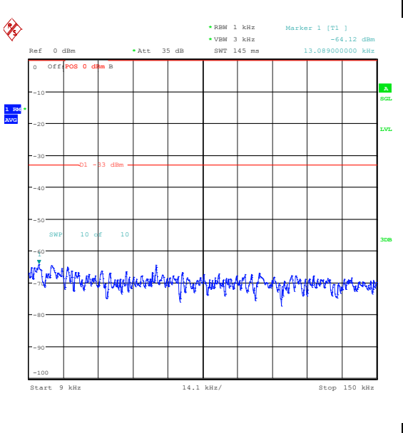
Band26_10MHz_16QAM_26915_50RB#0_0.009~0.15 0.15_0.009~0.15
