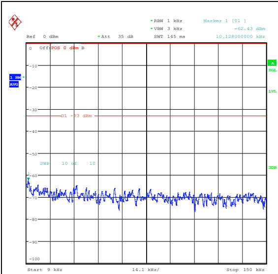
Band26_10MHz_QPSK_26840_50RB#0_0.009~0.15_0.009~0.15
