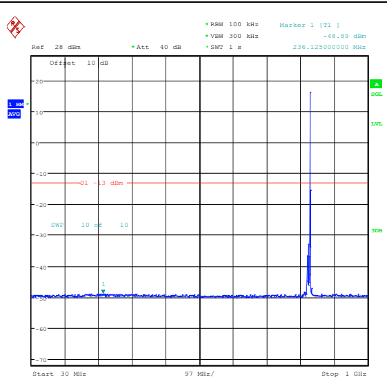
Band26_10MHz_16QAM_26840_1RB#49_30~1000_30~1000
