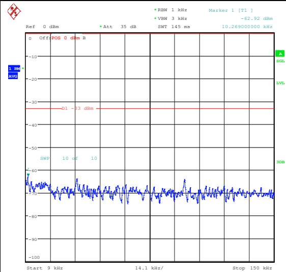
Band26_5MHz_QPSK_27015_1RB#24_0.009~0.15_0.009~0.15
