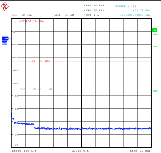
Band26_5MHz_QPSK_27015_1RB#24_0.15~30_0.15~30
