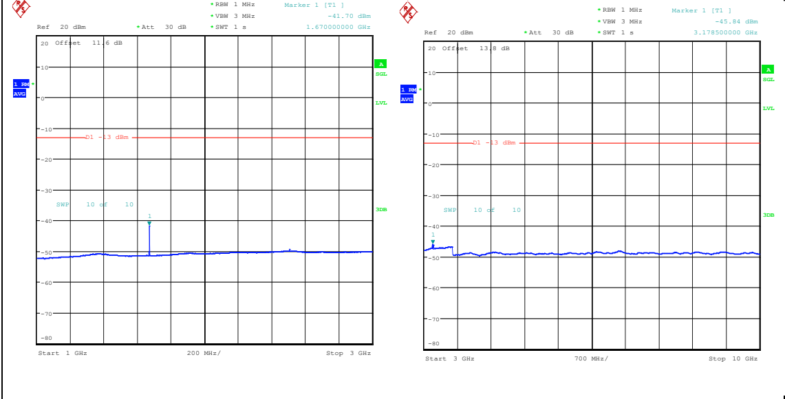
Band26_15MHz_16QAM_26965_1RB#0_1000~30001000~3000 Band26_15MHz_16QAM_26965_1RB#0_3000~100003000~10000
