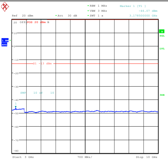
Band26_10MHz_16QAM_26990_50RB#0_3000~10000_3000~10000
