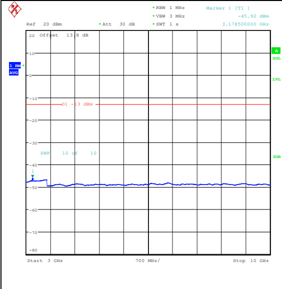
Band26_10MHz_QPSK_26915_1RB#0_3000~10_000_3000~10000
