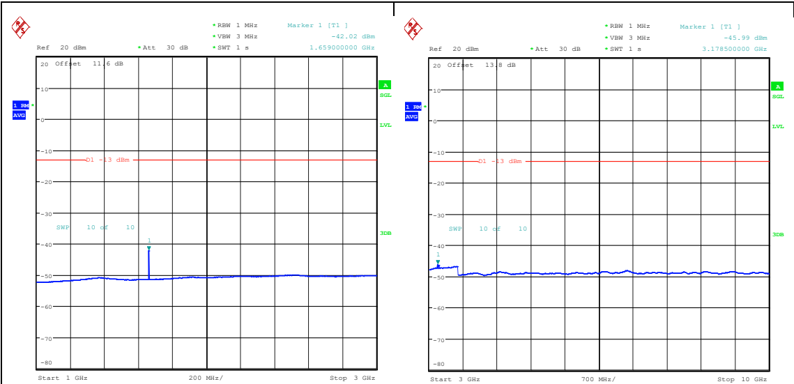
Band26_15MHz_16QAM_26915_1RB#0_1000~3000_1000~3000 Band26_15MHz_16QAM_26915_1RB#0_3000~10000_3000~10000
