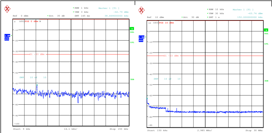
Band26_15MHz_QPSK_26915_75RB#0_0.009~0.15_0.009~0.15 Band26_15MHz_QPSK_26915_75RB#0_0.15~30_0.15~30
