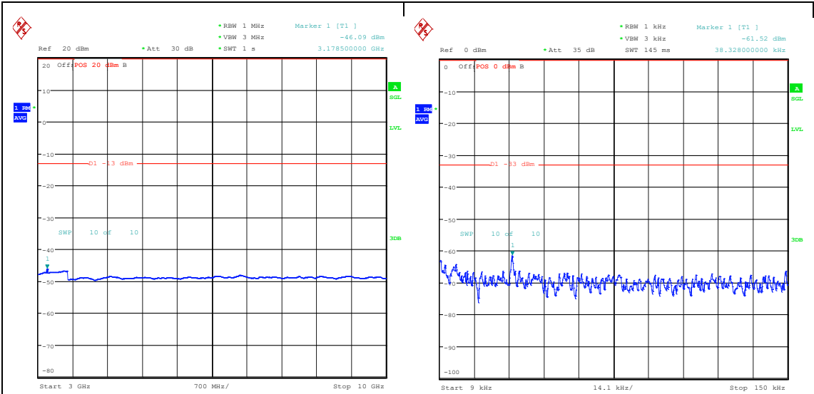
Band26_15MHz_QPSK_26915_75RB#0_3000~10000_3000~10000 Band26_15MHz_16QAM_26915_75RB#0_0.009~0.15_0.009~0.15
