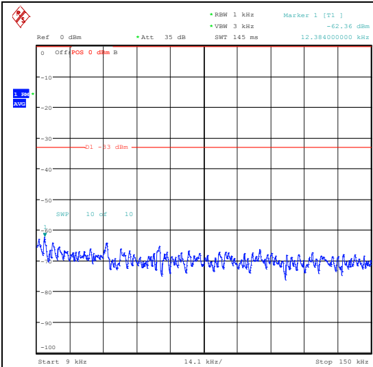
Band26_10MHz_QPSK_26840_1RB#0_0.009~0.15_0.009~0.15
