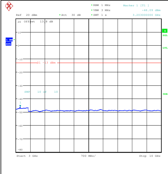
Band26_10MHz_QPSK_26840_1RB#49_3000~1 0000_3000~10000
