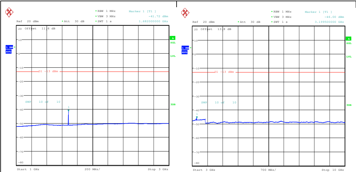
Band26_10MHz_16QAM_26915_1RB#49_1000~3000_1000~3000 Band26_10MHz_16QAM_26915_1RB#49_3000~10000_3000~10000
