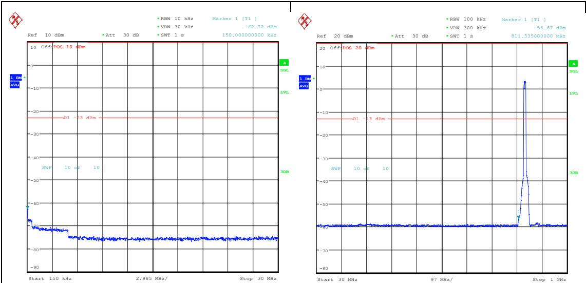
Band26_10MHz_16QAM_26915_50RB#0_0.15~30_0.15~30 Band26_10MHz_16QAM_26915_50RB#0_30~1000_30~1000
