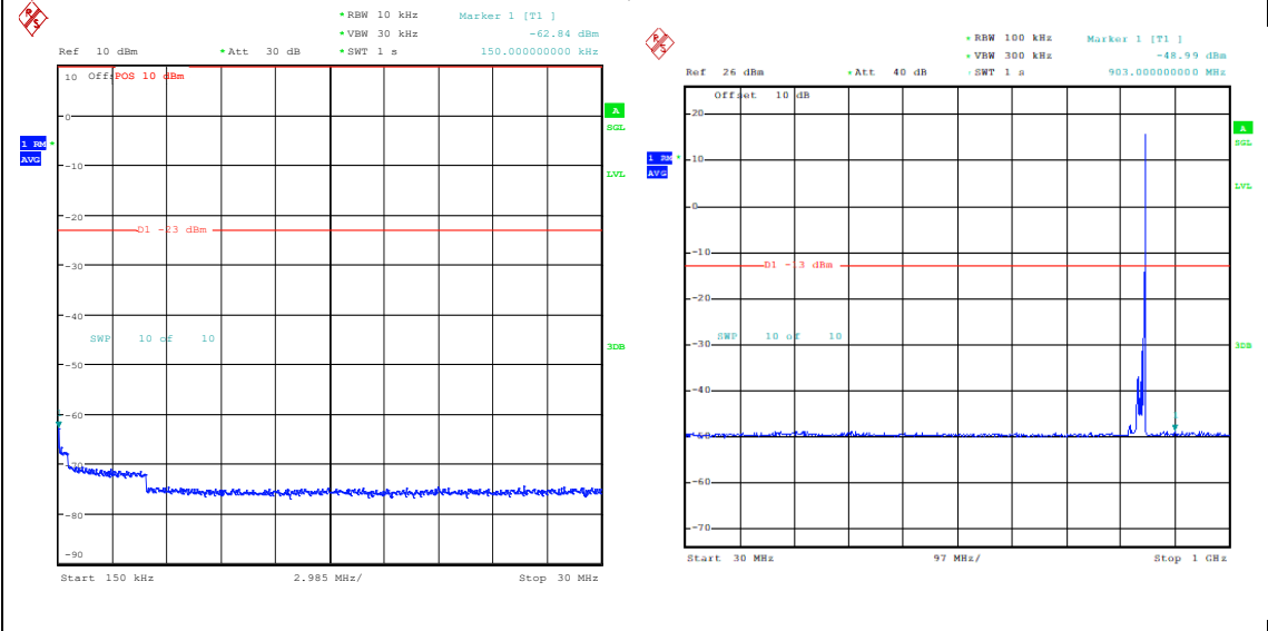
Band26_15MHz_16QAM_26965_1RB#74_0.15~30_0.15~30 Band26_15MHz_16QAM_26965_1RB#74_30~1000_0_30~1000
