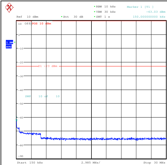
Band26_15MHz_16QAM_26915_1RB#74_0.15~30_0.15~30
