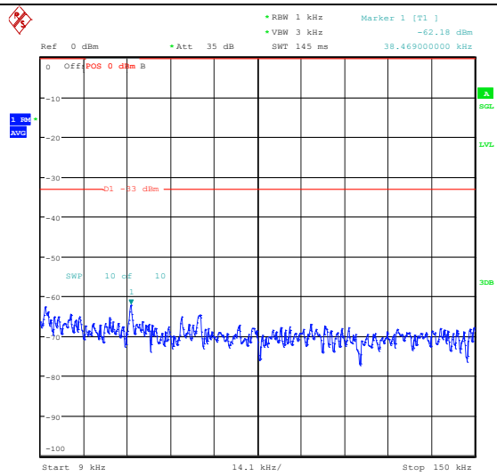
Band26_10MHz_16QAM_26840_1RB#0_0.009~0.15_0.009~0.15
