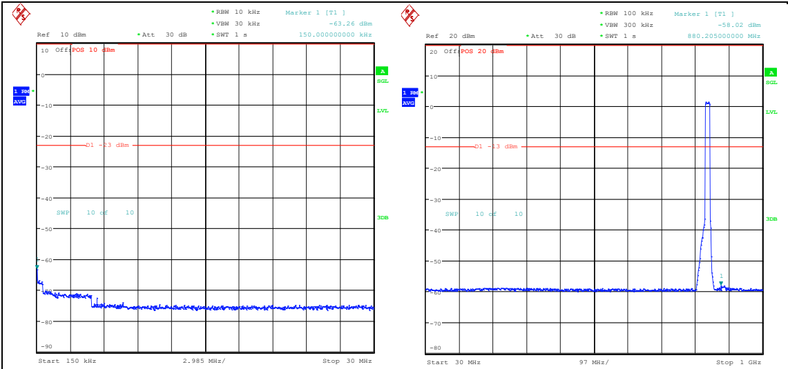
Band26_15MHz_16QAM_26965_75RB#0_0.15~30_0.15~30
