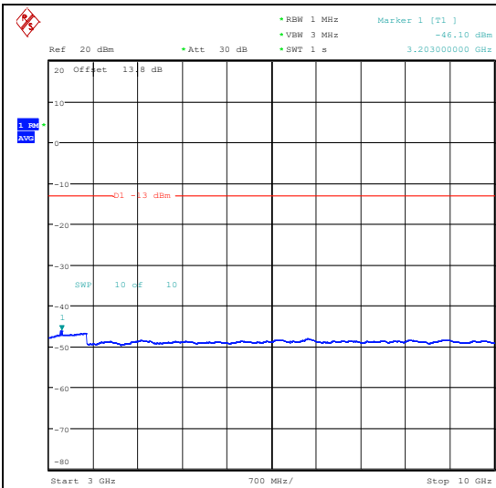
Band26_10MHz_QPSK_26840_1RB#0_3000~10000_3000~10000
