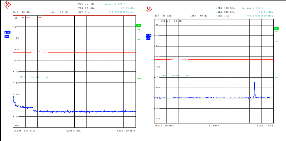
Band26_5MHz_16QAM_27015_1RB#24_0.15~30_0.15~30 Band26_5MHz_16QAM_27015_1RB#24_30~1000_30~1000
