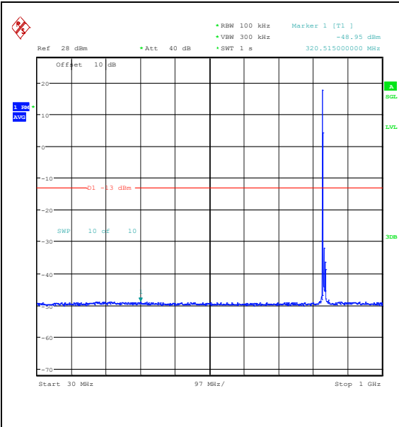
Band26_10MHz_QPSK_26915_1RB#0_30~1000_30~1000
