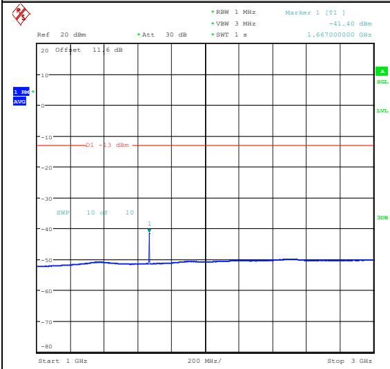
Band26_10MHz_16QAM_26840_1RB#49_0.15~30_0.15~30
