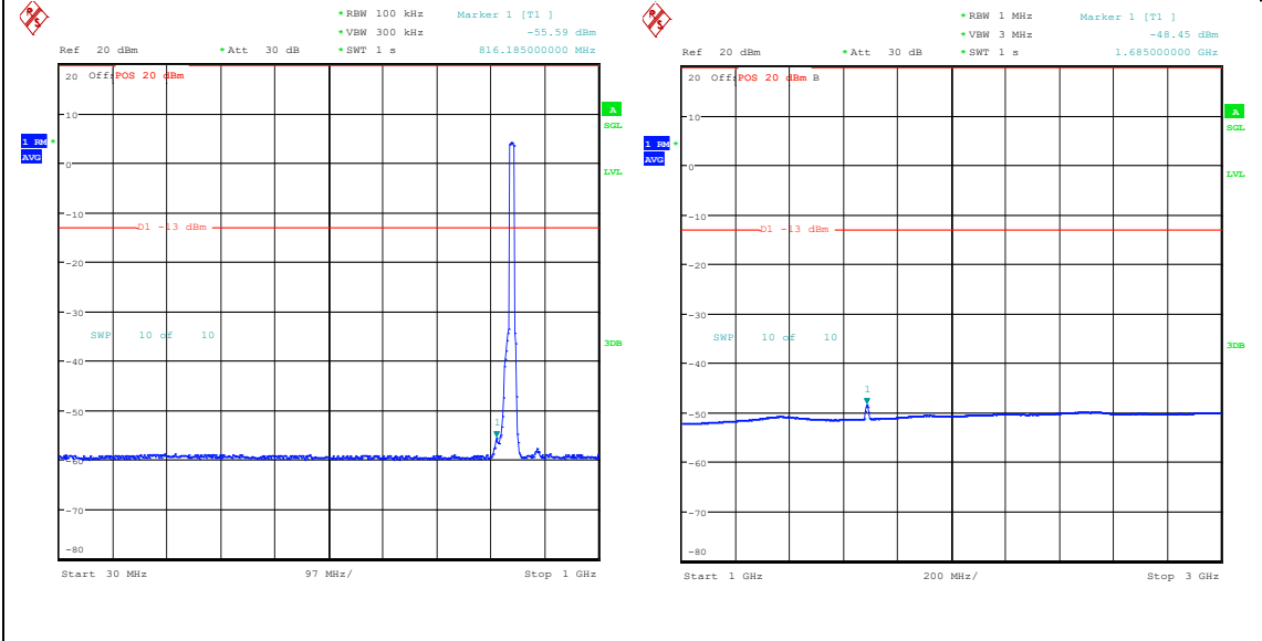
Band26_10MHz_QPSK_26990_50RB#0_30~1000_0_30~1000 Band26_10MHz_QPSK_26990_50RB#0_1000~3000_00_1000~3000
