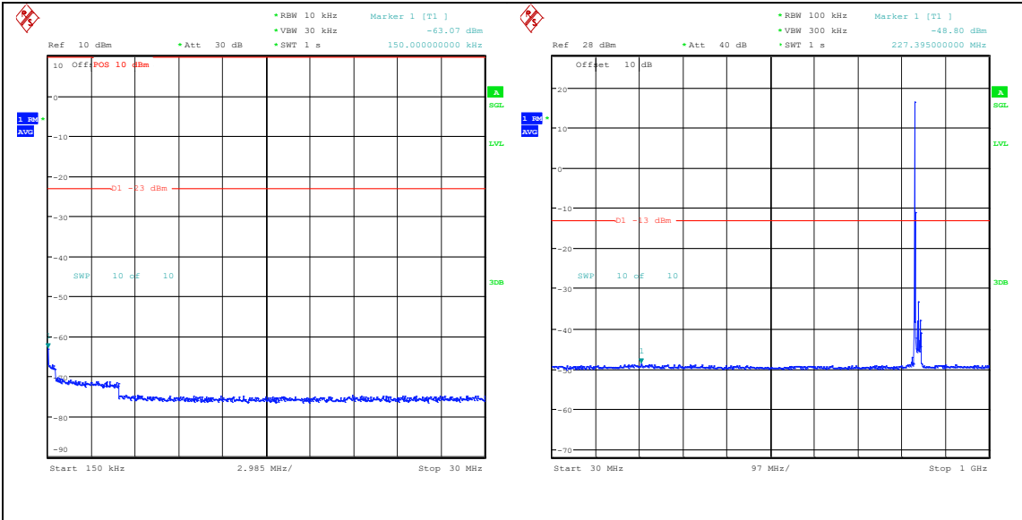
Band26_15MHz_16QAM_26965_1RB#0_0.15~300.15~30 Band26_15MHz_16QAM_26965_1RB#0_30~100030~1000
