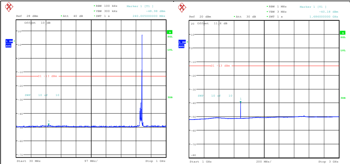
Band26_15MHz_QPSK_26915_1RB#74_30~100 0_30~1000 Band26_15MHz_QPSK_26915_1RB#74_1000~30 00_1000~3000
