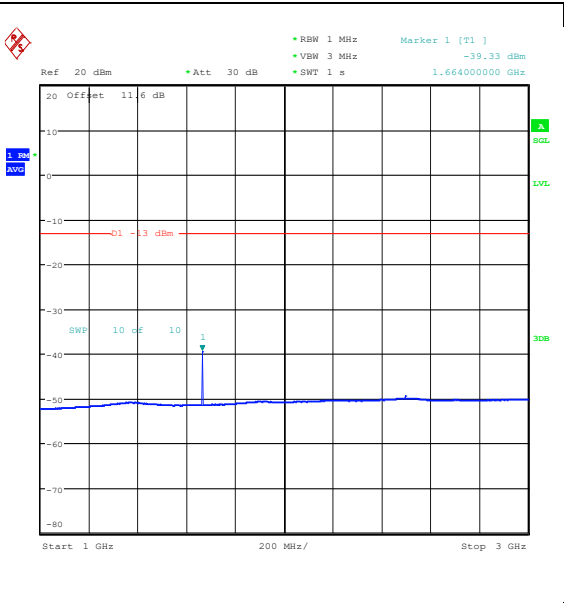
Band26_10MHz_QPSK_26915_1RB#0_1000~300_0_1000~3000
