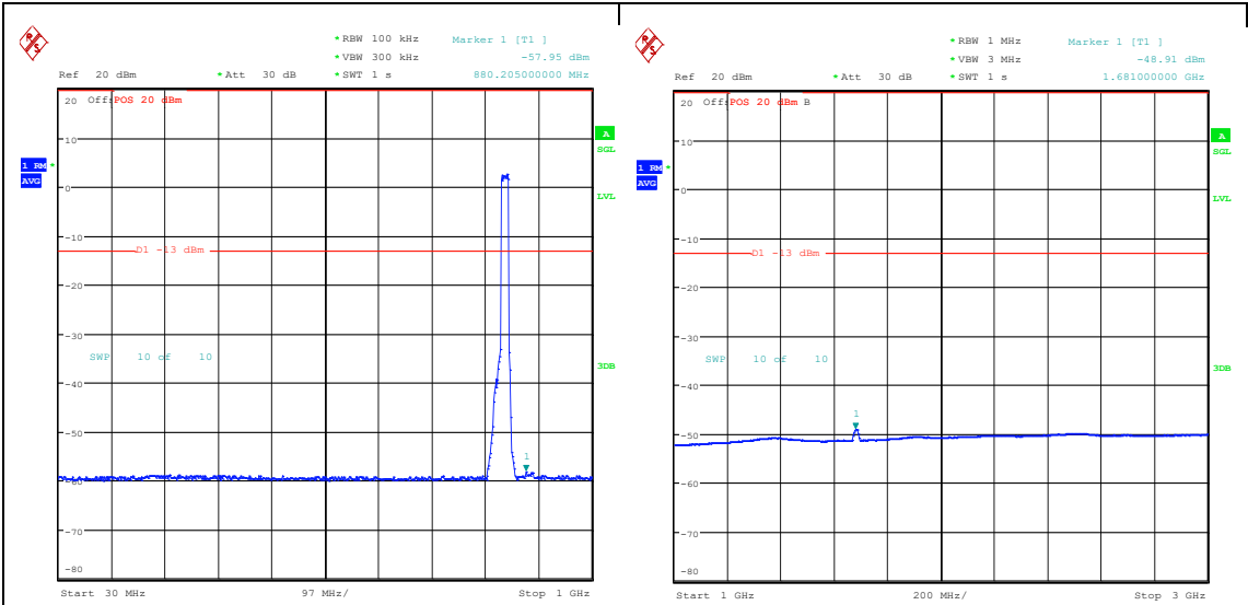
Band26_15MHz_QPSK_26965_75RB#0_30~100 0_30~1000 Band26_15MHz_QPSK_26965_75RB#0_1000~30 00_1000~3000
