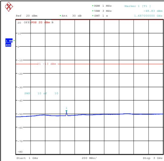
Band26_10MHz_16QAM_26990_50RB#0_1000~3000_1000~3000
