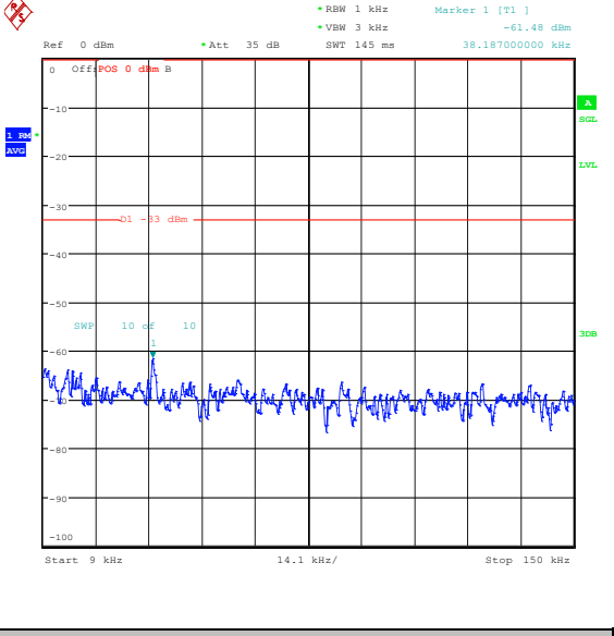
Band26_3MHz_16QAM_26775_1RB#14_0.009~0.15_0.009~0.15
