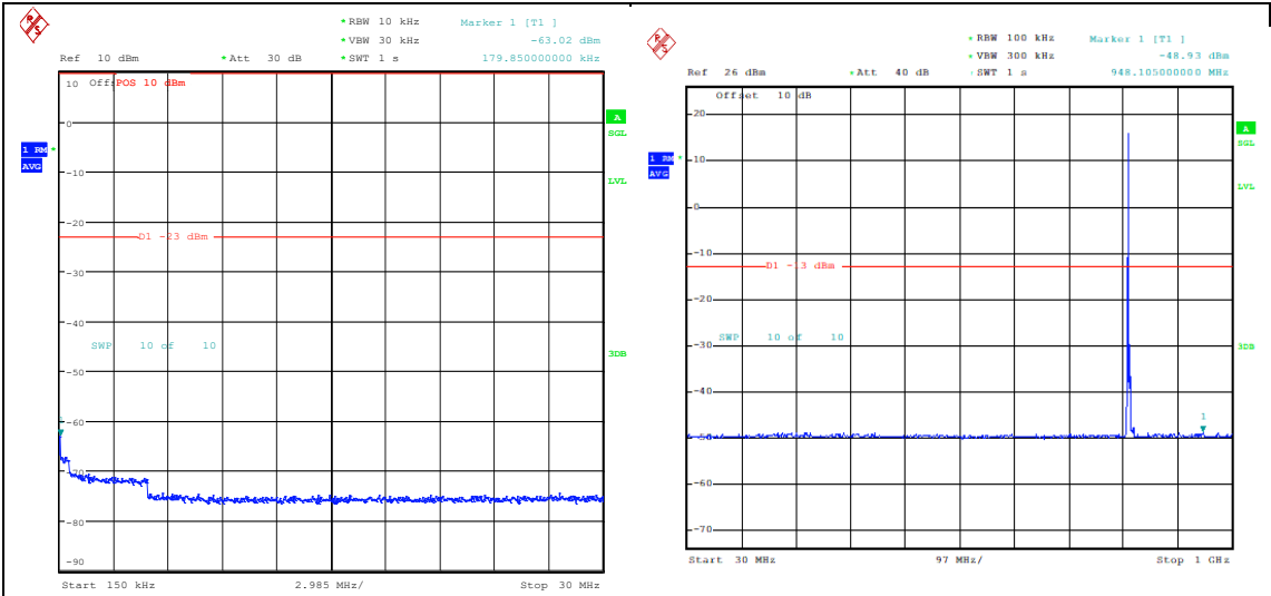
Band26_5MHz_16QAM_26715_1RB#0_0.15~30 _0.15~30
