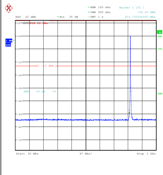
Band26_3MHz_QPSK_26775_15RB#0_30~1000_30~1000
