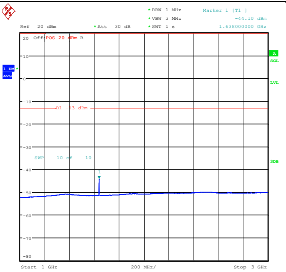
Band26_3MHz_QPSK_26740_15RB#0_1000~3000_0_1000~3000
