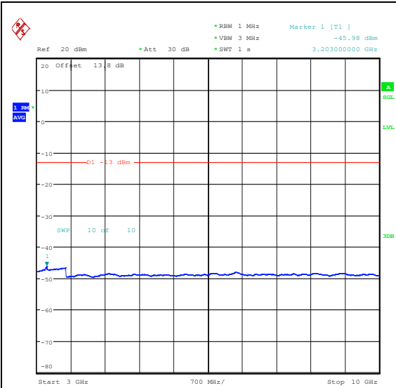
Band26_1.4MHz_QPSK_26783_1RB#5_3000~10000_3000~10000
