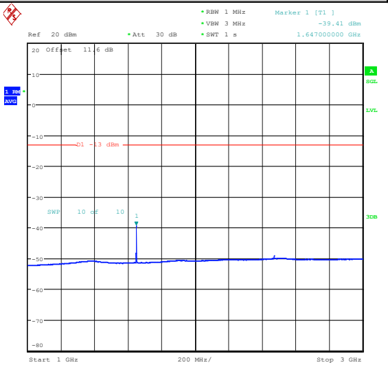
Band26_1.4MHz_QPSK_26783_1RB#5_1000~3000_00_1000~3000
