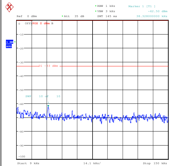
Band26_5MHz_16QAM_26740_25RB#0_1000~3000_1000~3000
