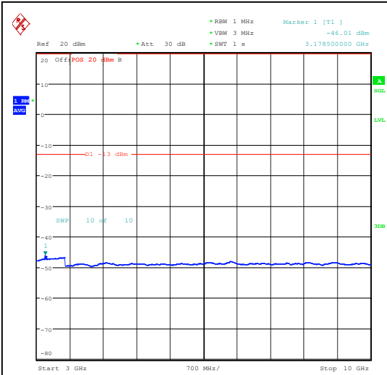
Band26_3MHz_QPSK_26775_15RB#0_3000~10000_3000~10000
