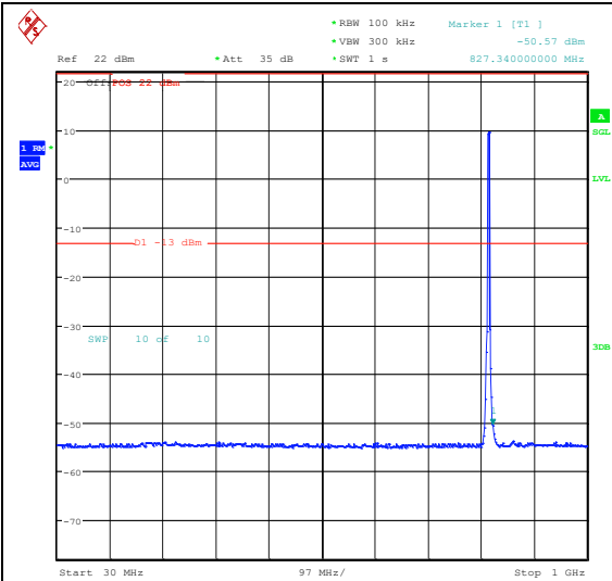
Band26_3MHz_QPSK_26740_15RB#0_30~1000_30~1000
