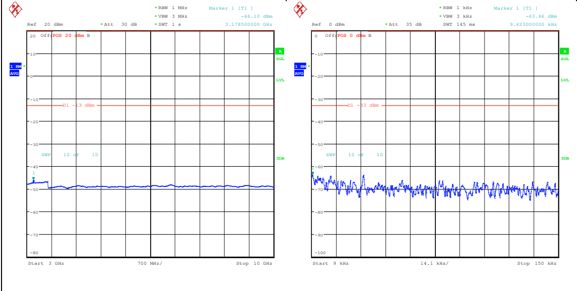
Band26_5MHz_QPSK_26765_25RB#0_3000~10000_000_3000~10000 Band26_5MHz_16QAM_26765_25RB#0_0.009~0.15_0.009~0.15
