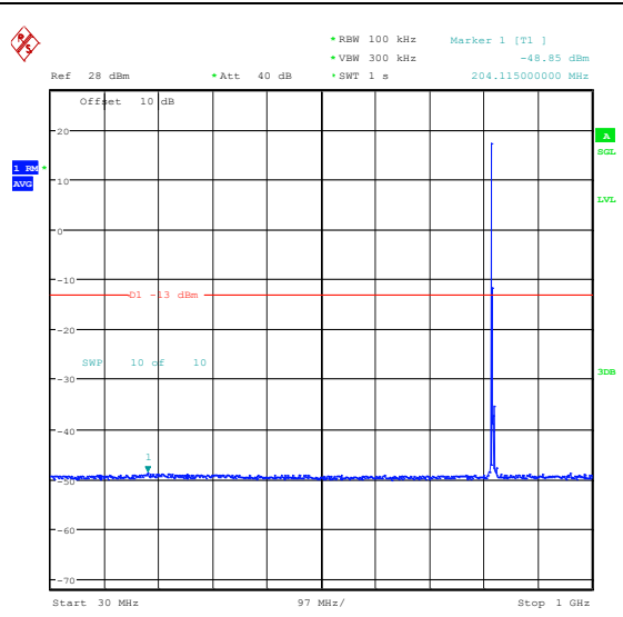
Band26_5MHz_16QAM_26765_1RB#0_30~1000_30~1000
