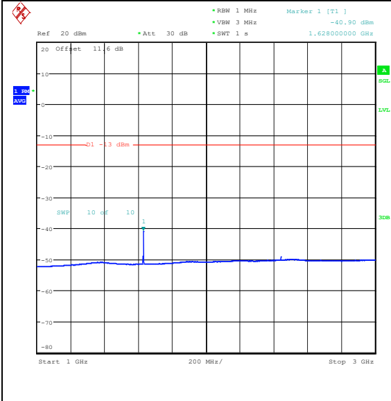
Band26_1.4MHz_16QAM_26697_1RB#0_1000~3000_1000~3000
