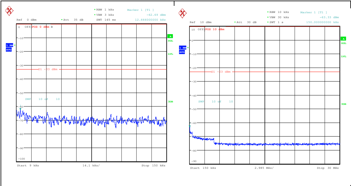
Band26_3MHz_QPSK_26705_15RB#0_0.009~0.15_0.009~0.15 Band26_3MHz_QPSK_26705_15RB#0_0.15~30_0.15~30
