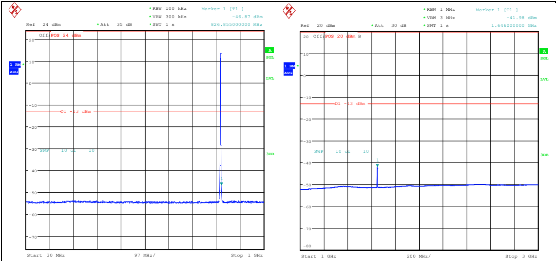
Band26_1.4MHz_QPSK_26783_6RB#0_30~1000_30~1000 Band26_1.4MHz_QPSK_26783_6RB#0_1000~3000_1000~3000
