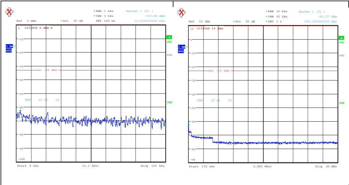
Band26_1.4MHz_QPSK_26697_1RB#5_0.009~0.15_0.009~0.15 Band26_1.4MHz_QPSK_26697_1RB#5_0.15~30_0.15~30
