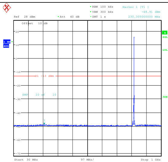
Band26_5MHz_16QAM_26740_1RB#24_0.15~30_0.15~30 Band26_5MHz_16QAM_26740_1RB#24_30~1000_30~1000
