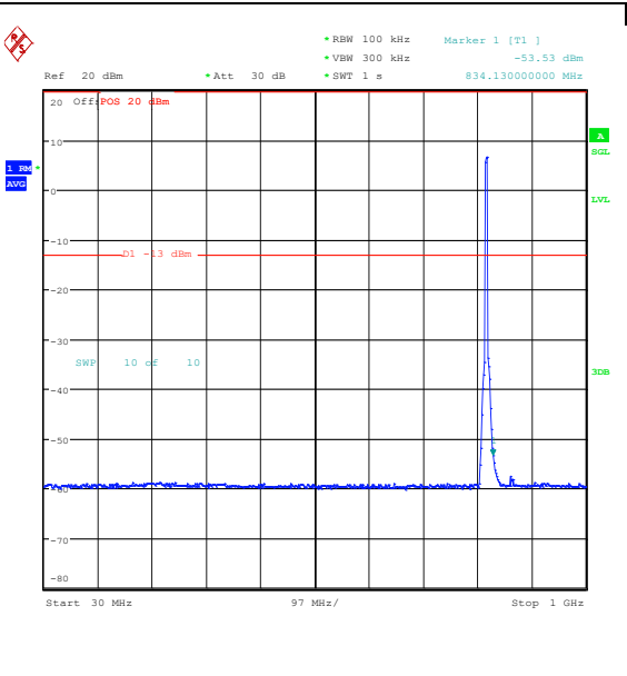
Band26_5MHz_16QAM_26765_25RB#0_30~1000 _30~1000
