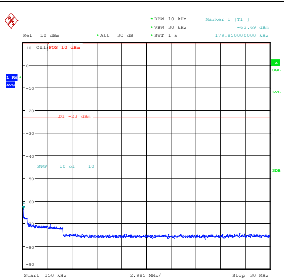
Band26_5MHz_QPSK_26740_25RB#0_0.15~30_0.15~30
