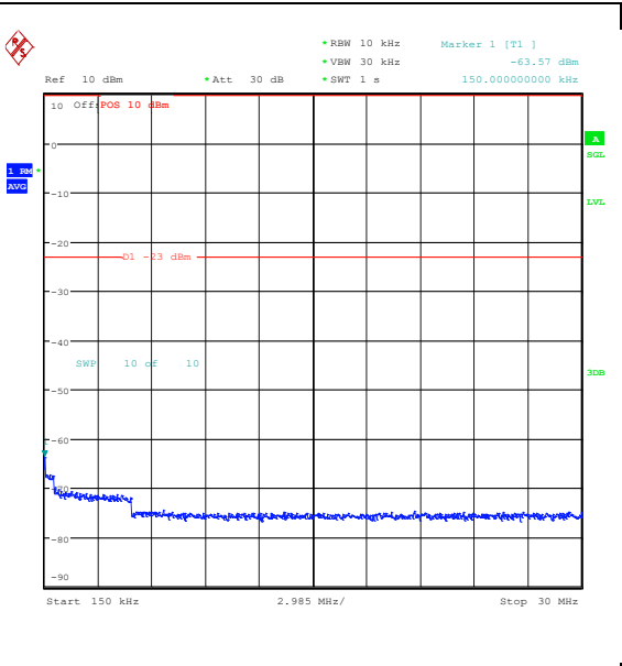
Band26_1.4MHz_QPSK_26783_1RB#5_0.15~30_0.15~30
