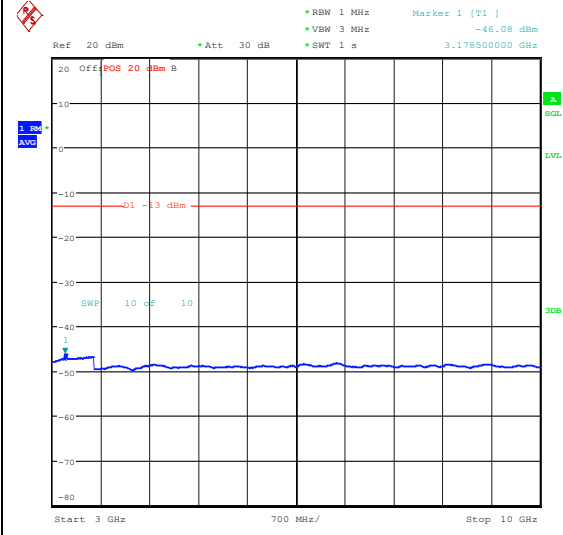
Band26_3MHz_QPSK_26740_15RB#0_3000~10000_000_3000~10000
