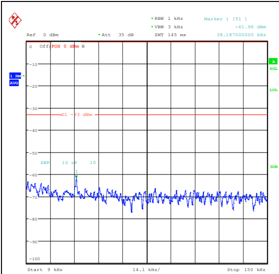
Band26_3MHz_QPSK_26705_1RB#0_0.009~0.15 5_0.009~0.15
