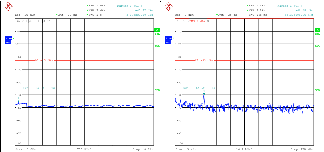
Band26_5MHz_QPSK_26765_1RB#24_3000~10000_3000~10000 Band26_5MHz_16QAM_26765_1RB#24_0.009~0.15_0.009~0.15
