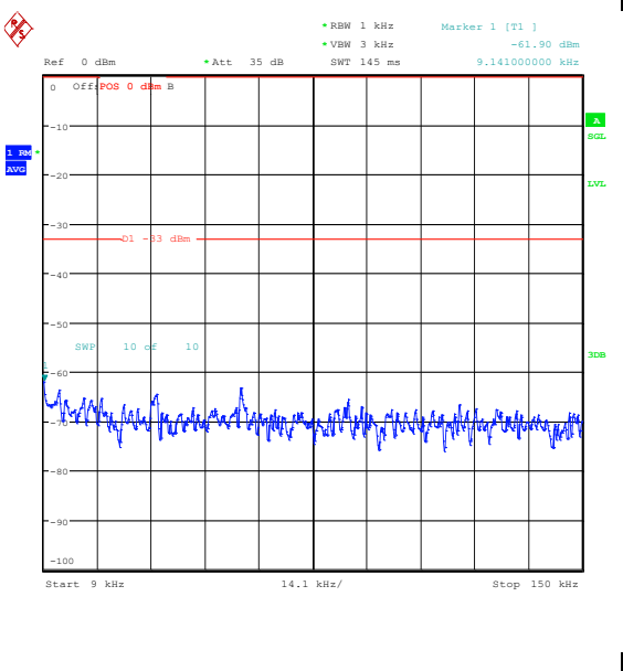
Band26_5MHz_16QAM_26715_25RB#0_0.009~0.15_0.009~0.15
