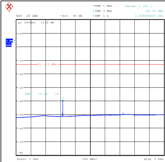
Band26_3MHz_16QAM_26705_1RB#0_1000~3000_00_1000~3000
