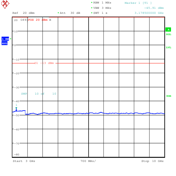
Band26_5MHz_16QAM_26765_25RB#0_3000~10 000_3000~10000
