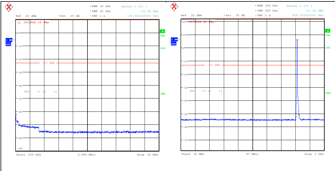
Band26_5MHz_16QAM_26715_25RB#0_0.15~3 0_0.15~30
