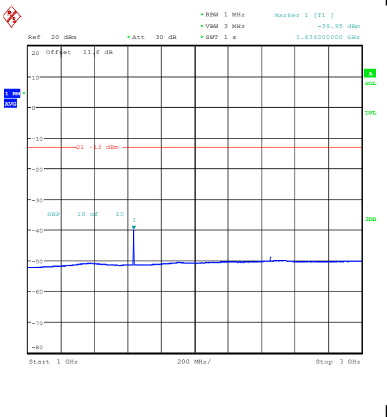
Band26_5MHz_QPSK_26740_1RB#0_1000~3000_1000~3000
