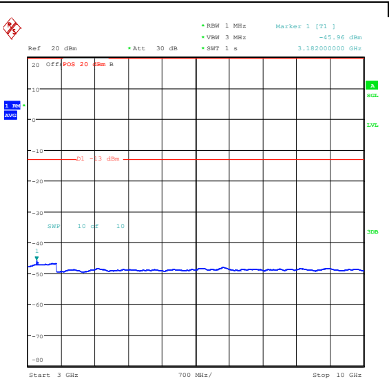
Band26_3MHz_16QAM_26705_15RB#0_1000~3000_1000~3000 Band26_3MHz_16QAM_26705_15RB#0_3000~10000_3000~10000
