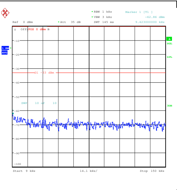
Band26_5MHz_16QAM_26740_25RB#0_0.009~0.15_0.009~0.15
