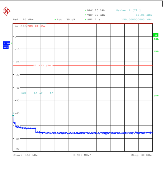
Band26_3MHz_QPSK_26775_1RB#0_0.15~30_0. 15~30
