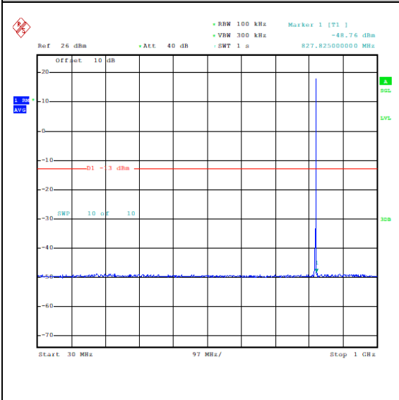
Band26_1.4MHz_QPSK_26783_1RB#5_30~1000_30~1000
