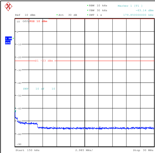
Band26_1.4MHz_16QAM_26740_1RB#5_0.15~3 0_0.15~30
