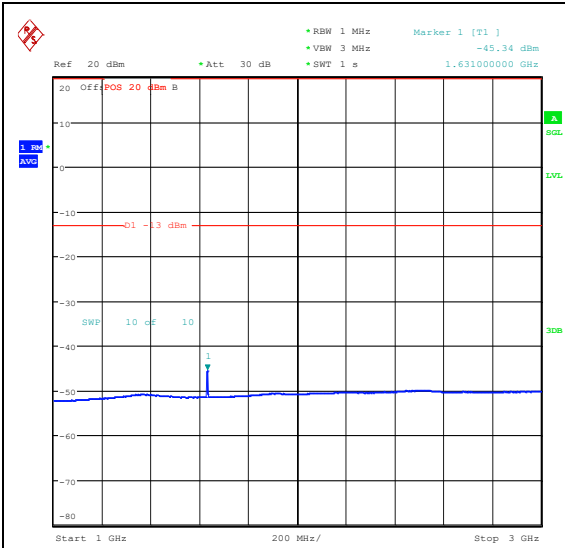
Band26_3MHz_16QAM_26705_15RB#0_1000~3000_1000~3000 Band26_3MHz_16QAM_26705_15RB#0_3000~10000_3000~10000
