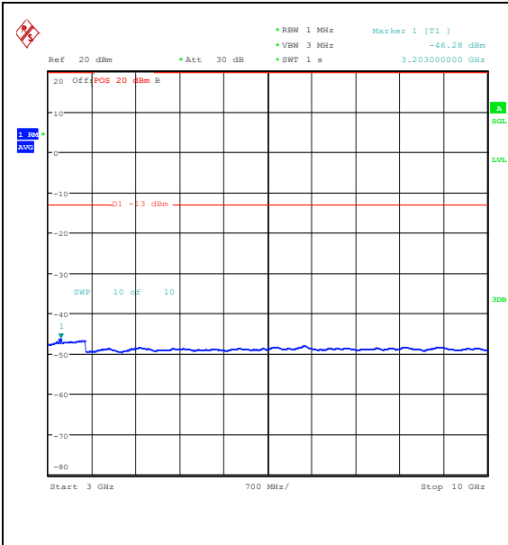
Band26_5MHz_QPSK_26740_25RB#0_3000~10000_3000~10000
