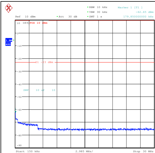
Band26_3MHz_16QAM_26740_15RB#0_0.15~30_0.15~30
