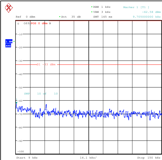
Band26_3MHz_QPSK_26740_1RB#14_0.009~0.15_0.009~0.15
