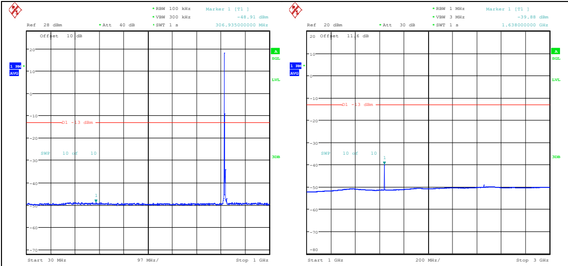
Band26_5MHz_QPSK_26765_1RB#0_30~1000_30~1000 Band26_5MHz_QPSK_26765_1RB#0_1000~3000_1000~3000
