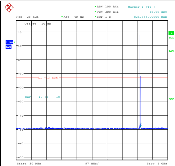
Band26_1.4MHz_QPSK_26783_1RB#0_30~1000_30~1000
