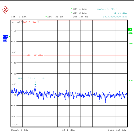
Band26_3MHz_16QAM_26775_15RB#0_0.009~0.15_0.009~0.15
