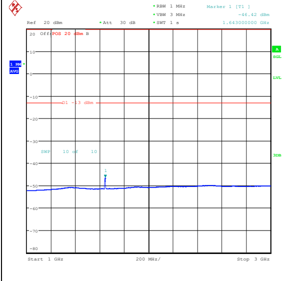
Band26_5MHz_16QAM_26765_25RB#0_1000~3 000_1000~3000
