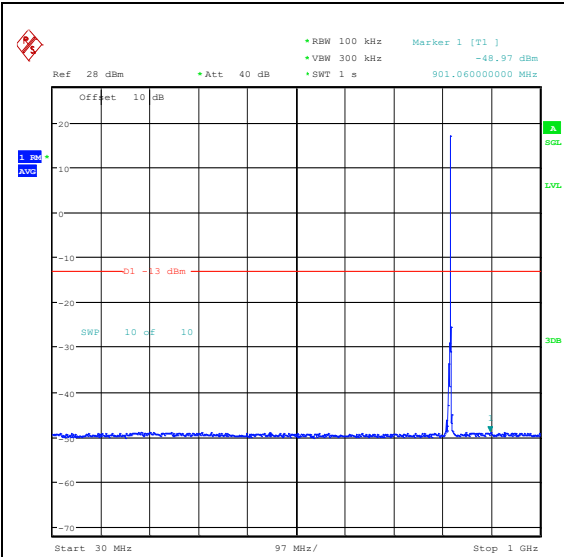
Band26_5MHz_QPSK_26740_1RB#24_30~1000_30~1000
