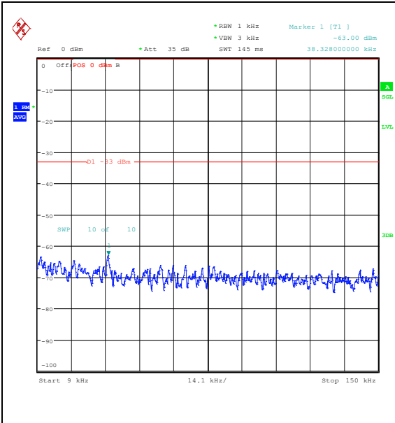
Band26_3MHz_QPSK_26775_1RB#0_0.009~0.15 5_0.009~0.15
