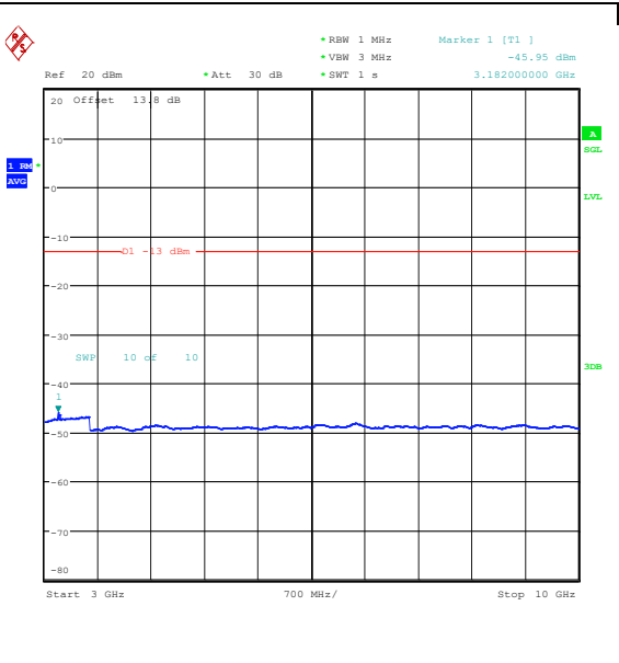
Band26_5MHz_16QAM_26715_1RB#24_3000~10000_3000~10000
