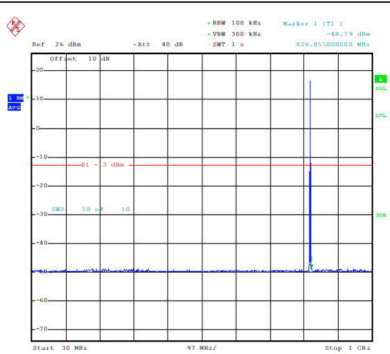
Band26_1.4MHz_16QAM_26783_1RB#0_30~1000 0_30~1000
