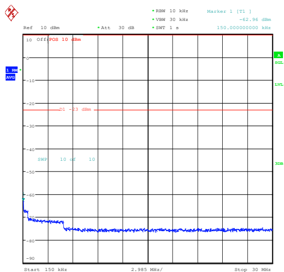
Band26_5MHz_QPSK_26765_1RB#24_0.15~30_0.15~30
