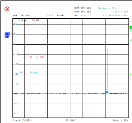
Band26_1.4MHz_QPSK_26740_1RB#5_30~1000_30~1000
