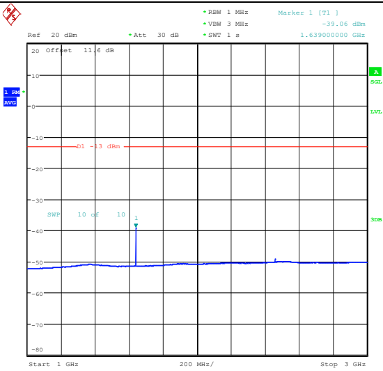
Band26_1.4MHz_QPSK_26740_1RB#5_1000~3000_00_1000~3000
