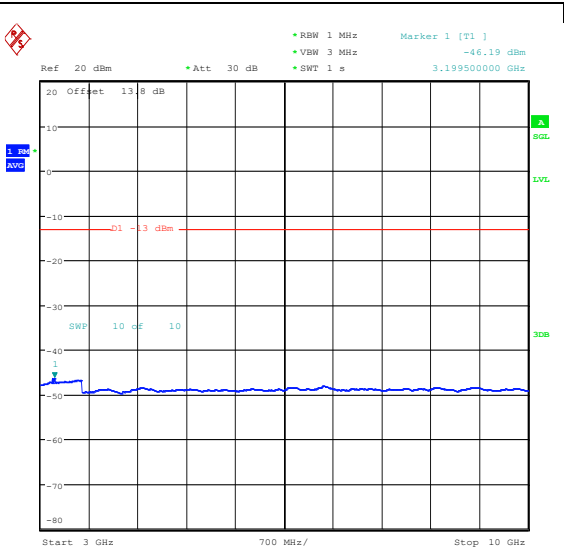
Band26_3MHz_16QAM_26775_1RB#0_3000~10000_00_3000~10000
