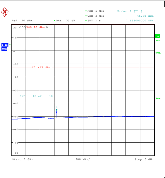
Band26_5MHz_QPSK_26715_25RB#0_1000~300_0_1000~3000
