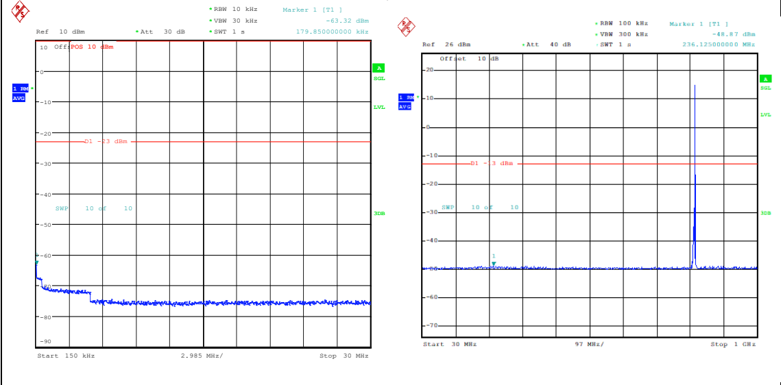
Band26_5MHz_16QAM_26715_1RB#24_0.15~30_0.15~30 Band26_5MHz_16QAM_26715_1RB#24_30~1000_30~1000
