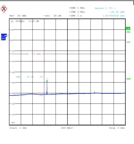
Band26_3MHz_QPSK_26775_1RB#14_1000~300_0_1000~3000
