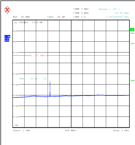
Band26_5MHz_16QAM_26715_1RB#24_1000~3000_1000~3000
