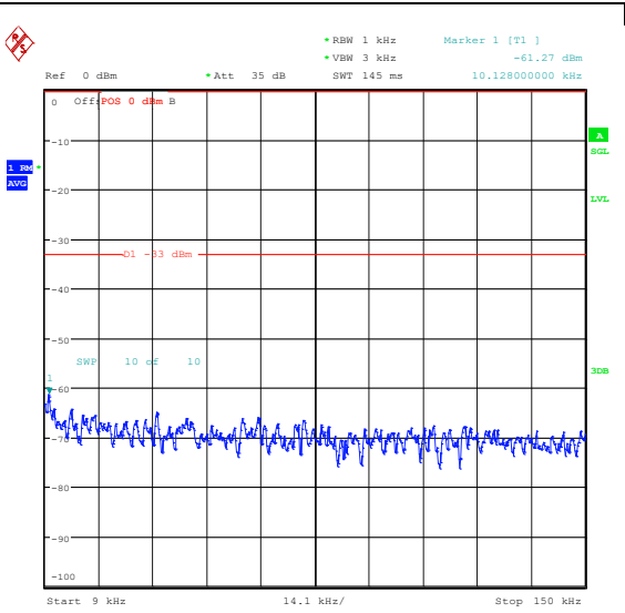
Band26_1.4MHz_16QAM_26783_1RB#5_0.009~0.15_0.009~0.15
