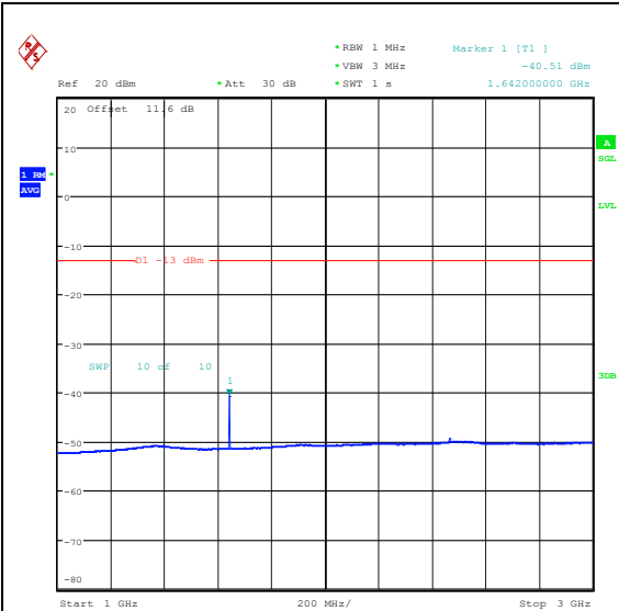
Band26_3MHz_16QAM_26775_1RB#0_1000~3000_00_1000~3000
