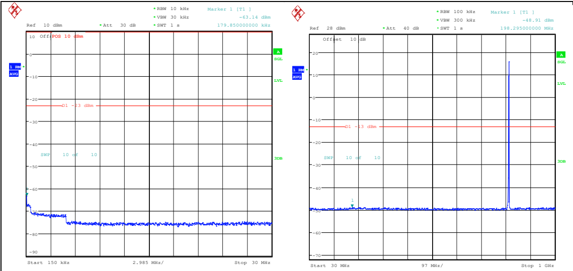
Band26_3MHz_16QAM_26705_1RB#14_0.15~30_0.15~30 Band26_3MHz_16QAM_26705_1RB#14_30~1000_30~1000
