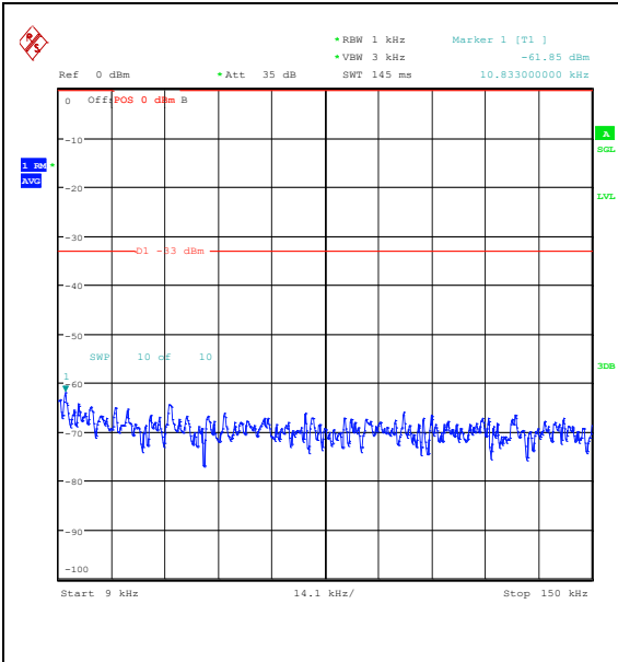
Band26_1.4MHz_QPSK_26783_1RB#5_0.009~0.15_0.009~0.15
