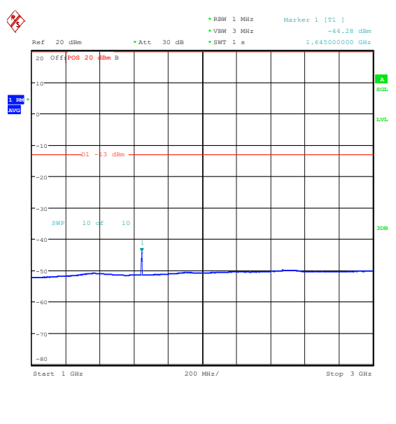
Band26_3MHz_QPSK_26775_15RB#0_1000~3000_0_1000~3000
