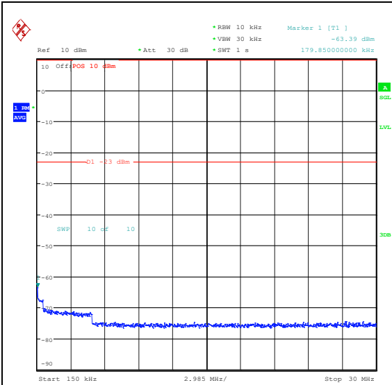
Band26_5MHz_16QAM_26765_1RB#0_0.15~30_0.15~30
