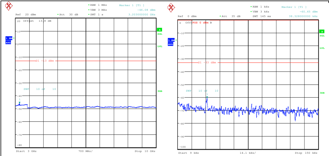
Band26_5MHz_QPSK_26740_1RB#0_3000~10000_3000~10000 Band26_5MHz_16QAM_26740_1RB#0_0.009~0.15_0.009~0.15
