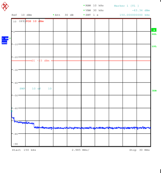
Band26_5MHz_QPSK_26715_25RB#0_0.15~30_0.15~30
