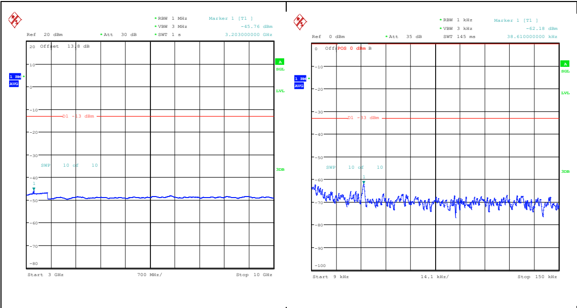
Band26_5MHz_QPSK_26715_1RB#24_3000~10000_3000~10000 Band26_5MHz_16QAM_26715_1RB#24_0.009~0.15_0.009~0.15
