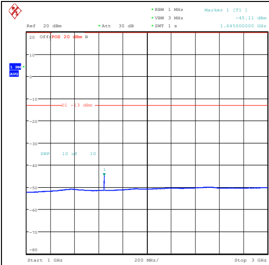
Band26_3MHz_16QAM_26775_15RB#0_1000~3000_1000~3000
