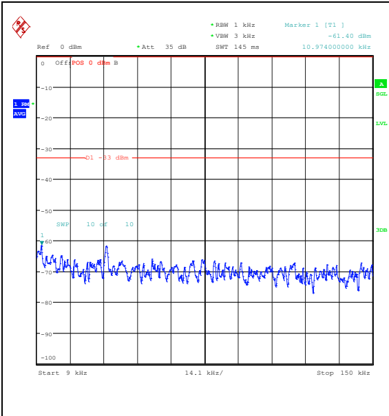
Band26_3MHz_QPSK_26775_15RB#0_0.009~0.15_0.009~0.15
