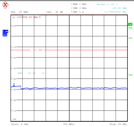
Band26_3MHz_16QAM_26775_15RB#0_3000~10000_3000~10000
