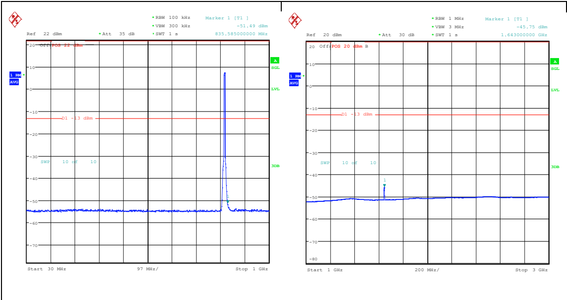
Band26_5MHz_QPSK_26765_25RB#0_30~1000_30~1000 Band26_5MHz_QPSK_26765_25RB#0_1000~3000_0_1000~3000
