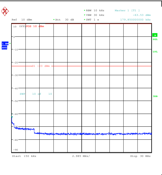
Band26_5MHz_QPSK_26740_1RB#0_0.15~30_0.15~30
