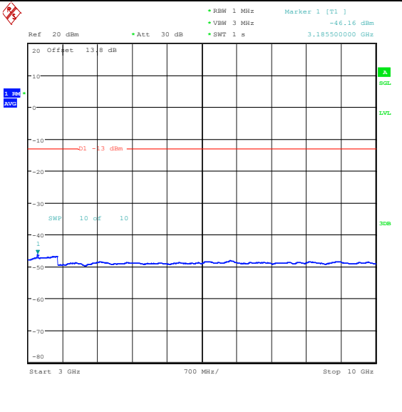
Band26_1.4MHz_16QAM_26697_1RB#0_3000~10000_3000~10000
