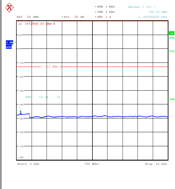
Band26_5MHz_QPSK_26715_25RB#0_3000~10_000_3000~10000
