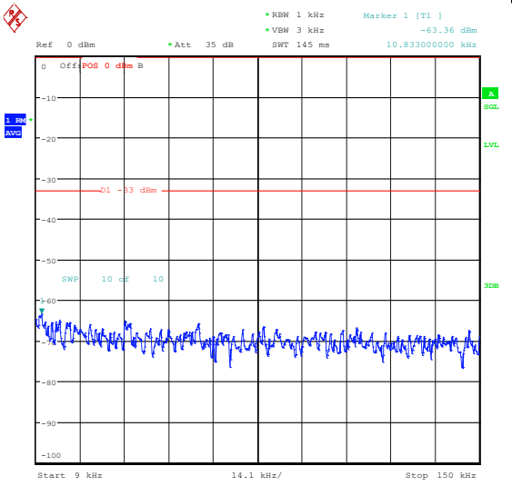
Band26_3MHz_16QAM_26740_15RB#0_0.009~0.15_0.009~0.15
