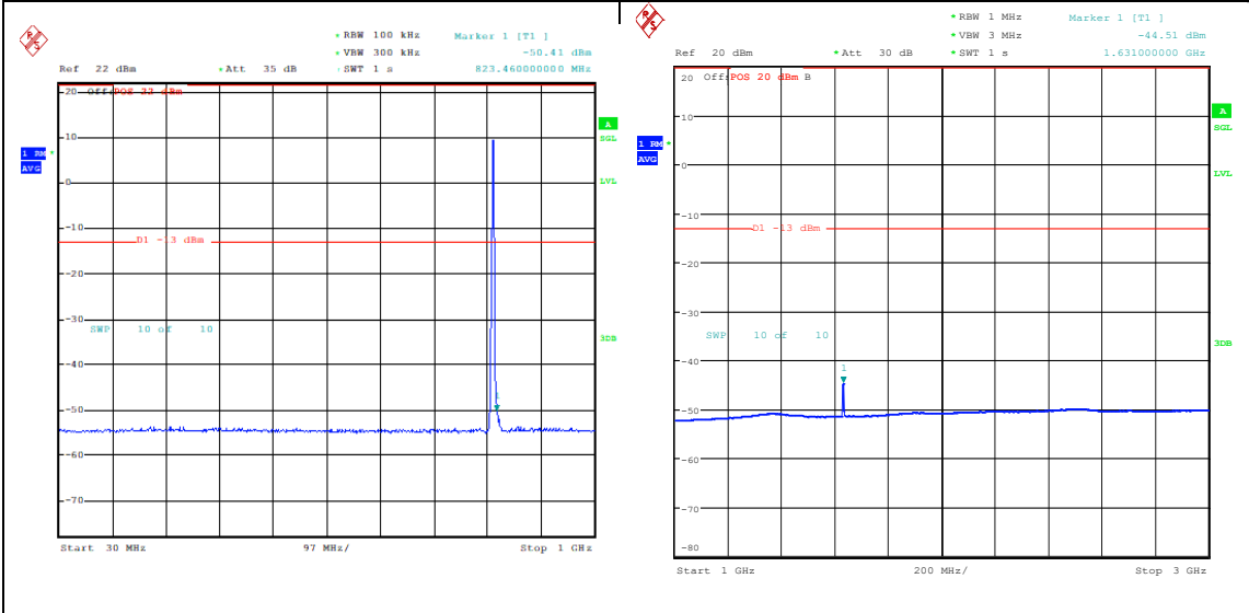
Band26_3MHz_QPSK_26705_15RB#0_30~1000_30~1000 Band26_3MHz_QPSK_26705_15RB#0_1000~3000_0_1000~3000
