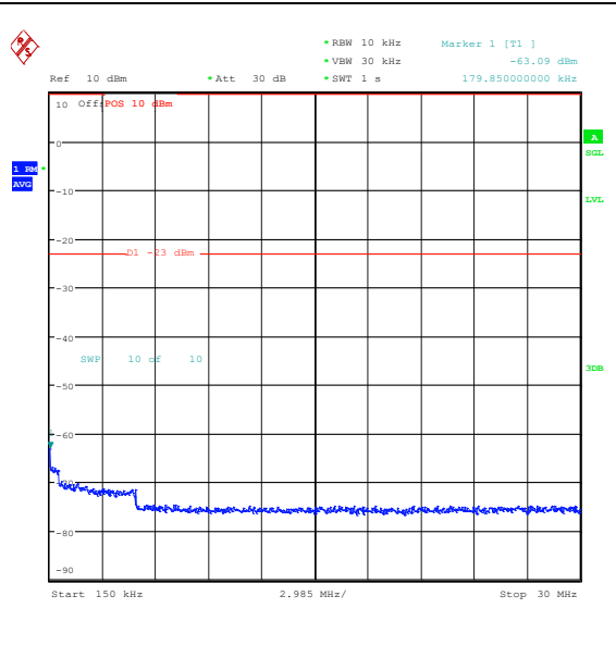
Band26_3MHz_QPSK_26775_15RB#0_0.15~30_0.15~30
