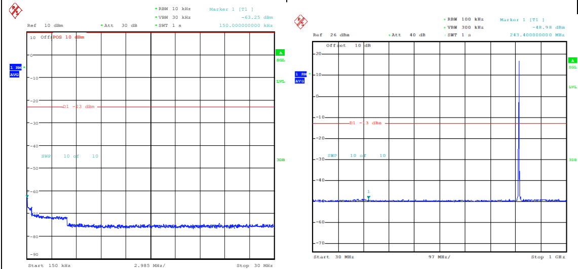
Band26_5MHz_16QAM_26740_1RB#0_0.15~30_0.15~30 Band26_5MHz_16QAM_26740_1RB#0_30~1000_30~1000
