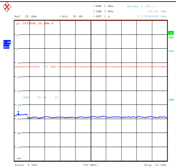
Band26_5MHz_16QAM_26740_25RB#0_3000~10000_3000~10000
