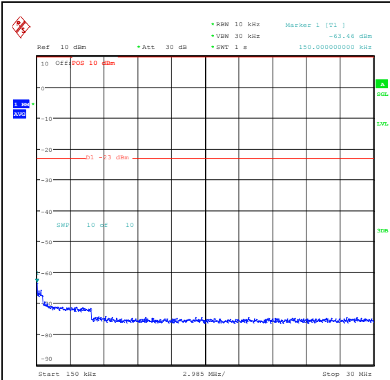
Band26_1.4MHz_16QAM_26697_6RB#0_0.15~3 0_0.15~30
