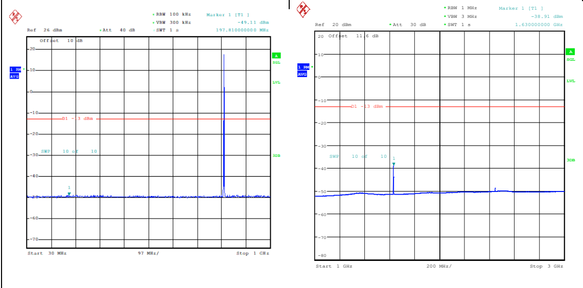
Band26_1.4MHz_QPSK_26697_1RB#5_30~1000_30~1000 Band26_1.4MHz_QPSK_26697_1RB#5_1000~3000_00_1000~3000
