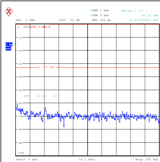
Band26_5MHz_QPSK_26740_25RB#0_0.009~0.15_0.009~0.15
