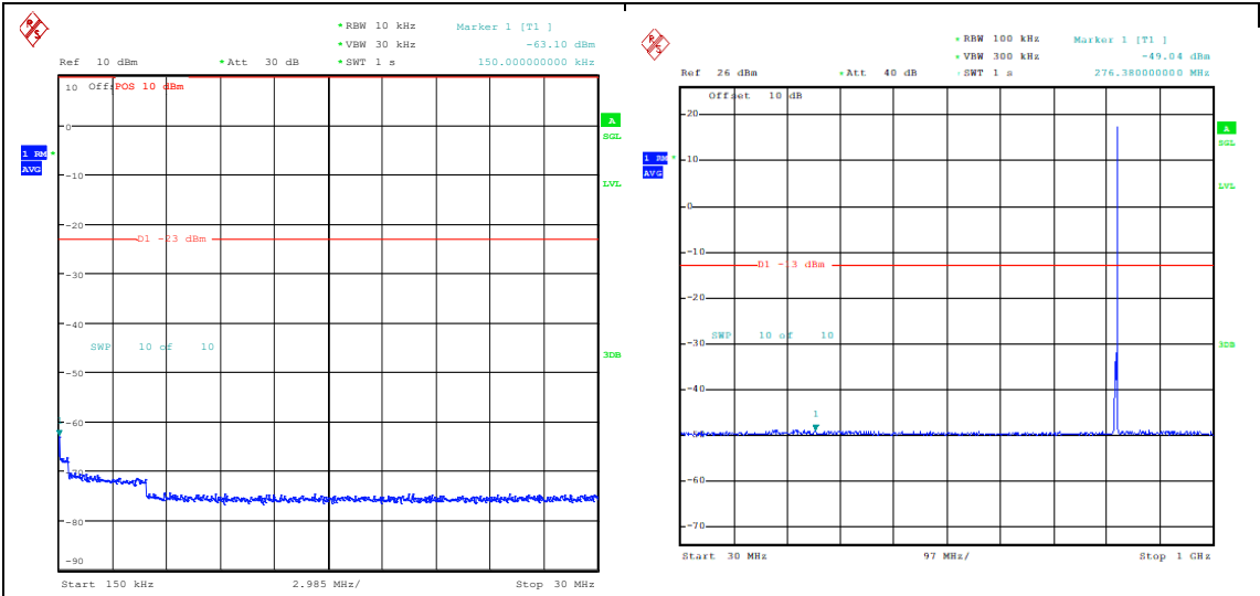
Band26_3MHz_16QAM_26775_1RB#14_0.15~3 0_0.15~30
