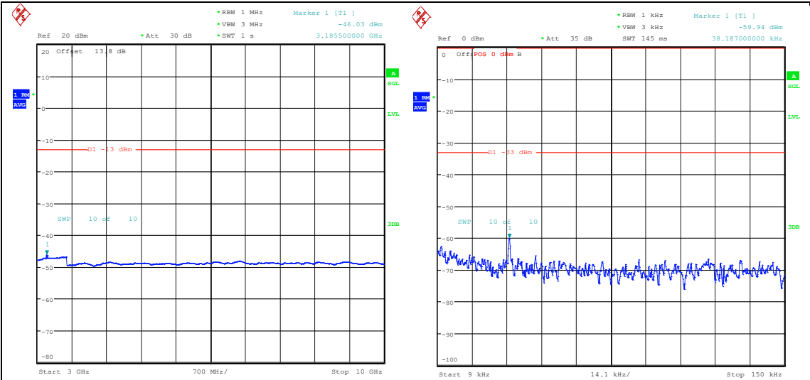
Band26_3MHz_QPSK_26705_1RB#0_3000~10000_3000~10000 Band26_3MHz_16QAM_26705_1RB#0_0.009~0.15_0.009~0.15
