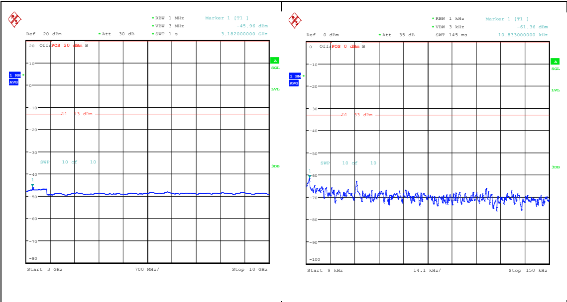
Band26_3MHz_QPSK_26705_15RB#0_3000~10000_3000~10000 Band26_3MHz_16QAM_26705_15RB#0_0.009~0.15_0.009~0.15
