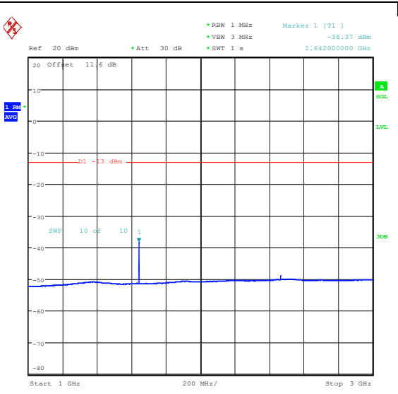
Band26_5MHz_QPSK_26740_1RB#24_1000~300_0_1000~3000
