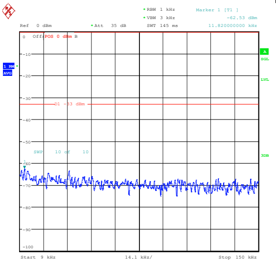
Band26_5MHz_QPSK_26740_1RB#24_1000~300_0_1000~3000
