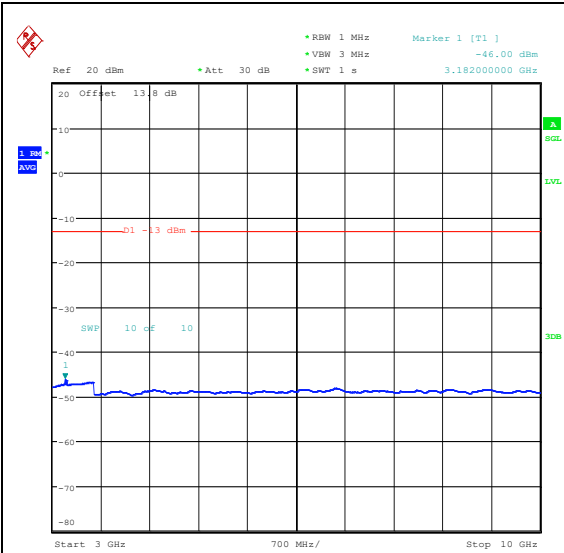
Band26_1.4MHz_QPSK_26740_1RB#0_3000~10000_3000~10000 Band26_1.4MHz_16QAM_26740_1RB#0_0.009~0.15_0.009~0.15
