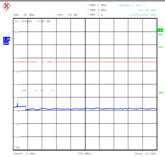
Band26_3MHz_16QAM_26705_1RB#0_3000~10000_00_3000~10000
