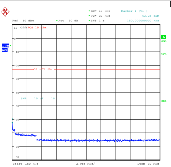
Band26_3MHz_QPSK_26705_1RB#0_0.15~30_0. 15~30
