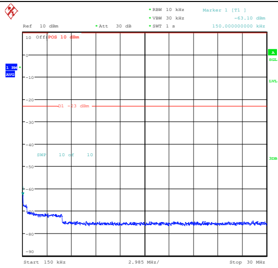
Band26_3MHz_QPSK_26740_1RB#14_0.15~30_0.15~30
