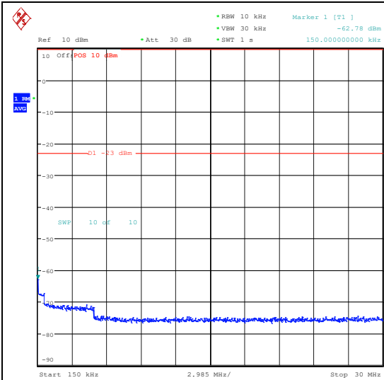
Band26_1.4MHz_16QAM_26783_1RB#0_0.15~30 0_0.15~30
