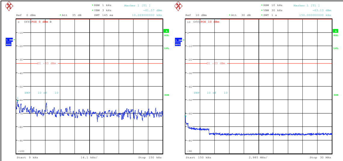
Band26_1.4MHz_QPSK_26740_1RB#0_0.009~0.15_0.009~0.15 Band26_1.4MHz_QPSK_26740_1RB#0_0.15~30_0.15~30
