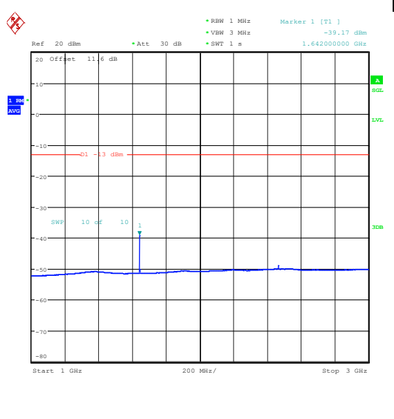
Band26_3MHz_QPSK_26775_1RB#0_1000~3000 _1000~3000
