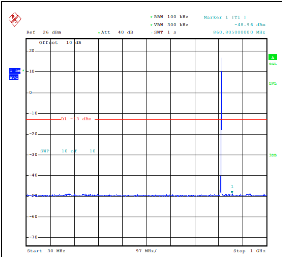
Band26_3MHz_QPSK_26705_1RB#14_30~1000_30~1000
