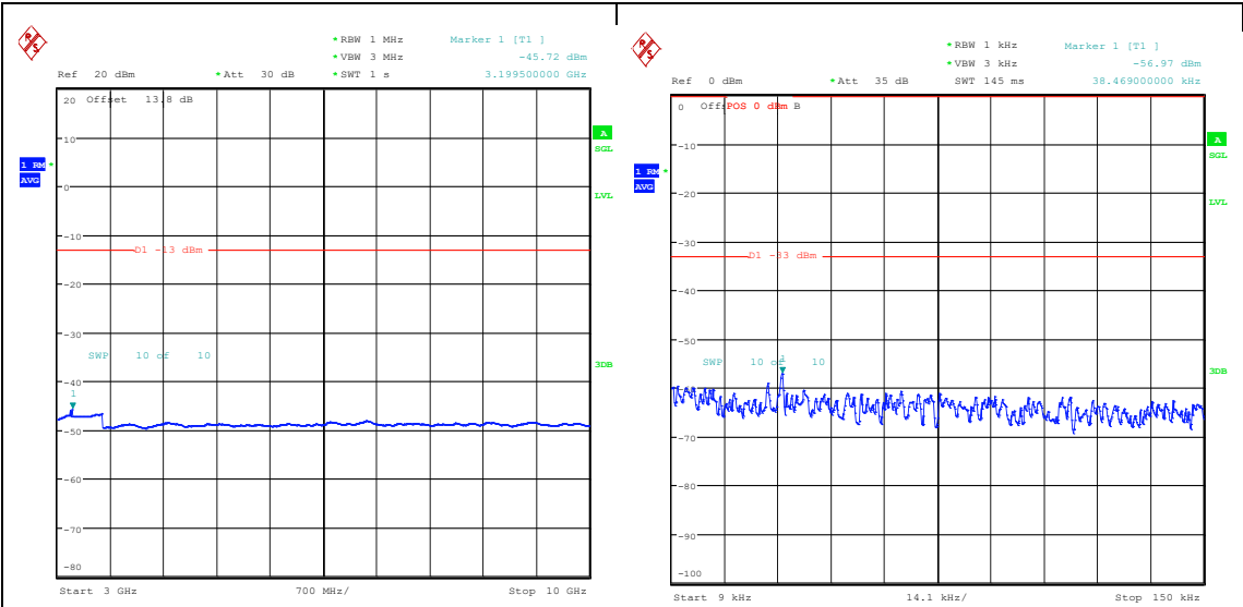
Band5_1.4MHz_QPSK_20643_1RB#5_3000~10000_3000~10000 Band5_1.4MHz_16QAM_20643_1RB#5_0.009~0.15_0.009~0.15
