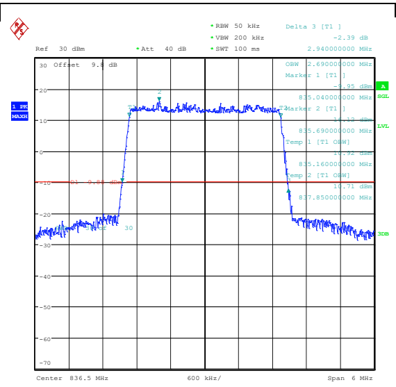
Band5-3MHz-16QAM-20525-15RB#0-PASS
