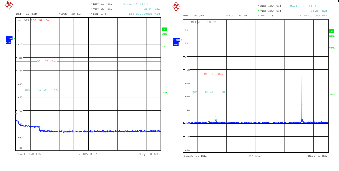
Band5_3MHz_16QAM_20415_1RB#0_0.15~30 0.15~30 Band5_3MHz_16QAM_20415_1RB#0_30~1000_3 0~1000
