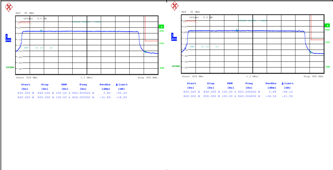
Band5_10MHz_QPSK_20600_50RB#0
