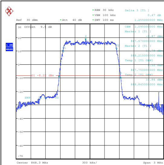
Band5-1.4MHz-QPSK-20643-6RB#0-PASS
