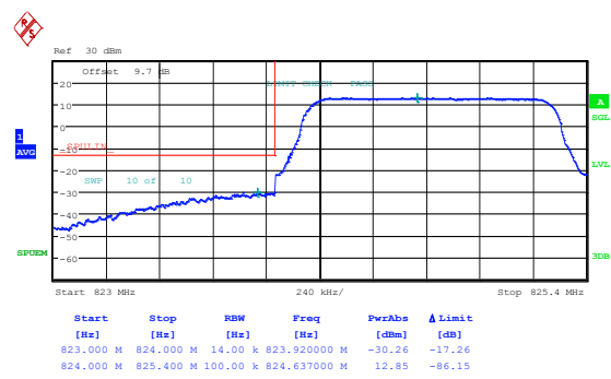
Band5_1.4MHz_16QAM_20407_1RB#5
