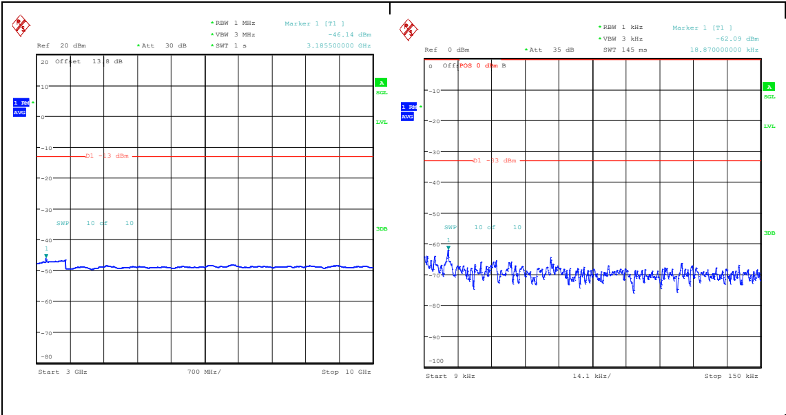
Band5_3MHz_QPSK_20415_1RB#0_3000~1000 0_3000~10000 Band5_3MHz_16QAM_20415_1RB#0_0.009~0.15 _0.009~0.15
