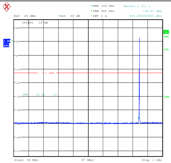
Band5_1.4MHz_16QAM_20643_6RB#0_30~1000_30~1000
