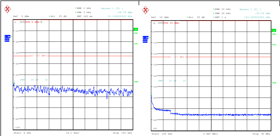
Band5_1.4MHz_QPSK_20407_1RB#5_0.009~0.15 5_0.009~0.15 Band5_1.4MHz_QPSK_20407_1RB#5_0.15~30_0.15~30
