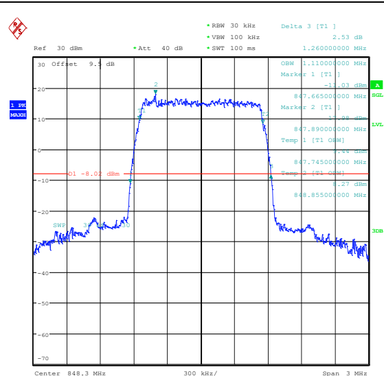
Band5-1.4MHz-16QAM-20643-6RB#0-PASS
