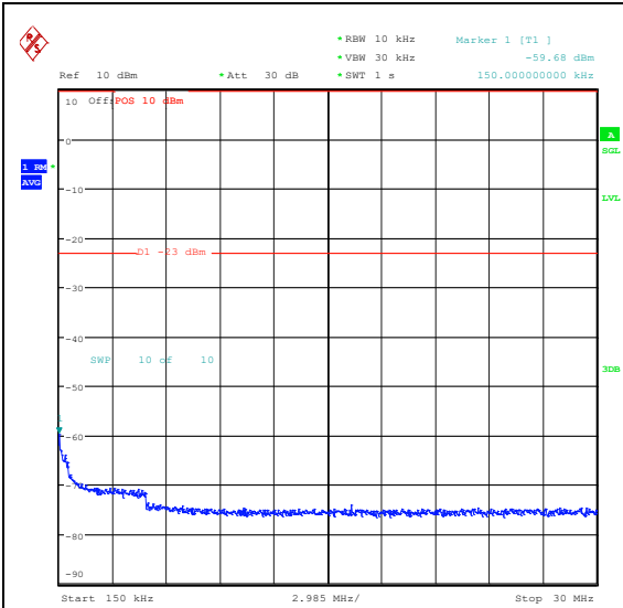
Band5_1.4MHz_16QAM_20407_6RB#0_0.15~30_0.15~30 Band5_1.4MHz_16QAM_20407_6RB#0_30~1000_30~1000
