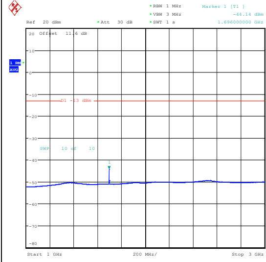
Band5_1.4MHz_16QAM_20643_6RB#0_1000~3000_1000~3000
