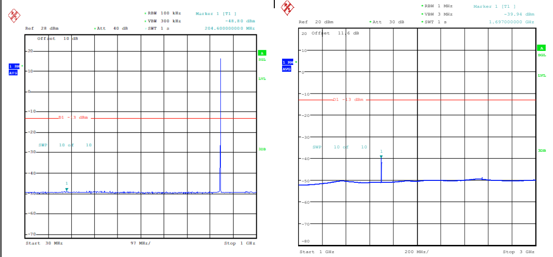
Band5_1.4MHz_QPSK_20643_1RB#5_30~1000_30~1000 Band5_1.4MHz_QPSK_20643_1RB#5_1000~3000_0_1000~3000
