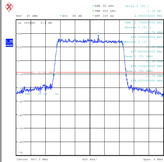
Band5-3MHz-QPSK-20525-15RB#0-PASS
