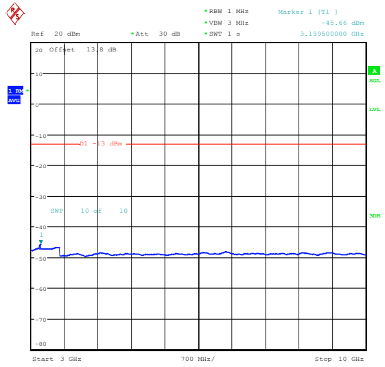
Band5_1.4MHz_16QAM_20643_6RB#0_3000~10000_3000~10000
