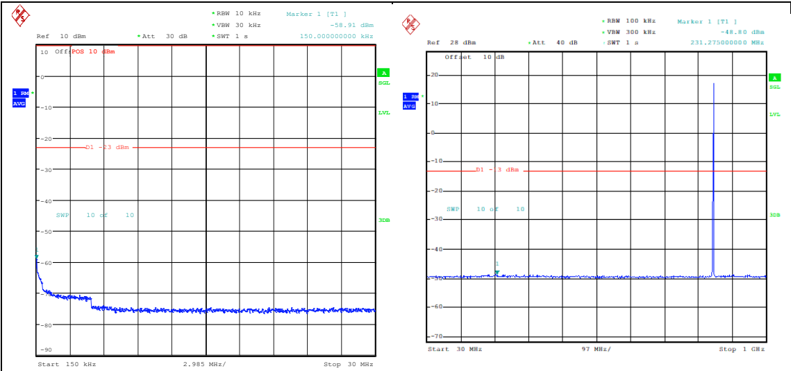
Band5_1.4MHz_16QAM_20643_1RB#0_0.15~30_0.15~30 Band5_1.4MHz_16QAM_20643_1RB#0_30~1000_30~1000
