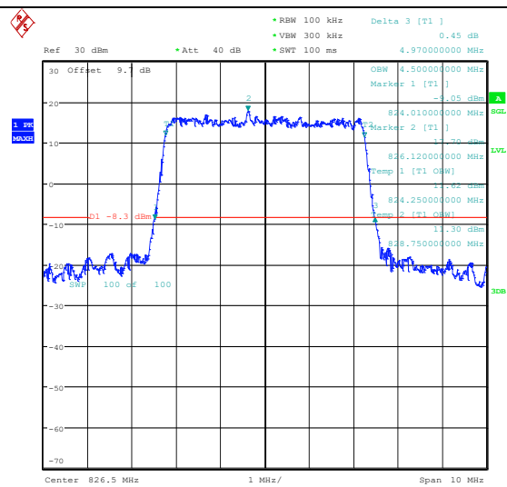
Band5-5MHz-16QAM-20425-25RB#0-PASS
