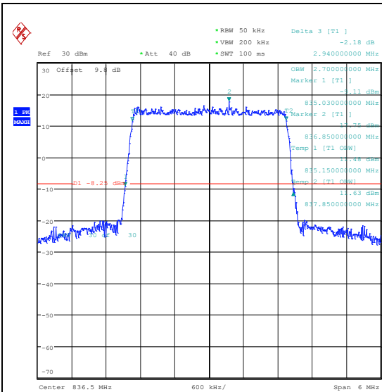
Band5-3MHz-QPSK-20525-15RB#0-PASS
