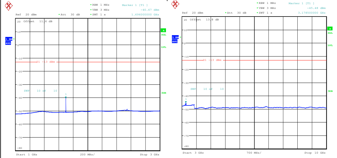
Band5_1.4MHz_16QAM_20643_1RB#0_1000~3000_1000~3000 Band5_1.4MHz_16QAM_20643_1RB#0_3000~10000_3000~10000
