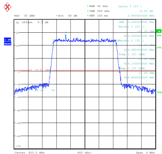
Band5-1.4MHz-16QAM-20643-6RB#0-PASS
