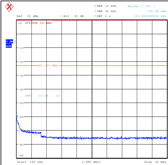
Band5_1.4MHz_16QAM_20643_6RB#0_0.15~30_0.15~30
