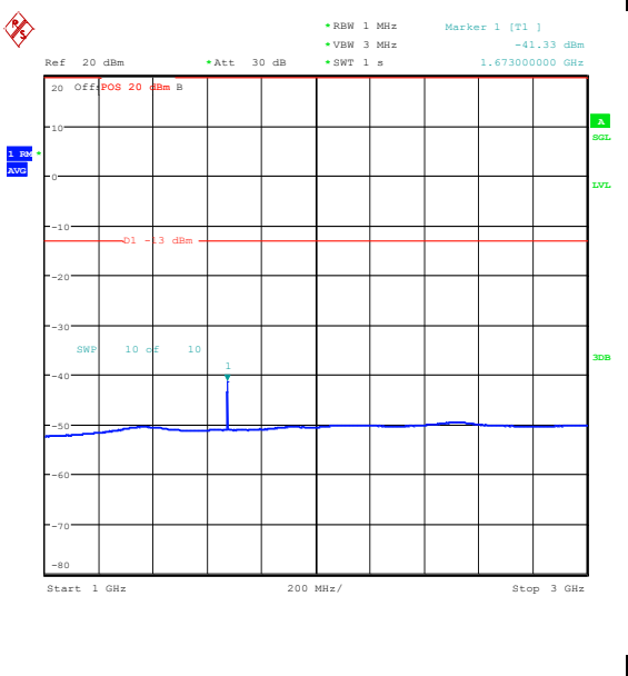
Band5_1.4MHz_QPSK_20525_6RB#0_1000~3000_0_1000~3000
