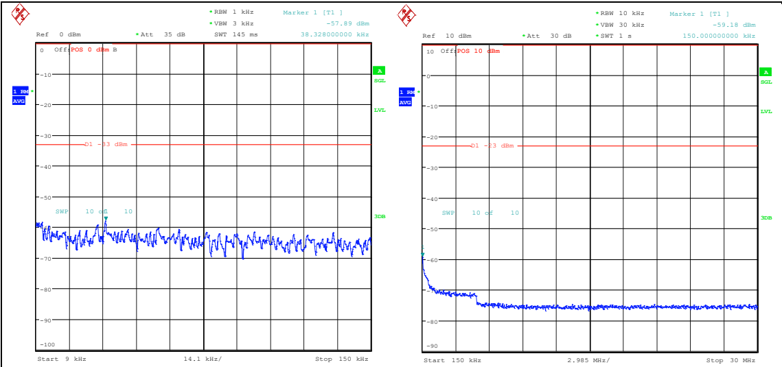
Band5_1.4MHz_QPSK_20643_1RB#5_0.009~0.15 5_0.009~0.15 Band5_1.4MHz_QPSK_20643_1RB#5_0.15~30_0.15~30
