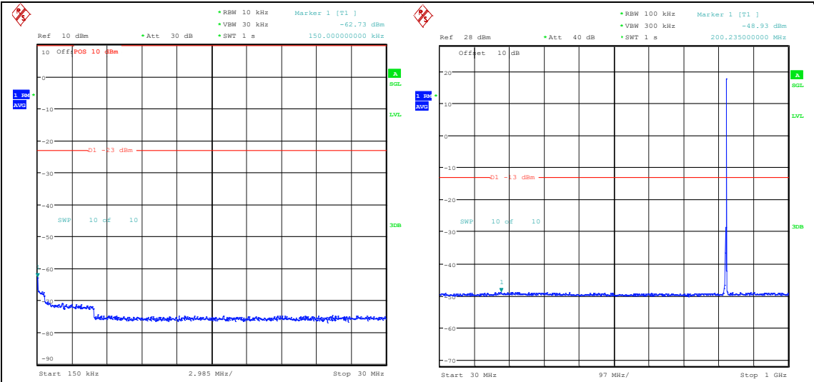
Band5_3MHz_16QAM_20415_1RB#14_0.15~30_0.15~30 Band5_3MHz_16QAM_20415_1RB#14_30~1000_30~1000
