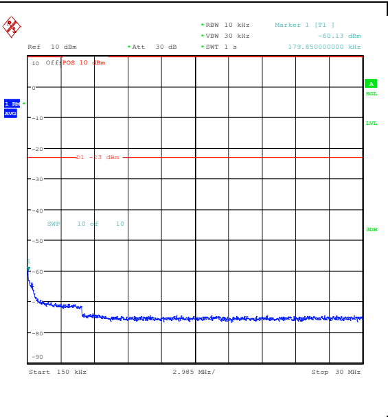
Band5_1.4MHz_QPSK_20525_6RB#0_0.15~30_0.15~30
