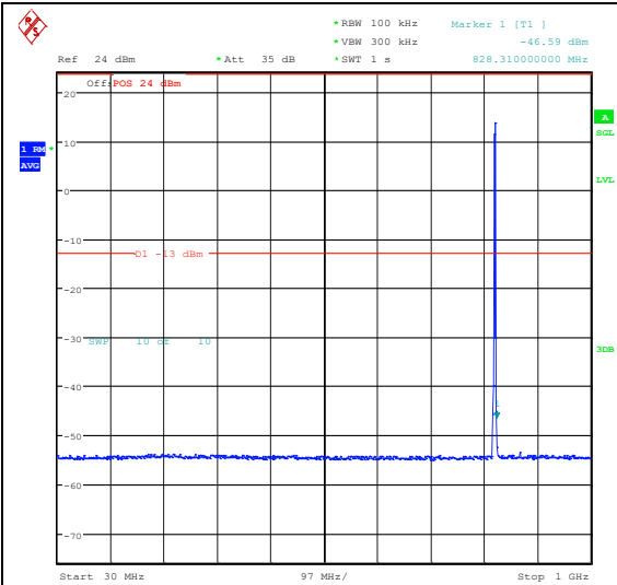
Band5_1.4MHz_QPSK_20407_6RB#0_30~1000_30~1000
