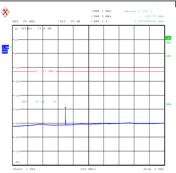
Band5_10MHz_QPSK_20600_1RB#49_1000~300_0_1000~3000
