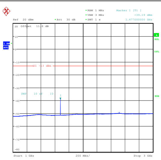
Band5_5MHz_QPSK_20525_1RB#24_1000~3000_1000~3000
