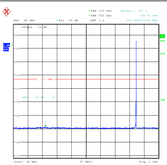
Band5_3MHz_16QAM_20635_1RB#14_30~1000_30~1000
