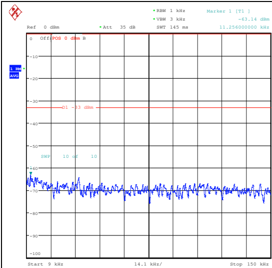
Band5_5MHz_QPSK_20525_1RB#0_0.009~0.15_0.009~0.15
