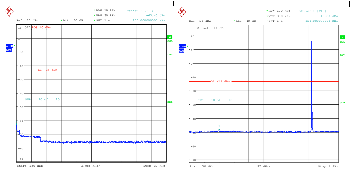
Band5_5MHz_16QAM_20425_1RB#0_0.15~30_0.15~30 Band5_5MHz_16QAM_20425_1RB#0_30~1000_30~1000
