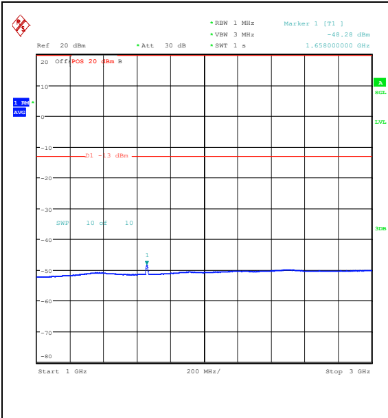
Band5_10MHz_16QAM_20450_50RB#0_1000~3000_1000~3000
