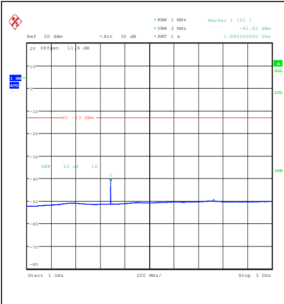
Band5_10MHz_16QAM_20525_1RB#49_1000~3000_1000~3000
