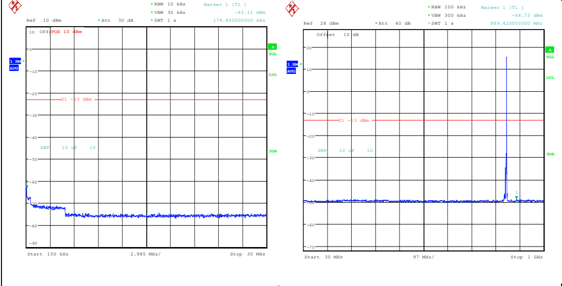
Band5_5MHz_16QAM_20625_1RB#24_0.15~30_0.15~30 Band5_5MHz_16QAM_20625_1RB#24_30~1000_30~1000
