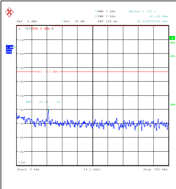
Band5_3MHz_QPSK_20635_15RB#0_0.009~0.15_5_0.009~0.15
