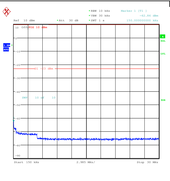
Band5_10MHz_QPSK_20600_1RB#0_0.15~30_0. 15~30
