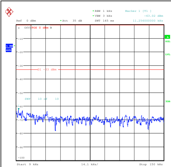
Band5_5MHz_QPSK_20425_1RB#24_0.009~0.15 5_0.009~0.15
