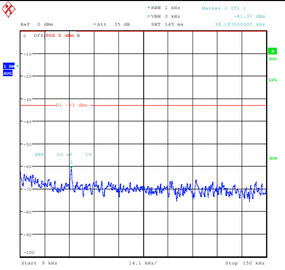
Band5_10MHz_QPSK_20600_1RB#49_1000~300_0_1000~3000
