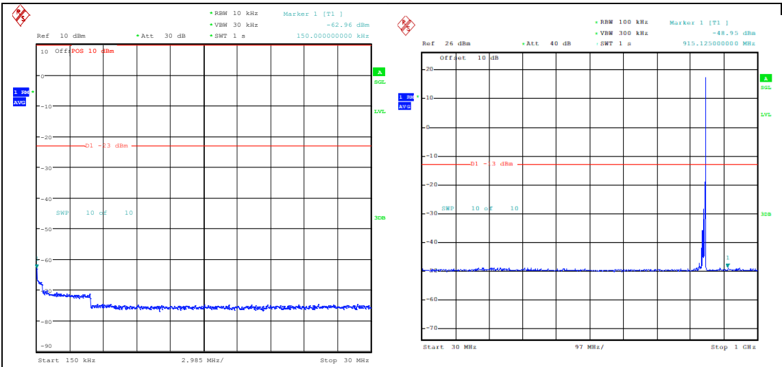
Band5_10MHz_16QAM_20600_1RB#49_0.15~30_0.15~30
