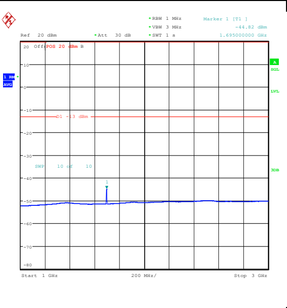
Band5_3MHz_QPSK_20635_15RB#0_1000~3000_1000~3000
