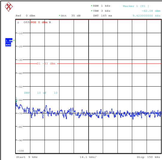
Band5_10MHz_QPSK_20600_50RB#0_0.009~0.15_0.009~0.15
