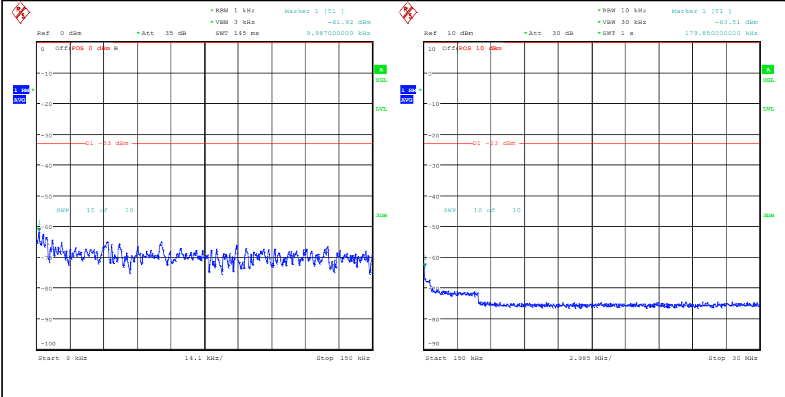
Band5_5MHz_QPSK_20625_1RB#0_0.009~0.15_0.009~0.15 Band5_5MHz_QPSK_20625_1RB#0_0.15~30_0.15~30
