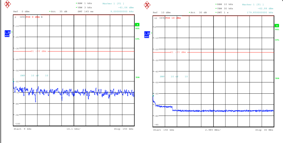
Band5_5MHz_QPSK_20425_1RB#0_0.009~0.15 _0.009~0.15 Band5_5MHz_QPSK_20425_1RB#0_0.15~30_0.1 5~30
