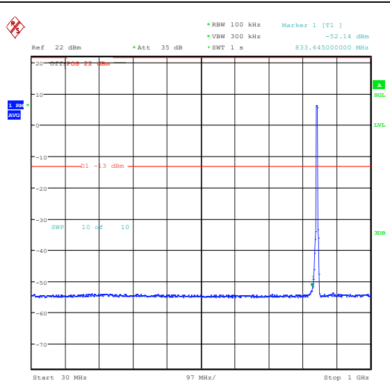
Band5_5MHz_16QAM_20625_25RB#0_30~1000_30~1000
