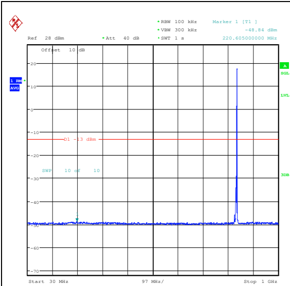
Band5_5MHz_QPSK_20525_1RB#24_30~1000_30~1000
