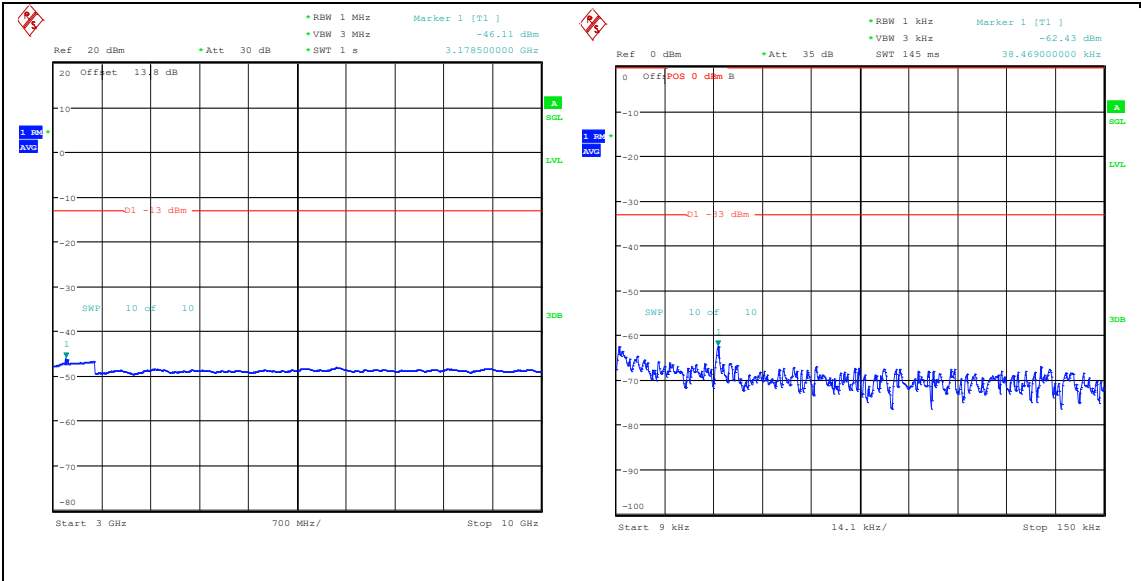
Band5_5MHz_QPSK_20625_1RB#24_3000~10000_3000~10000 Band5_5MHz_16QAM_20625_1RB#24_0.009~0.15_0.009~0.15
