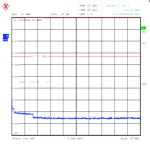
Band5_10MHz_QPSK_20525_50RB#0_0.15~30_0.15~30
