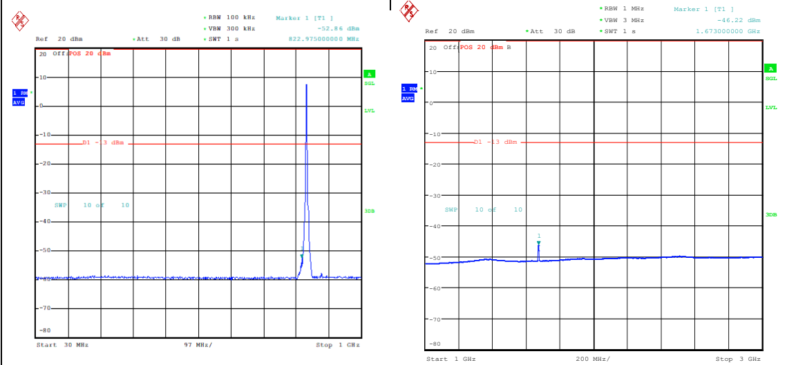
Band5_5MHz_QPSK_20525_25RB#0_30~1000_ 30~1000 Band5_5MHz_QPSK_20525_25RB#0_1000~3000 _1000~3000
