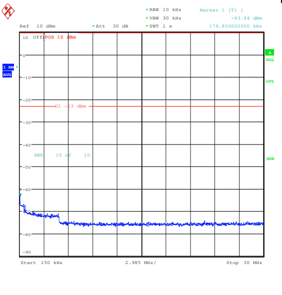
Band5_3MHz_QPSK_20525_15RB#0_0.15~30_0.15~30
