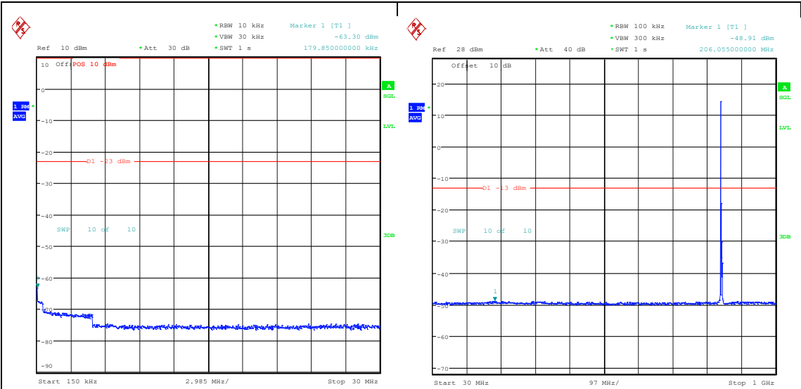
Band5_5MHz_16QAM_20625_1RB#0_0.15~30_0.15~30 Band5_5MHz_16QAM_20625_1RB#0_30~1000_30~1000
