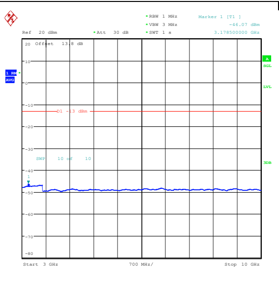
Band5_10MHz_16QAM_20525_1RB#49_3000~10000_3000~10000
