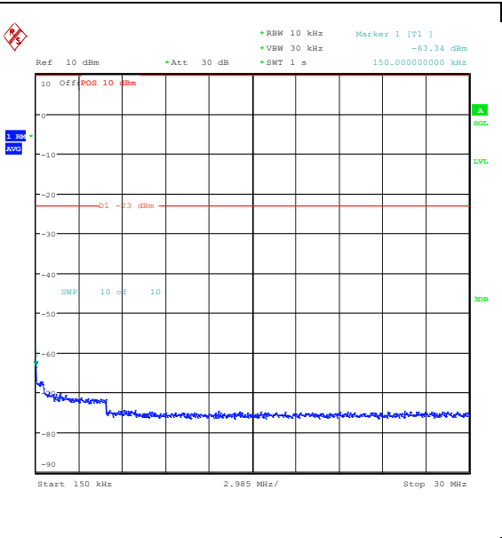
Band5_3MHz_QPSK_20635_15RB#0_0.15~30_0.15~30
