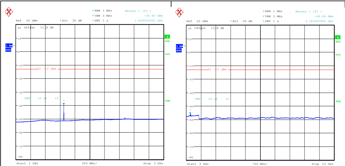
Band5_10MHz_16QAM_20450_1RB#0_1000~3000_00_1000~3000 Band5_10MHz_16QAM_20450_1RB#0_3000~10000_00_3000~10000
