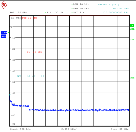
Band5_10MHz_QPSK_20525_1RB#49_0.15~30_0.15~30
