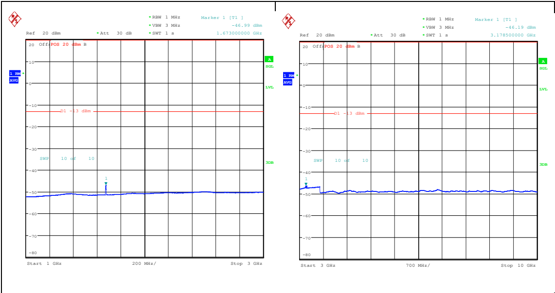
Band5_5MHz_16QAM_20525_25RB#0_1000~3000_00_1000~3000 Band5_5MHz_16QAM_20525_25RB#0_3000~10000_00_3000~10000
