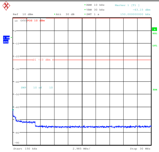
Band5_5MHz_QPSK_20525_1RB#0_0.15~30_0.15~30
