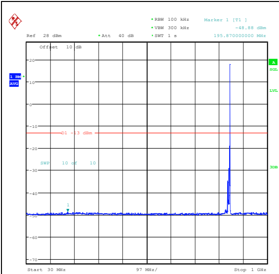
Band5_10MHz_QPSK_20600_1RB#49_30~1000_30~1000
