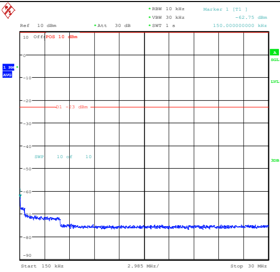
Band5_5MHz_QPSK_20625_1RB#24_0.15~30_0.15~30
