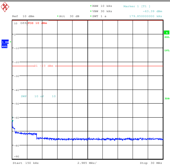
Band5_10MHz_QPSK_20600_50RB#0_0.15~30_0.15~30
