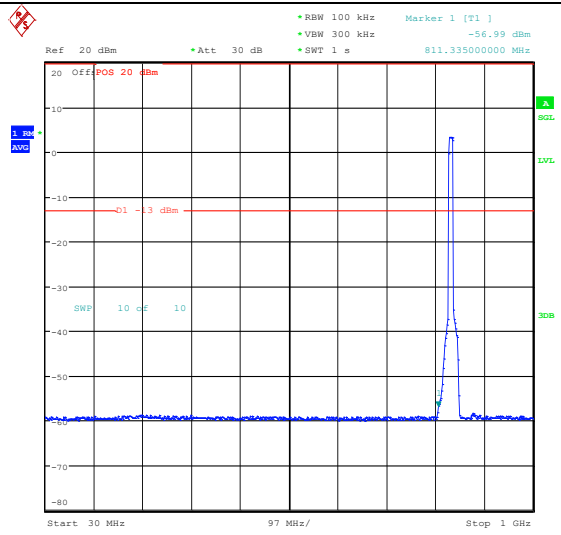
Band5_10MHz_16QAM_20525_50RB#0_30~1000 _30~1000
