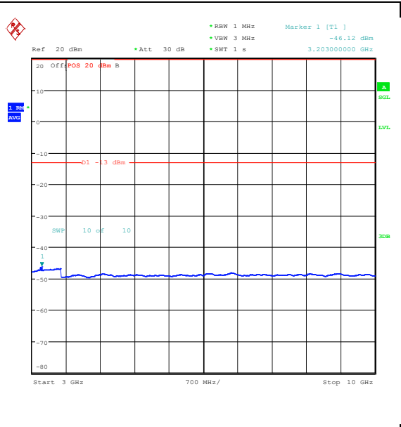
Band5_10MHz_16QAM_20450_50RB#0_3000~10000_000_3000~10000
