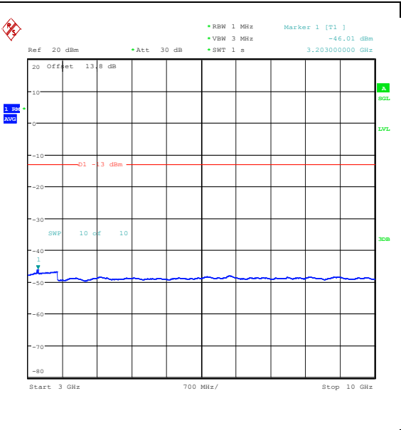
Band5_3MHz_16QAM_20525_1RB#14_3000~10000
