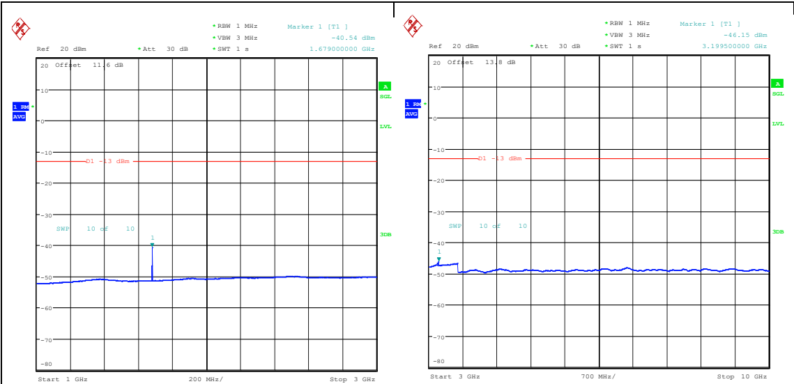
Band5_10MHz_16QAM_20600_1RB#0_1000~3000 00_1000~3000 Band5_10MHz_16QAM_20600_1RB#0_3000~10000 00_3000~10000
