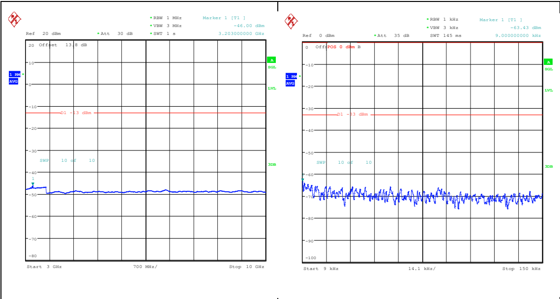
Band5_5MHz_QPSK_20525_1RB#0_3000~1000 0_3000~10000 Band5_5MHz_16QAM_20525_1RB#0_0.009~0.15 _0.009~0.15
