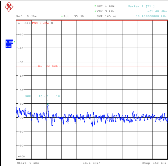
Band5_10MHz_QPSK_20525_1RB#49_0.009~0.15_0.009~0.15
