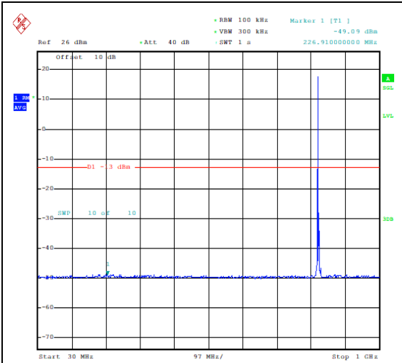
Band5_5MHz_QPSK_20425_1RB#0_30~1000_3 0~1000
