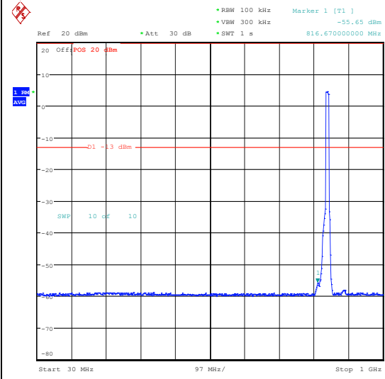
Band5_10MHz_QPSK_20600_50RB#0_30~1000_30~1000
