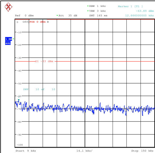
Band5_5MHz_QPSK_20625_1RB#24_0.009~0.15_0.009~0.15
