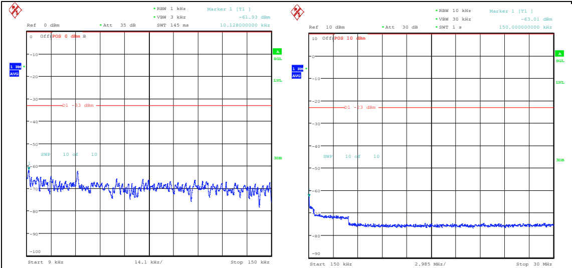
Band5_3MHz_QPSK_20525_1RB#14_0.009~0.15_0.009~0.15 Band5_3MHz_QPSK_20525_1RB#14_0.15~30_0.15~30
