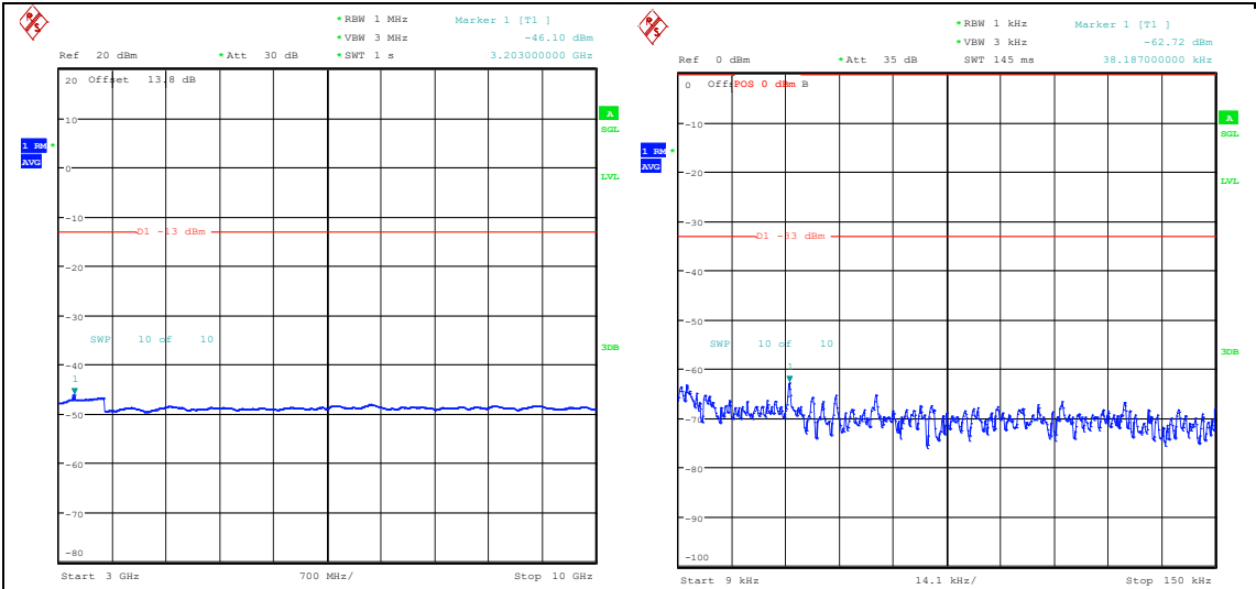
Band5_3MHz_QPSK_20525_1RB#14_3000~10000_3000~10000 Band5_3MHz_16QAM_20525_1RB#14_0.009~0.15_0.009~0.15
