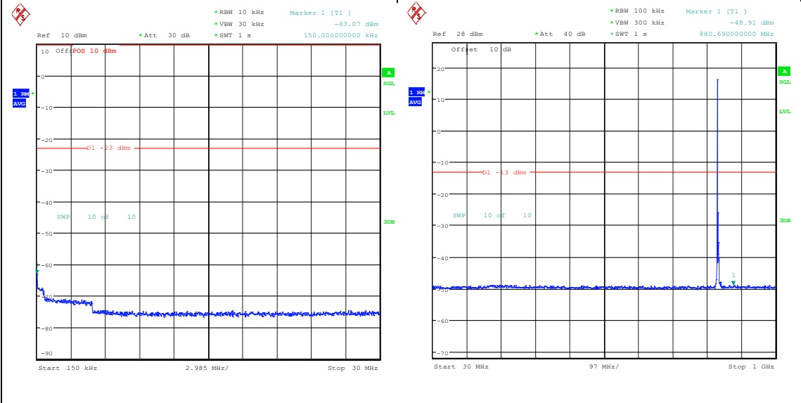
Band5_5MHz_16QAM_20525_1RB#0_0.15~30 0.15~30 Band5_5MHz_16QAM_20525_1RB#0_30~1000_3 0~1000
