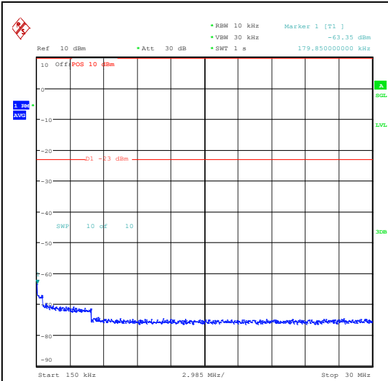
Band5_5MHz_16QAM_20625_25RB#0_0.15~30_0.15~30
