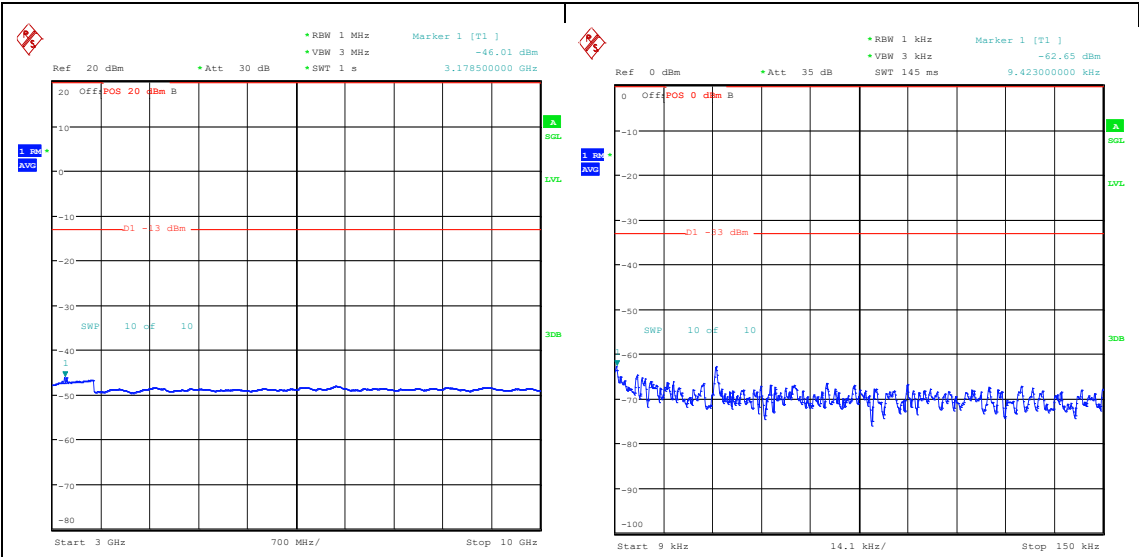
Band5_3MHz_QPSK_20635_15RB#0_3000~10000_3000~10000 Band5_3MHz_16QAM_20635_15RB#0_0.009~0.15_0.009~0.15
