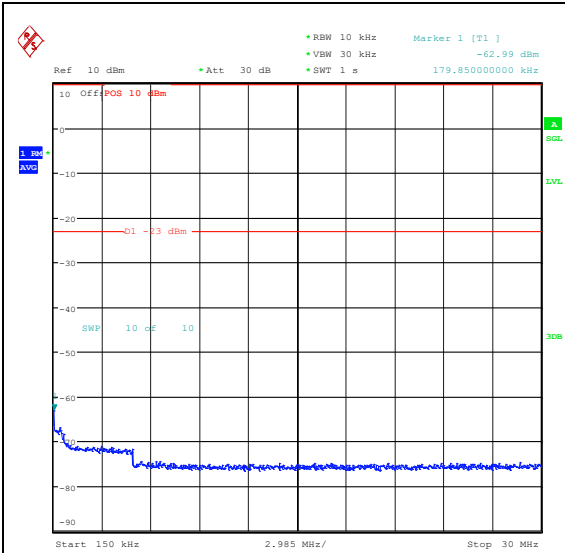
Band5_3MHz_16QAM_20635_1RB#14_0.15~30_0.15~30
