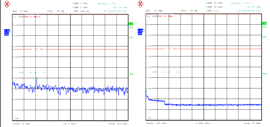
Band5_5MHz_QPSK_20425_25RB#0_0.009~0.15_0.009~0.15 Band5_5MHz_QPSK_20425_25RB#0_0.15~30_0.15~30
