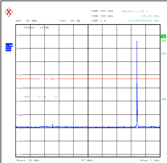
Band5_5MHz_QPSK_20625_1RB#0_30~1000_3 0~1000
