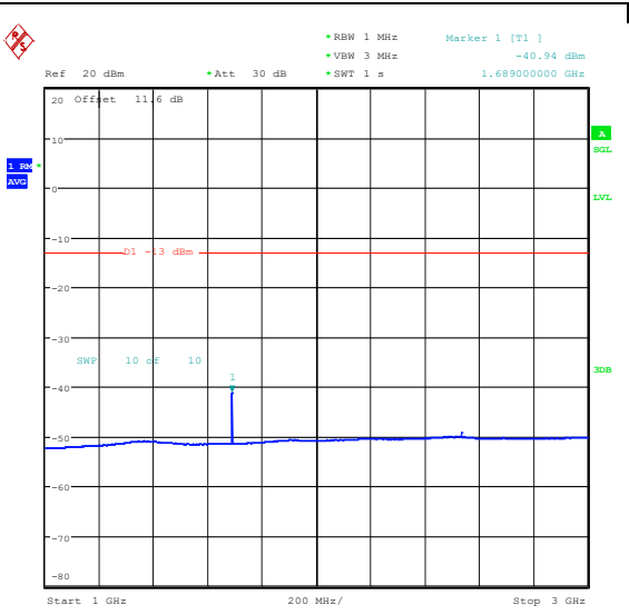
Band5_5MHz_QPSK_20625_1RB#0_1000~3000_ 1000~3000
