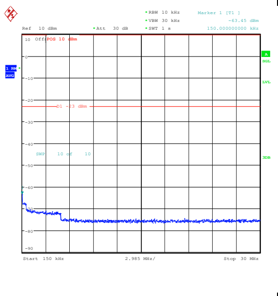
Band5_10MHz_QPSK_20525_1RB#0_0.15~30_0.15~30
