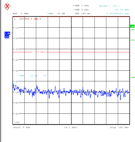
Band5_3MHz_QPSK_20525_15RB#0_0.009~0.15
