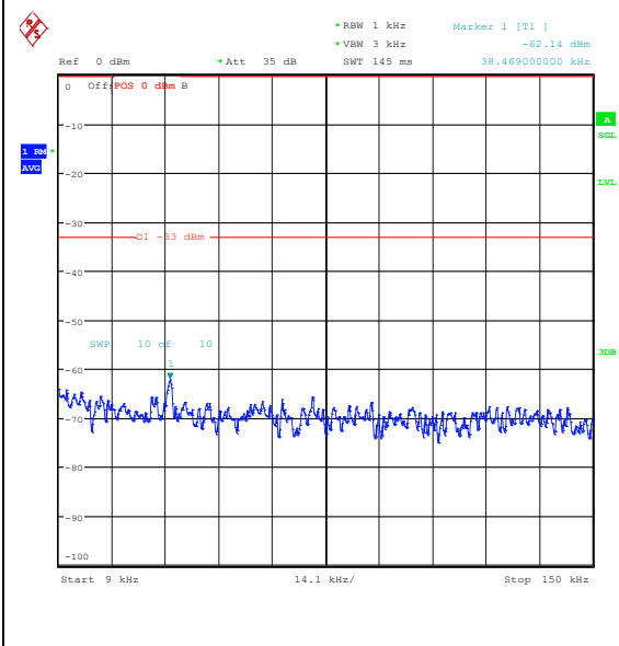
Band5_10MHz_QPSK_20525_50RB#0_0.009~0.15_0.009~0.15
