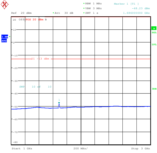
Band5_10MHz_QPSK_20600_50RB#0_1000~3000_0_1000~3000
