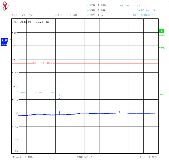
Band5_5MHz_QPSK_20425_1RB#0_1000~3000_1000~3000
