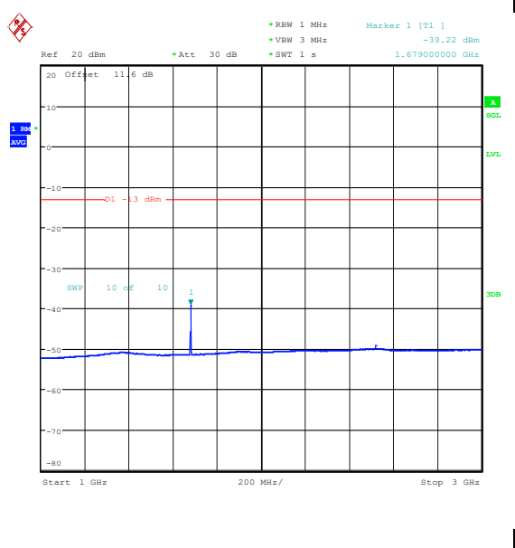
Band5_10MHz_QPSK_20600_1RB#0_1000~3000 _1000~3000
