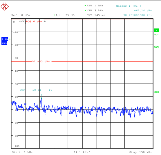
Band5_3MHz_16QAM_20635_1RB#0_0.009~0.15_0.009~0.15
