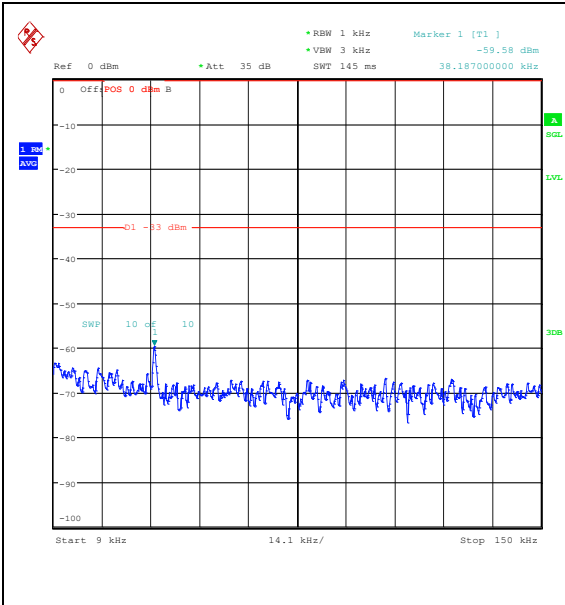
Band5_10MHz_QPSK_20600_1RB#0_0.009~0.15 5_0.009~0.15
