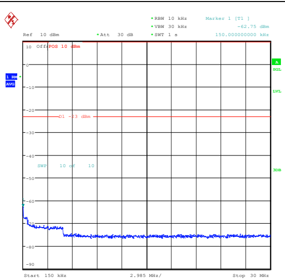
Band5_5MHz_QPSK_20425_1RB#24_0.15~30_0. 15~30
