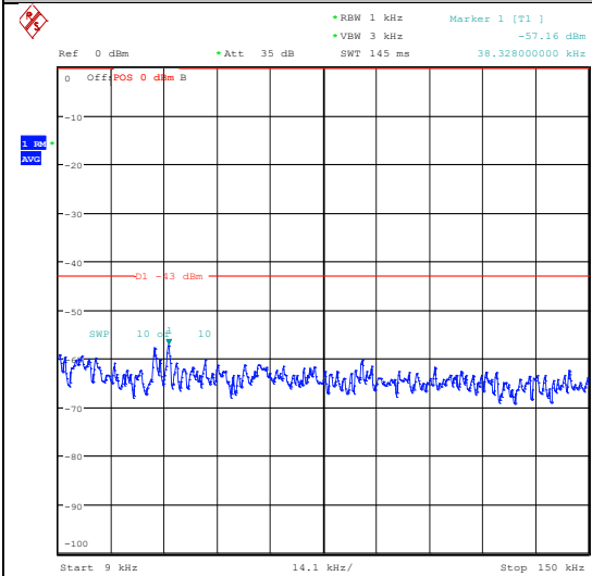
Band2_1.4MHz_16QAM_19193_1RB#0_1000~3000_1000~3000
