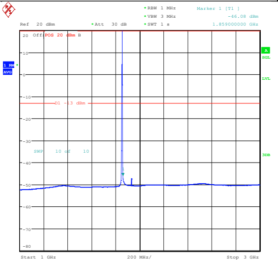
Band2_3MHz_QPSK_18615_1RB#14_0.15~30_0. 15~30
