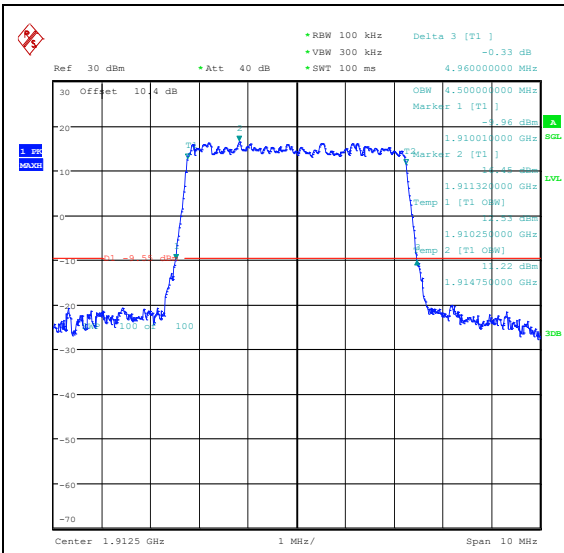
Band25-5MHz-QPSK-26665-25RB#0-PASS
