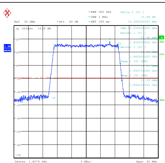
Band25-15MHz-16QAM-26115-75RB#0-PASS
