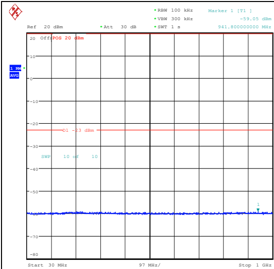
Band25_1.4MHz_QPSK_26047_1RB#5_30~1000_30~1000
