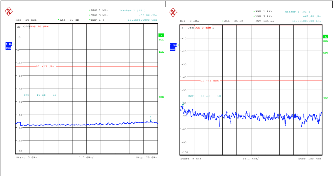
Band25_1.4MHz_QPSK_26047_6RB#0_3000~20000_3000~20000 Band25_1.4MHz_16QAM_26047_6RB#0_0.009~0.15_0.009~0.15
