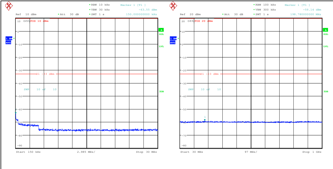
Band25_1.4MHz_16QAM_26365_1RB#0_0.15~30_0.15~30 Band25_1.4MHz_16QAM_26365_1RB#0_30~100_0_30~1000
