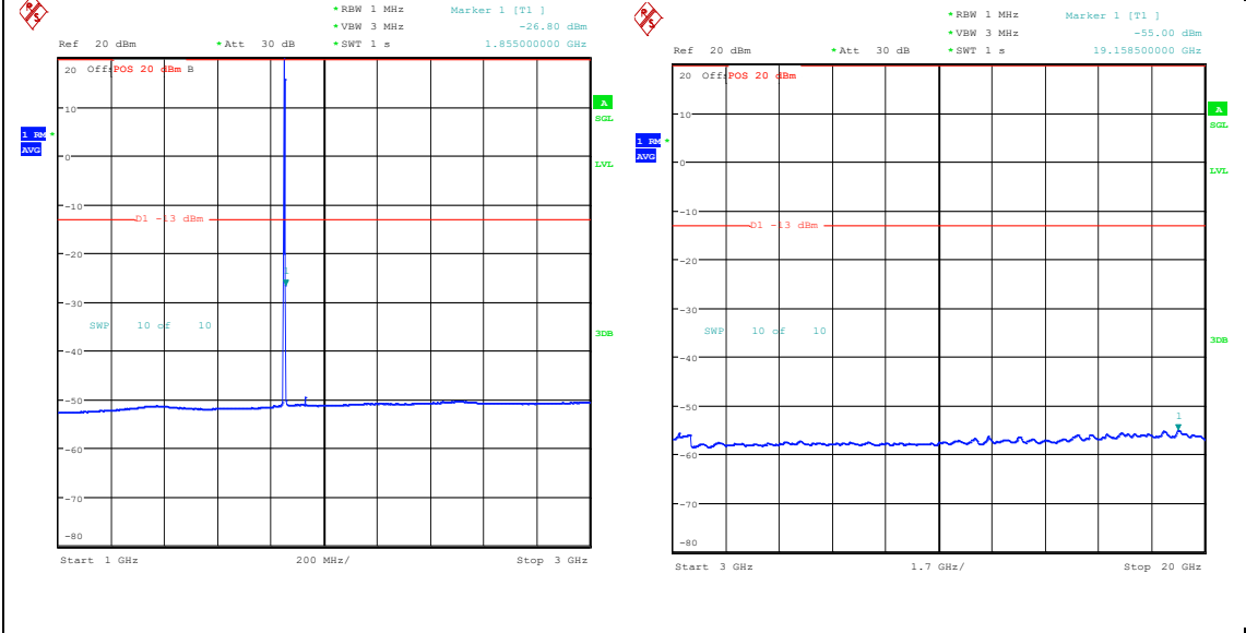
Band25_1.4MHz_16QAM_26047_1RB#5_1000~3000 3000_1000~3000 Band25_1.4MHz_16QAM_26047_1RB#5_3000~20000 0000_3000~20000
