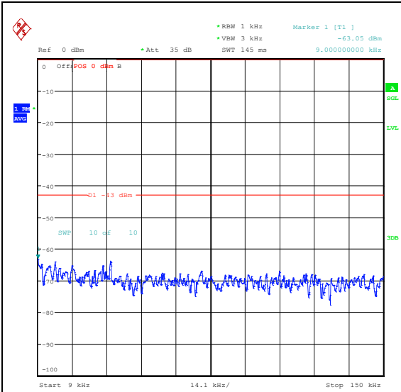
Band25_1.4MHz_QPSK_26047_6RB#0_0.009~0.15_0.009~0.15
