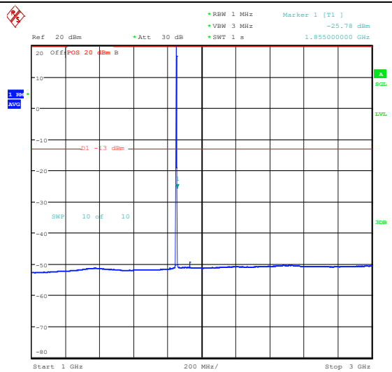
Band25_1.4MHz_QPSK_26047_1RB#5_1000~3000_00_1000~3000
