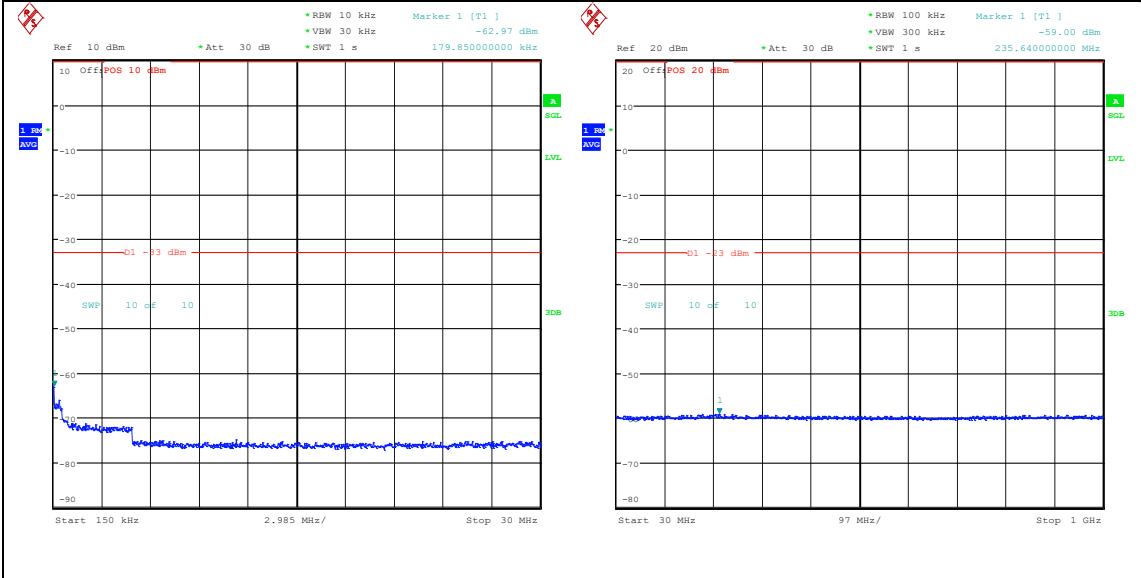
Band25_1.4MHz_16QAM_26047_6RB#0_0.15~30_0.15~30 Band25_1.4MHz_16QAM_26047_6RB#0_30~100_30~1000
