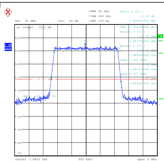
Band25-3MHz-16QAM-26365-15RB#0-PASS
