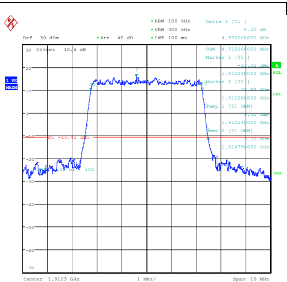
Band25-5MHz-16QAM-26665-25RB#0-PASS
