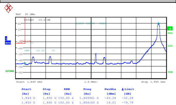
Band25_15MHz_16QAM_26115_1RB#0
