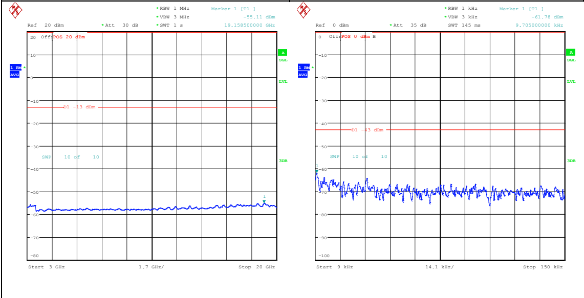
Band25_1.4MHz_QPSK_26365_1RB#0_3000~20000_000_3000~20000 Band25_1.4MHz_16QAM_26365_1RB#0_0.009~0.15_0.009~0.15
