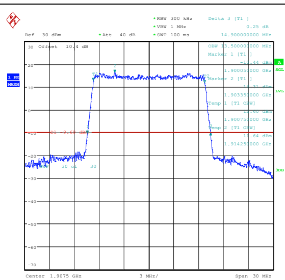
Band25-15MHz-16QAM-26615-75RB#0-PASS
