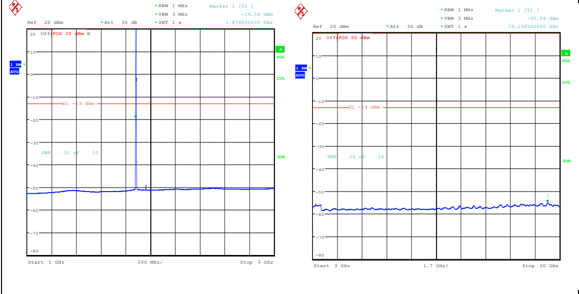
Band25_1.4MHz_16QAM_26365_1RB#0_1000~3000_1000~3000 Band25_1.4MHz_16QAM_26365_1RB#0_3000~20000_0000_3000~20000
