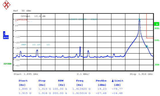
Band25_20MHz_16QAM_26590_1RB#0
