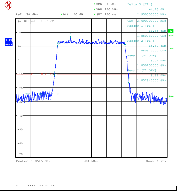
Band25-3MHz-16QAM-26055-15RB#0-PASS
