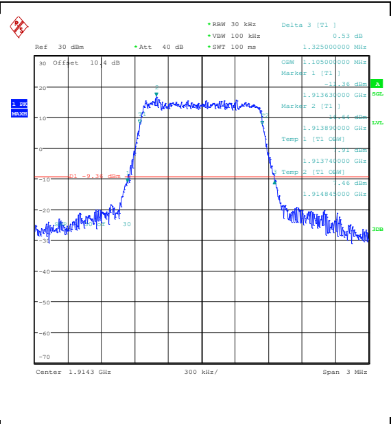
Band25-1.4MHz-16QAM-26683-6RB#0-PASS
