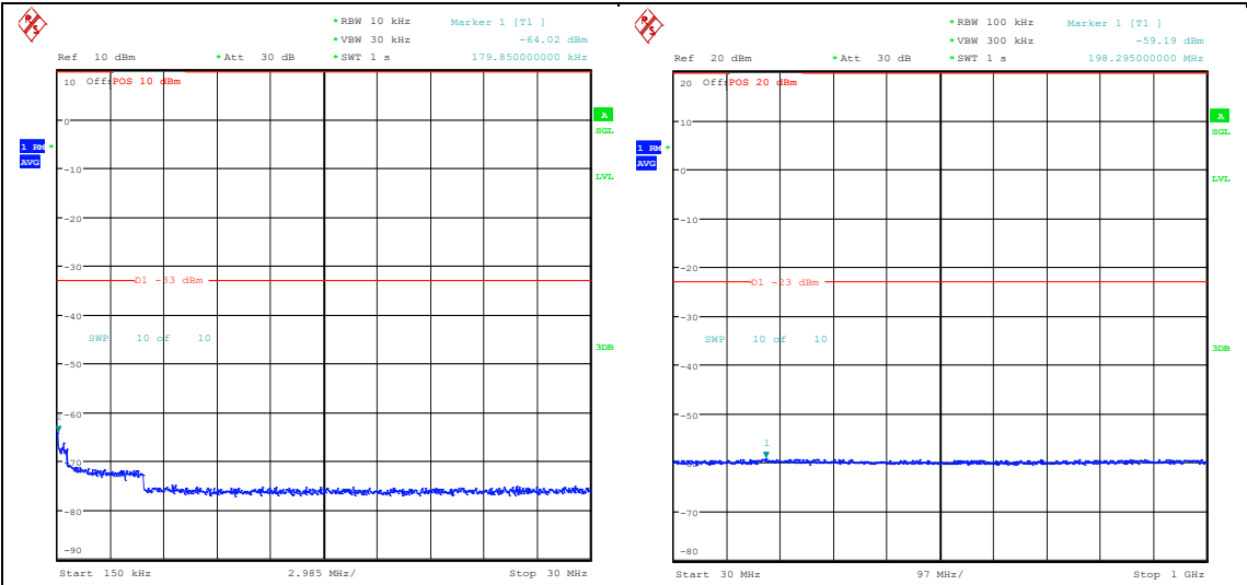
Band25_1.4MHz_16QAM_26365_6RB#0_0.15~30_0.15~30 Band25_1.4MHz_16QAM_26365_6RB#0_30~100_0_30~1000
