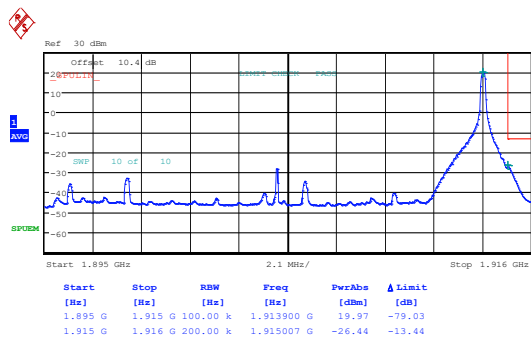
Band25_20MHz_QPSK_26590_1RB#0
