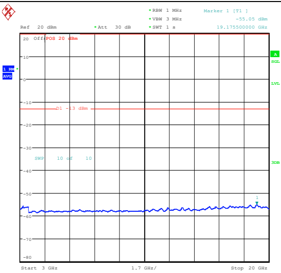
Band25_1.4MHz_16QAM_26047_1RB#0_3000~20000_3000~20000
