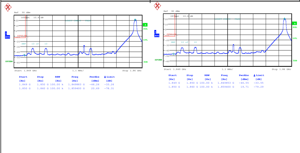
Band25_10MHz_QPSK_26090_1RB#49
