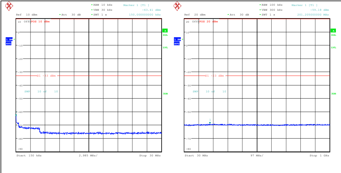
Band25_1.4MHz_16QAM_26047_1RB#5_0.15~30 0_0.15~30 Band25_1.4MHz_16QAM_26047_1RB#5_30~100 0_30~1000
