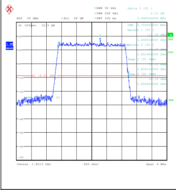
Band25-3MHz-QPSK-26055-15RB#0-PASS
