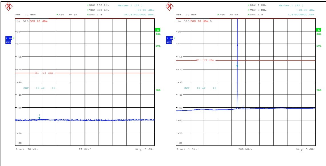
Band25_1.4MHz_QPSK_26365_1RB#0_30~1000_30~1000 Band25_1.4MHz_QPSK_26365_1RB#0_1000~3000_00_1000~3000
