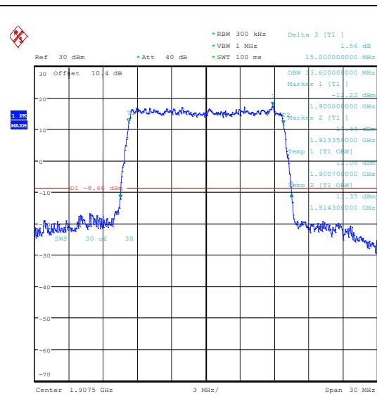
Band25-15MHz-QPSK-26615-75RB#0-PASS
