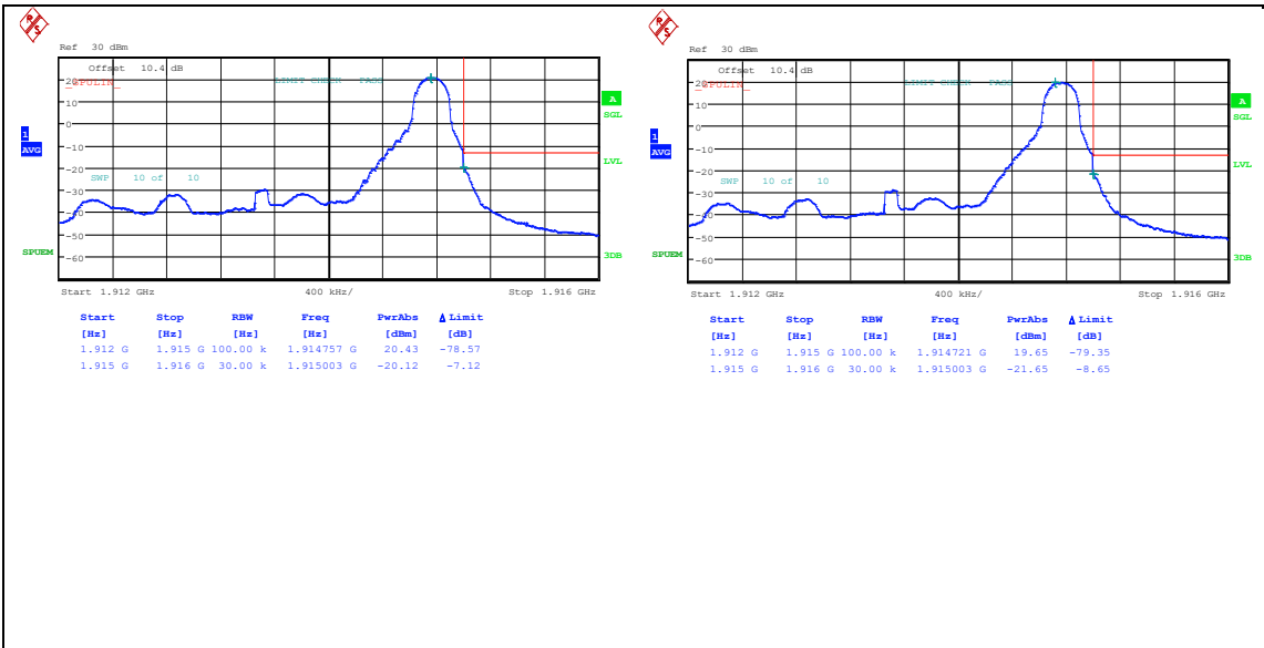
Band25_3MHz_QPSK_26675_1RB#14
