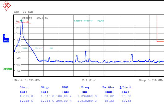
Band25_20MHz_QPSK_26140_100RB#0
