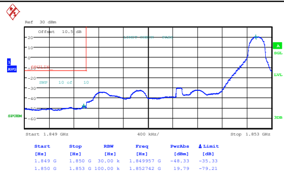
Band25_3MHz_16QAM_26055_1RB#0
