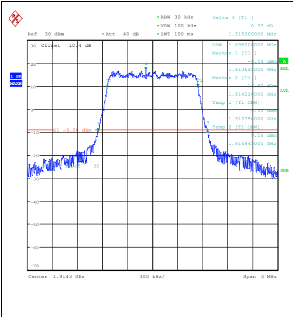
Band25-1.4MHz-QPSK-26683-6RB#0-PASS
