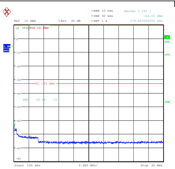
Band25_1.4MHz_QPSK_26047_6RB#0_0.15~30_0.15~30
