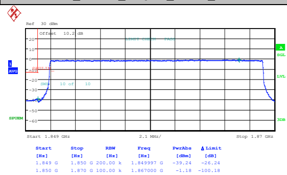
Band25_20MHz_16QAM_26140_1RB#99
