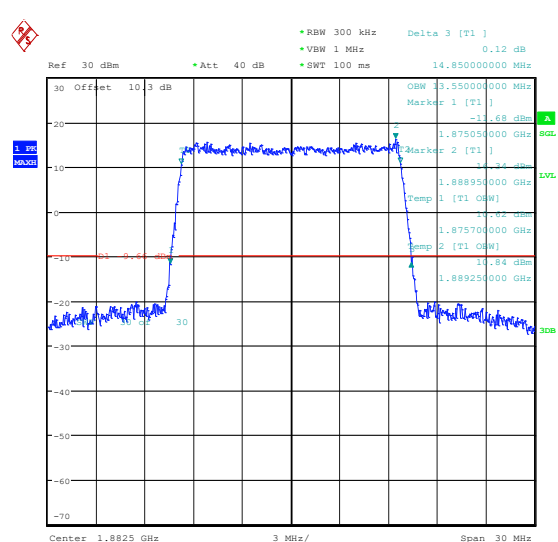
Band25-15MHz-16QAM-26115-75RB#0-PASS
