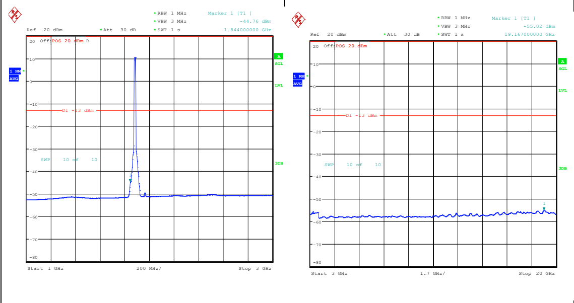
Band25_15MHz_16QAM_26365_75RB#0_1000~3000_1000~3000 Band25_15MHz_16QAM_26365_75RB#0_3000~20000_3000~20000
