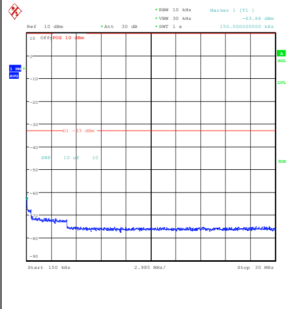
Band25_15MHz_16QAM_26615_1RB#0_0.15~30_0.15~30
