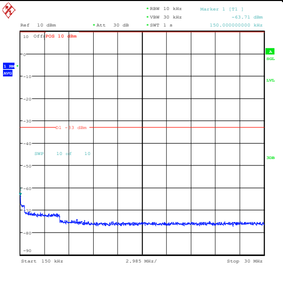
Band25_10MHz_QPSK_26640_50RB#0_0.15~30_0.15~30
