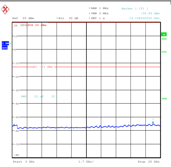
Band25_15MHz_16QAM_26615_75RB#0_3000~20000_0000_3000~20000
