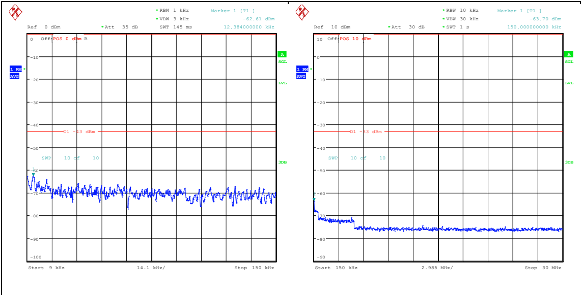
Band25_20MHz_QPSK_26365_100RB#0_0.009~0.15_0.009~0.15 Band25_20MHz_QPSK_26365_100RB#0_0.15~3_0_0.15~30
