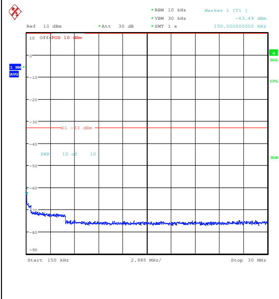
Band25_15MHz_16QAM_26365_1RB#74_0.15~30
