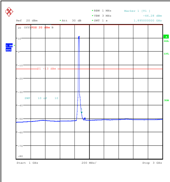
Band25_15MHz_16QAM_26115_75RB#0_1000~3000_1000~3000
