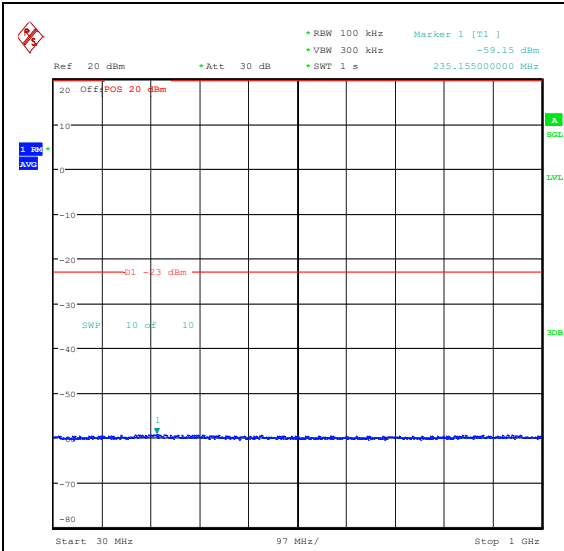
Band25_20MHz_QPSK_26140_1RB#0_30~1000_30~1000
