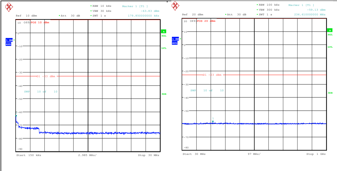
Band25_20MHz_16QAM_26590_1RB#0_0.15~3 0_0.15~30
