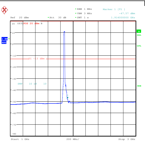
Band25_20MHz_QPSK_26140_100RB#0_1000~3000_000_1000~3000
