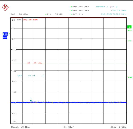
Band25_20MHz_16QAM_26590_100RB#0_30~10 00_30~1000
