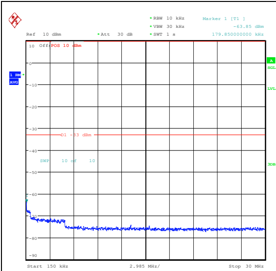
Band25_20MHz_16QAM_26590_100RB#0_0.15 ~30_0.15~30
