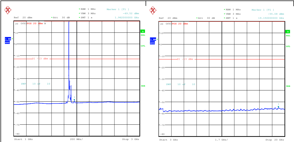
Band25_20MHz_16QAM_26365_1RB#0_1000~3000_1000~3000 Band25_20MHz_16QAM_26365_1RB#0_3000~20000_3000~20000
