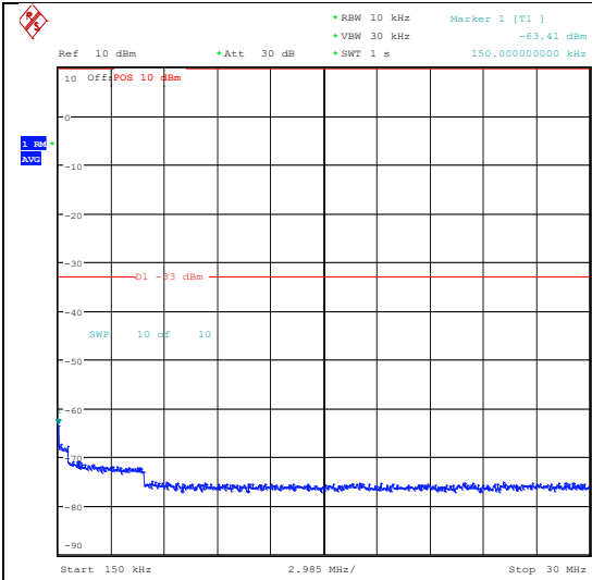
Band25_20MHz_16QAM_26365_1RB#99_0.15~30_0.15~30 Band25_20MHz_16QAM_26365_1RB#99_30~100_0_30~1000
