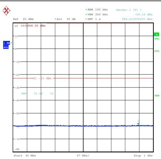
Band25_20MHz_16QAM_26140_1RB#0_30~1000 _30~1000
