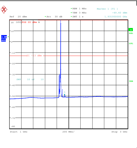
Band25_15MHz_QPSK_26115_1RB#74_1000~30 00_1000~3000
