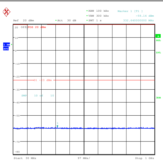
Band25_10MHz_16QAM_26640_50RB#0_30~100 0_30~1000
