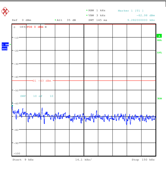
Band25_15MHz_16QAM_26615_1RB#0_0.009~0.15_0.009~0.15
