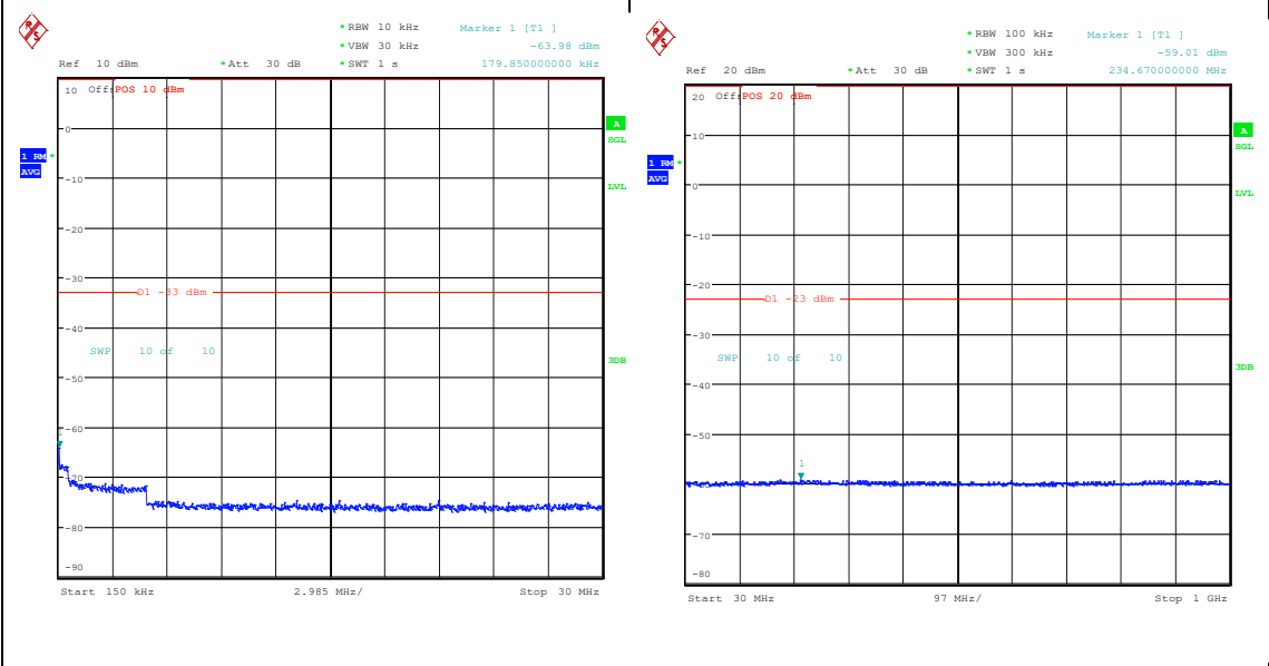
Band25_20MHz_16QAM_26365_100RB#0_0.15~30_0.15~30 Band25_20MHz_16QAM_26365_100RB#0_30~1000_30~1000
