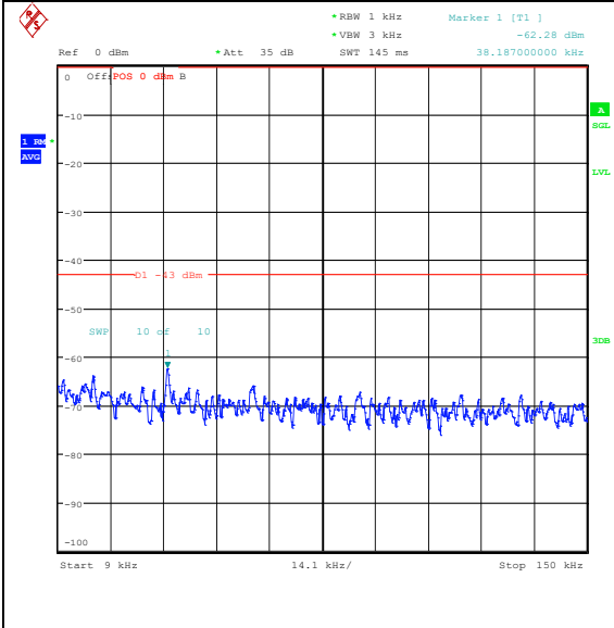
Band25_10MHz_QPSK_26640_50RB#0_0.009~0.15_0.009~0.15
