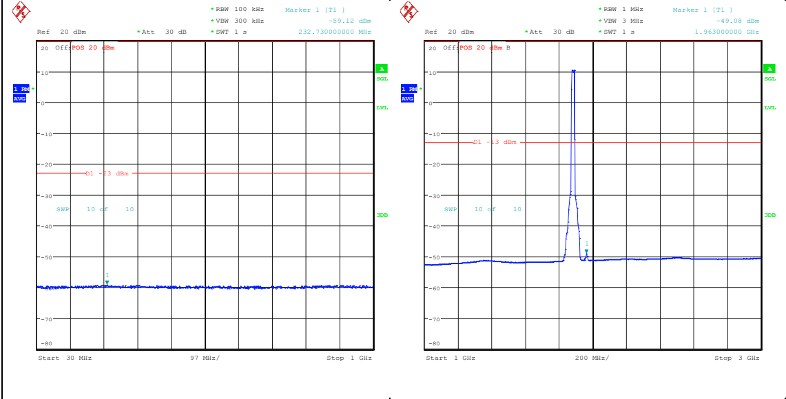
Band25_20MHz_QPSK_26365_100RB#0_30~1000_30~1000 Band25_20MHz_QPSK_26365_100RB#0_1000~3000_1000~3000
