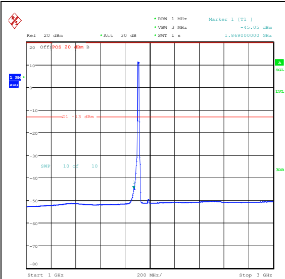
Band25_15MHz_16QAM_26615_75RB#0_1000~3000_1000~3000
