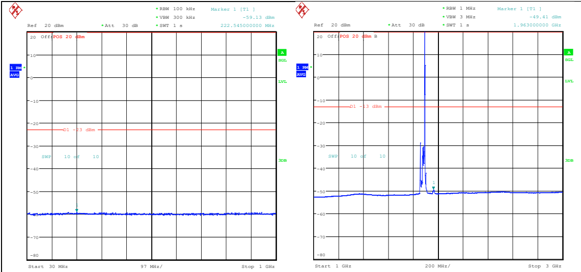
Band25_20MHz_QPSK_26365_1RB#99_30~1000_30~1000 Band25_20MHz_QPSK_26365_1RB#99_1000~3000_00_1000~3000
