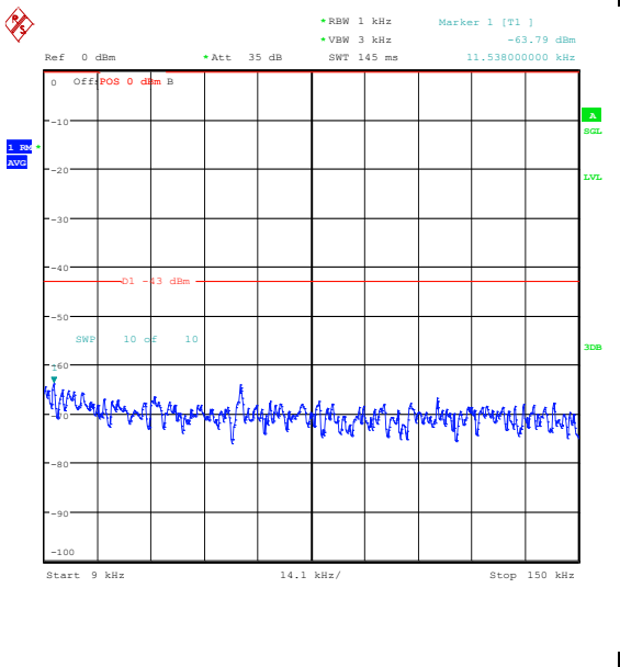
Band25_10MHz_16QAM_26640_50RB#0_0.009~ 0.15_0.009~0.15
