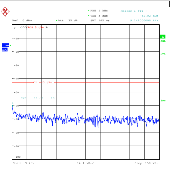
Band25_15MHz_16QAM_26365_1RB#74_0.009~0.15
