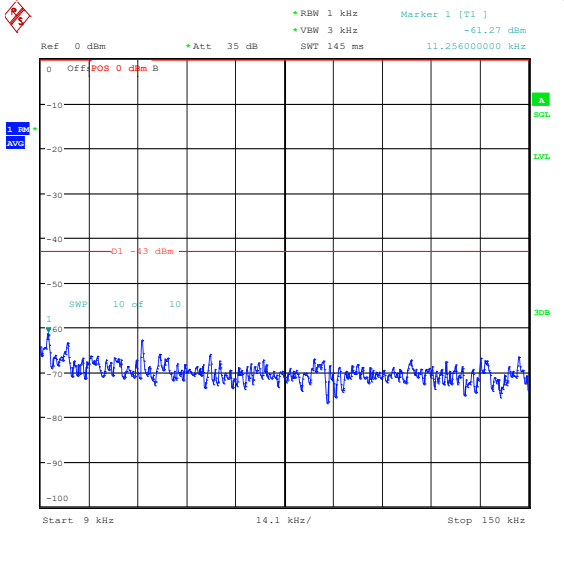
Band25_20MHz_16QAM_26590_1RB#0_0.009~0.15_15_0.009~0.15
