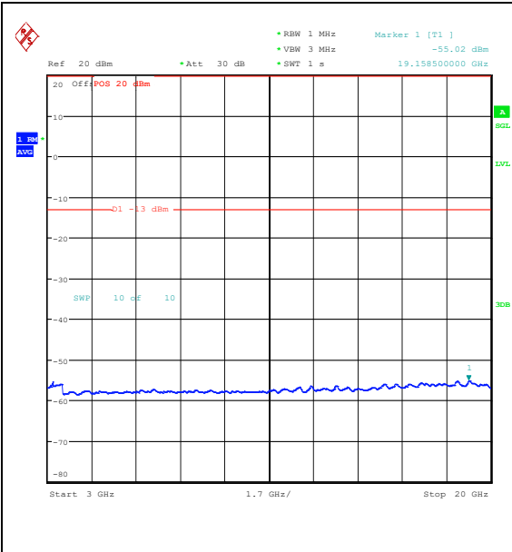
Band25_15MHz_QPSK_26615_1RB#0_3000~20000_3000~20000
