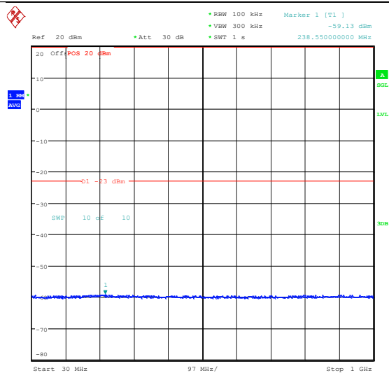
Band25_20MHz_16QAM_26365_1RB#99_0.15~30_0.15~30 Band25_20MHz_16QAM_26365_1RB#99_30~100_0_30~1000
