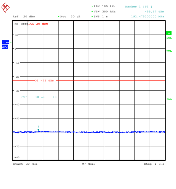
Band25_15MHz_16QAM_26615_1RB#0_30~1000_30~1000
