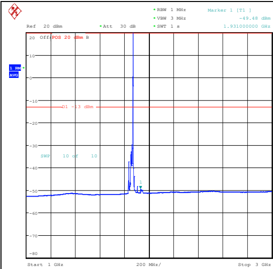
Band25_20MHz_16QAM_26140_1RB#99_1000~3000_1000~3000
