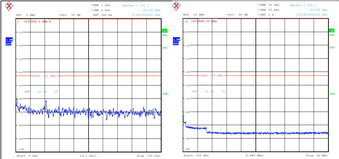
Band25_20MHz_QPSK_26365_1RB#0_0.009~0.15_0.009~0.15 Band25_20MHz_QPSK_26365_1RB#0_0.15~30_0.15~30
