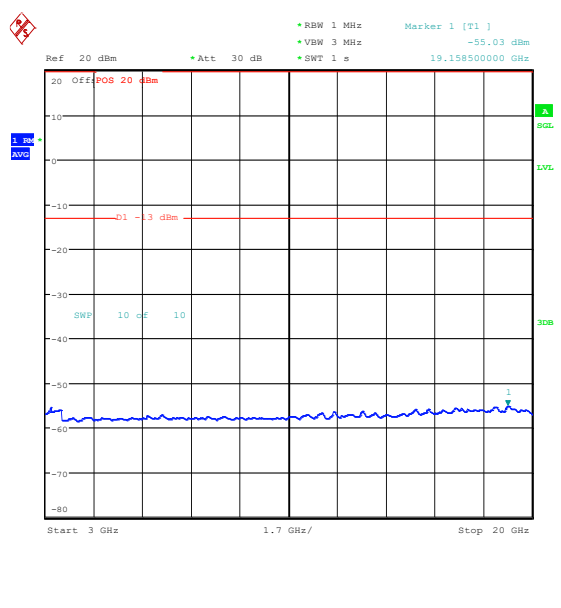
Band25_15MHz_16QAM_26365_1RB#0_3000~20 000_3000~20000
