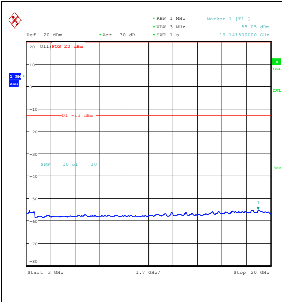
Band25_15MHz_QPSK_26365_1RB#74_3000~20000
