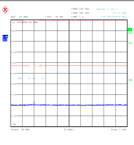
Band25_15MHz_16QAM_26365_1RB#0_30~1000 _30~1000
