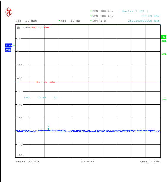
Band25_20MHz_QPSK_26590_1RB#0_30~1000_30~1000
