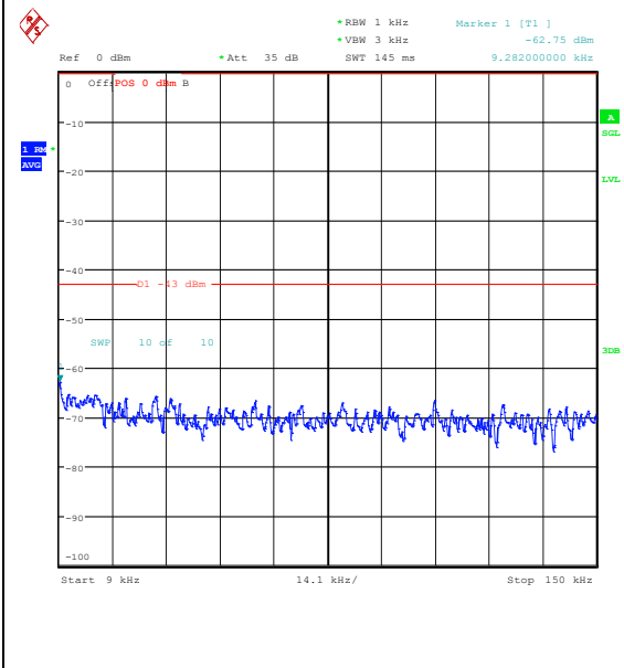
Band25_15MHz_QPSK_26365_1RB#0_0.009~0.15_0.009~0.15
