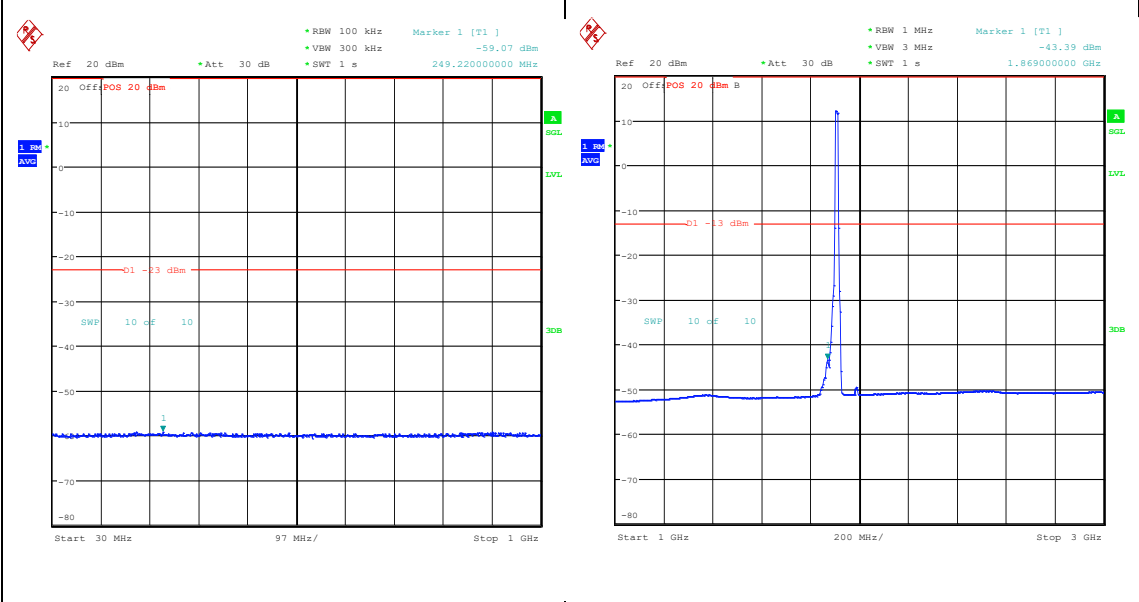
Band25_15MHz_QPSK_26615_75RB#0_30~1000_0_30~1000 Band25_15MHz_QPSK_26615_75RB#0_1000~3000_00_1000~3000
