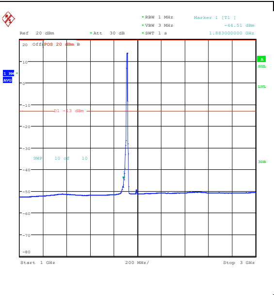
Band25_10MHz_QPSK_26640_50RB#0_1000~30 00_1000~3000
