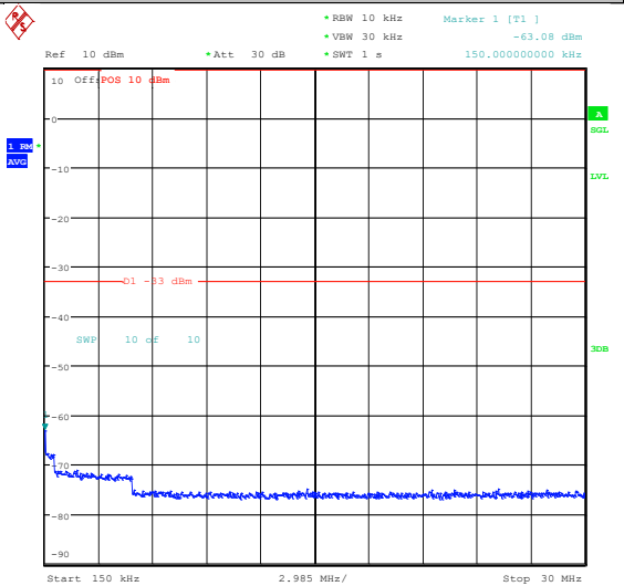
Band25_15MHz_16QAM_26615_75RB#0_3000~20000_0000_3000~20000
