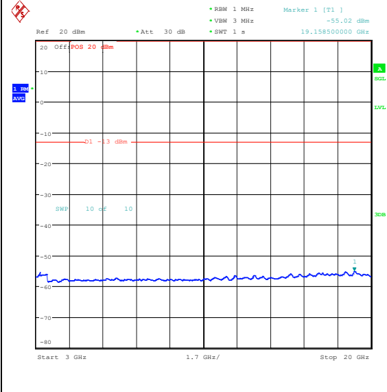
Band25_20MHz_QPSK_26590_1RB#0_3000~20000_000_3000~20000
