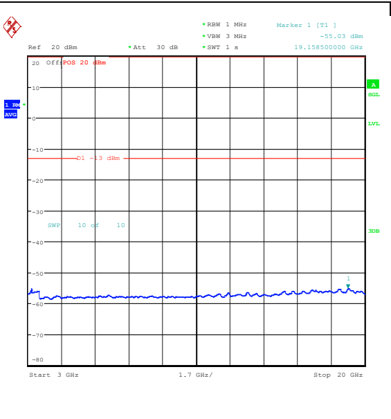
Band25_15MHz_16QAM_26115_1RB#0_3000~20000_3000~20000
