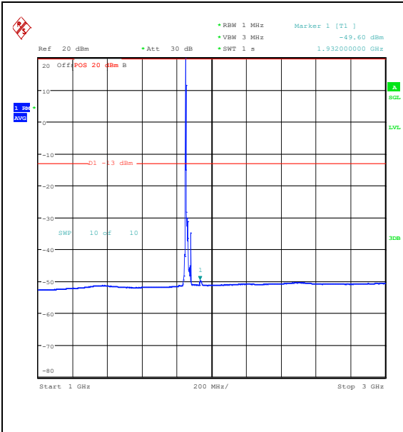
Band25_15MHz_16QAM_26115_1RB#0_1000~3000_1000~3000
