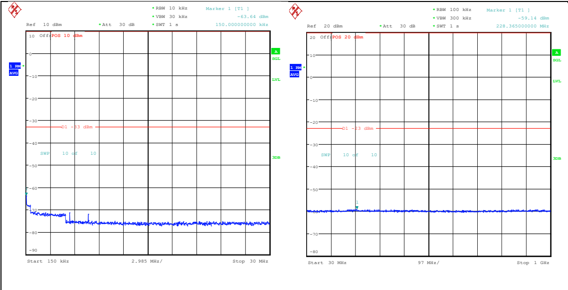
Band25_15MHz_16QAM_26365_75RB#0_0.15~30_0.15~30 Band25_15MHz_16QAM_26365_75RB#0_30~1000_0.30~1000
