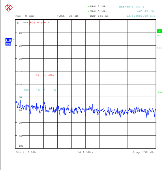
Band25_15MHz_QPSK_26115_1RB#74_0.009~0.15_0.009~0.15
