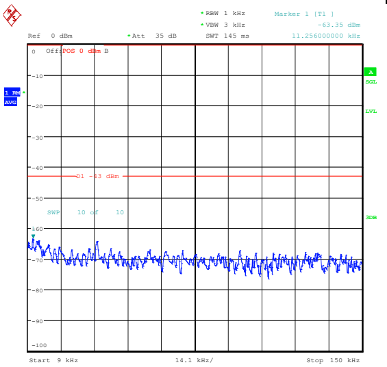
Band25_20MHz_QPSK_26140_100RB#0_1000~3000_000_1000~3000
