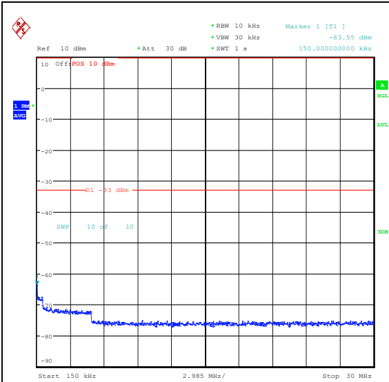
Band25_20MHz_16QAM_26140_1RB#0_0.15~3 0_0.15~30
