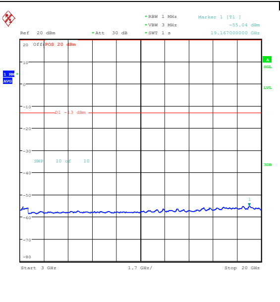
Band25_10MHz_16QAM_26640_1RB#49_3000~20000_0000_3000~20000
