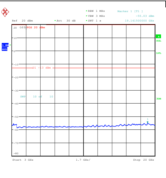
Band25_15MHz_16QAM_26115_75RB#0_3000~20000_0000_3000~20000
