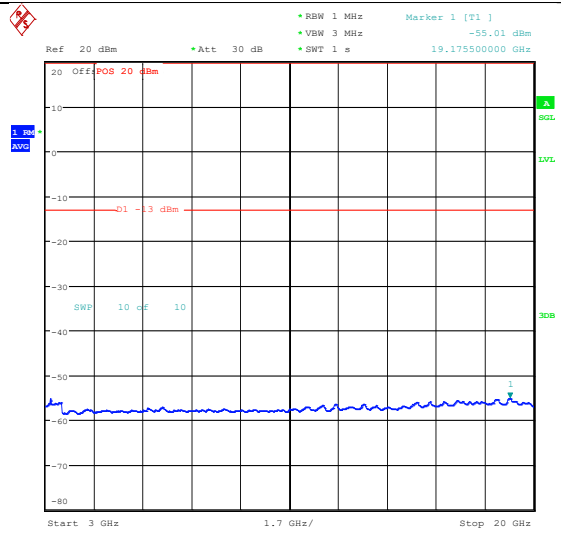
Band25_20MHz_16QAM_26140_1RB#99_3000~20000_3000~20000
