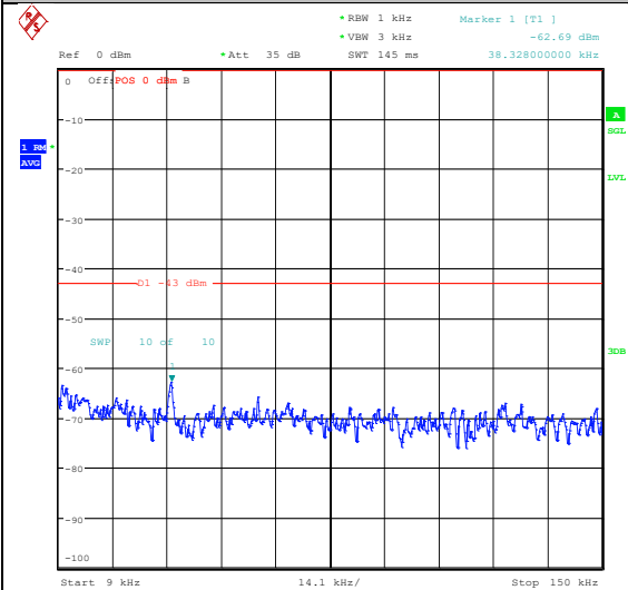
Band25_15MHz_16QAM_26615_75RB#0_1000~3000_1000~3000
