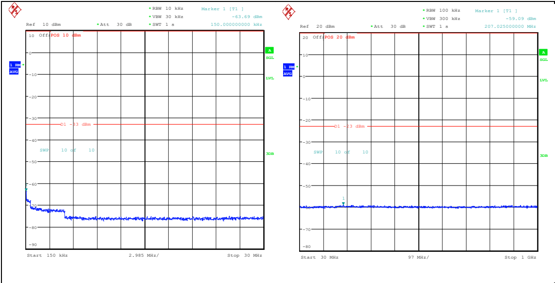
Band25_15MHz_16QAM_26615_1RB#74_0.15~30_0.15~30 Band25_15MHz_16QAM_26615_1RB#74_30~1000_0.30~1000
