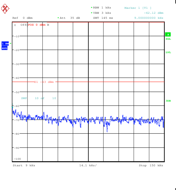
Band25_15MHz_16QAM_26115_1RB#74_0.009~ 0.15_0.009~0.15
