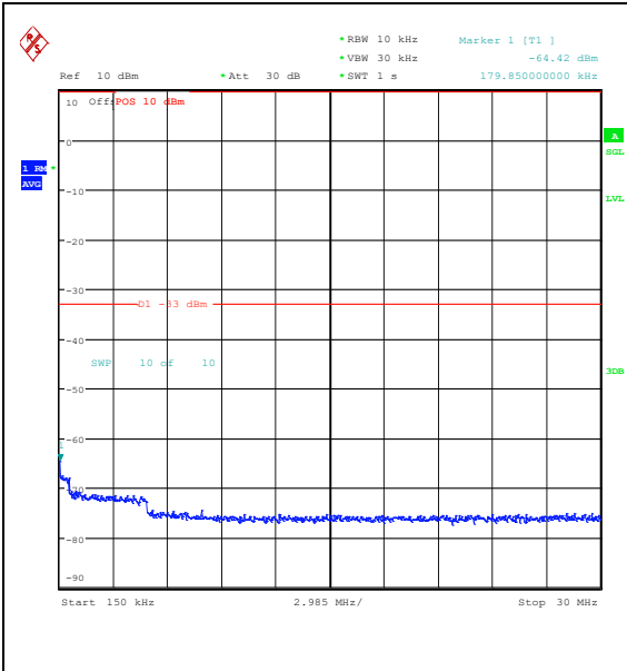
Band25_10MHz_16QAM_26640_50RB#0_0.15~ 30_0.15~30
