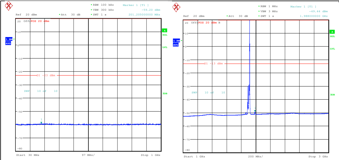
Band25_15MHz_QPSK_26615_1RB#74_30~100 0_30~1000 Band25_15MHz_QPSK_26615_1RB#74_1000~30 00_1000~3000
