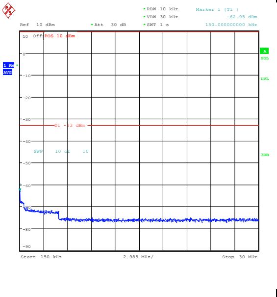
Band25_15MHz_QPSK_26365_1RB#0_0.15~30_0.15~30
