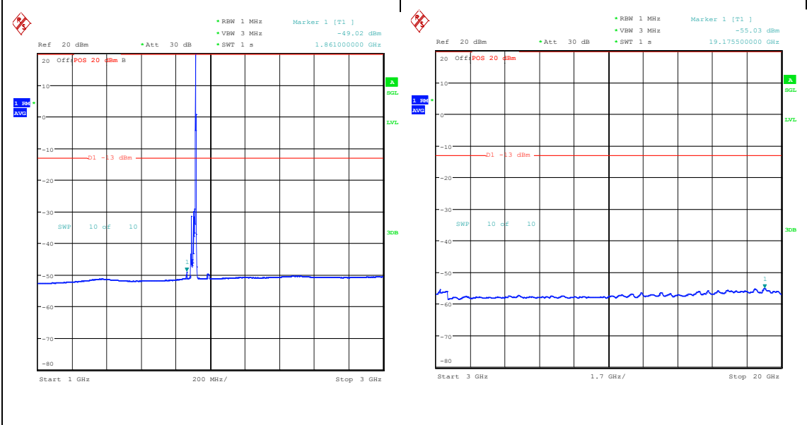
Band25_15MHz_16QAM_26615_1RB#74_1000~3000_1000~3000 Band25_15MHz_16QAM_26615_1RB#74_3000~20000_3000~20000
