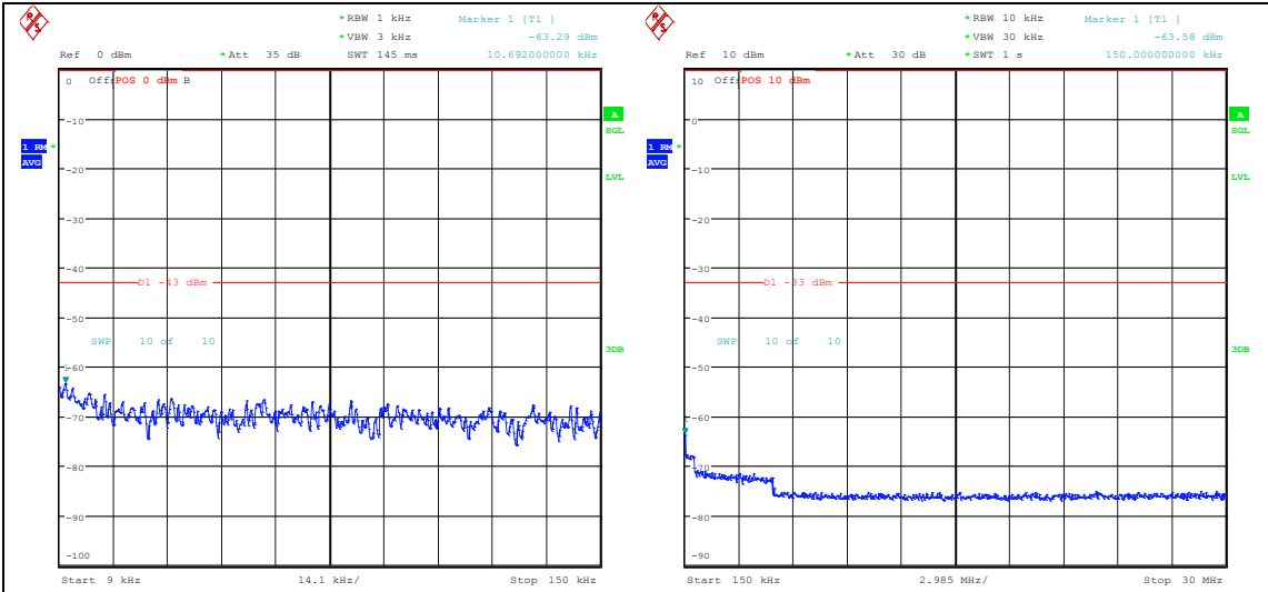
Band25_15MHz_QPSK_26115_1RB#0_0.009~0.15_0.009~0.15 Band25_15MHz_QPSK_26115_1RB#0_0.15~30_0.15~30
