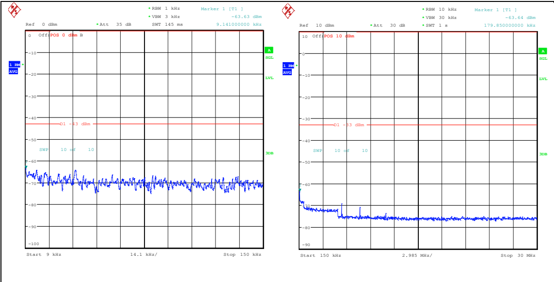
Band25_15MHz_QPSK_26615_75RB#0_0.009~0.15_0.009~0.15 Band25_15MHz_QPSK_26615_75RB#0_0.15~30_0.15~30
