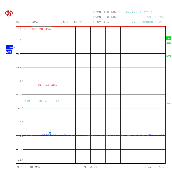
Band25_20MHz_QPSK_26140_100RB#0_30~1000_00_30~1000
