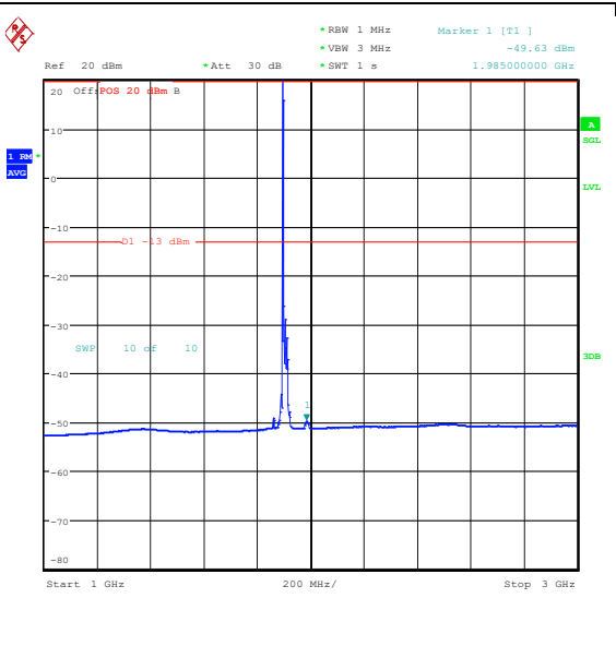
Band25_20MHz_QPSK_26590_1RB#0_1000~3000_0_1000~3000
