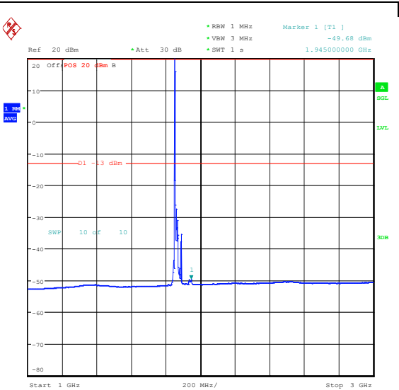
Band25_20MHz_QPSK_26140_1RB#0_1000~300_0_1000~3000
