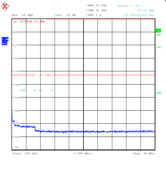
Band25_15MHz_QPSK_26115_1RB#74_0.15~30_0.15~30
