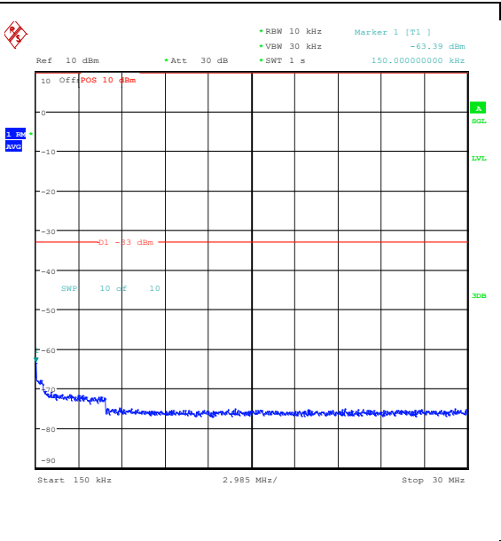
Band25_10MHz_QPSK_26640_1RB#49_0.15~30_0.15~30
