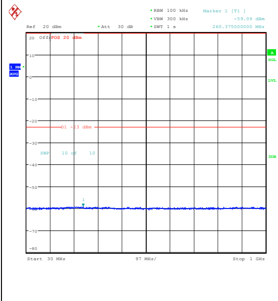
Band25_10MHz_QPSK_26365_50RB#0_30~100_0_30~1000
