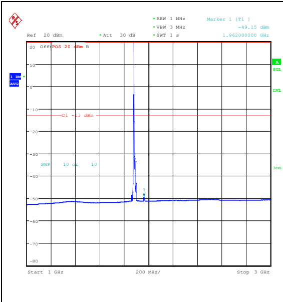
Band25_10MHz_16QAM_26365_1RB#0_1000~3000_1000~3000
