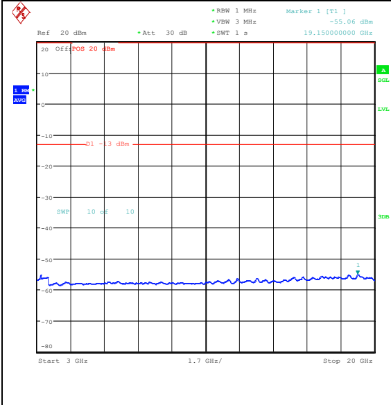
Band25_3MHz_QPSK_26055_1RB#0_3000~20000_3000~20000
