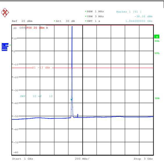
Band25_3MHz_QPSK_26055_15RB#0_1000~3000_0_1000~3000
