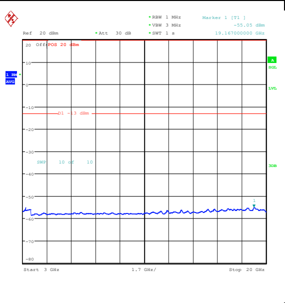
Band25_5MHz_16QAM_26365_25RB#0_3000~20000_3000~20000
