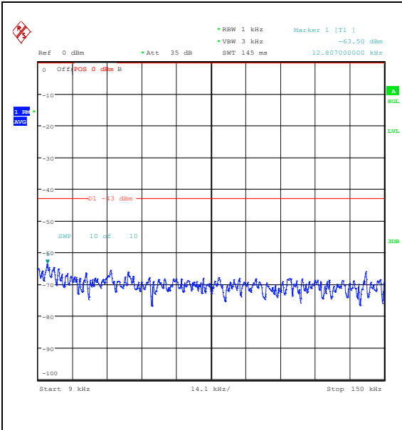
Band25_5MHz_QPSK_26665_25RB#0_0.009~0.15_0.009~0.15
