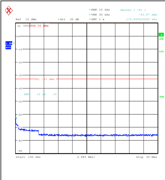
Band25_10MHz_16QAM_26640_1RB#0_0.15~3 0_0.15~30
