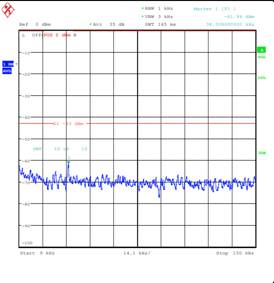
Band25_3MHz_16QAM_26055_1RB#0_0.009~0.15_0.009~0.15
