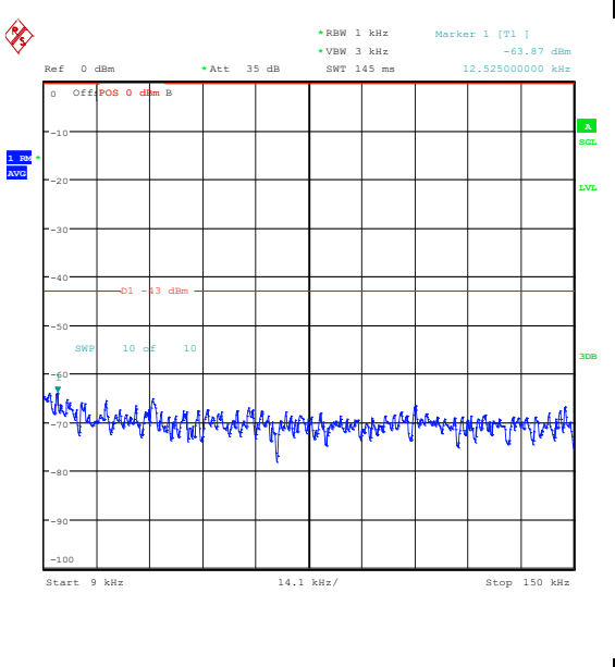
Band25_10MHz_16QAM_26640_1RB#0_0.009~0.15_0.009~0.15
