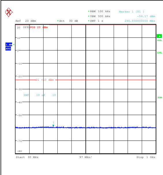
Band25_5MHz_QPSK_26665_25RB#0_30~1000_30~1000
