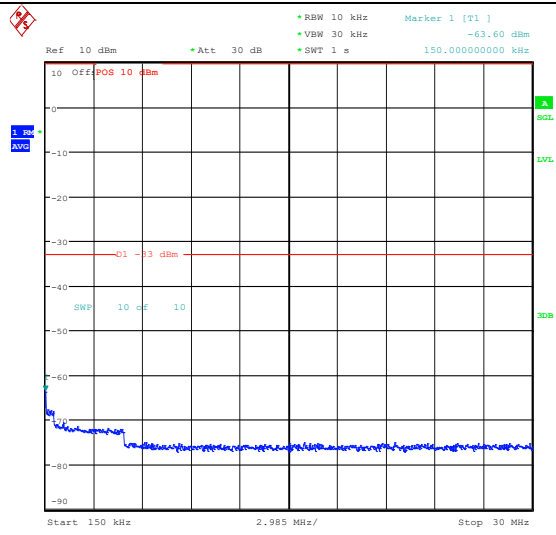
Band25_5MHz_QPSK_26065_1RB#0_0.15~30_0.15~30
