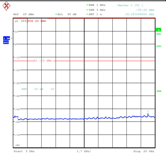
Band25_5MHz_16QAM_26365_1RB#0_3000~200_00_3000~20000
