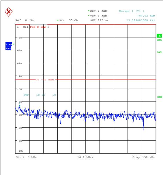
Band25_10MHz_QPSK_26090_1RB#49_0.009~0.15_0.009~0.15
