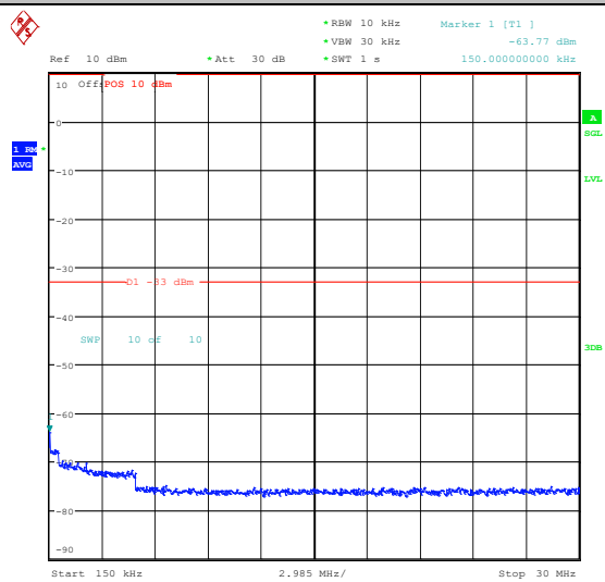
Band25_3MHz_16QAM_26055_1RB#14_3000~20000_3000~20000
