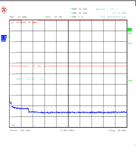
Band25_1.4MHz_QPSK_26683_6RB#0_0.15~30_0.15~30
