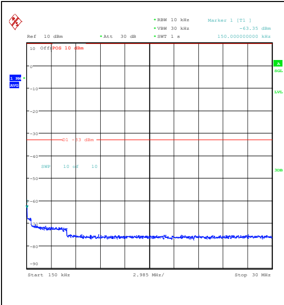
Band25_5MHz_16QAM_26365_1RB#0_0.15~30_0.15~30
