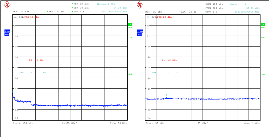
Band25_3MHz_16QAM_26365_1RB#14_0.15~3 0_0.15~30 Band25_3MHz_16QAM_26365_1RB#14_30~1000 _30~1000
