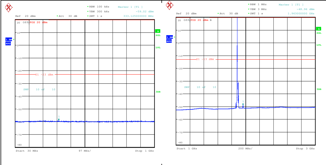
Band25_10MHz_QPSK_26365_1RB#0_30~1000_30~1000 Band25_10MHz_QPSK_26365_1RB#0_1000~3000_0_1000~3000
