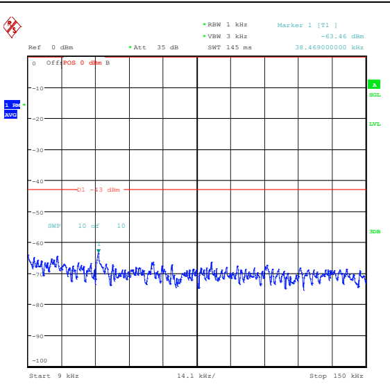
Band25_3MHz_16QAM_26055_1RB#14_0.009~0.15_0.009~0.15
