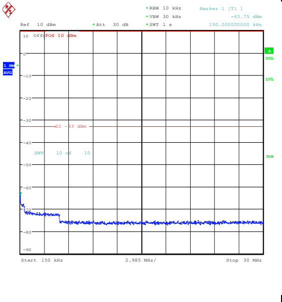
Band25_3MHz_QPSK_26365_1RB#14_0.15~30_0.15~30
