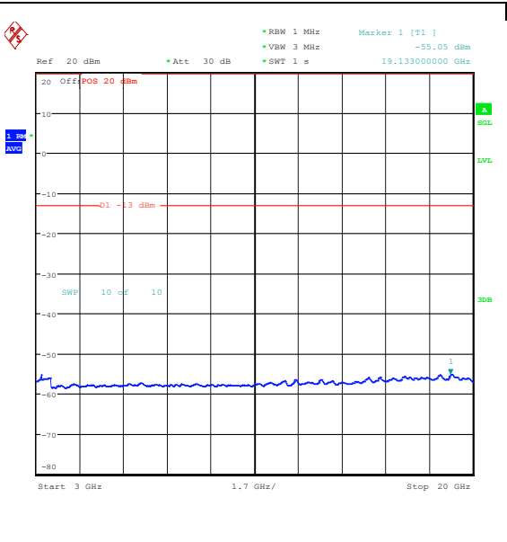
Band25_5MHz_16QAM_26365_1RB#24_3000~20000_3000~20000
