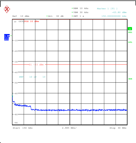
Band25_5MHz_QPSK_26665_25RB#0_0.15~30_0.15~30
