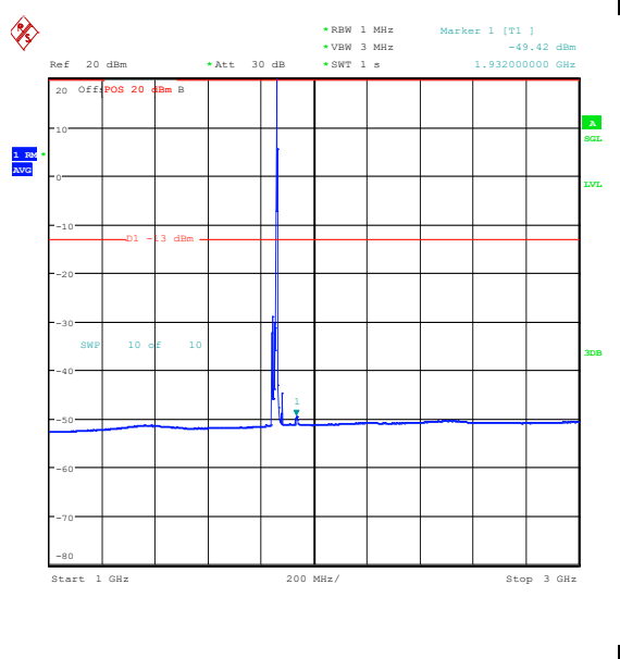
Band25_10MHz_QPSK_26090_1RB#49_1000~3000_1000~3000
