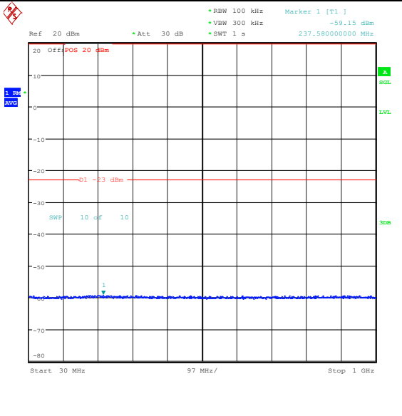
Band25_1.4MHz_16QAM_26683_6RB#0_30~100_30~100
