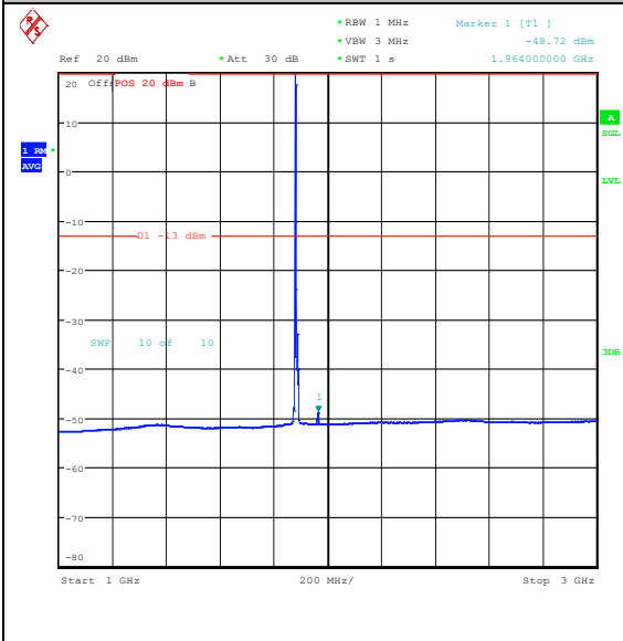
Band25_5MHz_16QAM_26365_1RB#0_1000~30_00_1000~3000
