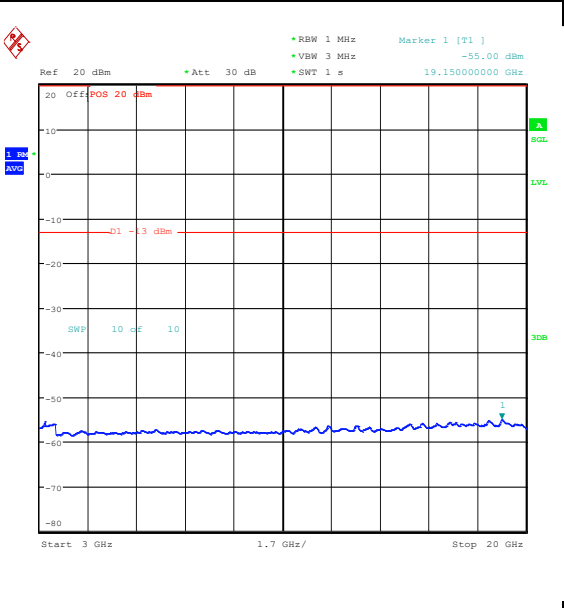
Band25_5MHz_16QAM_26665_1RB#24_3000~20 000_3000~20000
