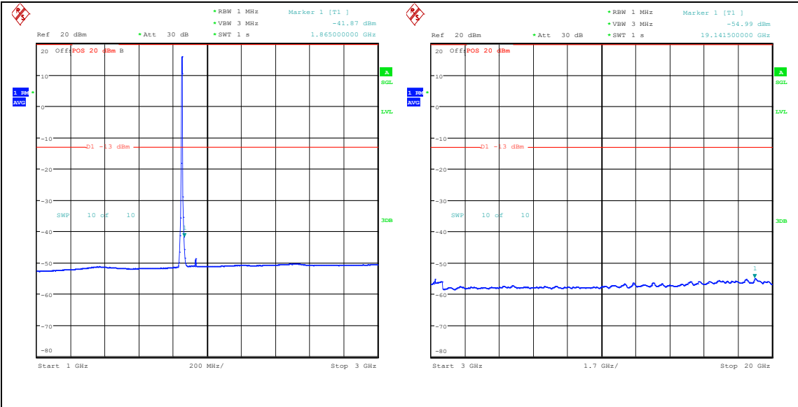
Band25_5MHz_16QAM_26065_25RB#0_1000~3000_1000~3000 Band25_5MHz_16QAM_26065_25RB#0_3000~20000_3000~20000
