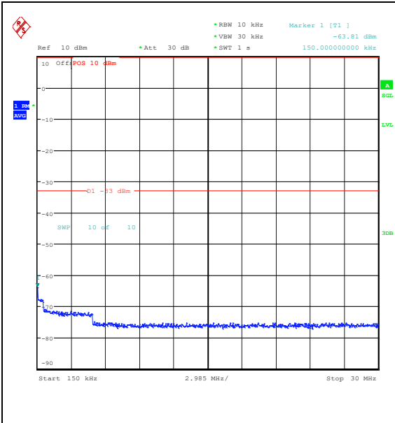
Band25_10MHz_16QAM_26090_1RB#0_0.15~3 0_0.15~30
