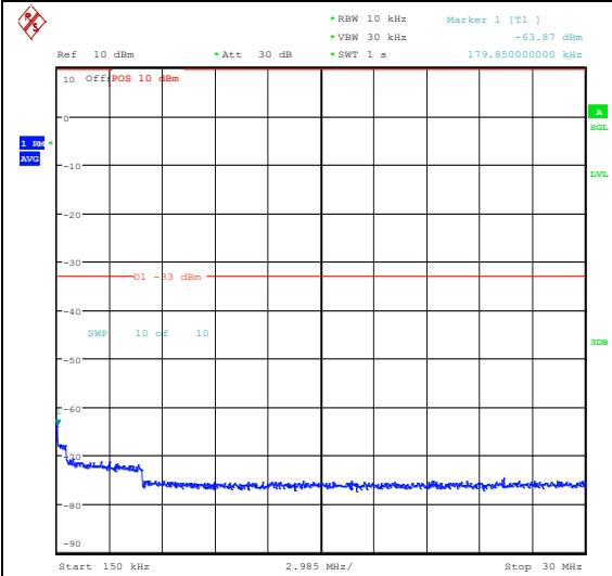
Band25_3MHz_QPSK_26675_1RB#14_3000~20000_3000~20000
