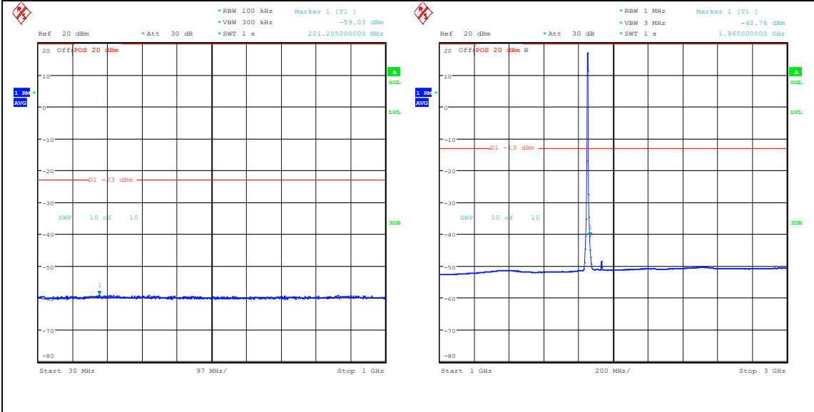
Band25_5MHz_QPSK_26065_25RB#0_30~1000_30~1000 Band25_5MHz_QPSK_26065_25RB#0_1000~3000_1000~3000
