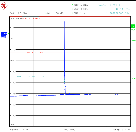
Band25_3MHz_QPSK_26675_15RB#0_1000~300_0_1000~3000
