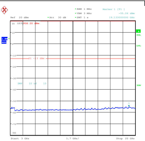
Band25_10MHz_16QAM_26090_1RB#49_3000~20000_0000_3000~20000
