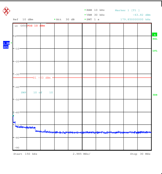
Band25_10MHz_QPSK_26365_50RB#0_0.15~30_0.15~30
