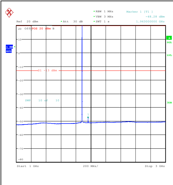
Band25_3MHz_16QAM_26365_1RB#0_1000~3000_00_1000~3000
