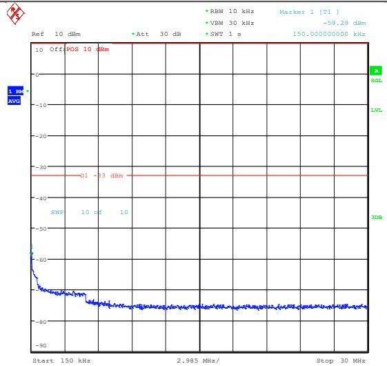
Band4_10MHz_16QAM_20350_1RB#49_3000~20000_000_3000~20000
