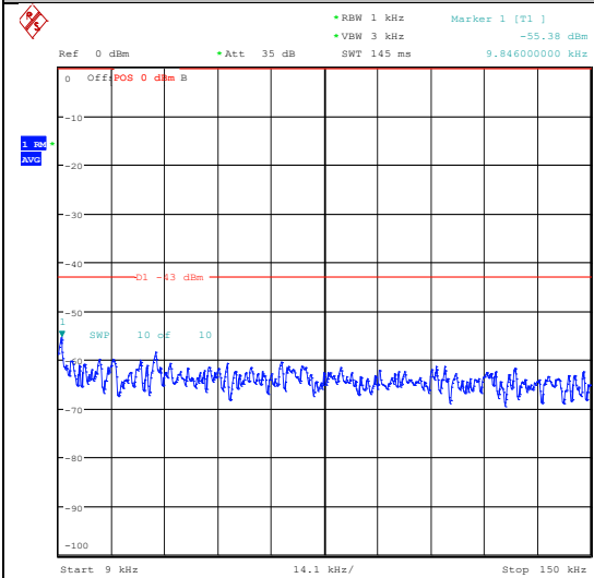
Band4_5MHz_16QAM_19975_1RB#0_1000~3000_1000~3000
