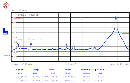
Band66_15MHz_QPSK_132597_1RB#0
