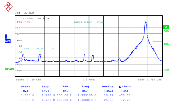
Band66_15MHz_16QAM_132597_1RB#0
