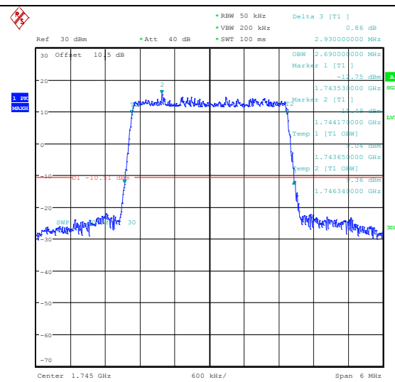
Band66-3MHz-16QAM-132322-15RB#0-PASS
