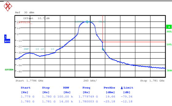
Band66_1.4MHz_16QAM_132665_1RB#0
