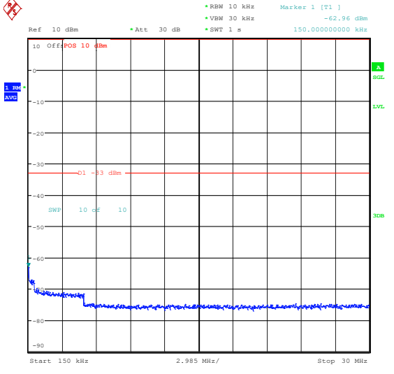
Band66_1.4MHz_16QAM_131979_1RB#0_3000~20000_3000~20000
