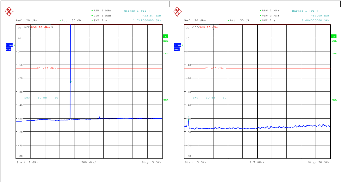
Band66_1.4MHz_16QAM_132322_1RB#5_1000 ~3000_1000~3000 Band66_1.4MHz_16QAM_132322_1RB#5_3000~ 20000_3000~20000
