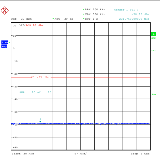
Band66_1.4MHz_16QAM_132322_6RB#0_30~1000_00_30~1000
