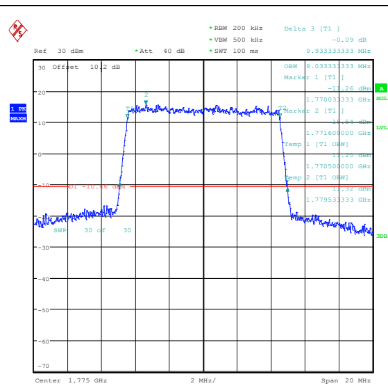
Band66-10MHz-16QAM-132622-50RB#0-PASS
