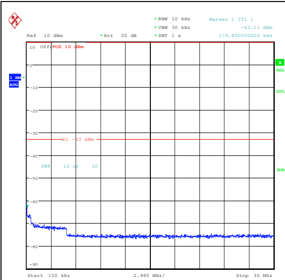
Band66_1.4MHz_16QAM_132322_6RB#0_0.15~30_0.15~30
