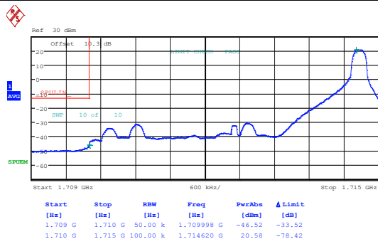
Band66_5MHz_QPSK_131997_1RB#0
