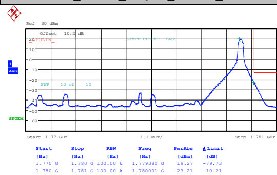
Band66_10MHz_16QAM_132622_1RB#0
