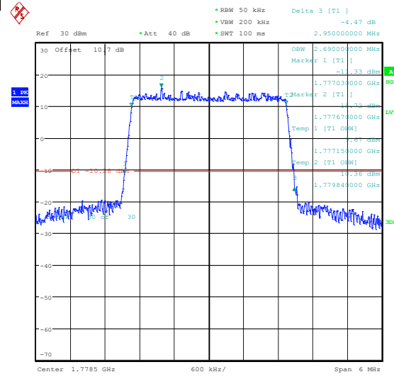
Band66-3MHz-16QAM-132322-15RB#0-PASS
