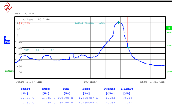
Band66_3MHz_16QAM_132657_1RB#0
