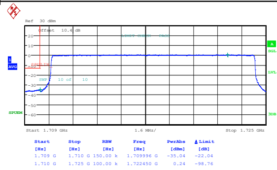
Band66_15MHz_16QAM_132047_1RB#74
