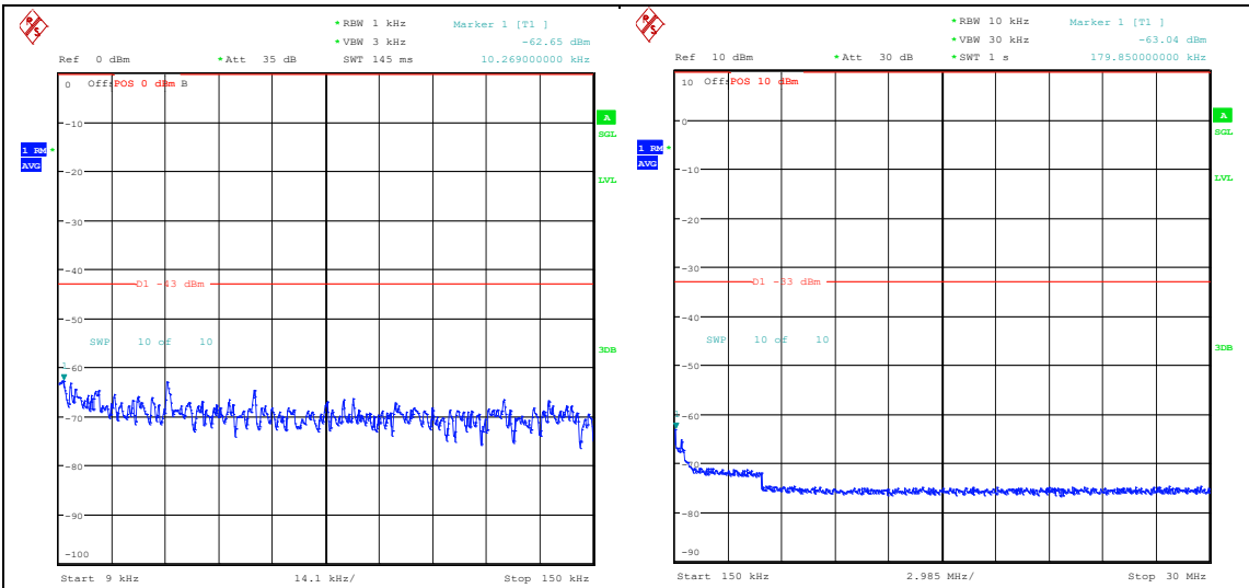
Band66_1.4MHz_QPSK_132665_6RB#0_0.009~0.15_0.009~0.15 Band66_1.4MHz_QPSK_132665_6RB#0_0.15~30_0.15~30
