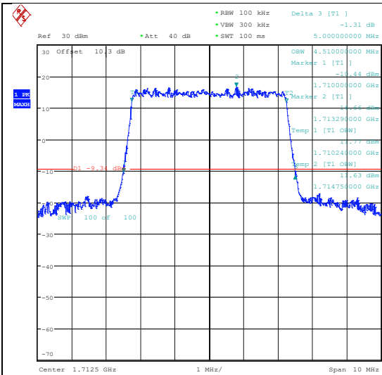
Band66-5MHz-QPSK-131997-25RB#0-PASS
