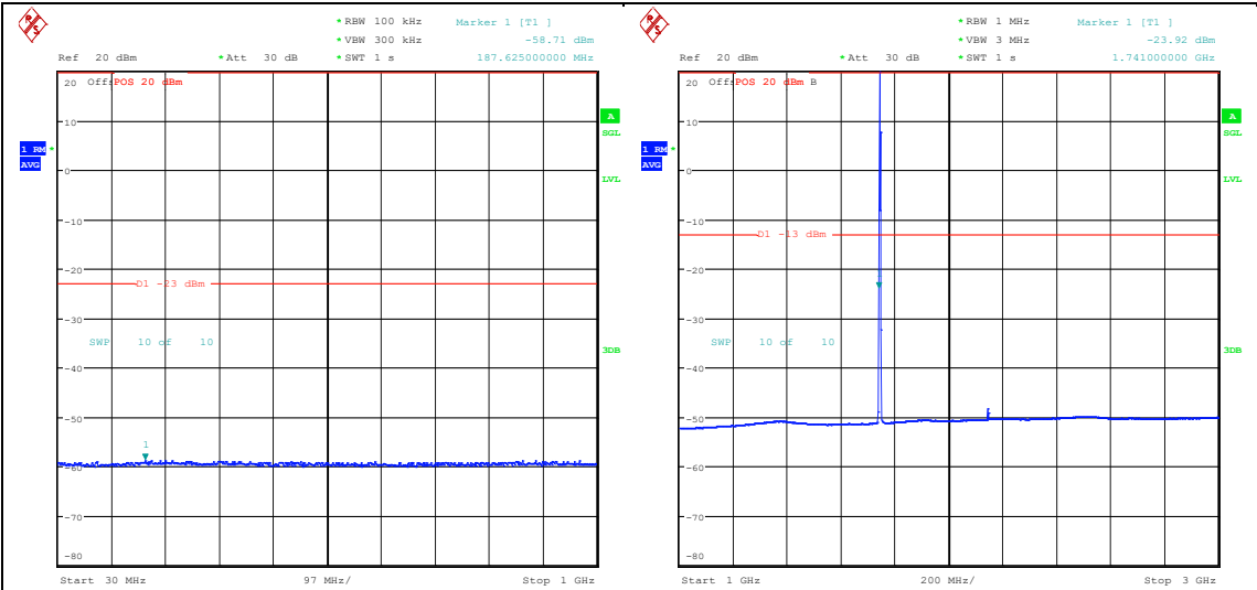
Band66_1.4MHz_QPSK_132322_1RB#0_30~100 0_30~1000 Band66_1.4MHz_QPSK_132322_1RB#0_1000~3 000_1000~3000
