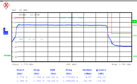
Band66_5MHz_16QAM_132647_1RB#24
