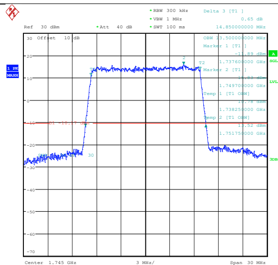
Band66-15MHz-16QAM-132322-75RB#0-PASS
