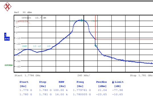
Band66_1.4MHz_QPSK_132665_1RB#0
