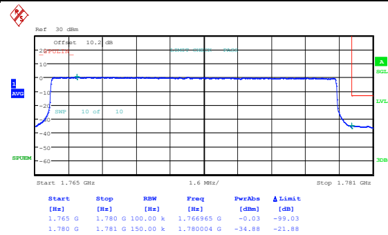
Band66_15MHz_16QAM_132597_1RB#74
