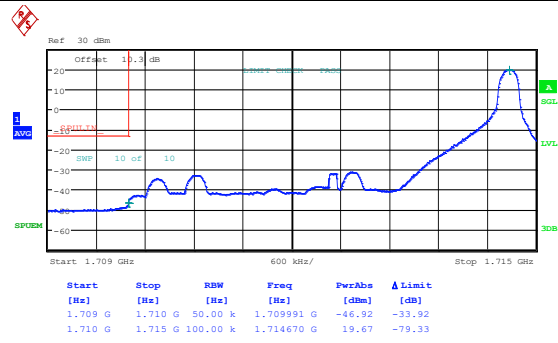
Band66_5MHz_16QAM_131997_1RB#0
