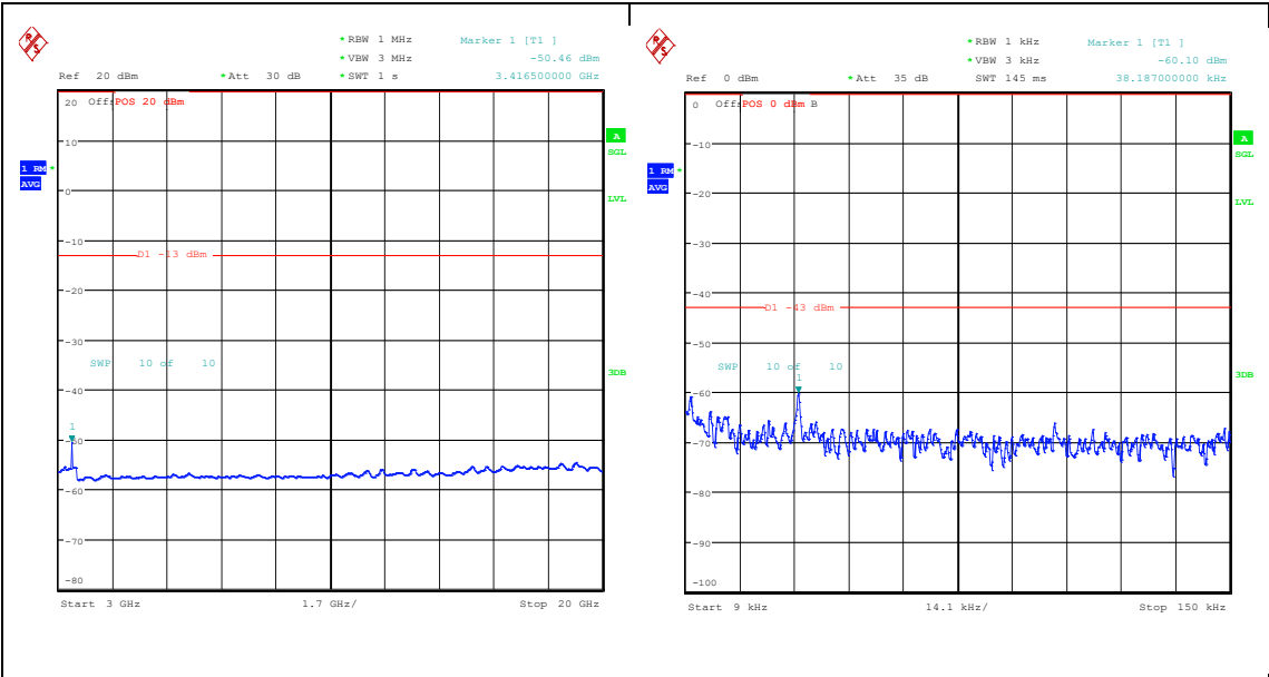
Band66_1.4MHz_QPSK_131979_6RB#0_3000~20000_3000~20000 Band66_1.4MHz_16QAM_131979_6RB#0_0.009~0.15_0.009~0.15
