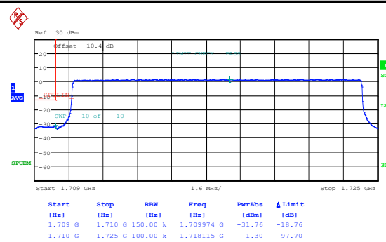
Band66_15MHz_QPSK_132047_1RB#74
