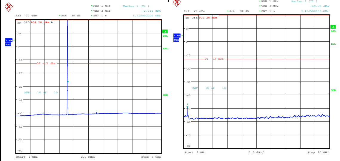
Band66_1.4MHz_16QAM_131979_1RB#5_1000~3000_1000~3000 Band66_1.4MHz_16QAM_131979_1RB#5_3000~20000_3000~20000
