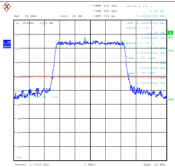
Band66-5MHz-16QAM-131997-25RB#0-PASS
