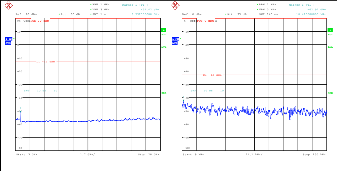
Band66_15MHz_QPSK_132597_1RB#74_3000~20000_20000_3000~20000 Band66_15MHz_16QAM_132597_1RB#74_0.009~0.15_0.009~0.15
