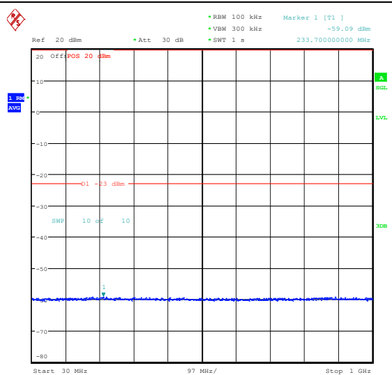
Band66_15MHz_16QAM_132597_1RB#74_30~10 00_30~1000
