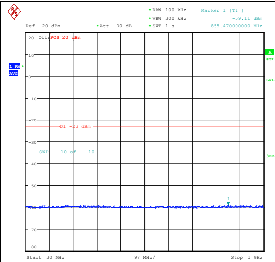
Band66_15MHz_QPSK_132322_1RB#0_30~1000_0_30~1000
