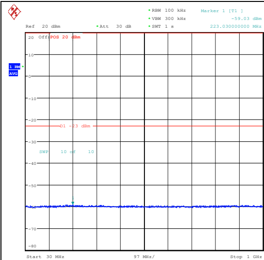
Band66_15MHz_QPSK_132322_75RB#0_30~1000_30~1000
