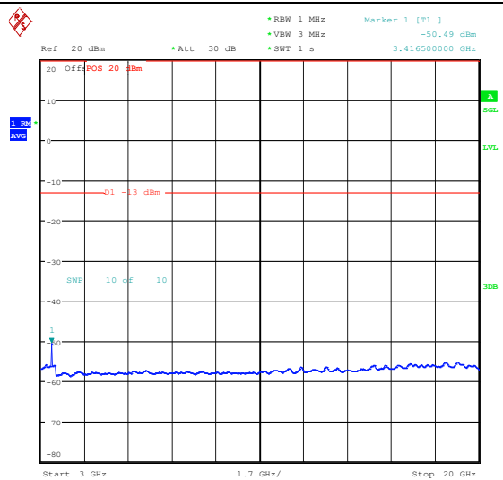
Band66_15MHz_16QAM_132047_1RB#0_3000~20000_3000~20000
