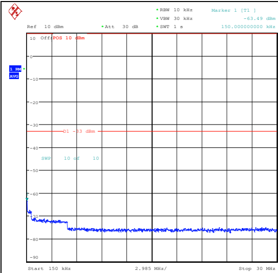
Band66_20MHz_16QAM_132072_1RB#0_0.15~30_0.15~30
