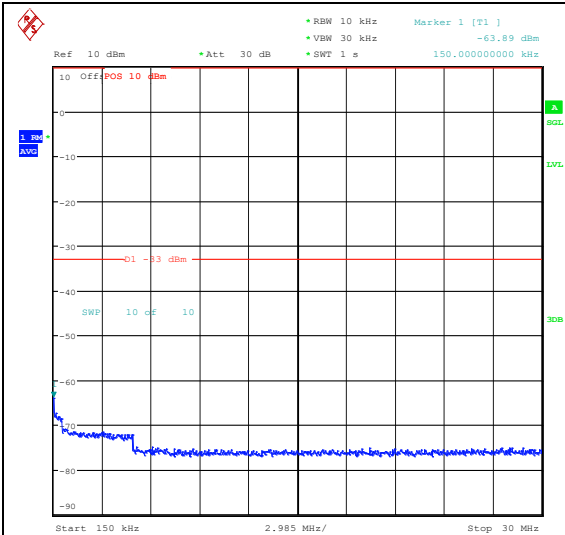
Band66_20MHz_16QAM_132572_1RB#0_0.15~30_0.15~30
