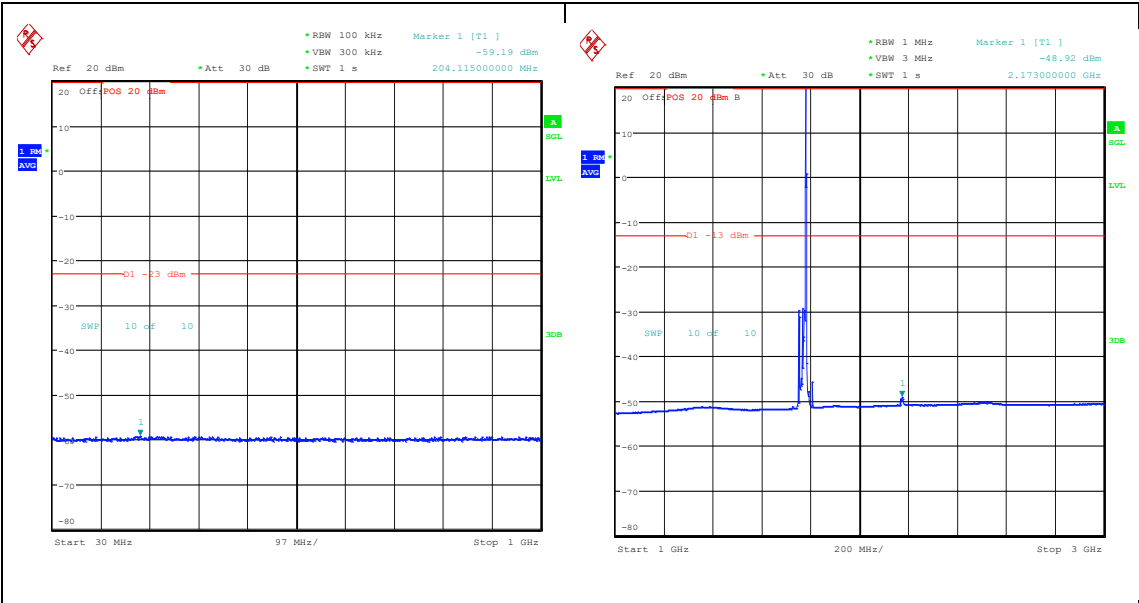
Band66_15MHz_QPSK_132597_1RB#74_30~1000_00_30~1000 Band66_15MHz_QPSK_132597_1RB#74_1000~3000_000_1000~3000
