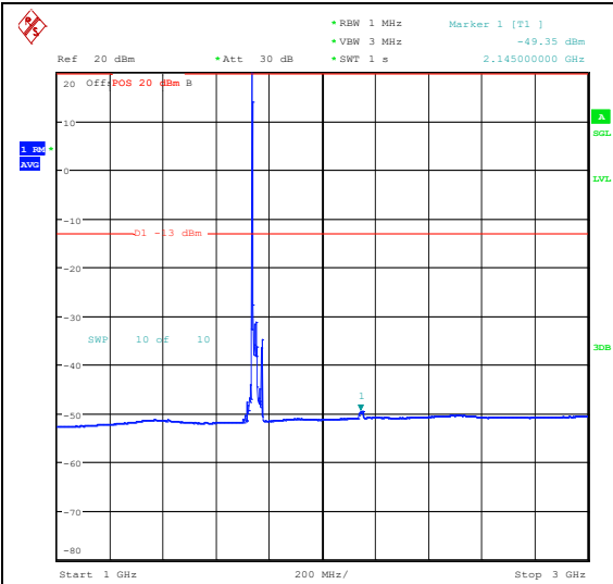
Band66_20MHz_16QAM_132322_1RB#0_1000~3000_1000~3000
