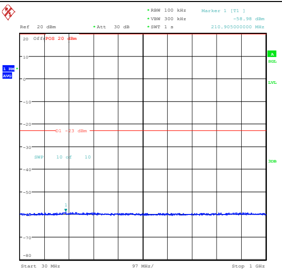
Band66_20MHz_16QAM_132072_1RB#0_30~1000_0_30~1000
