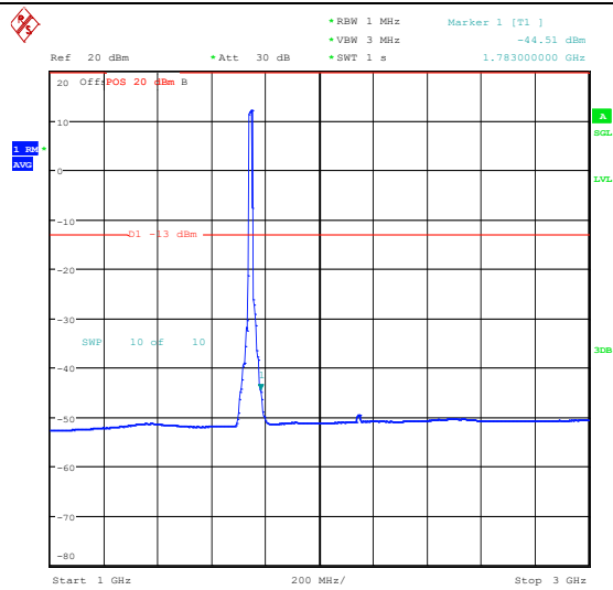
Band66_15MHz_QPSK_132322_75RB#0_1000~3000_1000~3000
