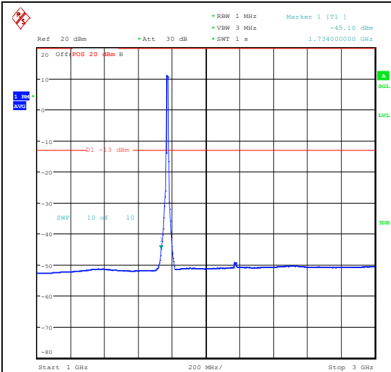
Band66_15MHz_16QAM_132597_75RB#0_1000 ~3000_1000~3000
