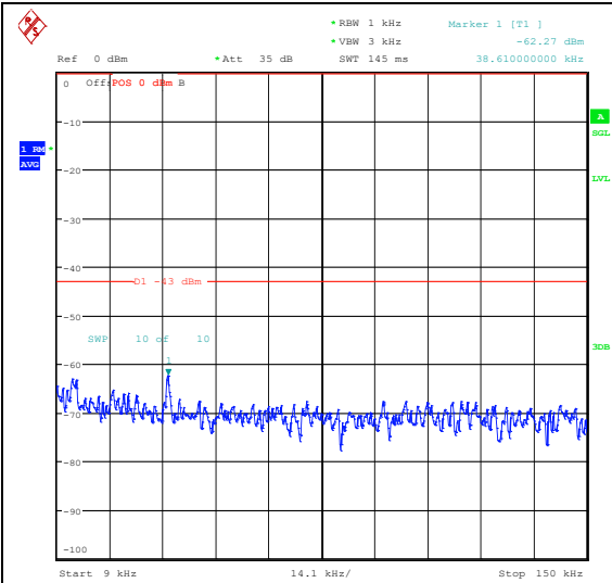
Band66_15MHz_QPSK_132047_75RB#0_0.009~0.15_0.009~0.15
