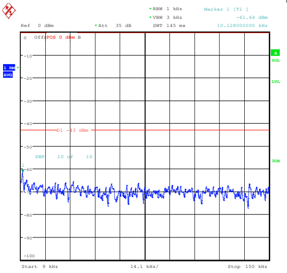
Band66_15MHz_QPSK_132322_1RB#0_1000~3000_00_1000~3000
