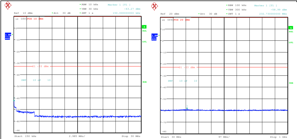
Band66_15MHz_16QAM_132322_1RB#0_0.15~30_0.15~30
