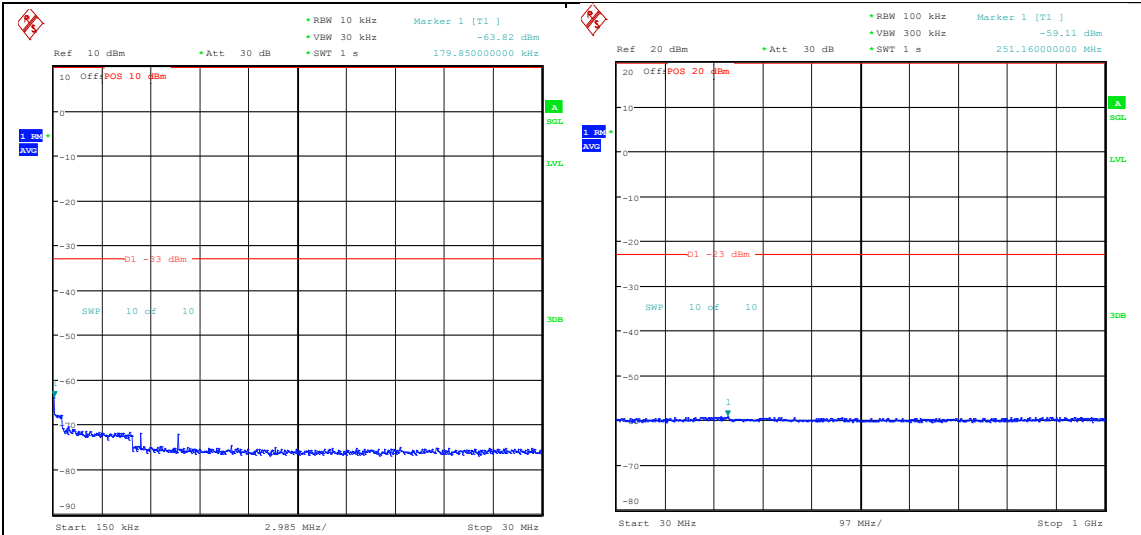
Band66_15MHz_16QAM_132322_75RB#0_0.15 ~30_0.15~30
