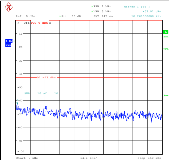
Band66_15MHz_QPSK_132597_75RB#0_0.009~0.15_0.009~0.15
