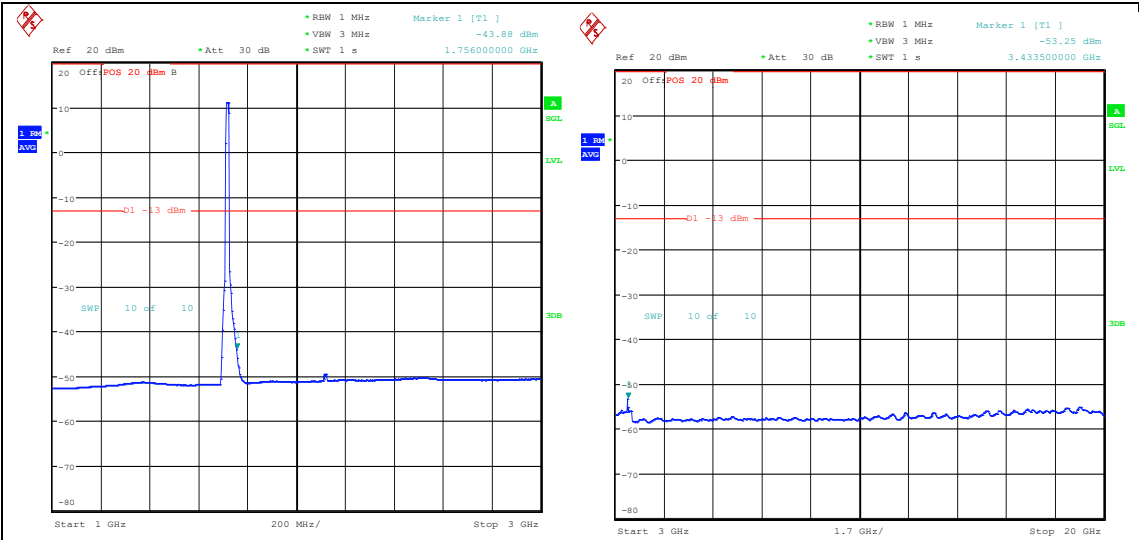
Band66_15MHz_16QAM_132047_75RB#0_1000~3000_1000~3000 Band66_15MHz_16QAM_132047_75RB#0_3000~20000_3000~20000
