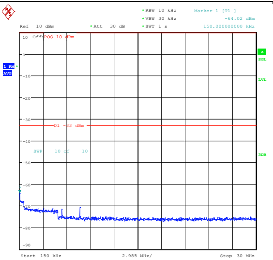
Band66_15MHz_QPSK_132047_75RB#0_0.15~3_0_0.15~30
