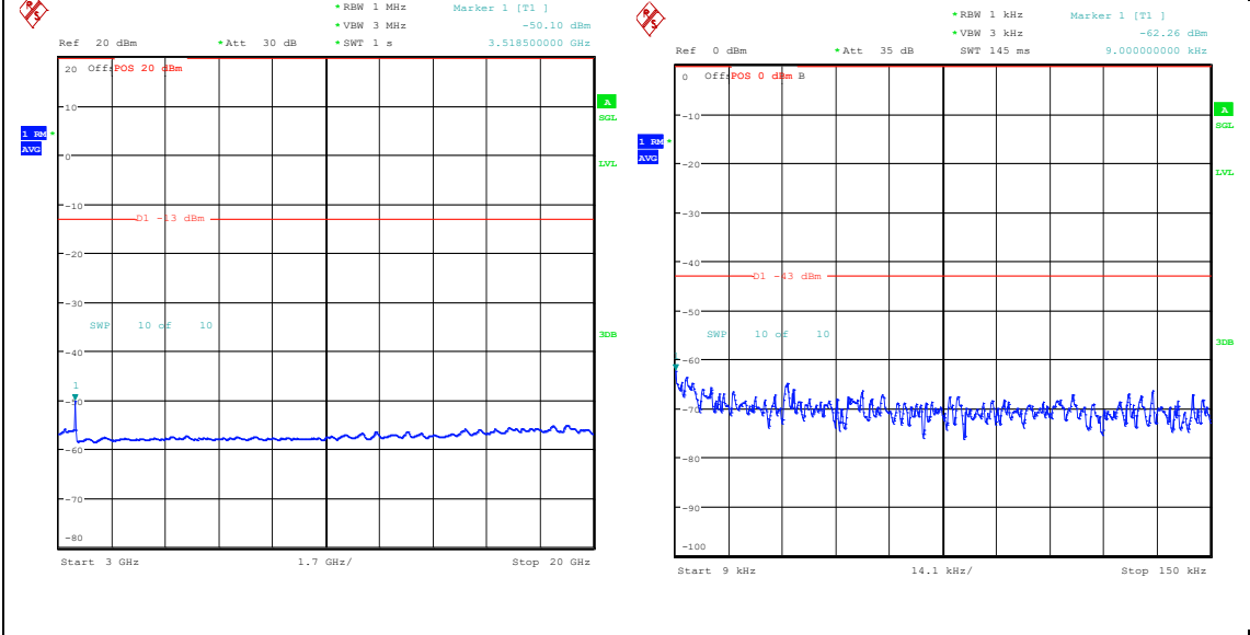
Band66_20MHz_QPSK_132572_1RB#0_3000~2 0000_3000~20000 Band66_20MHz_16QAM_132572_1RB#0_0.009~ 0.15_0.009~0.15
