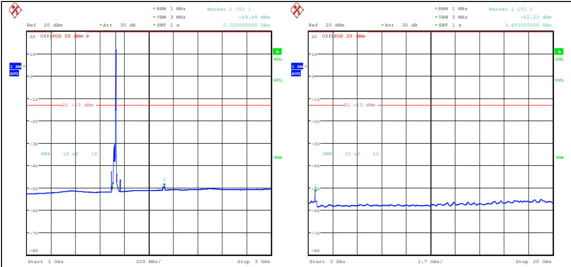
Band66_20MHz_16QAM_132072_1RB#99_1000~3000_1000~3000 Band66_20MHz_16QAM_132072_1RB#99_3000~20000_3000~20000
