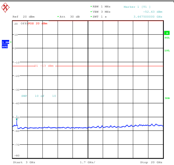
Band66_20MHz_16QAM_132322_1RB#0_3000~20000_3000~20000
