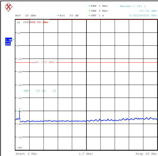
Band66_15MHz_QPSK_132322_1RB#74_3000~20000_3000~20000
