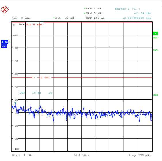
Band66_15MHz_16QAM_132047_75RB#0_0.009~-0.15_0.009~0.15
