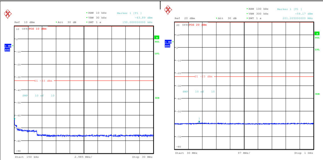
Band66_20MHz_16QAM_132322_1RB#99_0.15 ~30_0.15~30 Band66_20MHz_16QAM_132322_1RB#99_30~10 00_30~1000
