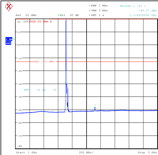
Band66_15MHz_16QAM_132047_1RB#0_1000~3000_1000~3000
