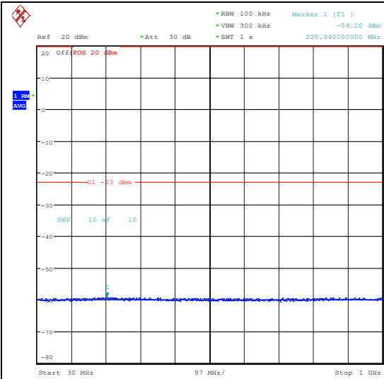
Band66_15MHz_QPSK_132047_1RB#74_30~1000_30~1000
