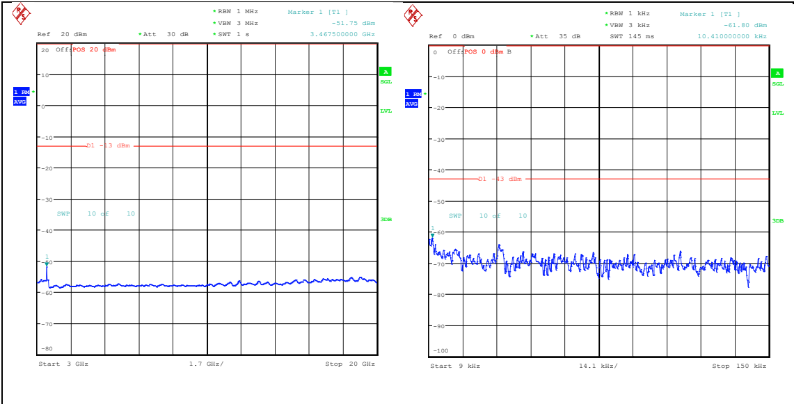
Band66_20MHz_QPSK_132322_1RB#0_3000~20000_3000~20000 Band66_20MHz_16QAM_132322_1RB#0_0.009~0.15_0.009~0.15
