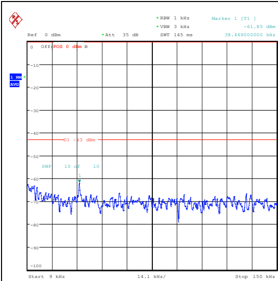
Band66_20MHz_QPSK_132322_100RB#0_0.009 ~0.15_0.009~0.15
