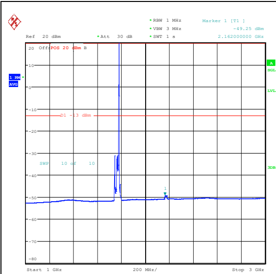
Band66_20MHz_16QAM_132572_1RB#99_1000 ~3000_1000~3000
