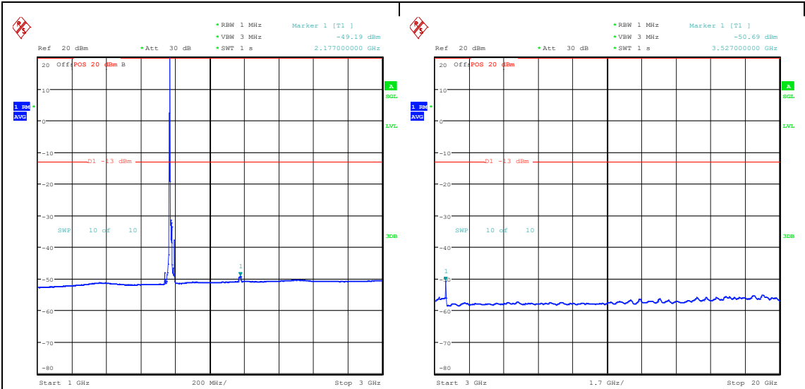
Band66_15MHz_16QAM_132597_1RB#0_1000~3000_1000~3000 Band66_15MHz_16QAM_132597_1RB#0_3000~20000_3000~20000
