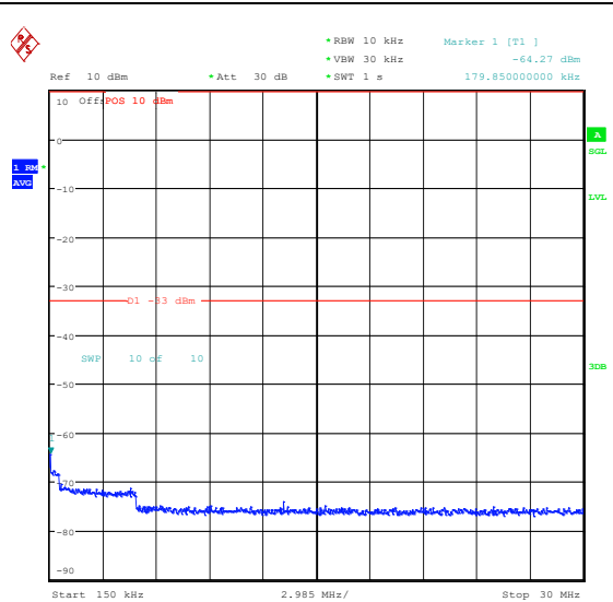
Band66_20MHz_QPSK_132322_100RB#0_0.15~30 30_0.15~30
