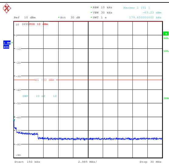
Band66_15MHz_QPSK_132322_1RB#74_0.15~3 0_0.15~30
