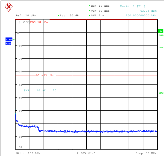
Band66_15MHz_16QAM_132597_1RB#74_0.15 ~30_0.15~30
