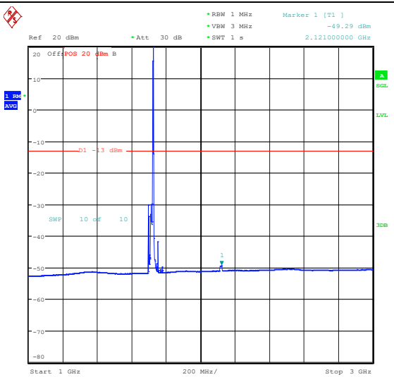
Band66_15MHz_QPSK_132047_1RB#74_1000~3000_1000~3000
