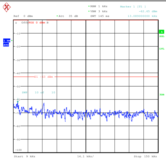
Band66_20MHz_16QAM_132322_100RB#0_0.00 9~0.15_0.009~0.15
