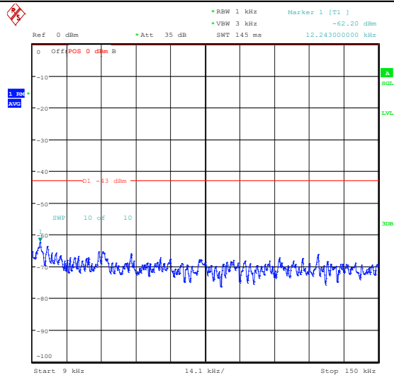
Band66_20MHz_QPSK_132572_100RB#0_1000~3000_1000~3000
