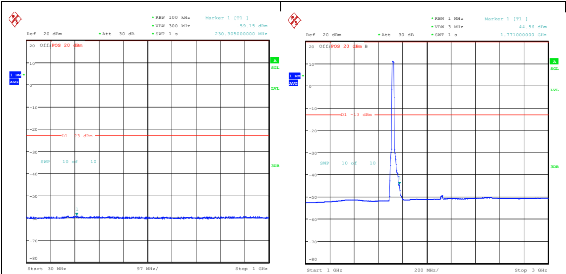
Band66_20MHz_QPSK_132072_100RB#0_30~1000_30~1000 Band66_20MHz_QPSK_132072_100RB#0_1000~3000_1000~3000
