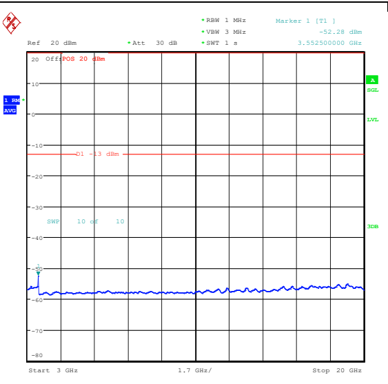
Band66_20MHz_16QAM_132572_1RB#99_3000~ 20000_3000~20000
