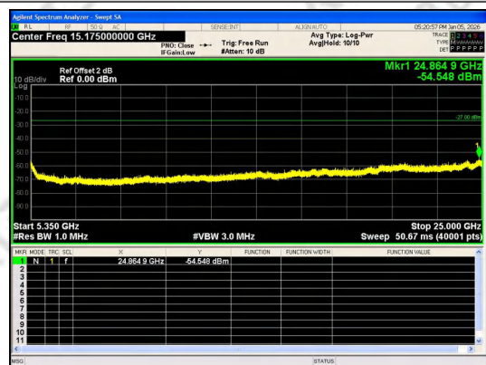
Spurious Emission:5350~25000.0 MHz IEEE 802.11ax_Channel 42_80MHz_Antenna 0_RU&Index SU
