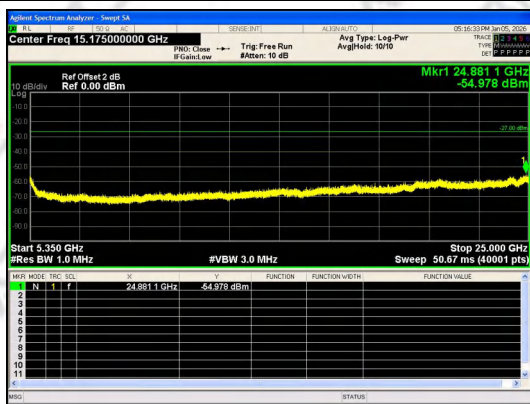
Spurious Emission:5350~25000.0 MHz IEEE 802.11ax_Channel 46_40MHz_Antenna 0_RU&Index SU
