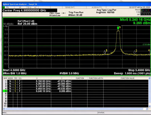
Out Of Band Emission IEEE 802.11ax_Channel 48_20MHz_Antenna 0_RU&Index SU
