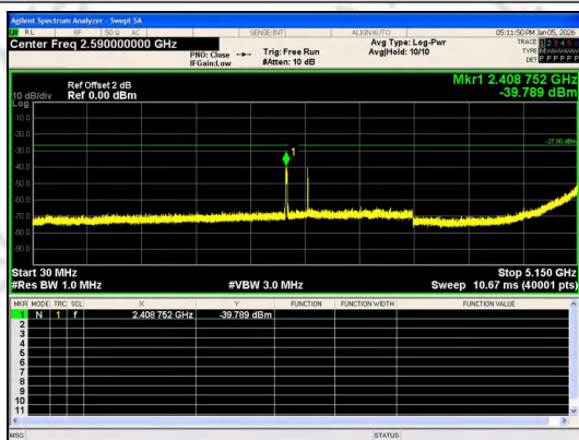
Spurious Emission:30.0~5150 MHz IEEE 802.11ax_Channel 38_40MHz_Antenna 0_RU&Index SU
