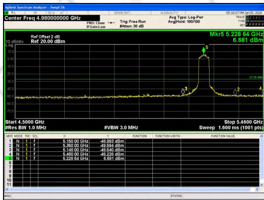
Out Of Band Emission IEEE 802.11ax_Channel 46_40MHz_Antenna 0_RU&Index SU
