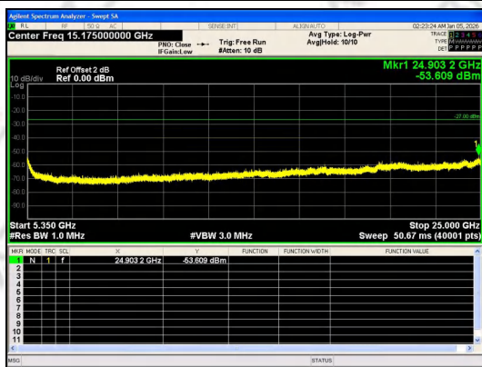
Spurious Emission:5350~25000.0 MHz IEEE 802.11ax_Channel 48_20MHz_Antenna 0_RU&Index SU
