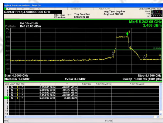
Out Of Band Emission IEEE 802.11ax_Channel 42_80MHz_Antenna 0_RU&Index SU
