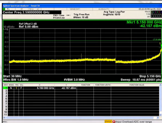
Spurious Emission:30.0~5150 MHz IEEE 802.11ax_Channel 42_80MHz_Antenna 0_RU&Index SU
