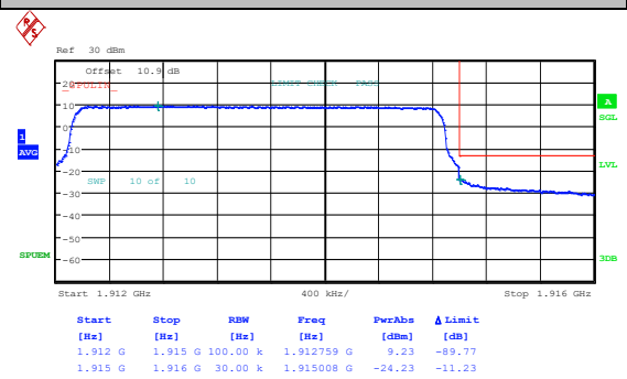
Band25_3MHz_16QAM_26675_1RB#14
