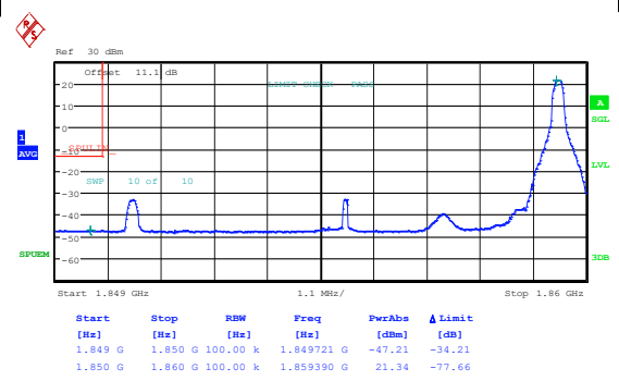
Band25_10MHz_16QAM_26090_1RB#0
