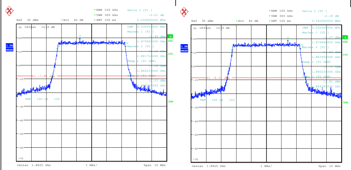
Band25-5MHz-QPSK-26065-25RB#0-PASS Band25-5MHz-16QAM-26065-25RB#0-PASS
