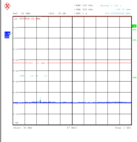
Band25_1.4MHz_QPSK_26365_1RB#0_30~1000_30~1000
