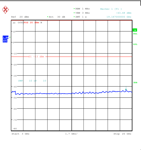
Band25_1.4MHz_16QAM_26365_1RB#0_3000~20000_3000~20000
