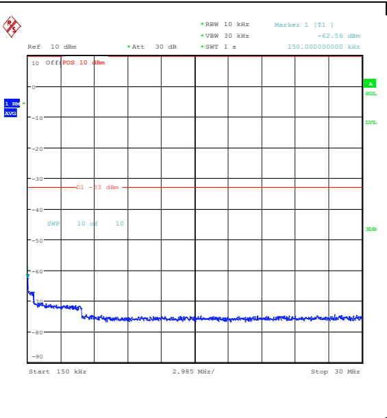
Band25_1.4MHz_QPSK_26365_1RB#0_0.15~30_0.15~30
