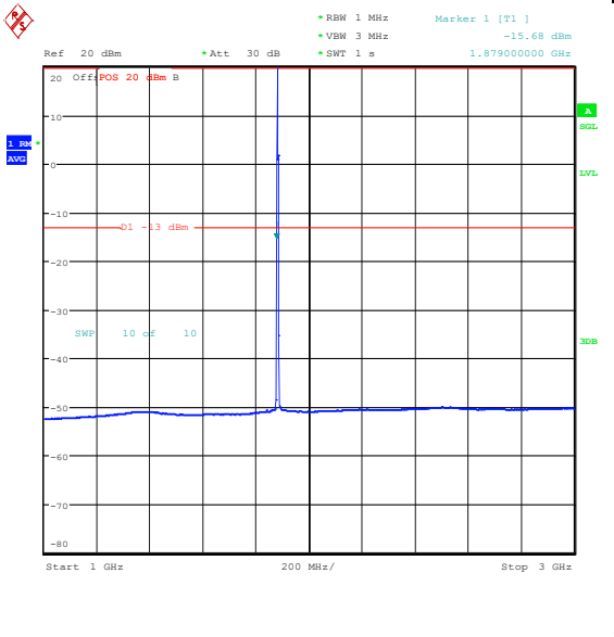
Band25_1.4MHz_QPSK_26365_1RB#0_1000~3000_1000~3000
