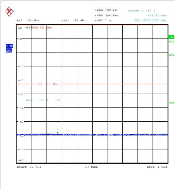
Band25_1.4MHz_QPSK_26047_1RB#0_30~1000_30~1000
