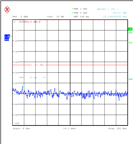
Band25_1.4MHz_QPSK_26365_1RB#0_0.009~0.15_15_0.009~0.15
