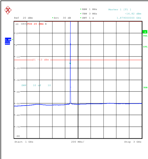
Band25_1.4MHz_16QAM_26365_1RB#0_1000~3000_1000~3000
