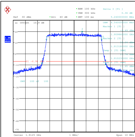
Band25-5MHz-QPSK-26665-25RB#0-PASS
