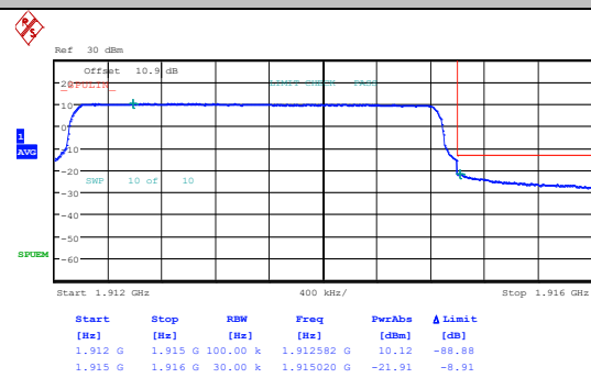
Band25_3MHz_QPSK_26675_1RB#14
