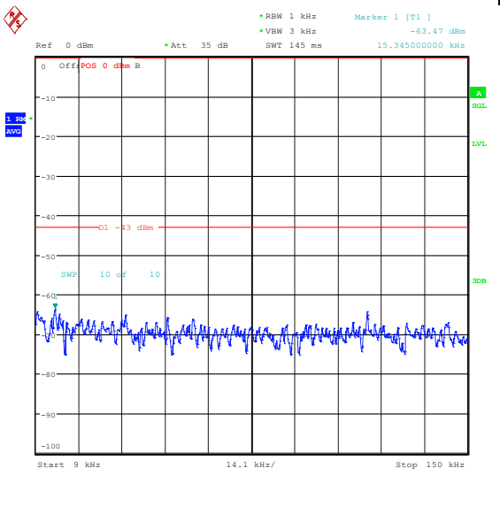
Band25_1.4MHz_16QAM_26047_1RB#0_0.009~0.15_0.009~0.15
