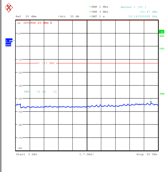
Band25_1.4MHz_QPSK_26047_1RB#0_3000~20000_000_3000~20000
