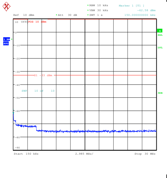
Band25_1.4MHz_QPSK_26683_1RB#0_0.15~30_0.15~30
