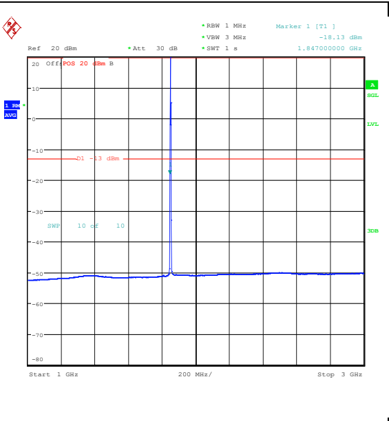
Band25_1.4MHz_QPSK_26047_1RB#0_1000~3000_00_1000~3000
