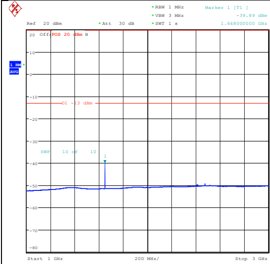
Band26_3MHz_16QAM_26805_1RB#0_0.15~30_0.15~30
