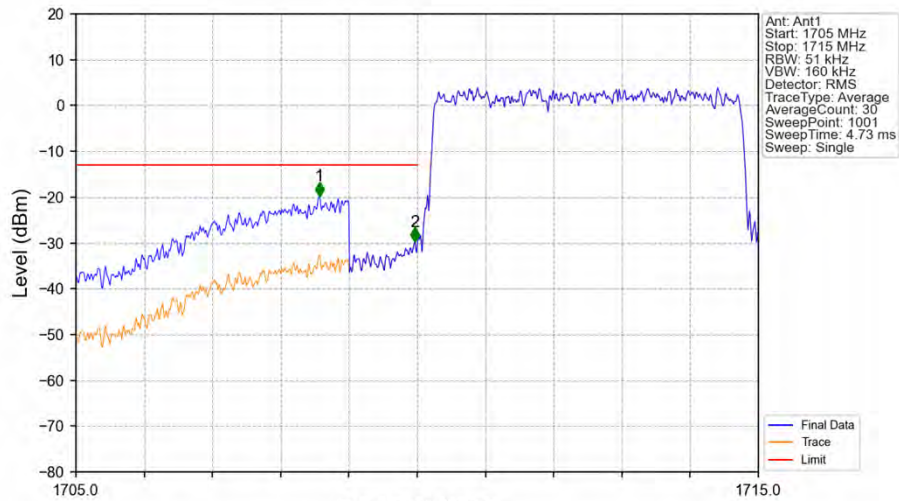
Band66_5MHz_16QAM_LCH_1712.5MHz_RB_25_0_NTNV
