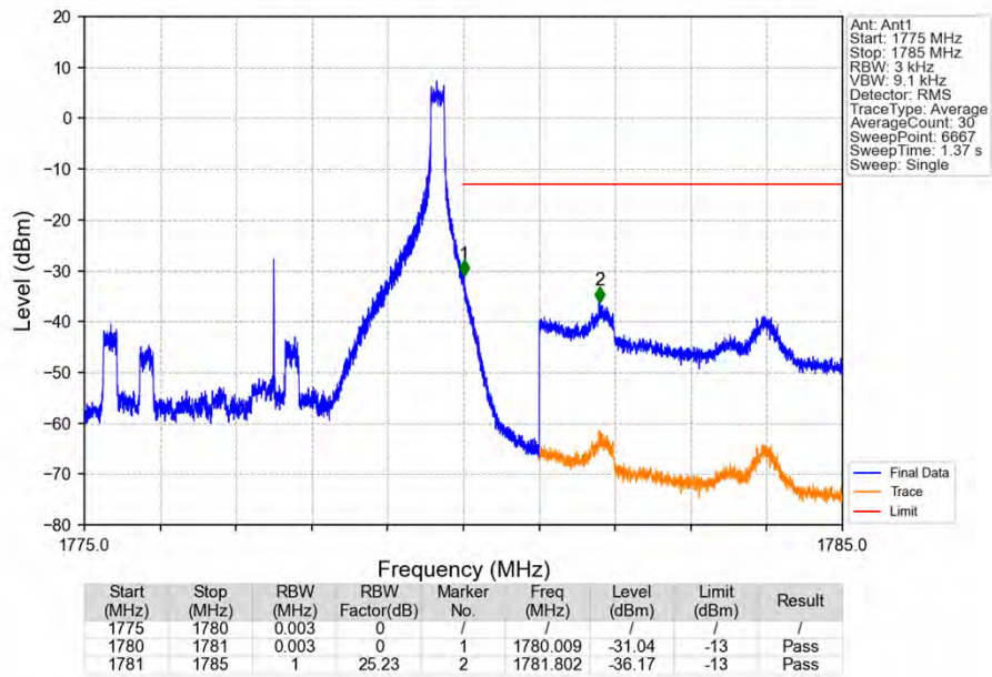
Band66_5MHz_16QAM_HCH_1777.5MHz_RB_1_24_NTNV
