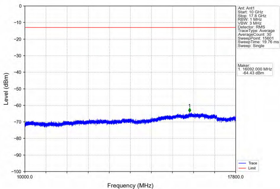
Band66_10MHz_QPSK_LCH_1715MHz_RB_50_0_NTNV
