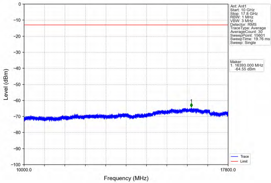
Band66_5MHz_QPSK_LCH_1712.5MHz_RB_25_0_NTNV
