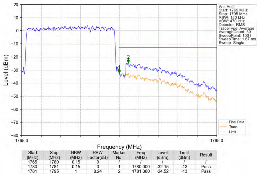
Band66_15MHz_16QAM_HCH_1772.5MHz_RB_75_0_NTNV
