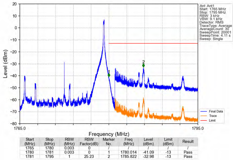
Band66_15MHz_QPSK_HCH_1772.5MHz_RB_1_74_NTNV
