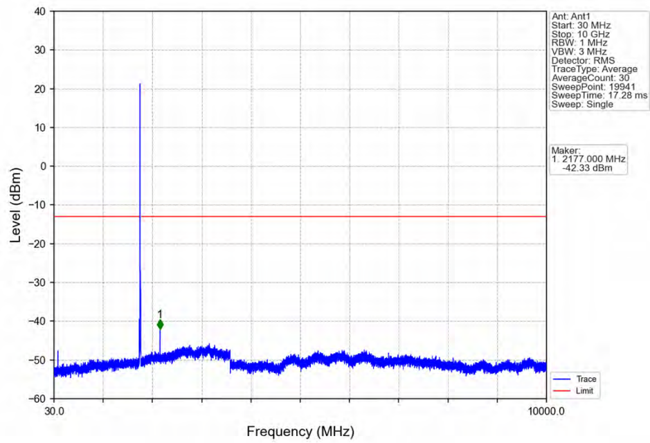
Band66_10MHz_QPSK_HCH_1775MHz_RB_1_0_NTNV
