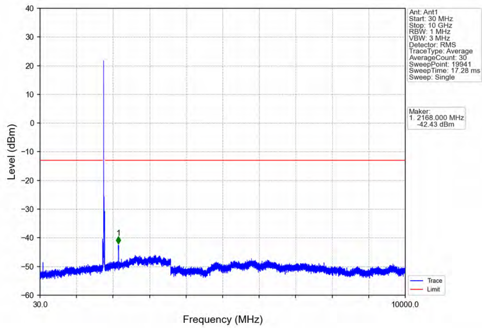
Band66_15MHz_QPSK_HCH_1772.5MHz_RB_1_0_NTNV
