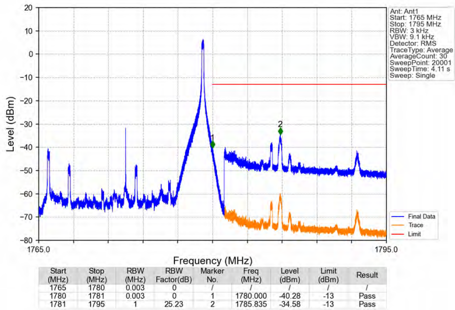
Band66_15MHz_16QAM_HCH_1772.5MHz_RB_1_74_NTNV
