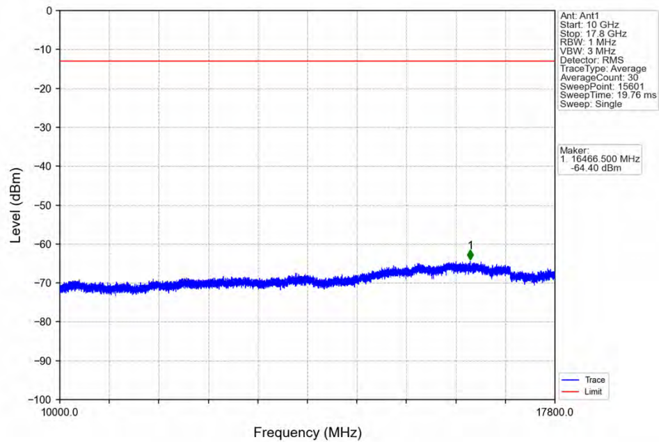
Band66_5MHz_16QAM_MCH_1745MHz_RB_1_0_NTNV
