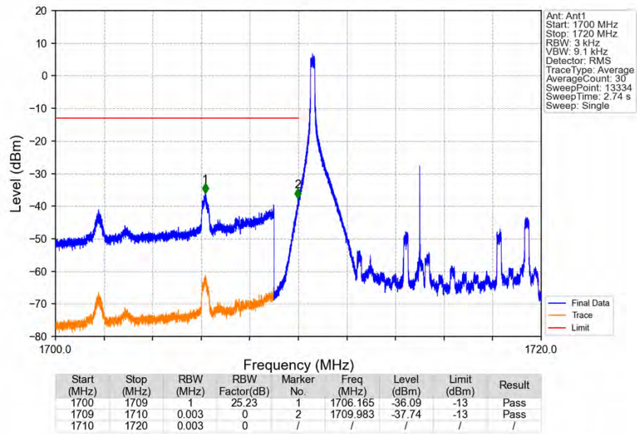
Band66_10MHz_16QAM_LCH_1715MHz_RB_1_0_NTNV
