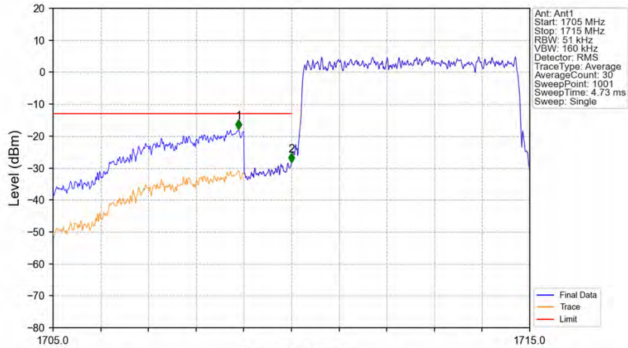
Band66_5MHz_QPSK_LCH_1712.5MHz_RB_25_0_NTNV
