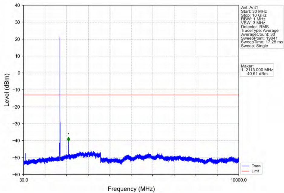
Band66_10MHz_16QAM_LCH_1715MHz_RB_1_0_NTNV
