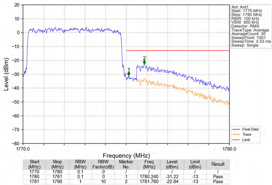
Band66_10MHz_16QAM_HCH_1775MHz_RB_50_0_NTNV
