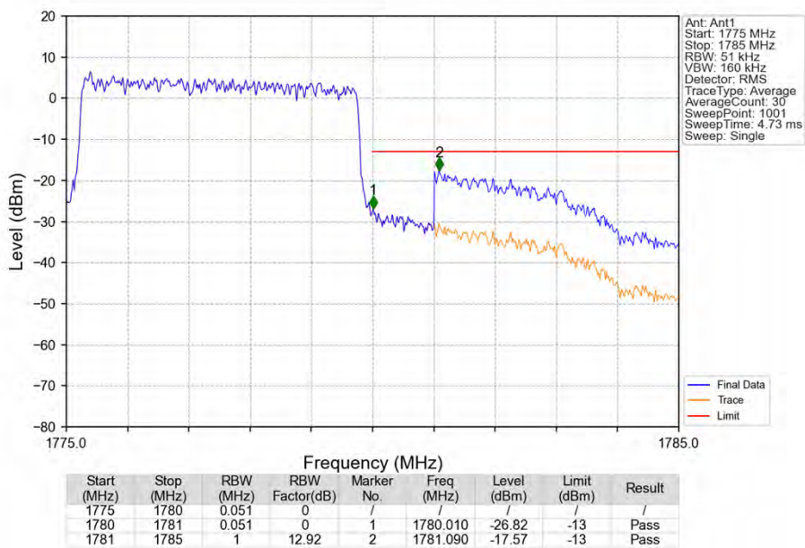
Band66_5MHz_QPSK_HCH_1777.5MHz_RB_25_0_NTNV
