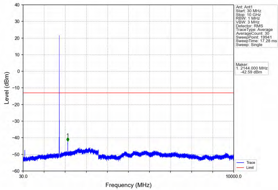
Band66_5MHz_16QAM_MCH_1745MHz_RB_1_0_NTNV
