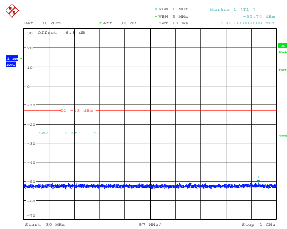
Band25-1.4MHz-16QAM-26683-1RB#0-Range3:30~1000MHz
