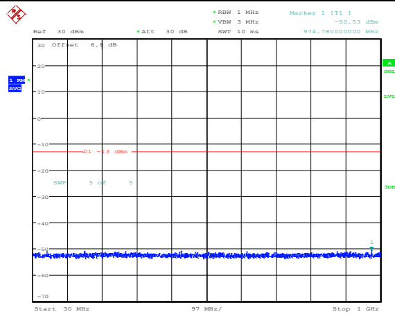
Band25-20MHz-QPSK-26140-1RB#0-Range3:30~1000MHz
