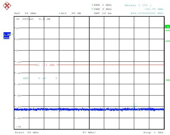
Band25-5MHz-16QAM-26665-1RB#0-Range3:30~1000MHz
