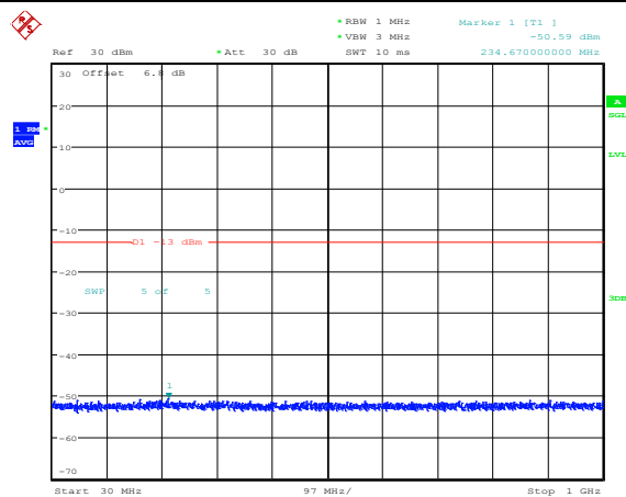
Band25-1.4MHz-16QAM-26047-1RB#0-Range3:30~1000MHz
