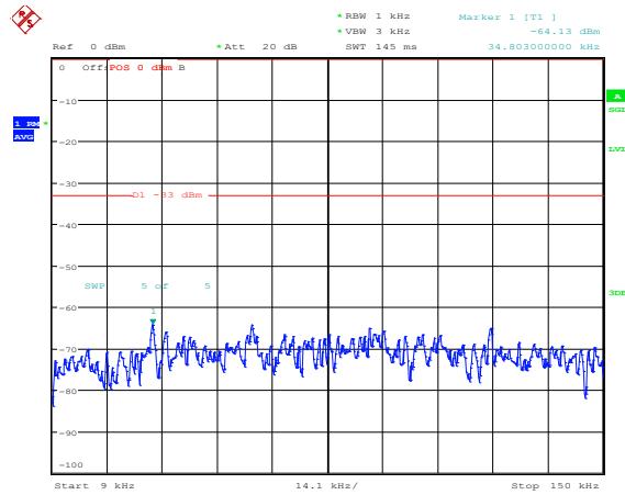
Band25-10MHz-QPSK-26365-1RB#0-Range1:0.009~0.15MHz
