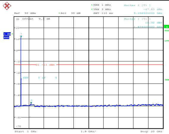
Band25-5MHz-16QAM-26365-1RB#0-Range4:1000~20000MHz
