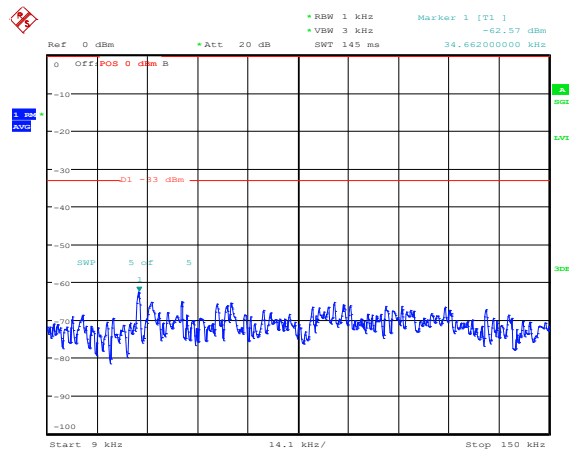
Band25-10MHz-QPSK-26640-1RB#0-Range1:0.009~0.15MHz
