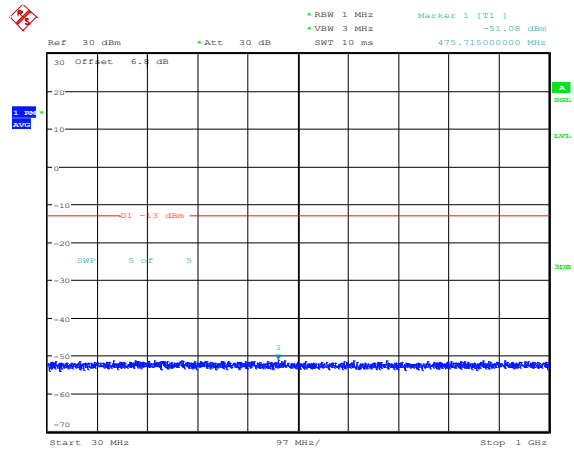
Band25-10MHz-QPSK-26090-1RB#0-Range3:30~1000MHz
