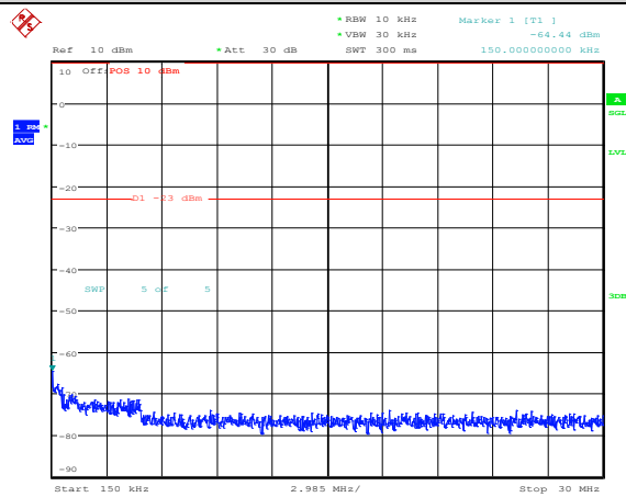
Band25-1.4MHz-16QAM-26047-1RB#0-Range2:0.15~30MHz
