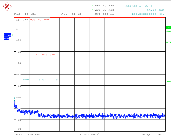
Band25-5MHz-16QAM-26365-1RB#0-Range2:0.15~30MHz
