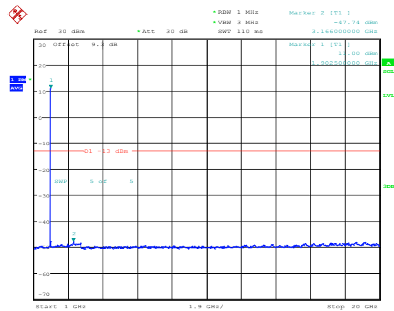
Band25-10MHz-QPSK-26640-1RB#0-Range4:1000~20000MHz
