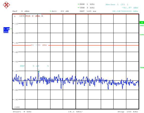
Band25-10MHz-16QAM-26640-1RB#0-Range1:0.009~0.15MHz
