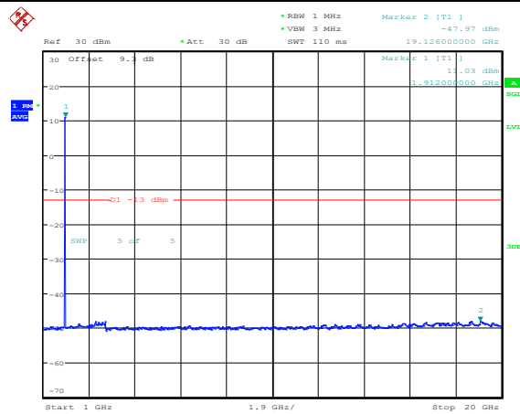
Band25-3MHz-16QAM-26675-1RB#0-Range4:1000~20000MHz
