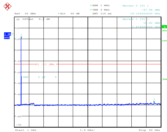
Band25-10MHz-16QAM-26365-1RB#0-Range4:1000~20000MHz
