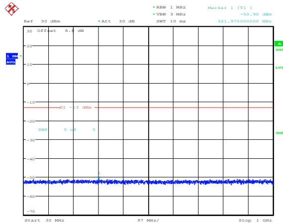
Band25-15MHz-16QAM-26115-1RB#0-Range3:30~1000MHz
