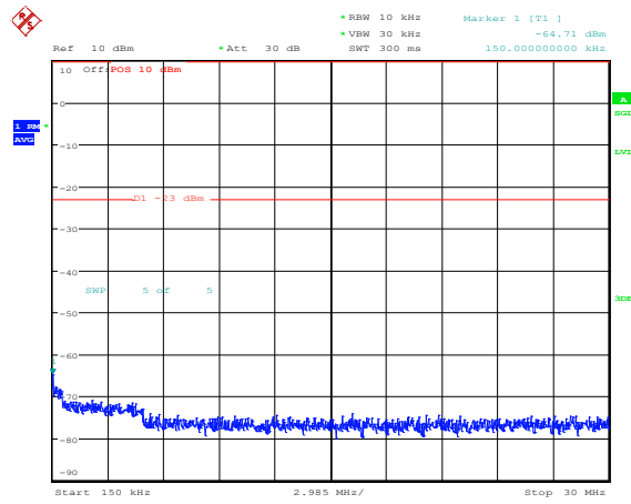
Band25-15MHz-16QAM-26115-1RB#0-Range2:0.15~30MHz
