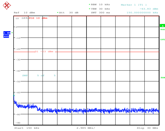
Band25-5MHz-16QAM-26065-1RB#0-Range2:0.15~30MHz
