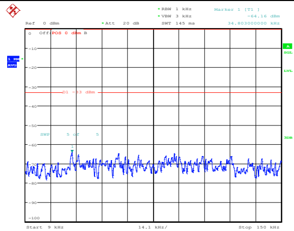
Band25-15MHz-QPSK-26615-1RB#0-Range1:0.009~0.15MHz
