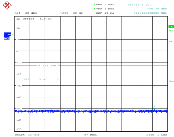
Band25-5MHz-16QAM-26065-1RB#0-Range3:30~1000MHz
