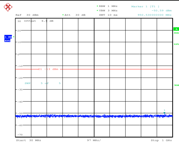
Band25-3MHz-QPSK-26055-1RB#0-Range3:30~1000MHz
