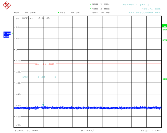
Band25-15MHz-QPSK-26615-1RB#0-Range3:30~1000MHz
