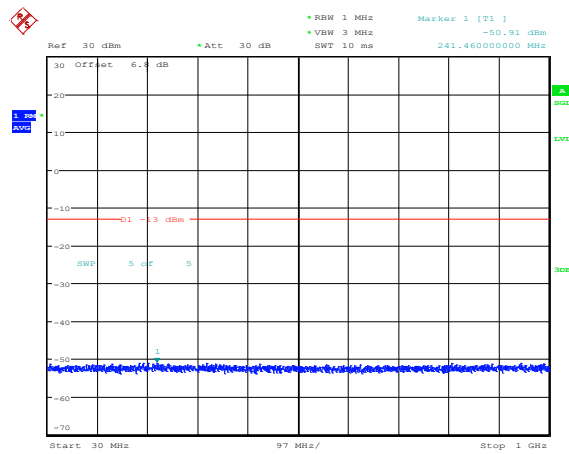
Band25-10MHz-16QAM-26640-1RB#0-Range3:30~1000MHz
