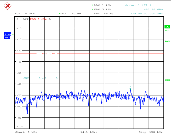
Band25-20MHz-QPSK-26590-1RB#0-Range1:0.009~0.15MHz
