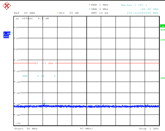
Band25-3MHz-16QAM-26675-1RB#0-Range3:30~1000MHz
