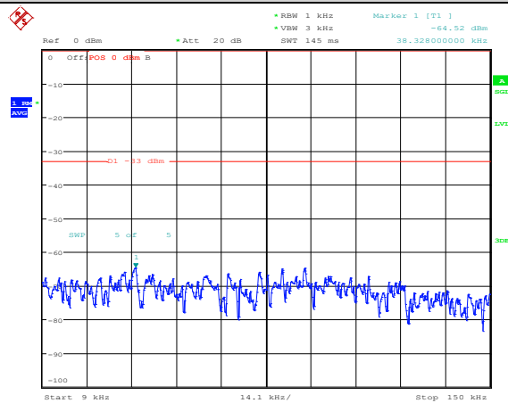
Band25-5MHz-16QAM-26665-1RB#0-Range1:0.009~0.15MHz
