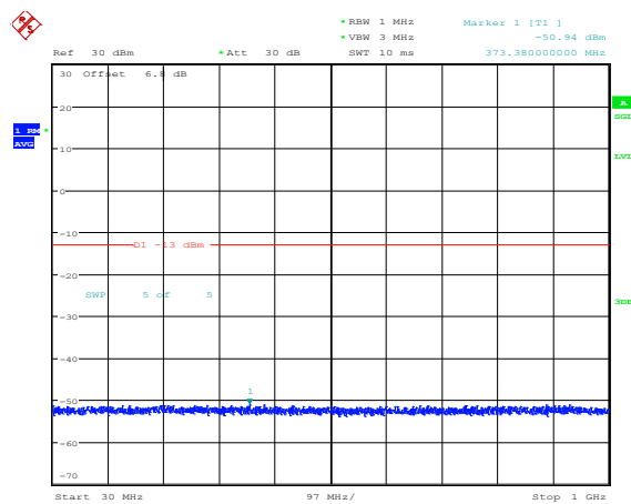
Band25-1.4MHz-QPSK-26683-1RB#0-Range3:30~1000MHz
