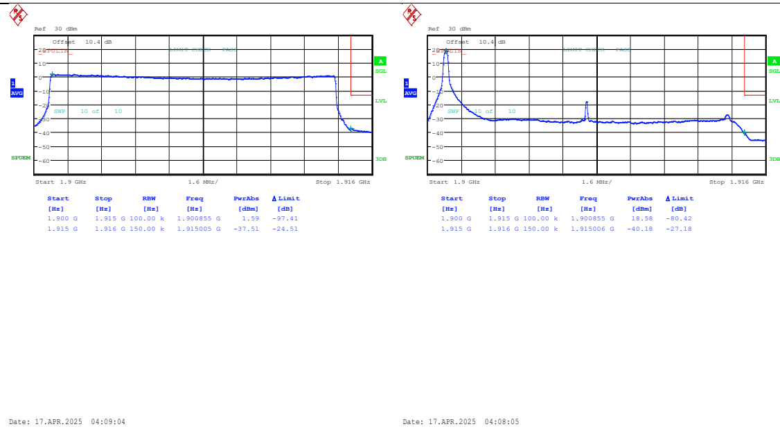
Band25-15MHz-QPSK-26615-75RB#0-PASS
