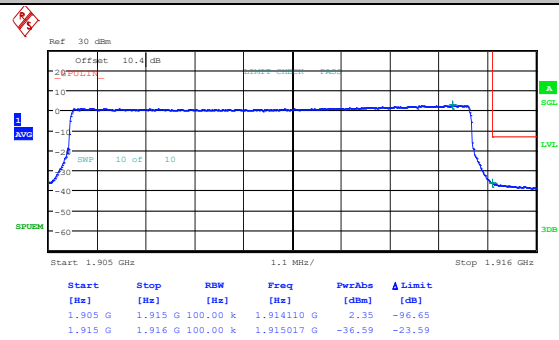
Band25-10MHz-16QAM-26640-1RB#0-PASS
