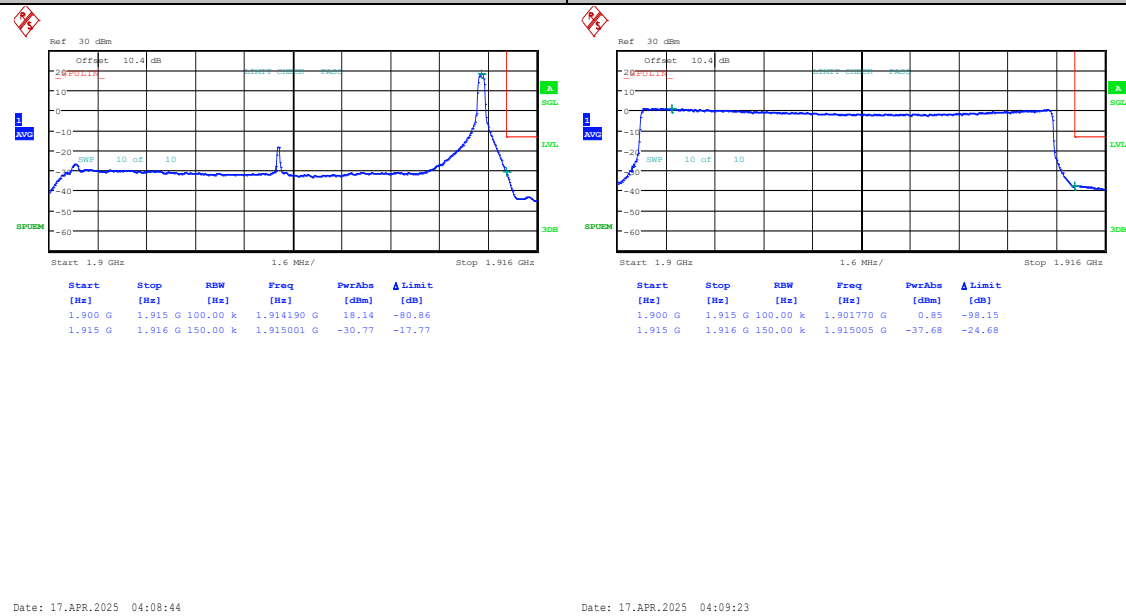
Band25-15MHz-16QAM-26615-1RB#74-PASS
