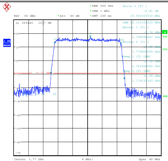
Band66-20MHz-16QAM-132322-100RB#0-PASS
