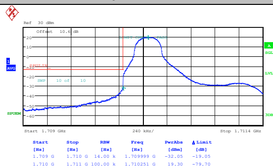
Band66-1.4MHz-QPSK-131979-1RB#5-PASS
