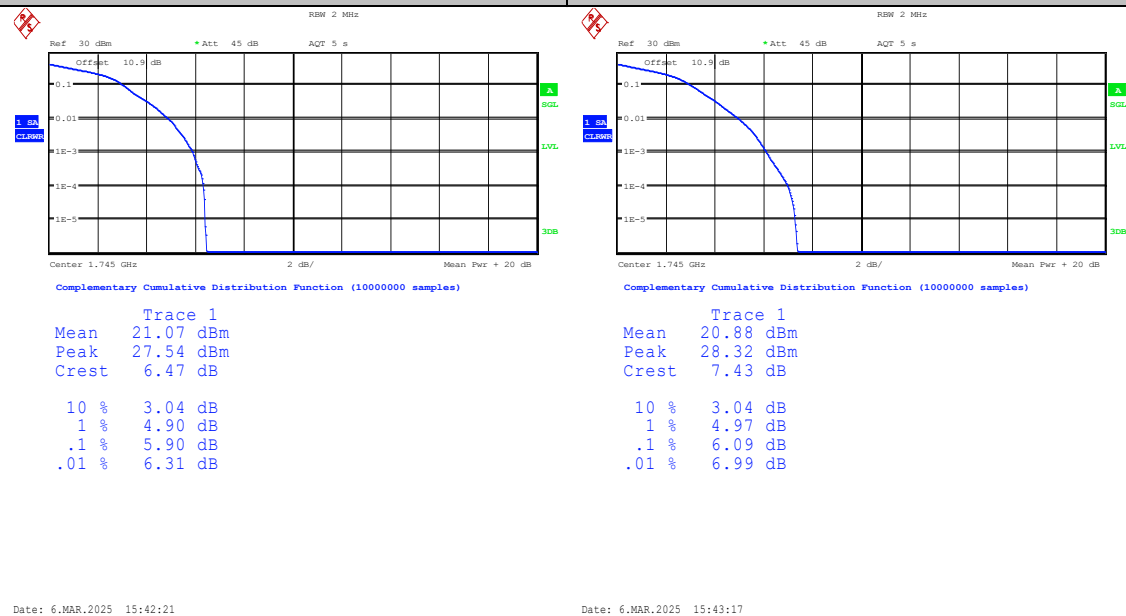
Band66-1.4MHz-16QAM-132322-1RB#0-PASS
