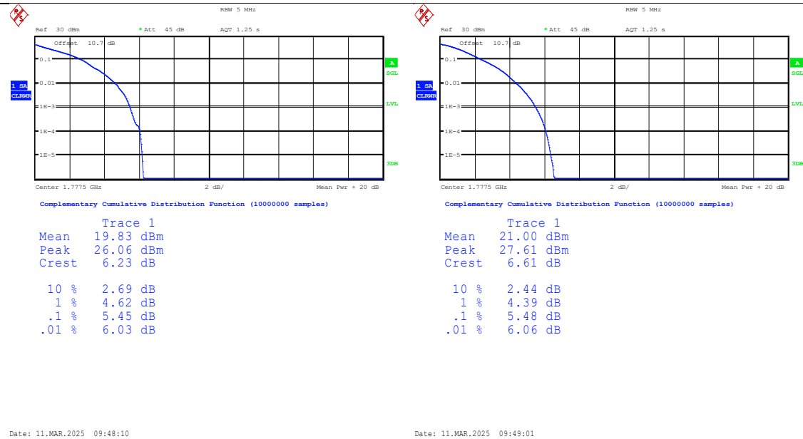
Band66-5MHz-QPSK-132647-1RB#0-PASS
