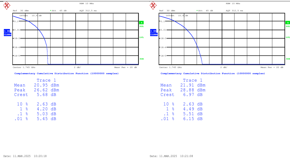
Band66-10MHz-QPSK-132322-1RB#0-PASS
