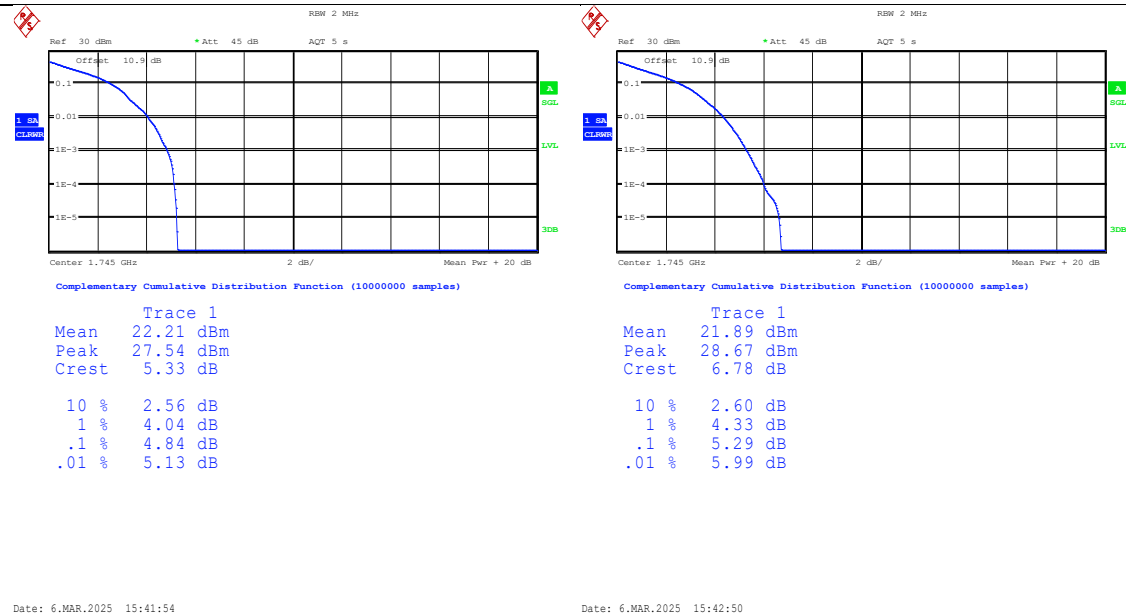
Band66-1.4MHz-QPSK-132322-1RB#0-PASS
