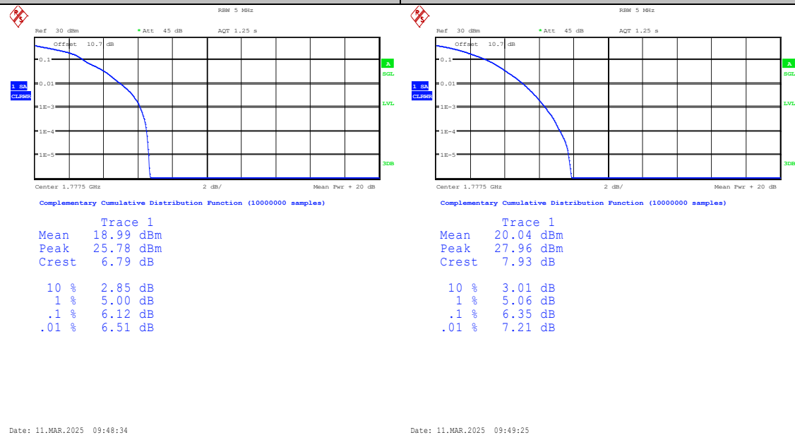
Band66-5MHz-16QAM-132647-1RB#0-PASS
