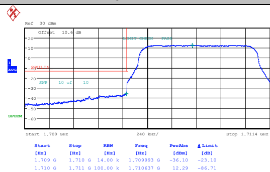
Band66-1.4MHz-QPSK-131979-1RB#0-PASS
