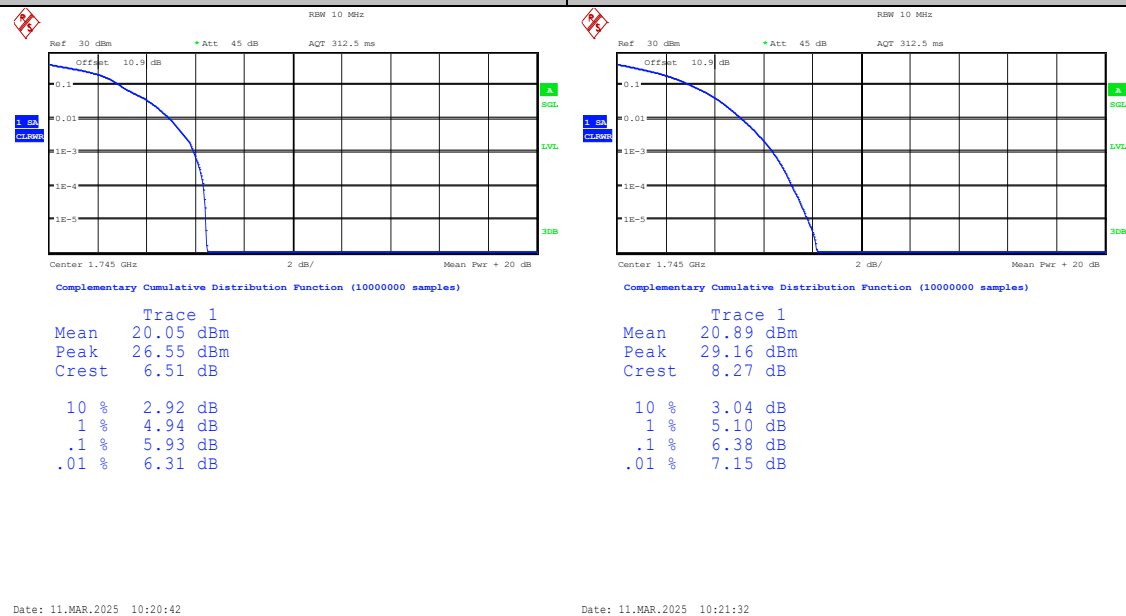
Band66-10MHz-16QAM-132322-1RB#0-PASS
