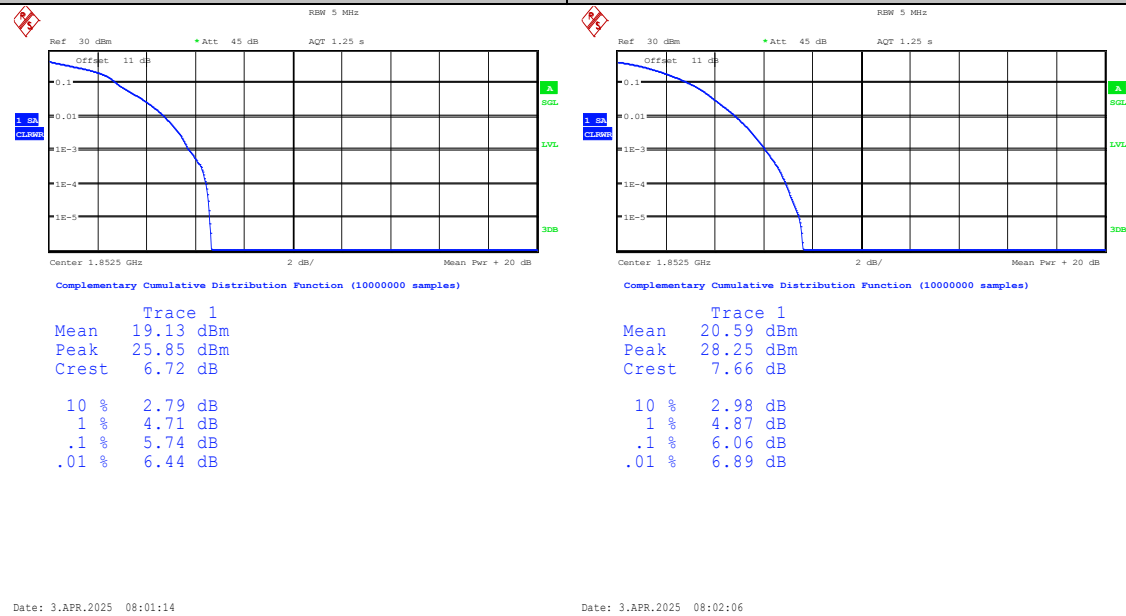
Band25-5MHz-16QAM-26065-1RB#0-PASS
