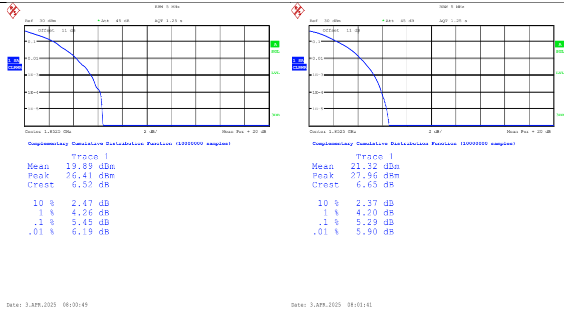
Band25-5MHz-QPSK-26065-1RB#0-PASS
