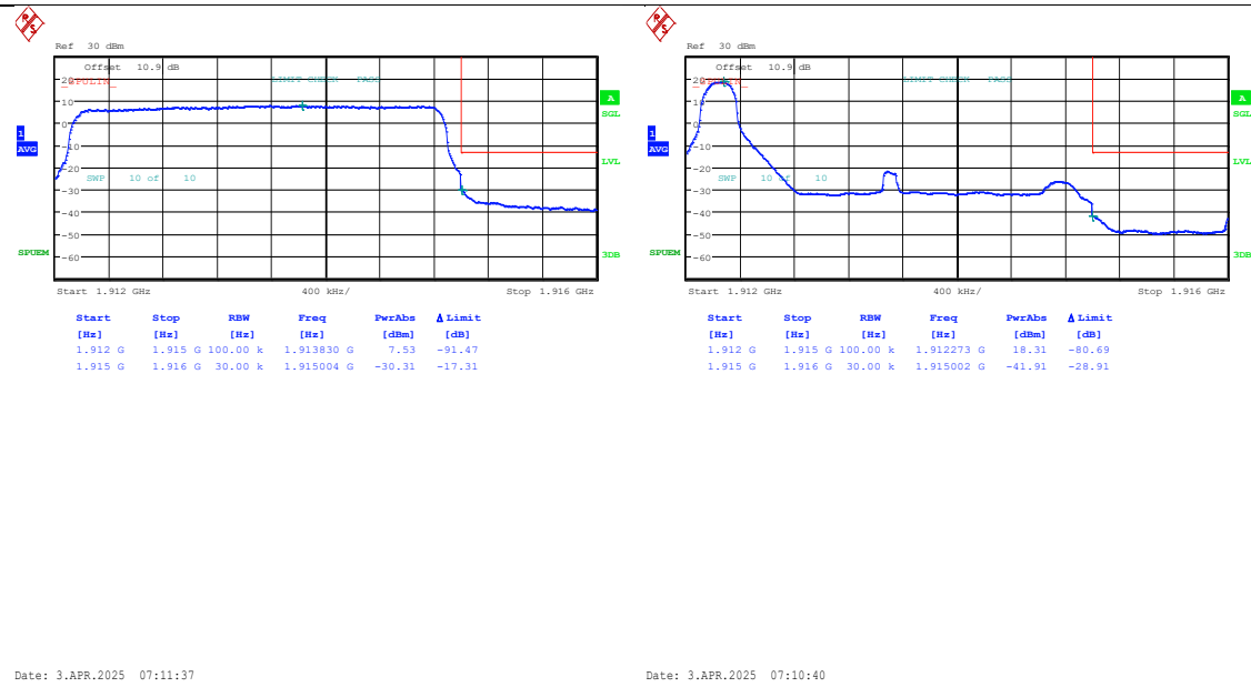
Band25-3MHz-QPSK-26675-15RB#0-PASS
