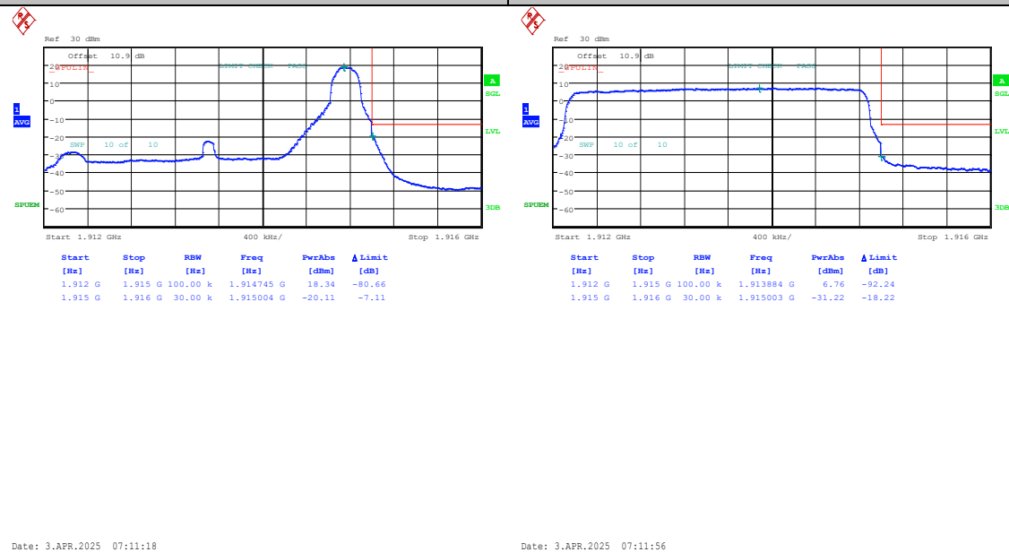
Band25-3MHz-16QAM-26675-1RB#14-PASS
