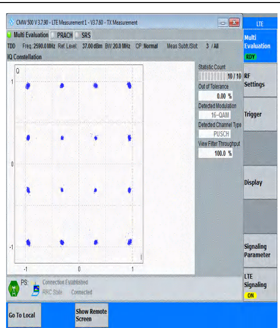
Band41(2535-2655)-20MHz-16QAM-40590-100RB #0-PASS
