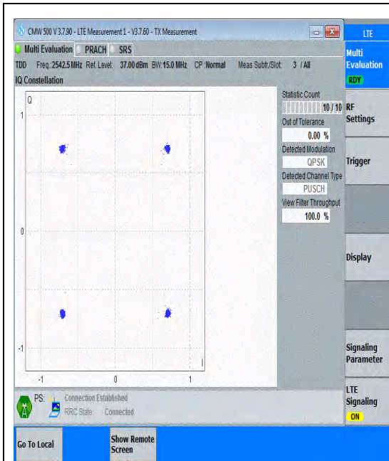
Band41(2535-2655)-15MHz-QPSK-40115-75RB# 0-PASS
