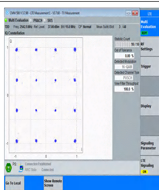
Band41(2535-2655)-15MHz-16QAM-40115-75RB# 0-PASS
