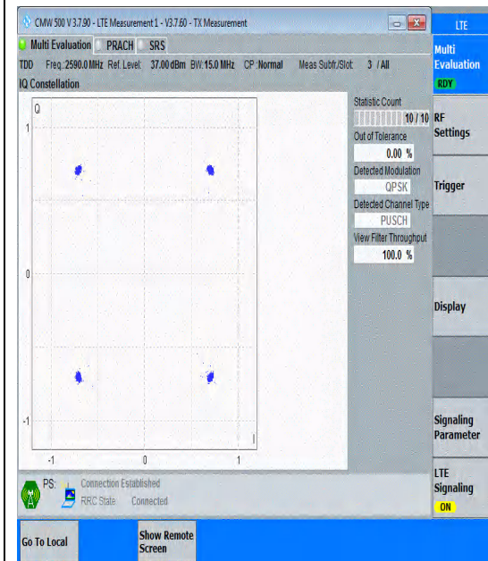
Band41(2535-2655)-15MHz-QPSK-40590-75RB# 0-PASS
