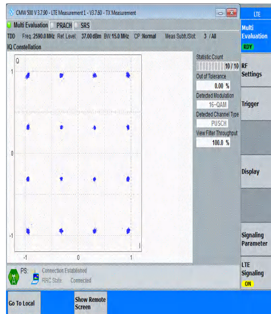
Band41(2535-2655)-15MHz-16QAM-40590-75RB# 0-PASS
