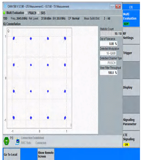
Band41(2535-2655)-20MHz-16QAM-41140-100RB #0-PASS
