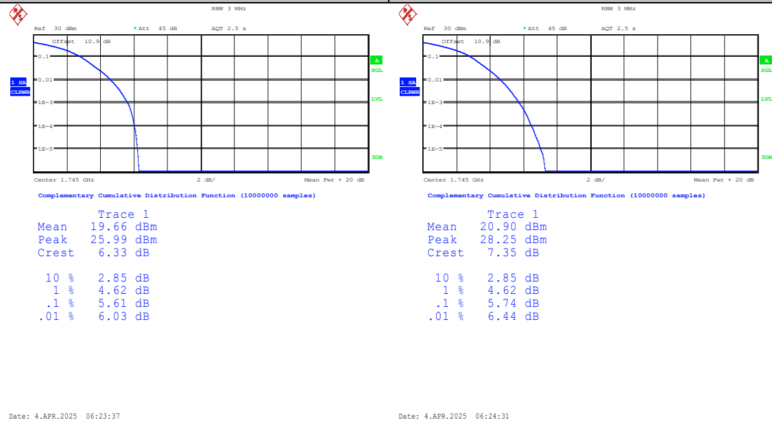
Band66-3MHz-16QAM-132322-1RB#0-PASS
