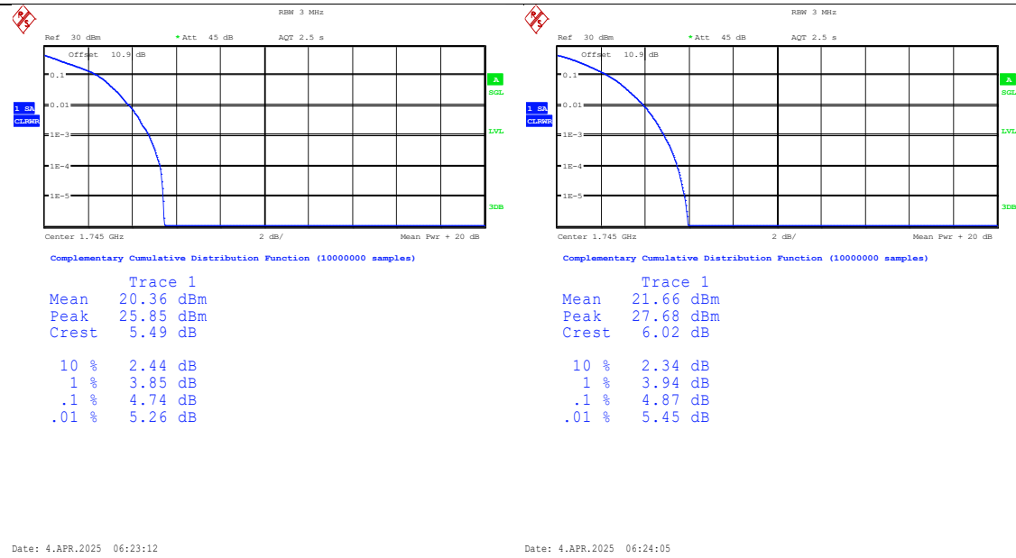
Band66-3MHz-QPSK-132322-1RB#0-PASS
