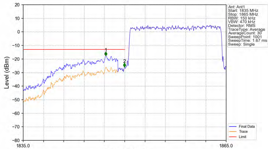
Band2_15MHz_QPSK_LCH_1857.5MHz_RB_75_0_NTNV
