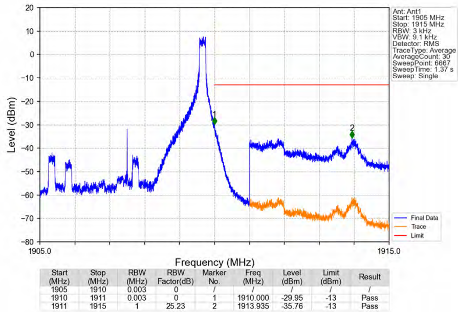
Band2_5MHz_16QAM_HCH_1907.5MHz_RB_1_24_NTNV
