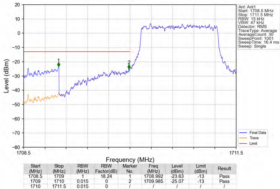
Band4_1.4MHz_QPSK_LCH_1710.7MHz_RB_6_0_NTNV
