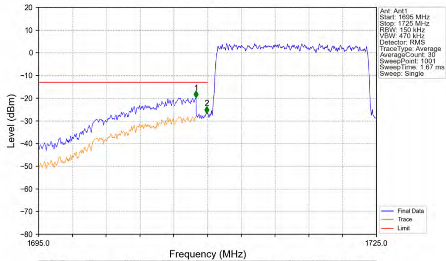
Band4_15MHz_16QAM_LCH_1717.5MHz_RB_75_0_NTNV
