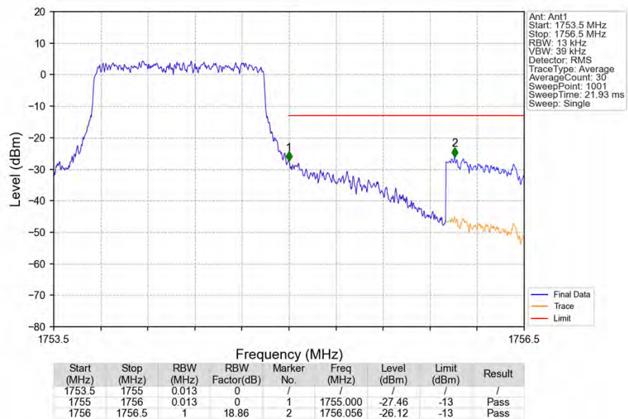
Band4_1.4MHz_16QAM_HCH_1754.3MHz_RB_6_0_NTNV
