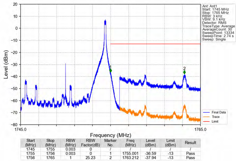
Band4_10MHz_16QAM_HCH_1750MHz_RB_1_49_NTNV
