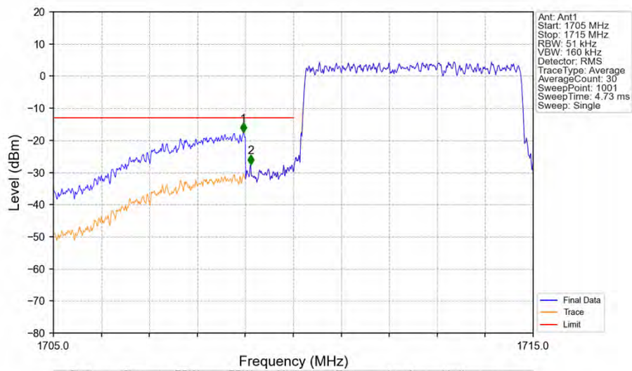
Band4_5MHz_16QAM_LCH_1712.5MHz_RB_25_0_NTNV
