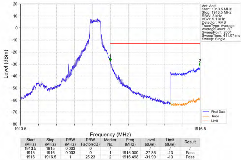
Band25_1.4MHz_QPSK_HCH_1914.3MHz_RB_1_5_NTNV
