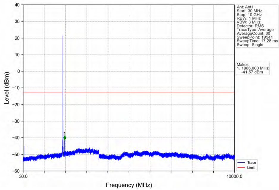
Band25_15MHz_16QAM_HCH_1907.5MHz_RB_1_0_NTNV
