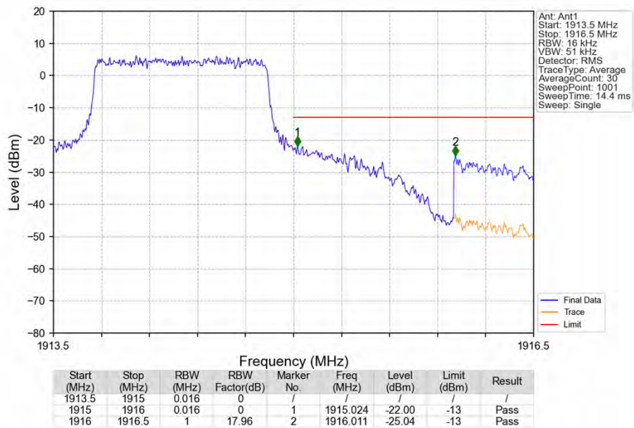
Band25_1.4MHz_16QAM_HCH_1914.3MHz_RB_6_0_NTNV
