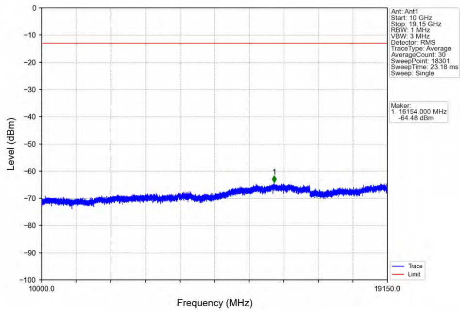
Band25_1.4MHz_16QAM_LCH_1850.7MHz_RB_6_0_NTNV
