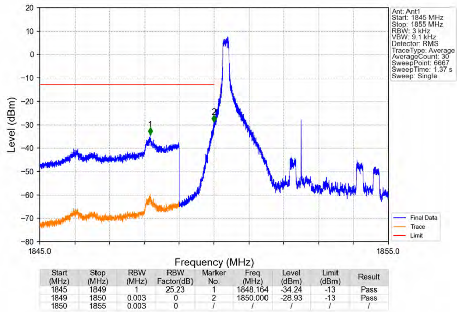
Band25_5MHz_16QAM_LCH_1852.5MHz_RB_1_0_NTNV
