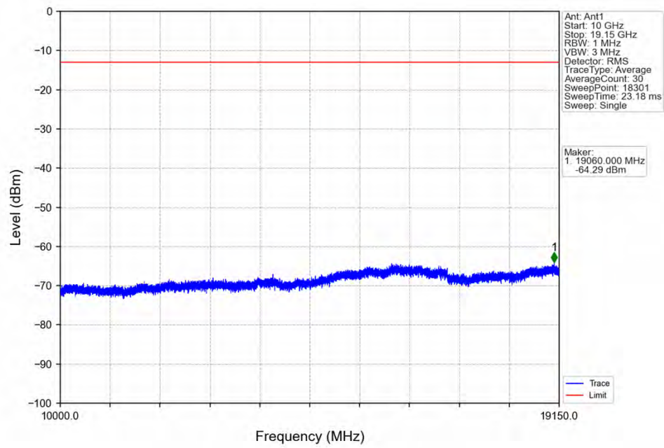
Band25_1.4MHz_QPSK_LCH_1850.7MHz_RB_6_0_NTNV
