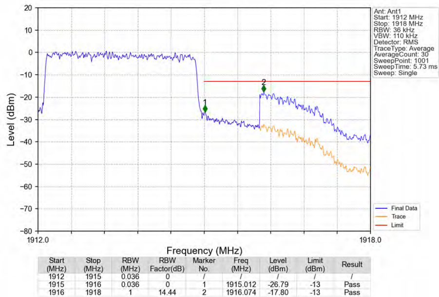
Band25_3MHz_16QAM_HCH_1913.5MHz_RB_15_0_NTNV
