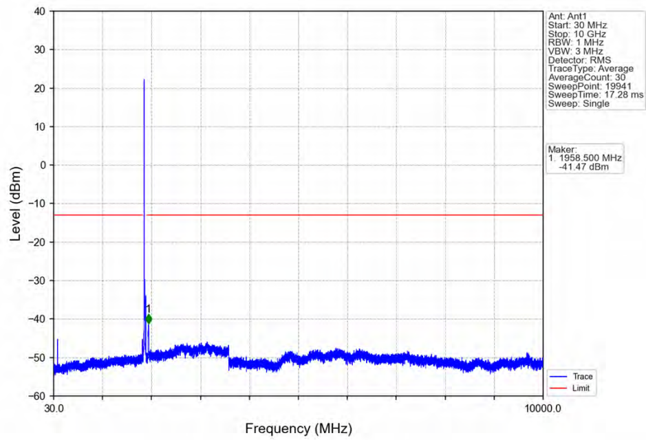
Band25_20MHz_16QAM_MCH_1882.5MHz_RB_1_0_NTNV
