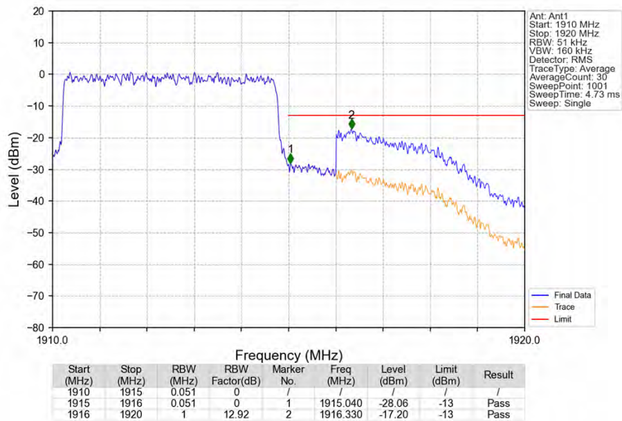
Band25_5MHz_QPSK_HCH_1912.5MHz_RB_25_0_NTNV
