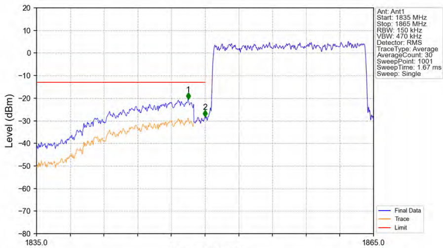
Band25_15MHz_16QAM_LCH_1857.5MHz_RB_75_0_NTNV
