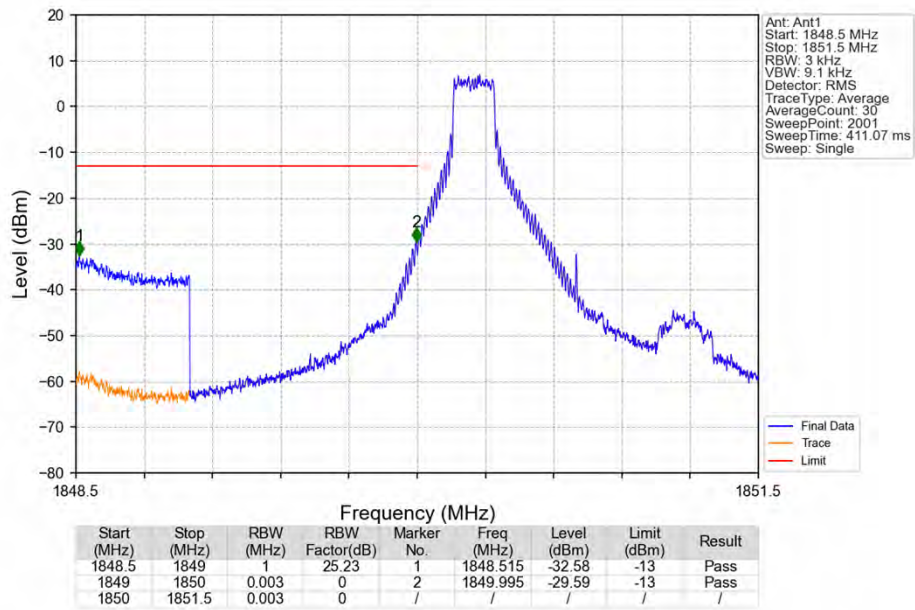
Band25_1.4MHz_16QAM_LCH_1850.7MHz_RB_1_0_NTNV
