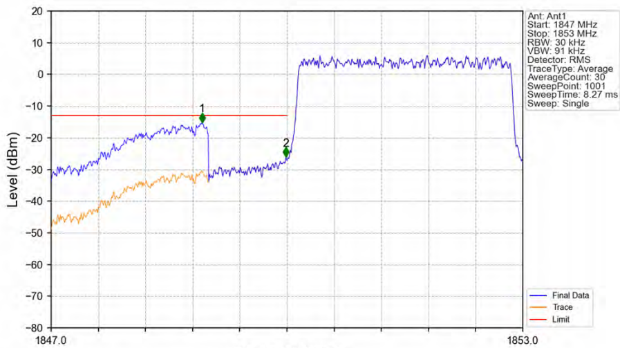
Band25_3MHz_QPSK_LCH_1851.5MHz_RB_15_0_NTNV
