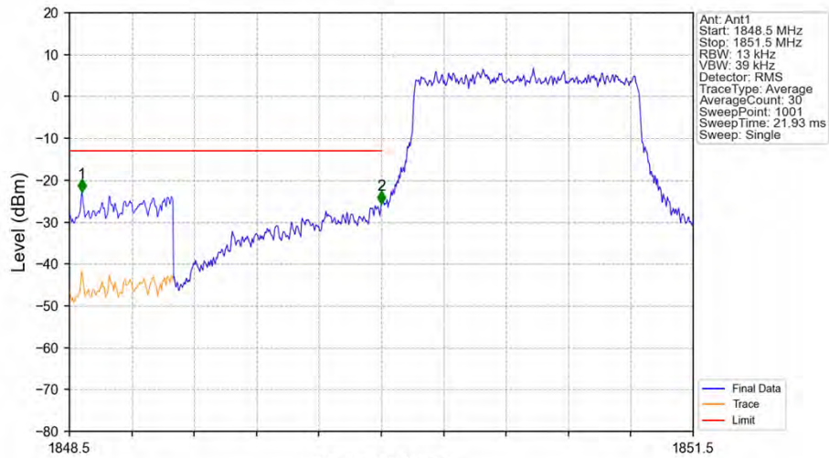
Band25_1.4MHz_QPSK_LCH_1850.7MHz_RB_6_0_NTNV
