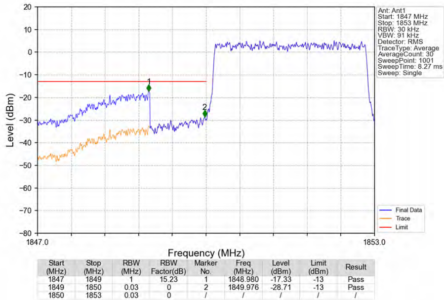
Band25_3MHz_16QAM_LCH_1851.5MHz_RB_15_0_NTNV
