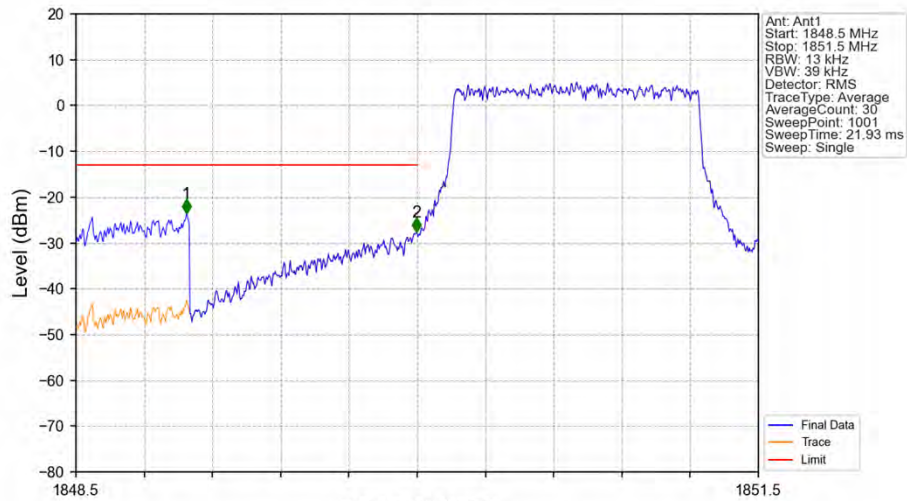
Band25_1.4MHz_16QAM_LCH_1850.7MHz_RB_6_0_NTNV
