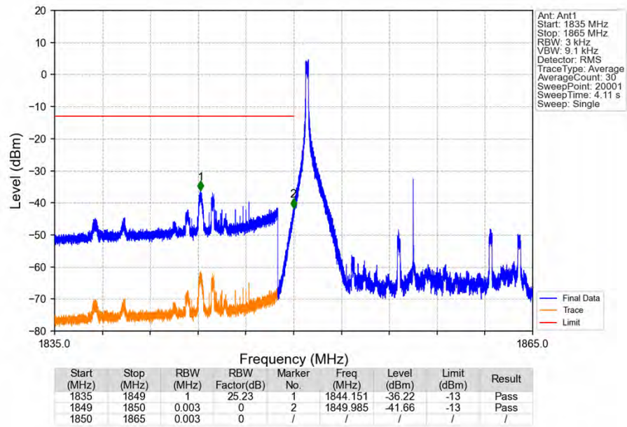
Band25_15MHz_16QAM_LCH_1857.5MHz_RB_1_0_NTNV
