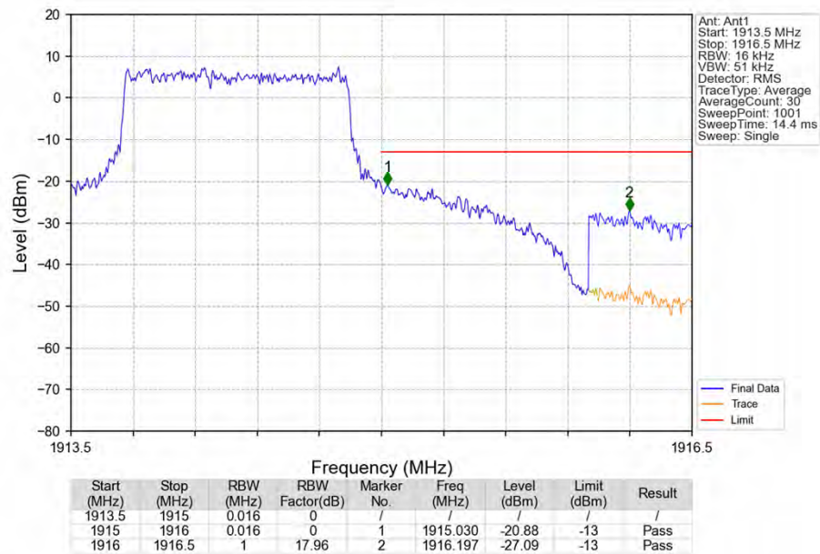
Band25_1.4MHz_QPSK_HCH_1914.3MHz_RB_6_0_NTNV
