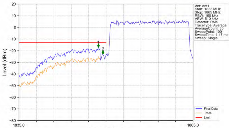
Band25_15MHz_QPSK_LCH_1857.5MHz_RB_75_0_NTNV
