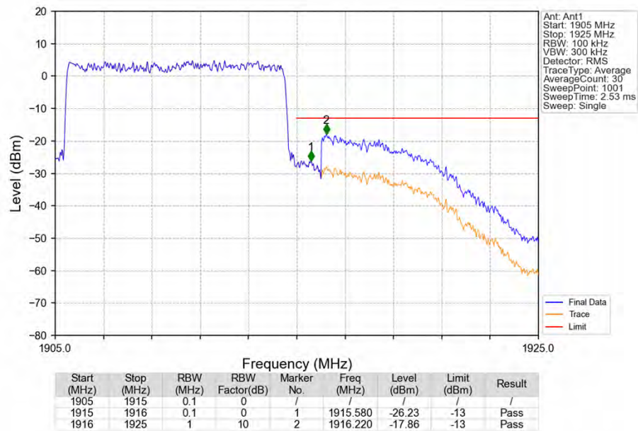
Band25_10MHz_16QAM_HCH_1910MHz_RB_50_0_NTNV
