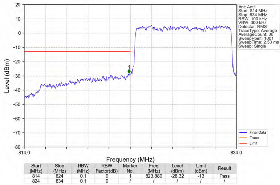
Band26b_10MHz_QPSK_LCH_829MHz_RB_50_0_NTNV
