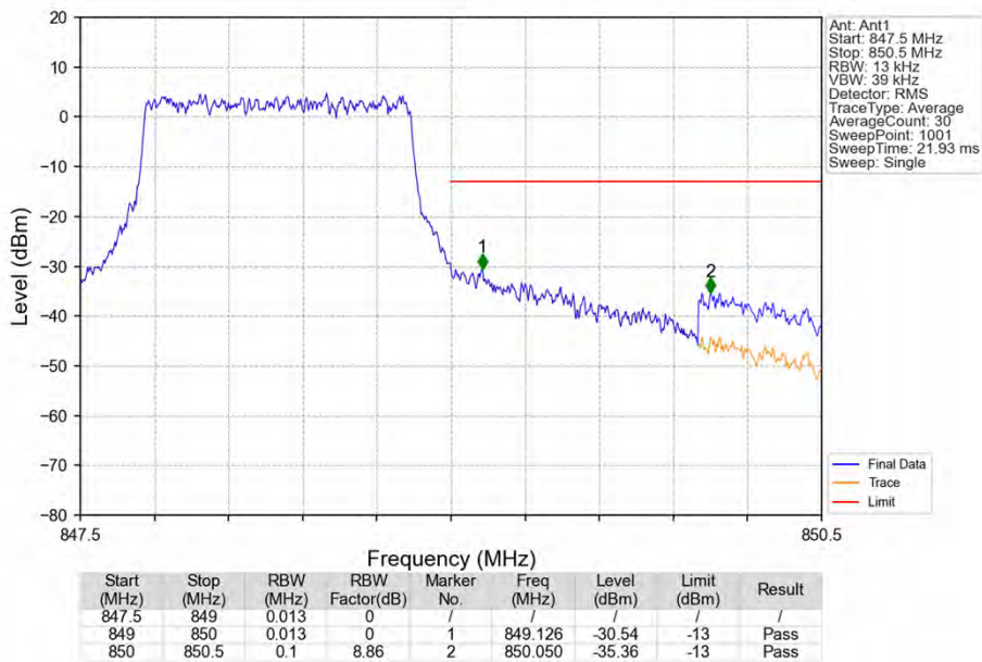
Band26b_1.4MHz_16QAM_HCH_848.3MHz_RB_6_0_NTNV
