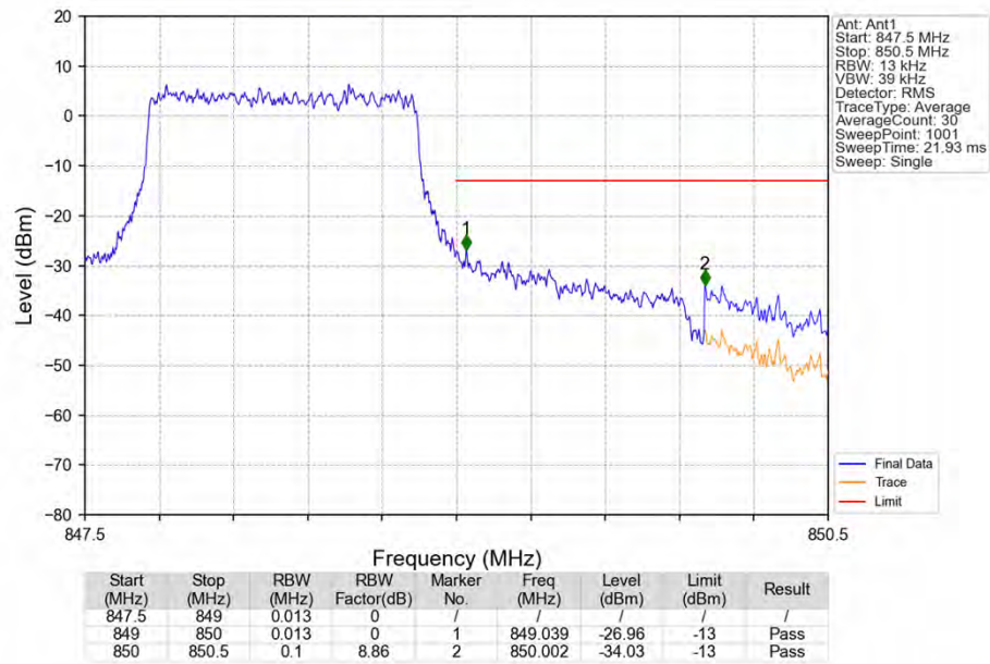
Band26b_1.4MHz_QPSK_HCH_848.3MHz_RB_6_0_NTNV
