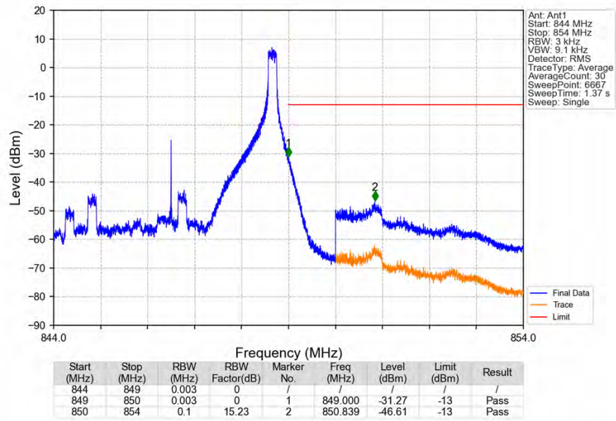
Band26b_5MHz_16QAM_HCH_846.5MHz_RB_1_24_NTNV
