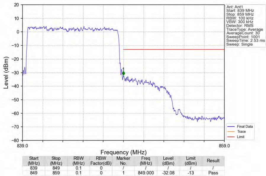
Band26b_10MHz_16QAM_HCH_844MHz_RB_50_0_NTNV
