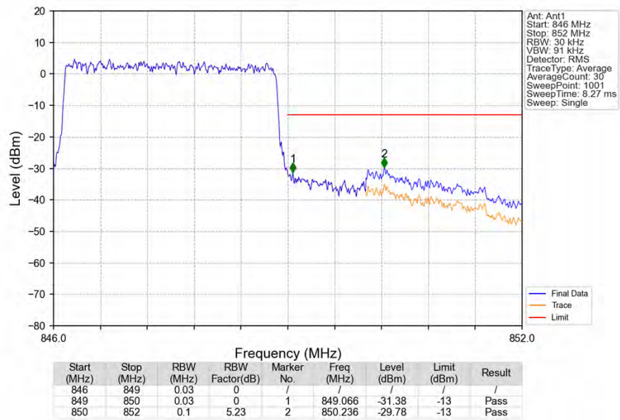
Band26b_3MHz_16QAM_HCH_847.5MHz_RB_15_0_NTNV
