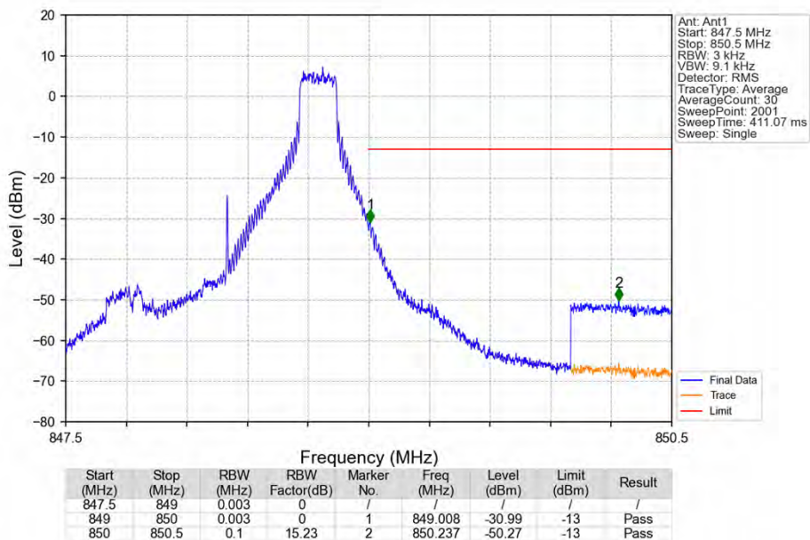
Band26b_1.4MHz_16QAM_HCH_848.3MHz_RB_1_5_NTNV
