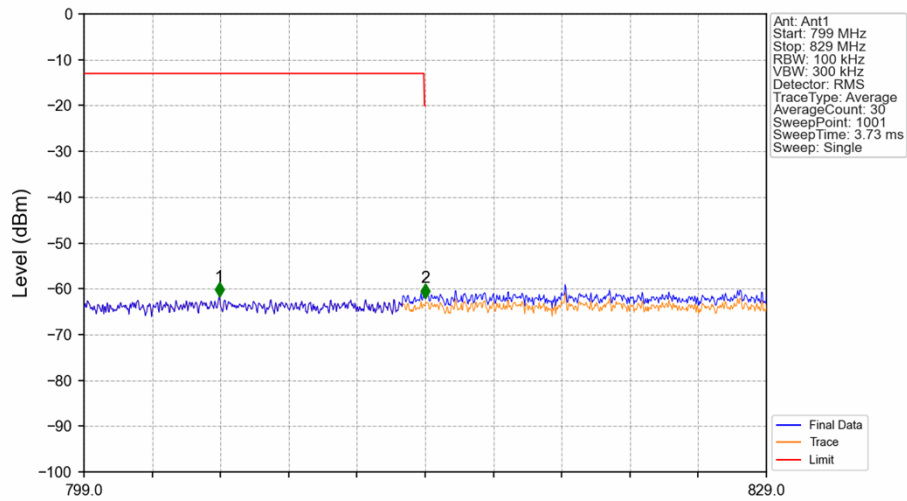
Band26c_15MHz_16QAM_LCH_821.5MHz_RB_75_0_NTNV
