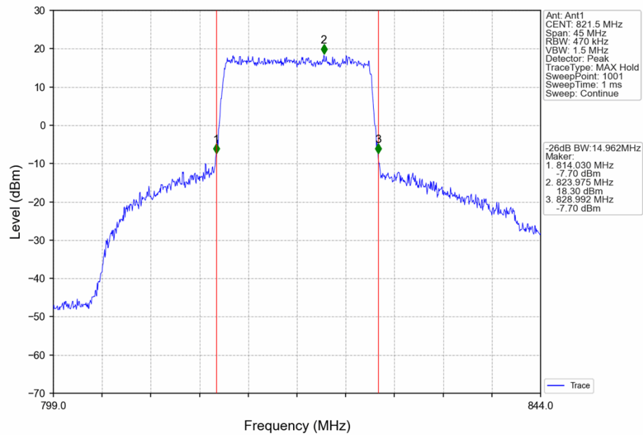
Band26c_15MHz_16QAM_LCH_821.5MHz_RB_75_0_NTNV
