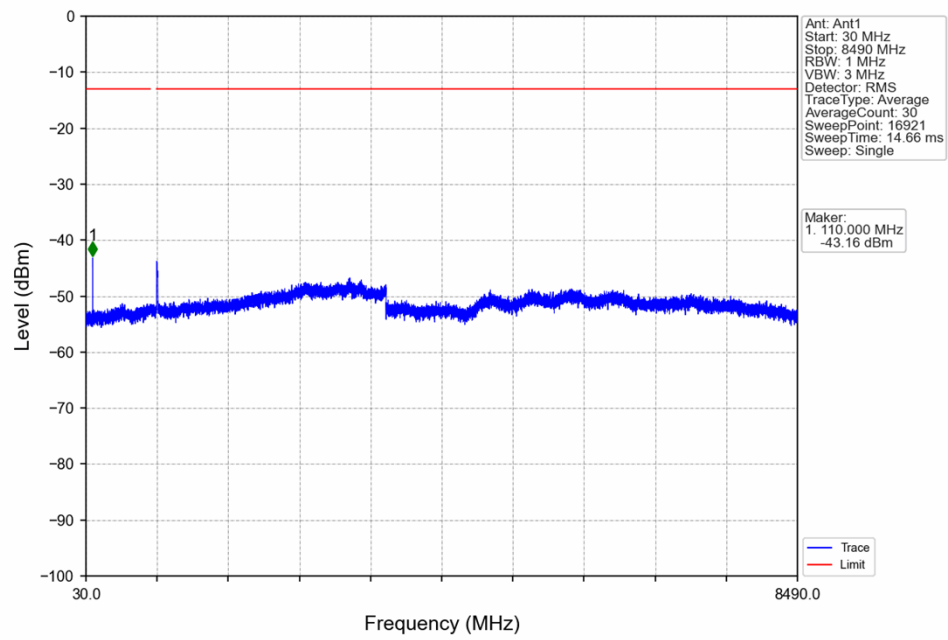
Band26c_15MHz_16QAM_HCH_841.5MHz_RB_1_0_NTNV
