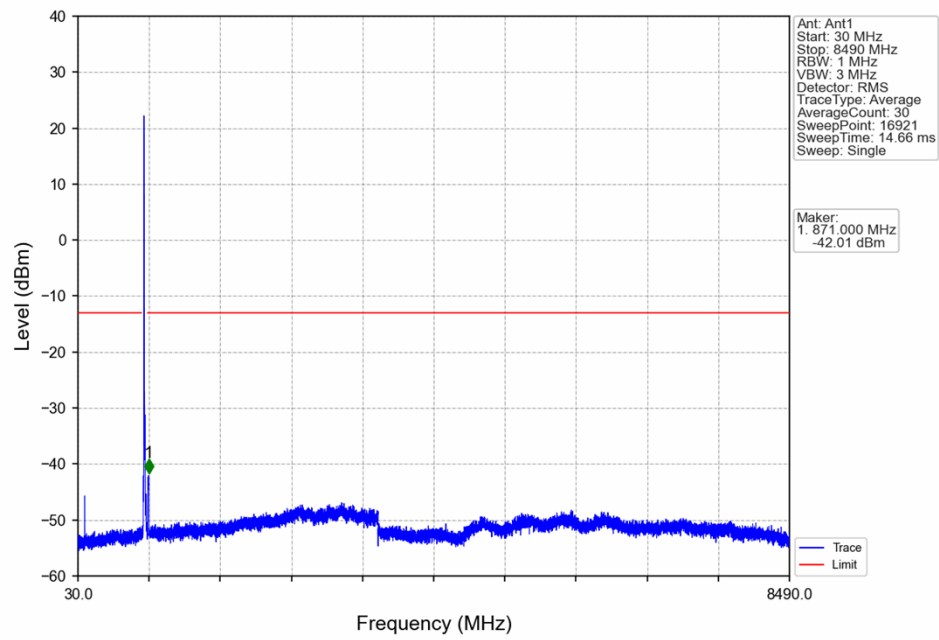
Band26c_15MHz_16QAM_LCH_821.5MHz_RB_75_0_NTNV
