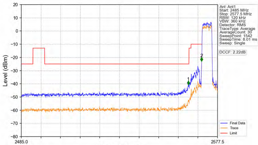
Band38_5MHz_16QAM_LCH_2572.5MHz_RB_25_0_NTNV
