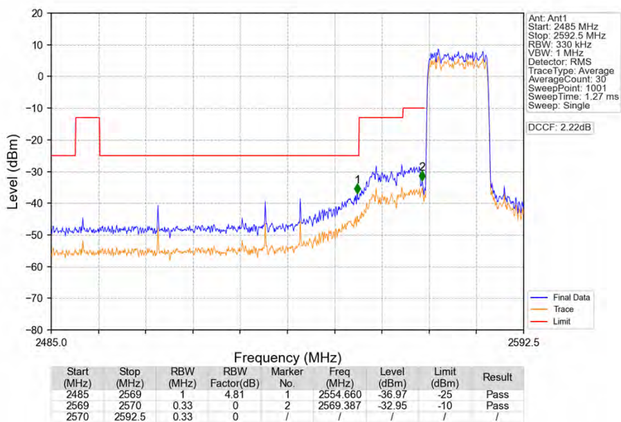
Band38_15MHz_QPSK_LCH_2577.5MHz_RB_75_0_NTNV
