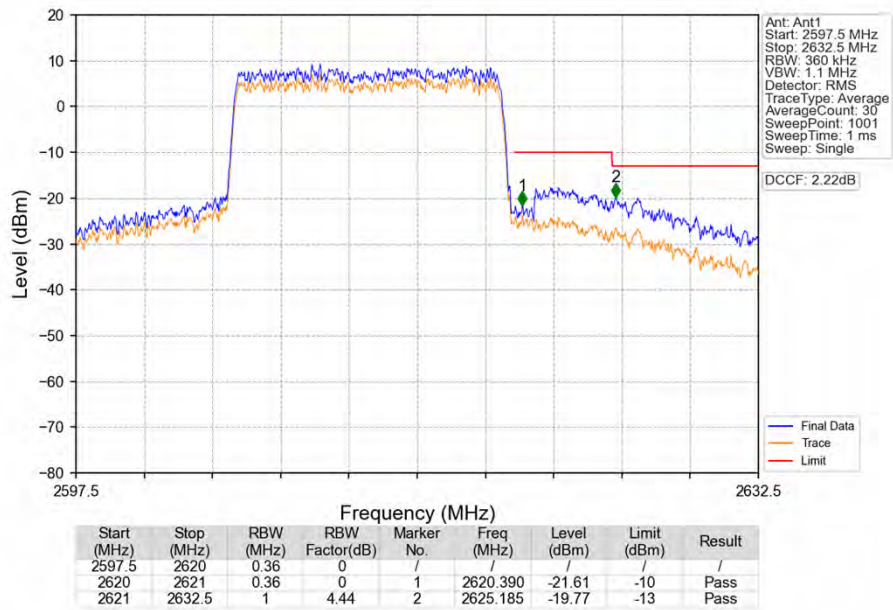
Band38_15MHz_QPSK_HCH_2612.5MHz_RB_75_0_NTNV
