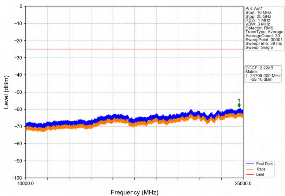
Band38_5MHz_16QAM_HCH_2617.5MHz_RB_1_0_NTNV
