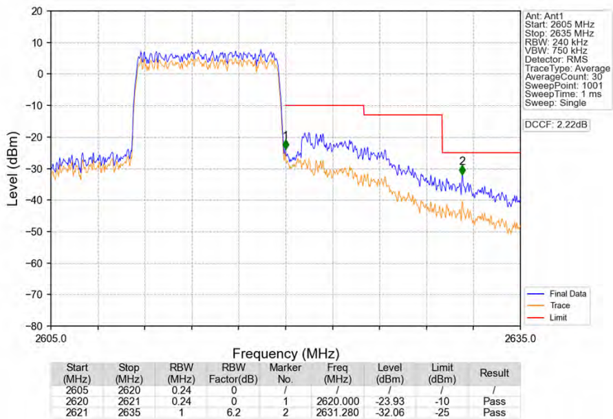
Band38_10MHz_16QAM_HCH_2615MHz_RB_50_0_NTNV
