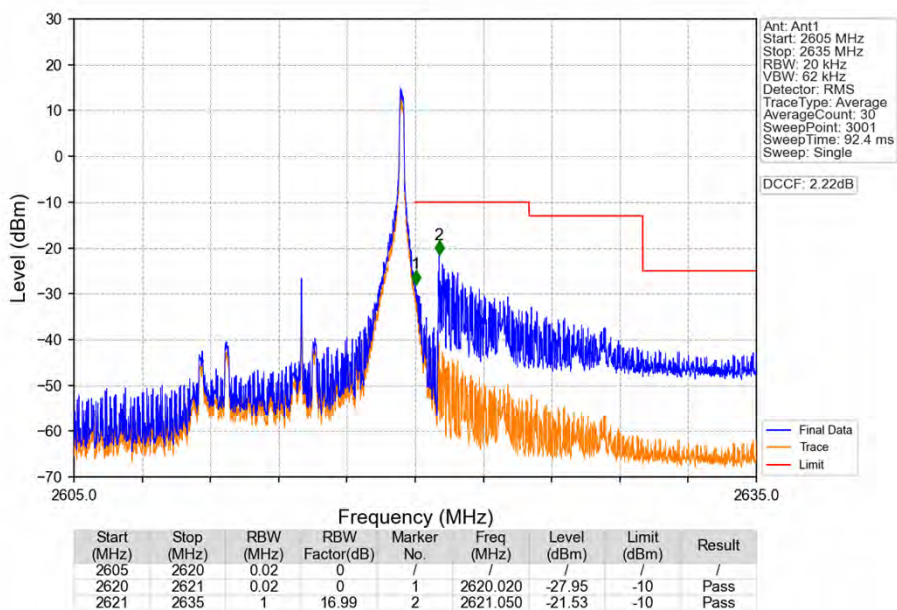
Band38_10MHz_16QAM_HCH_2615MHz_RB_1_49_NTNV
