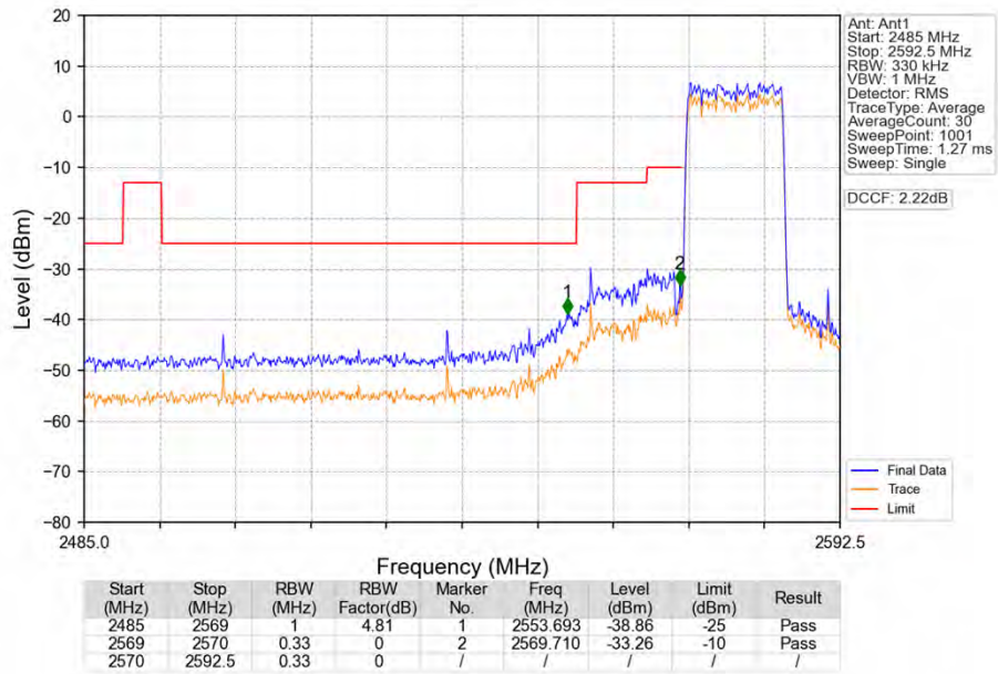
Band38_15MHz_16QAM_LCH_2577.5MHz_RB_75_0_NTNV
