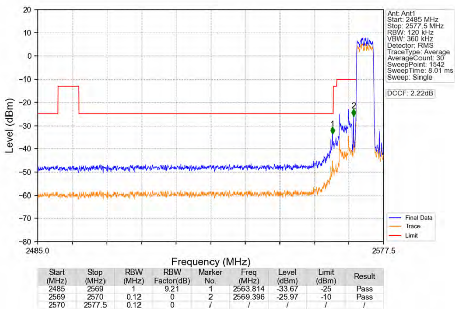
Band38_5MHz_QPSK_LCH_2572.5MHz_RB_25_0_NTNV
