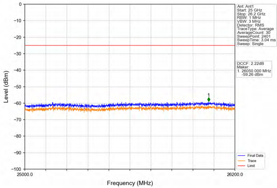
Band38_15MHz_QPSK_HCH_2612.5MHz_RB_1_74_NTNV
