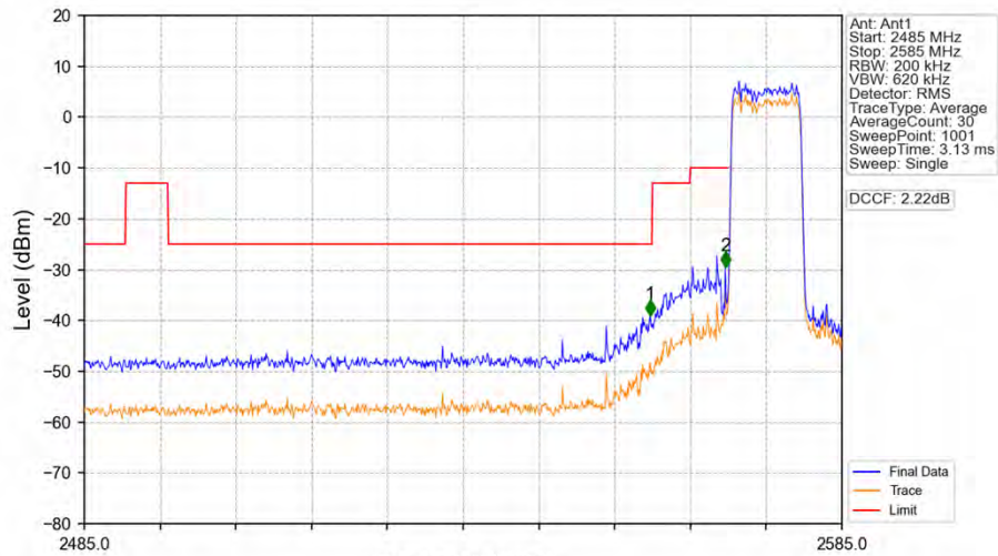
Band38_10MHz_16QAM_LCH_2575MHz_RB_50_0_NTNV
