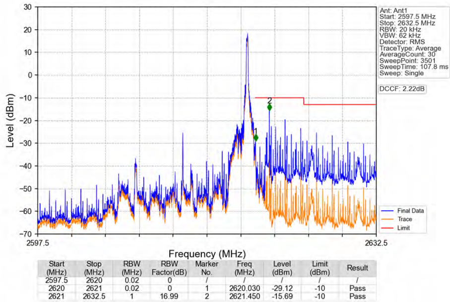
Band38_15MHz_QPSK_HCH_2612.5MHz_RB_1_74_NTNV
