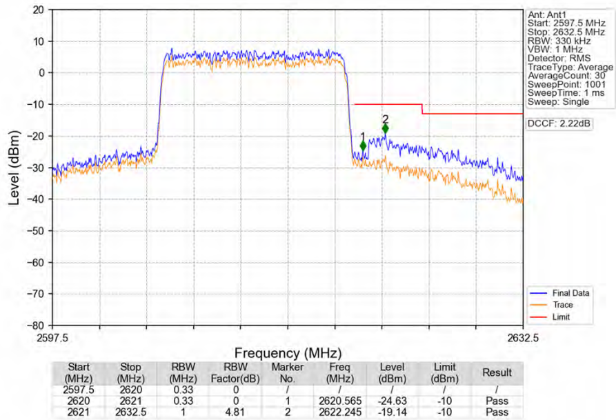
Band38_15MHz_16QAM_HCH_2612.5MHz_RB_75_0_NTNV
