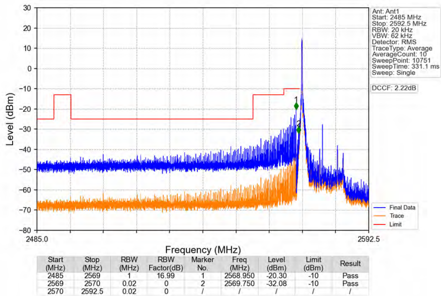
Band38_15MHz_16QAM_LCH_2577.5MHz_RB_1_0_NTNV
