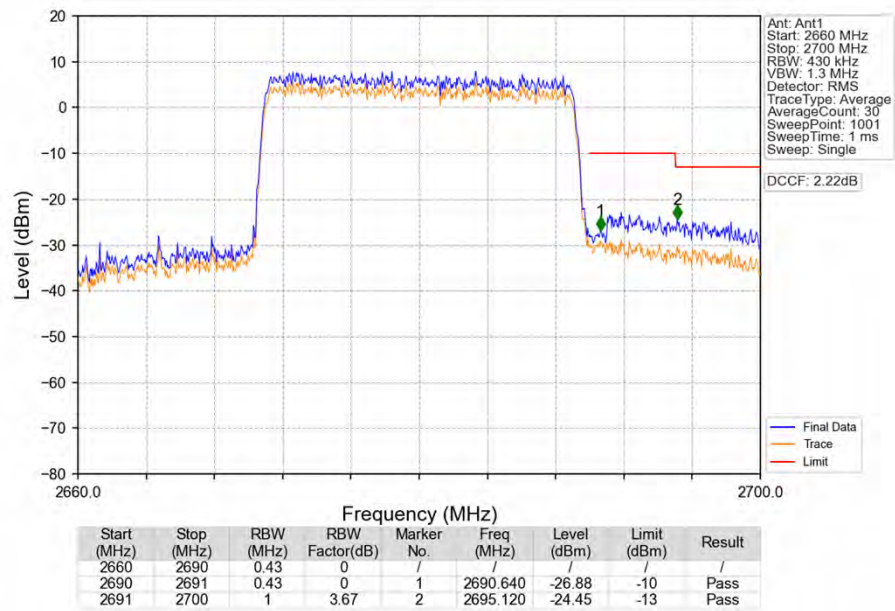
Band41_20MHz_16QAM_HCH_2680MHz_RB_100_0_NTNV
