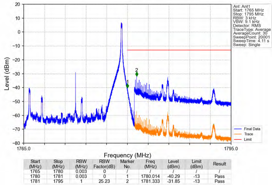
Band66_15MHz_QPSK_HCH_1772.5MHz_RB_1_74_NTNV
