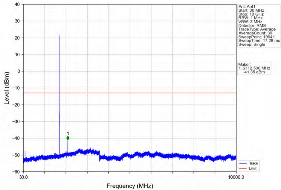
Band66_3MHz_16QAM_LCH_1711.5MHz_RB_1_0_NTNV
