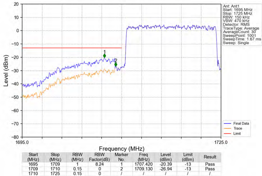
Band66_15MHz_QPSK_LCH_1717.5MHz_RB_75_0_NTNV
