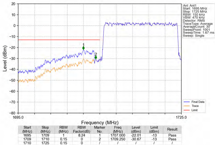
Band66_15MHz_16QAM_LCH_1717.5MHz_RB_75_0_NTNV
