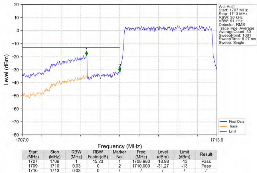
Band66_3MHz_16QAM_LCH_1711.5MHz_RB_15_0_NTNV
