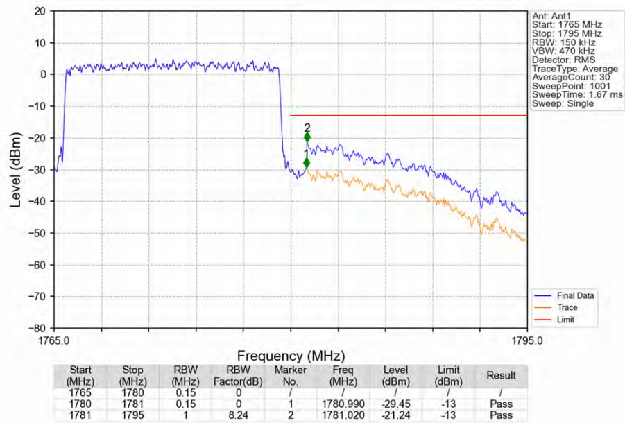
Band66_15MHz_QPSK_HCH_1772.5MHz_RB_75_0_NTNV
