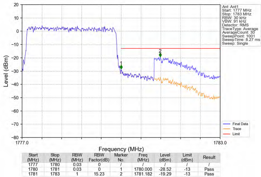
Band66_3MHz_16QAM_HCH_1778.5MHz_RB_15_0_NTNV
