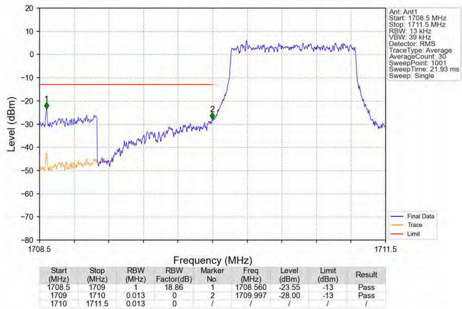
Band66_1.4MHz_QPSK_LCH_1710.7MHz_RB_6_0_NTNV
