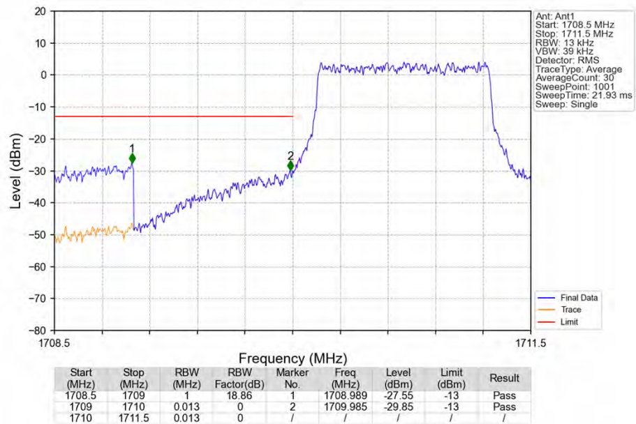
Band66_1.4MHz_16QAM_LCH_1710.7MHz_RB_6_0_NTNV
