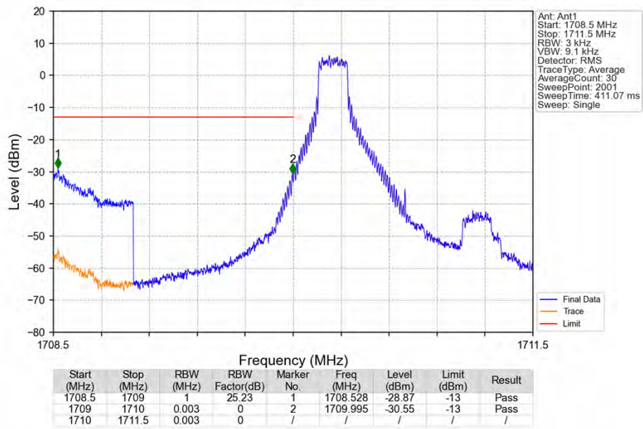
Band66_1.4MHz_16QAM_LCH_1710.7MHz_RB_1_0_NTNV
