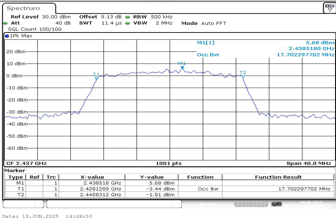
11N20SISO-Ant1-2437
