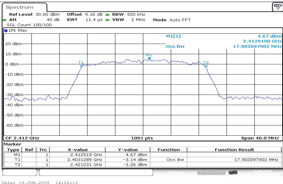
11N20SISO-Ant1-2412
