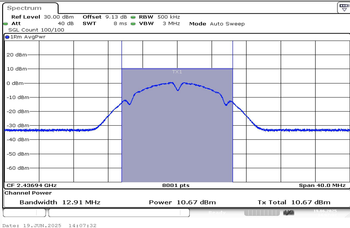
11B-Ant1-2437-PASS
