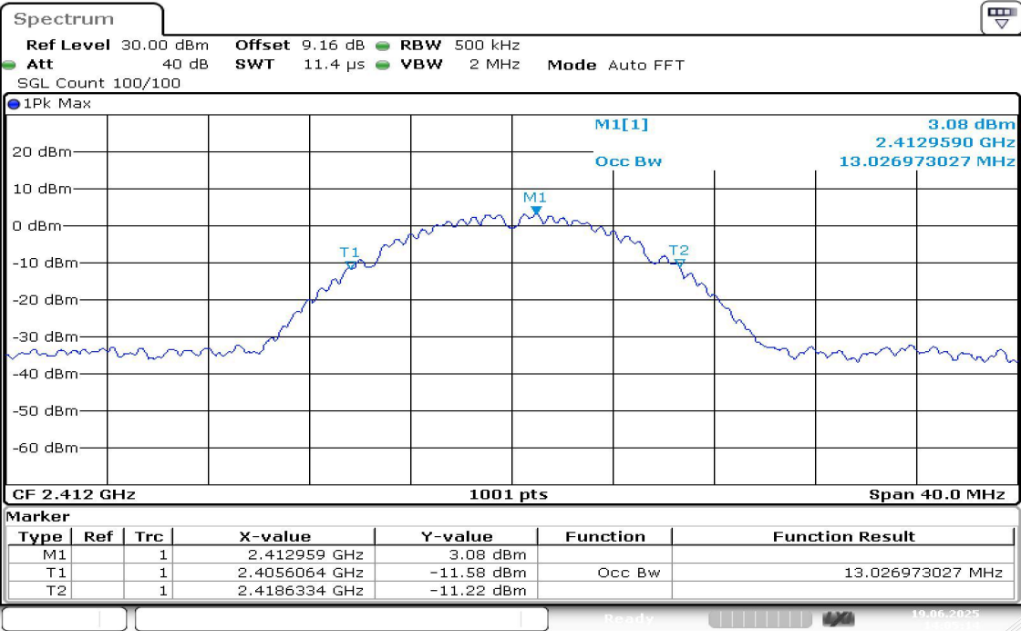
11B-Ant1-2412
