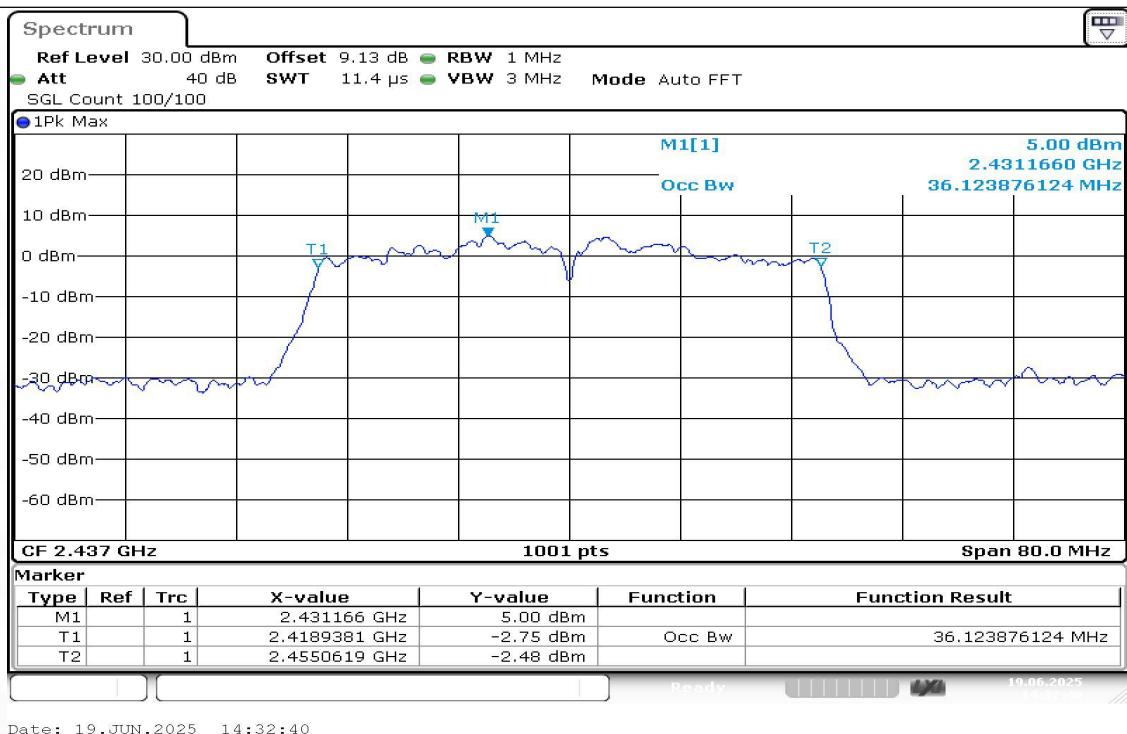
11N40SISO-Ant1-2437
