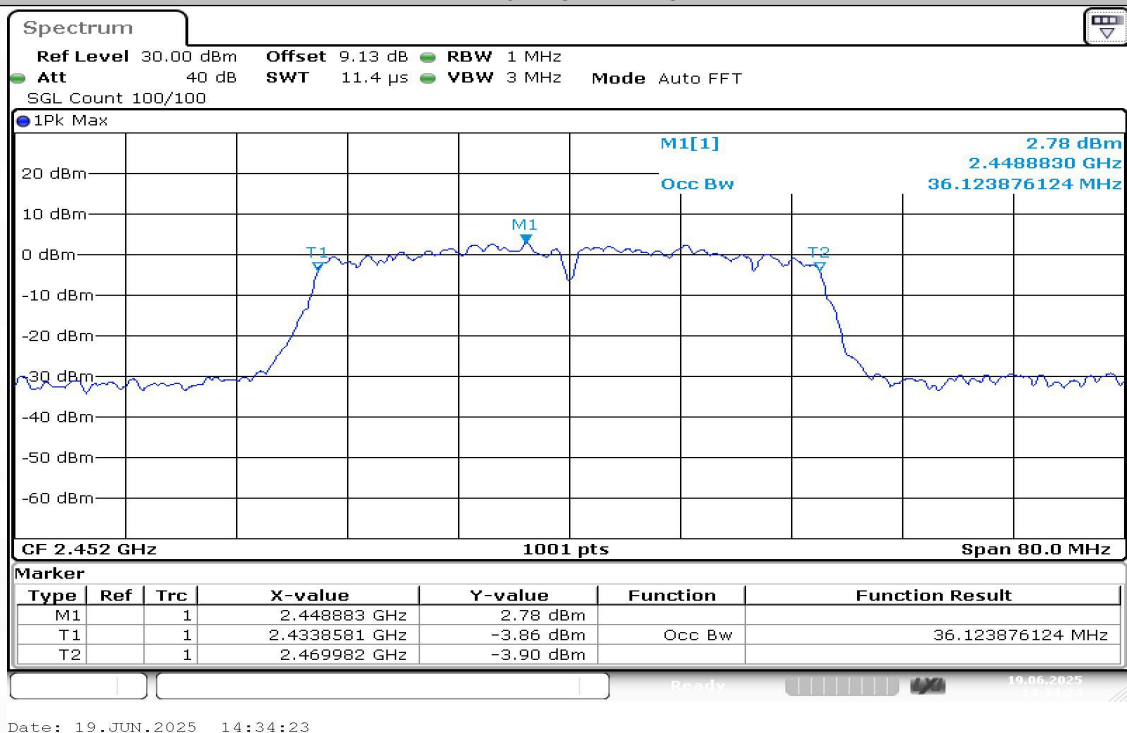
11N40SISO-Ant1-2452
