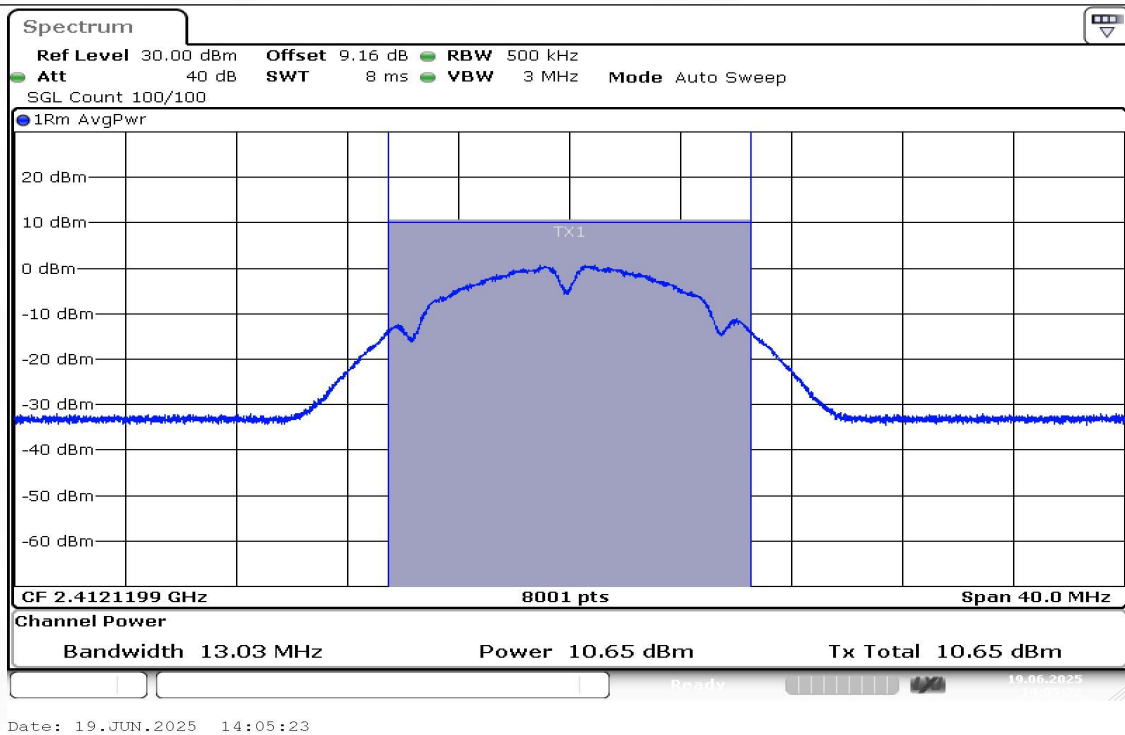
11B-Ant1-2412-PASS
