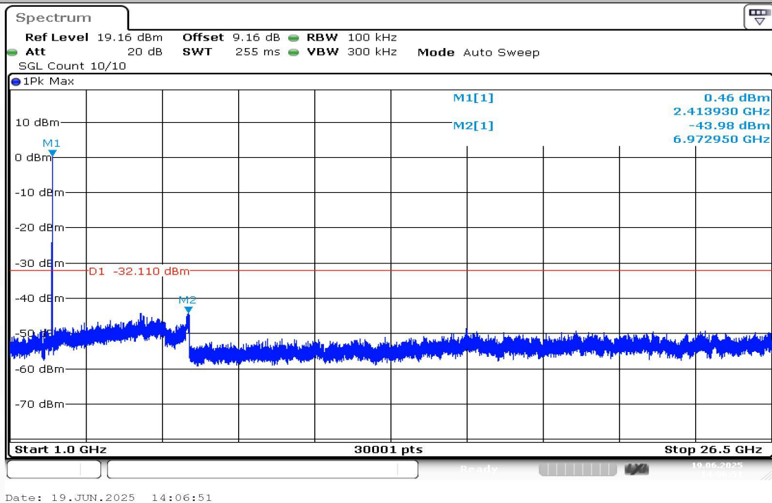
11B-Ant1-2412-1000~26500-PASS
