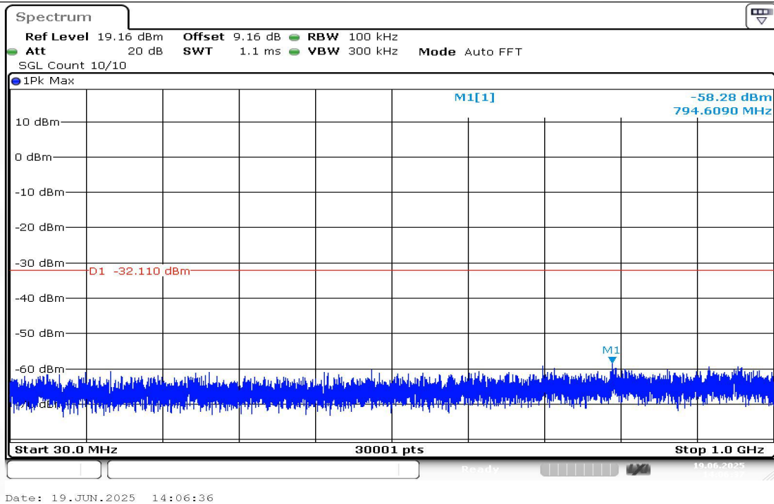
11B-Ant1-2412-30~1000-PASS
