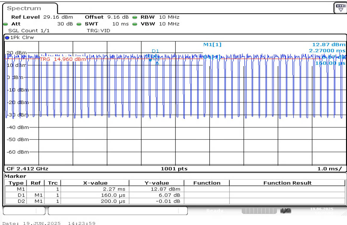
NTNV-11N20SISO-Ant1-2412
