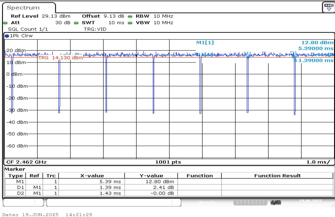
NTNV-11G-Ant1-2462
