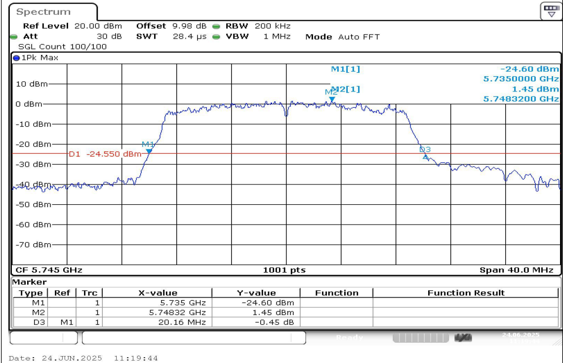
11N20SISO-Ant1-5745
