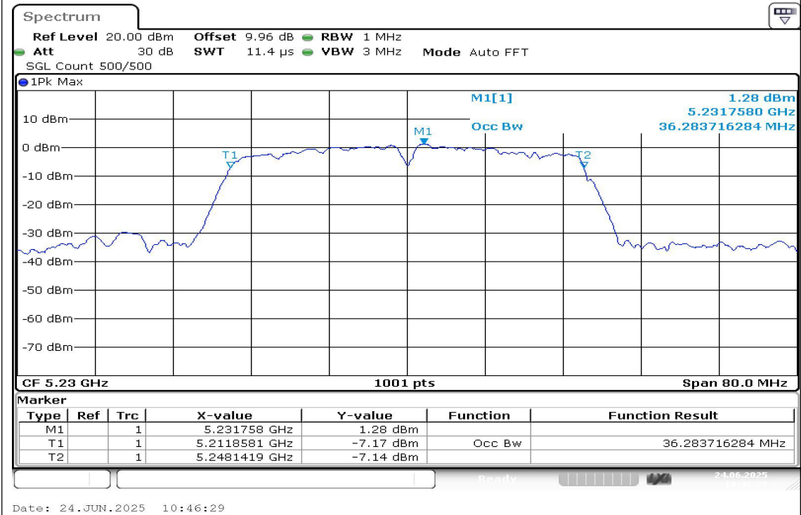
11AC40SISO-Ant1-5230
