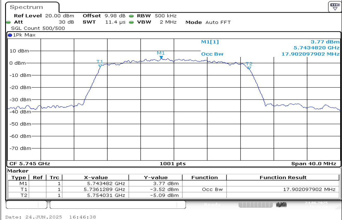
11AC20SISO-Ant1-5745
