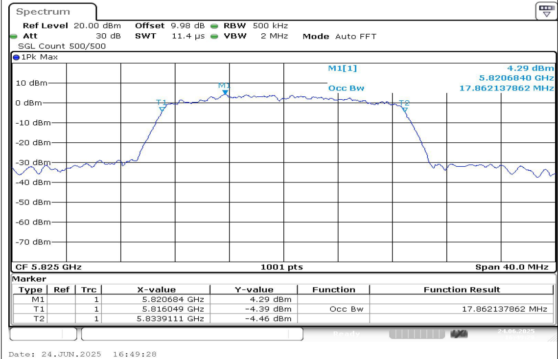
11AC20SISO-Ant1-5825
