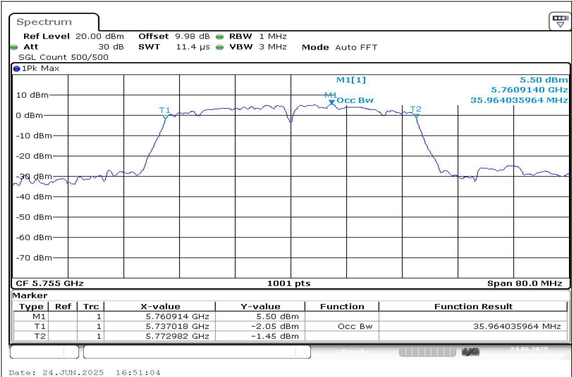
11AC40SISO-Ant1-5755
