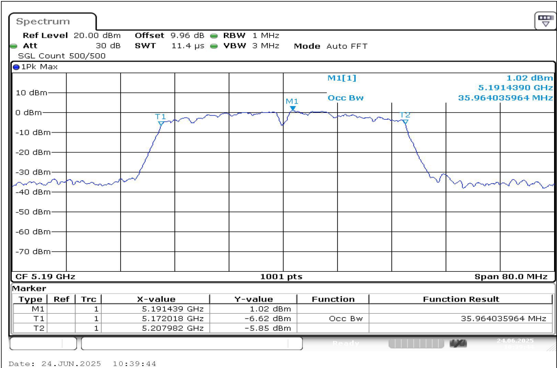
11AC40SISO-Ant1-5190
