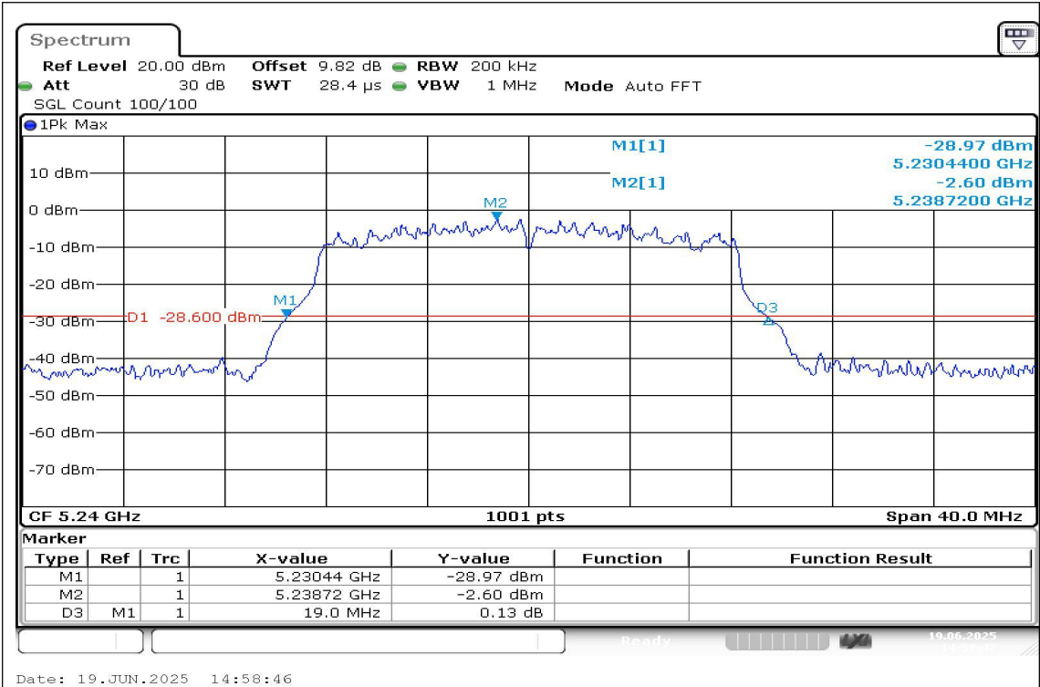
11A-Ant1-5240
