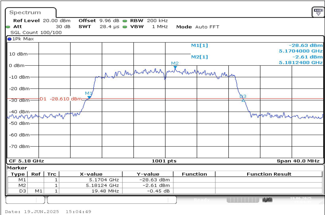
11N20SISO-Ant1-5180
