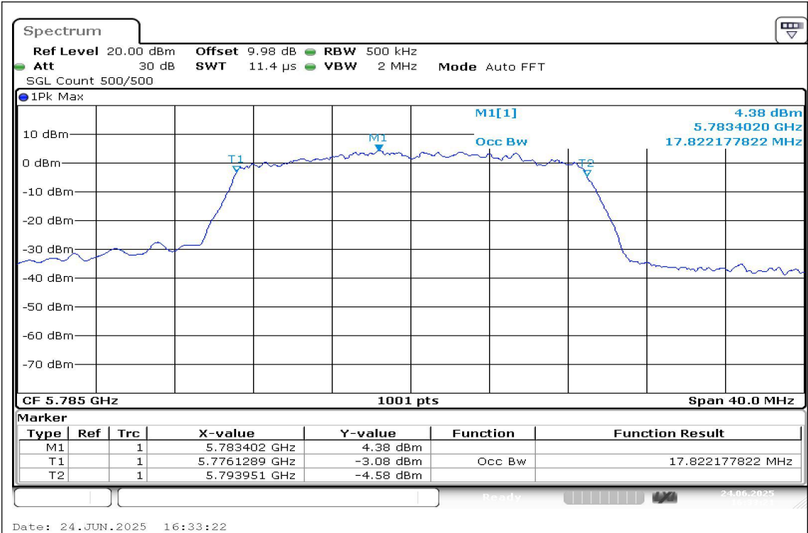
11N20SISO-Ant1-5785
