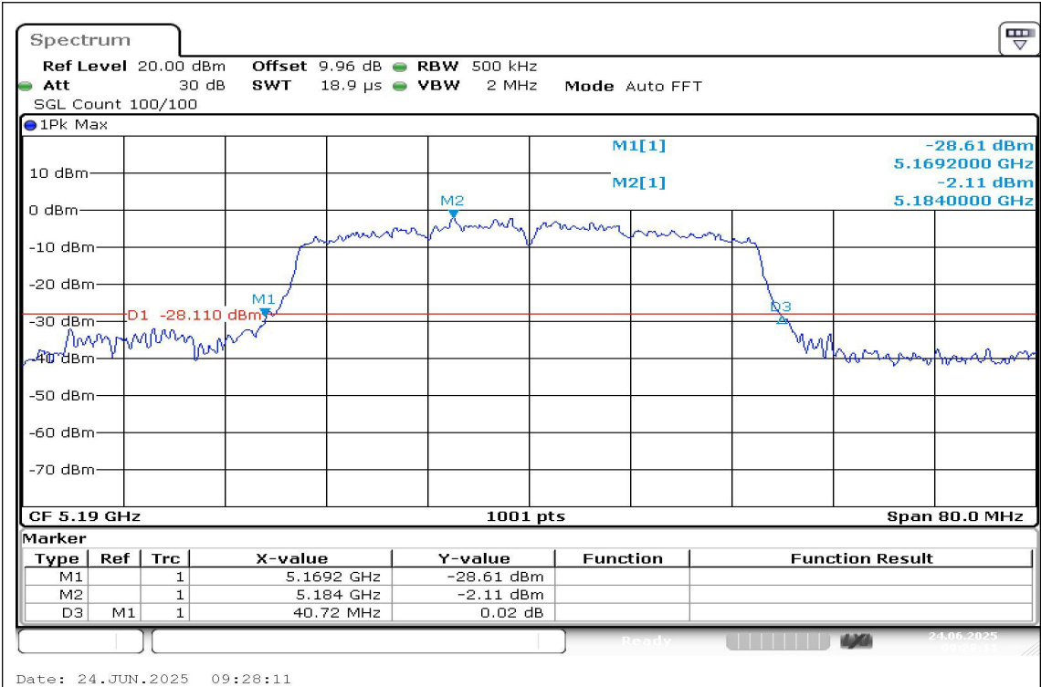
11N40SISO-Ant1-5190
