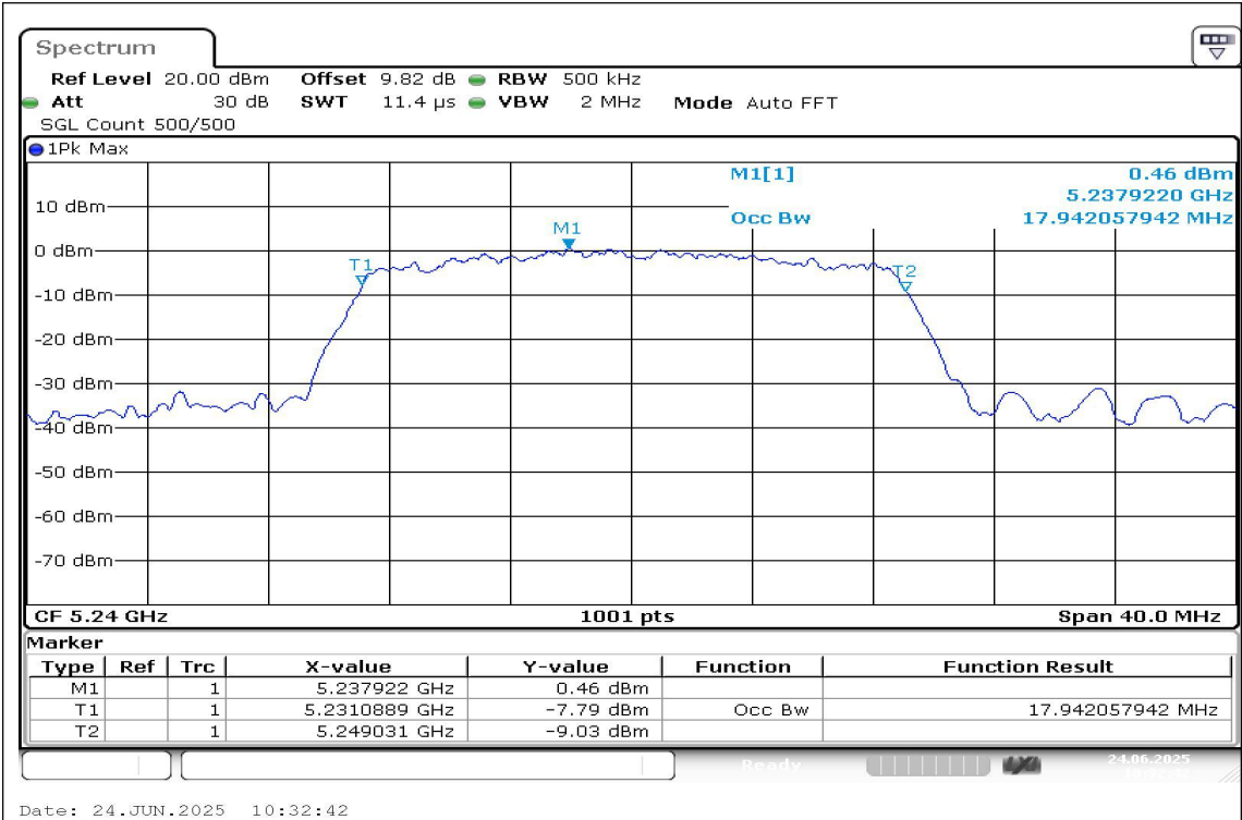
11AC20SISO-Ant1-5240
