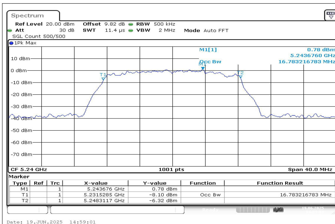
11A-Ant1-5240
