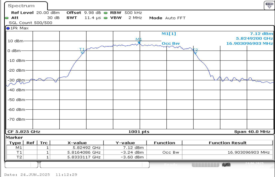
11A-Ant1-5825
