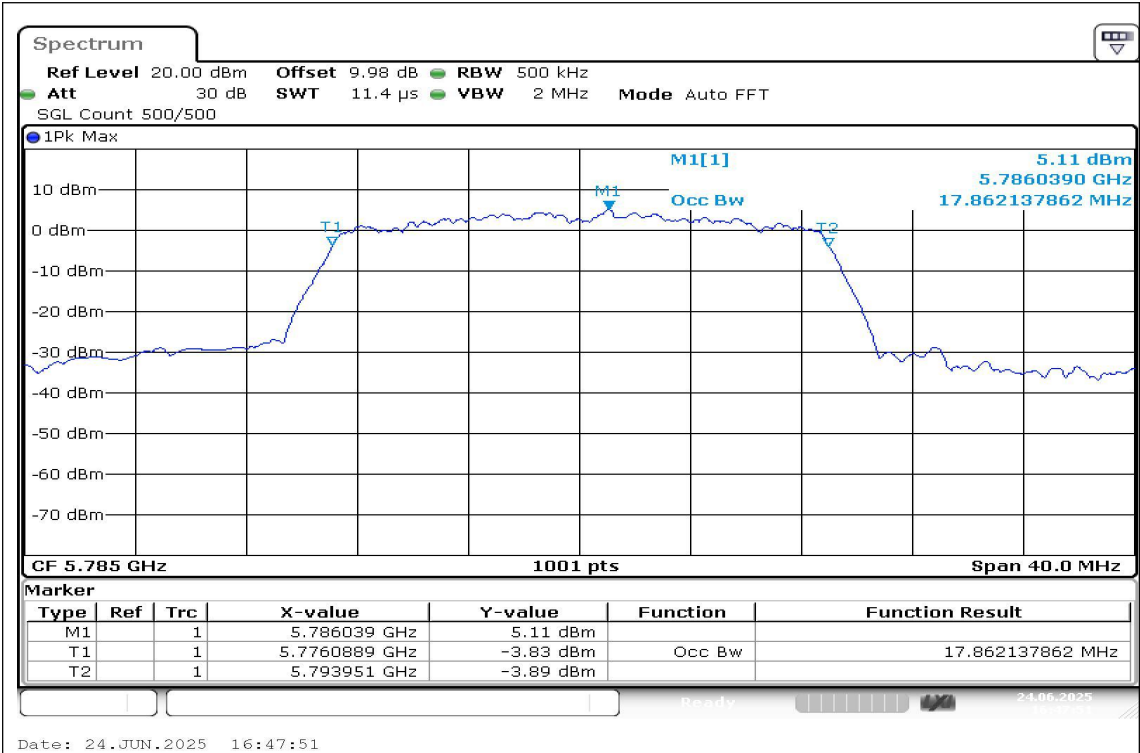
11AC20SISO-Ant1-5785
