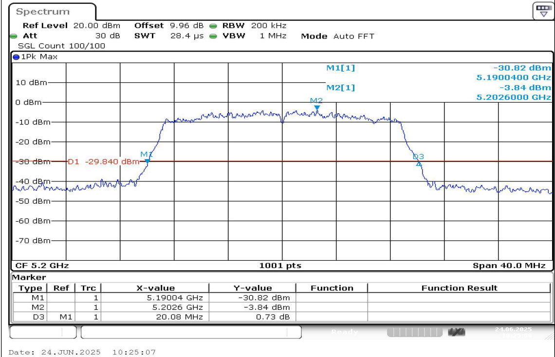
11AC20SISO-Ant1-5200
