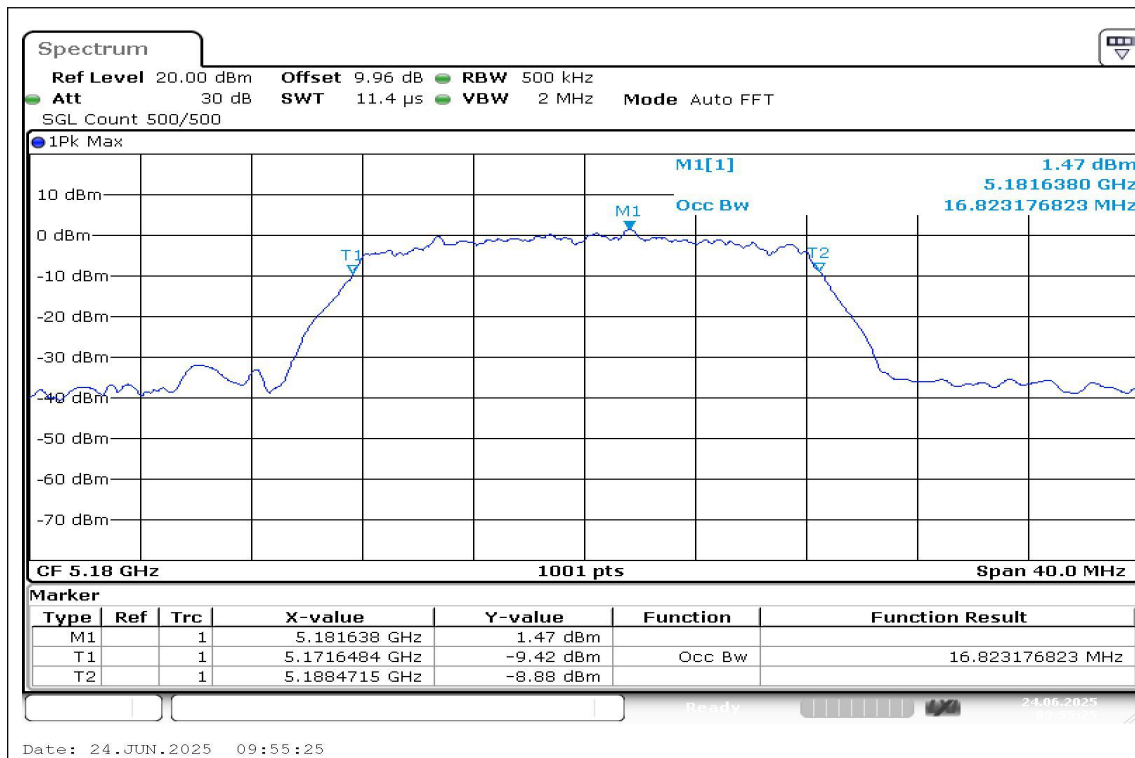
11A-Ant1-5180
