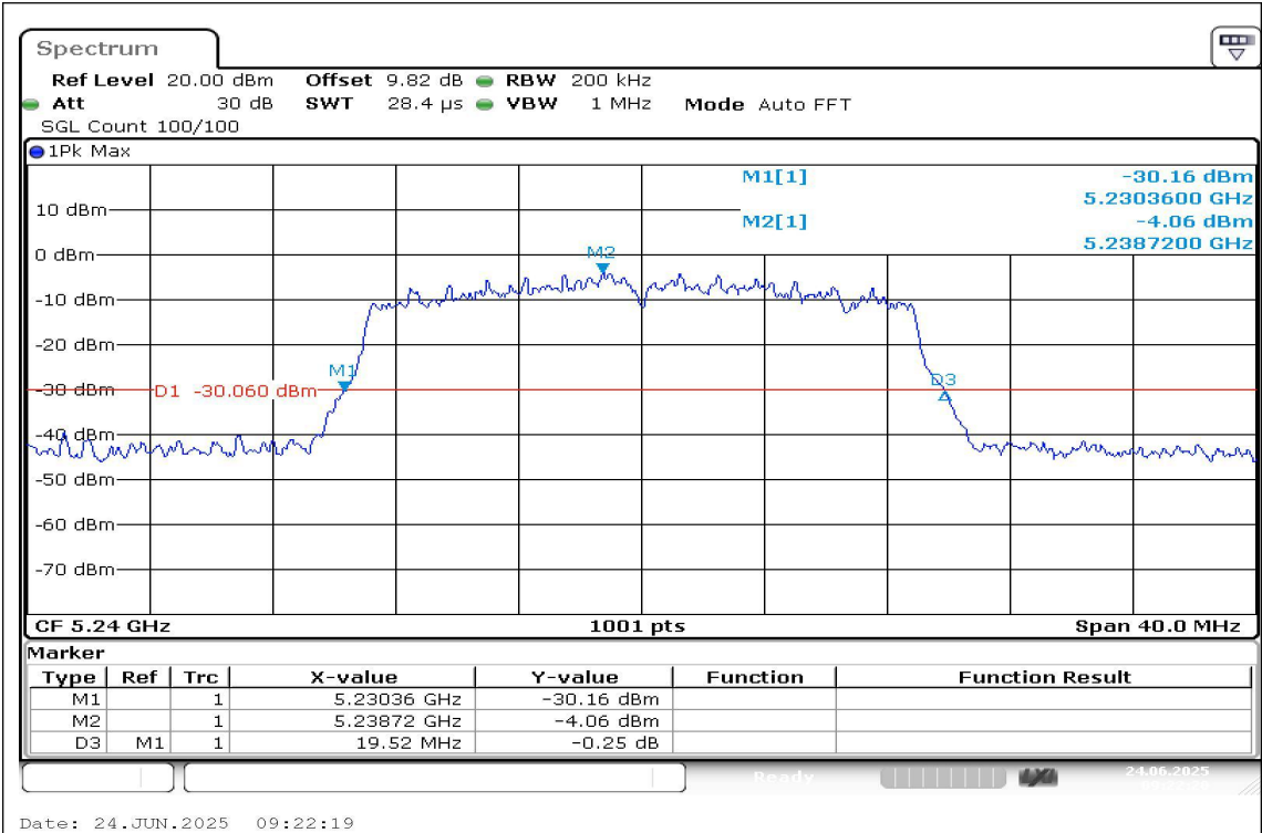
11N20SISO-Ant1-5240
