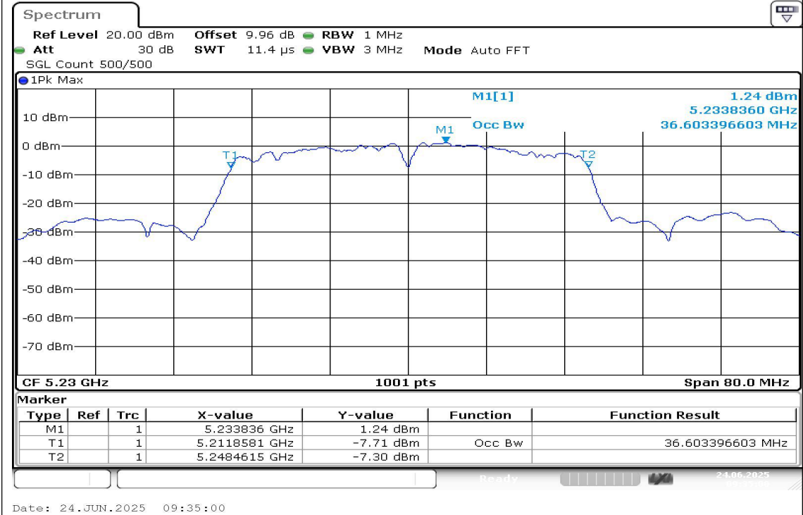
11N40SISO-Ant1-5230
