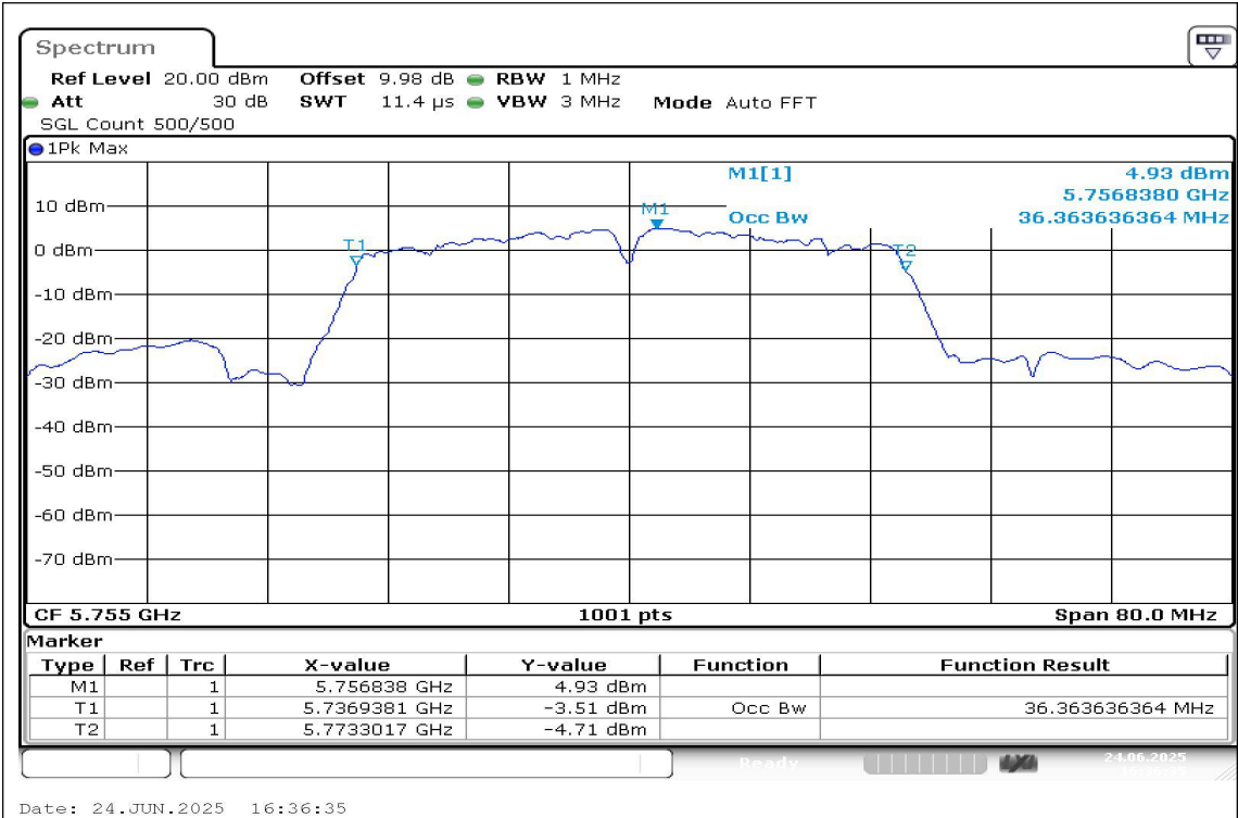
11N40SISO-Ant1-5755
