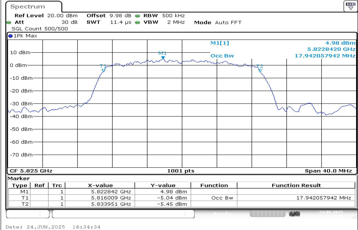
11N20SISO-Ant1-5825
