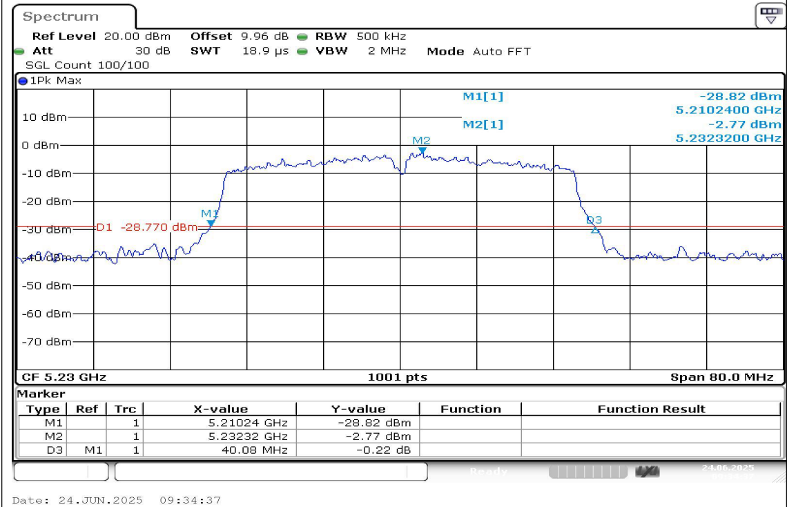
11N40SISO-Ant1-5230
