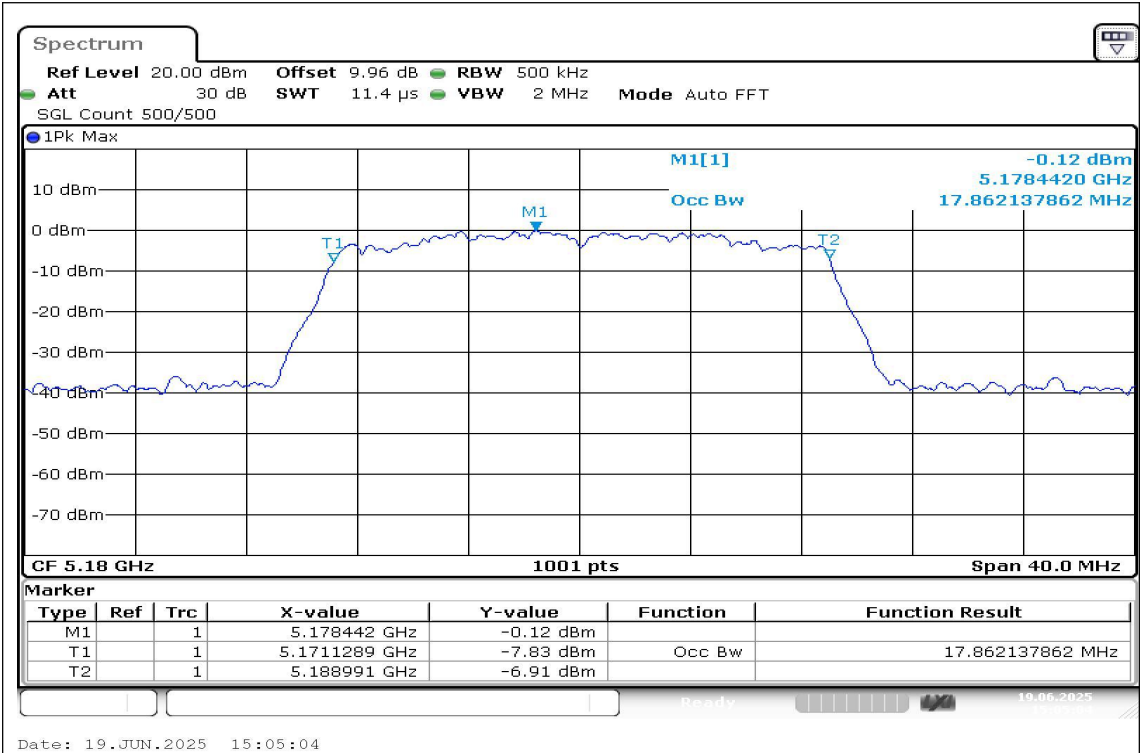
11N20SISO-Ant1-5180
