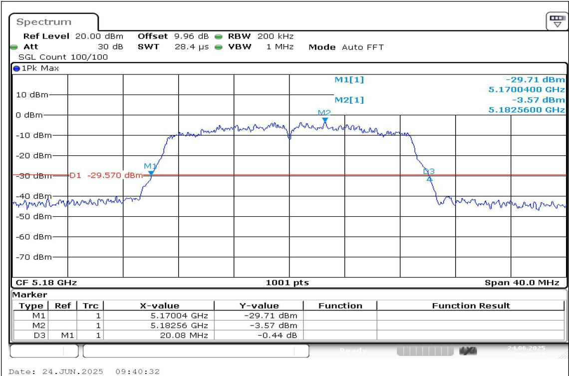
11AC20SISO-Ant1-5180
