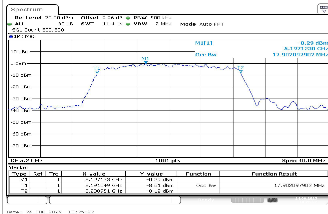
11AC20SISO-Ant1-5200
