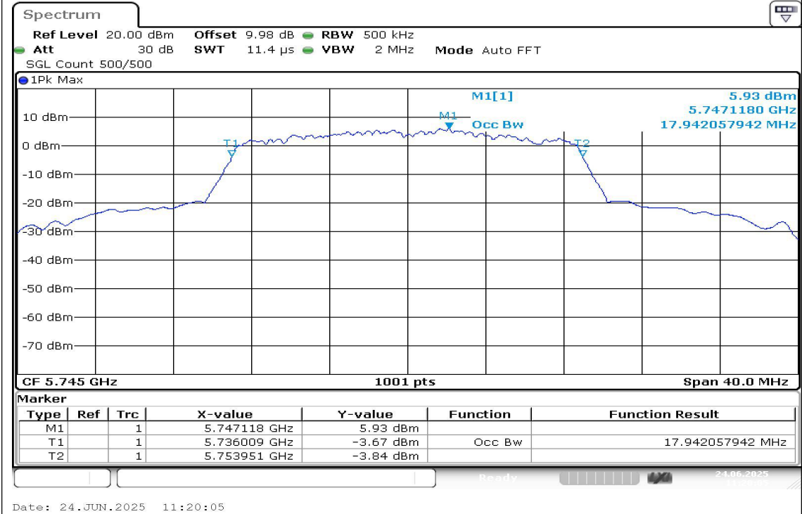
11N20SISO-Ant1-5745
