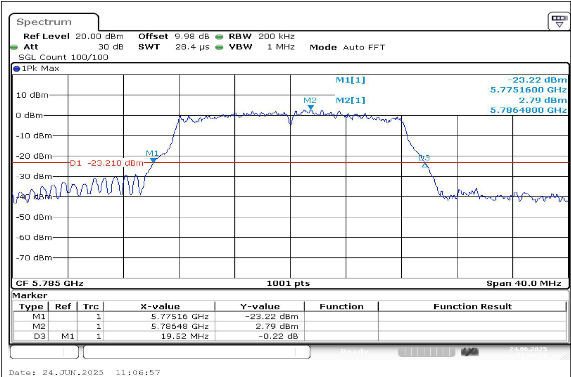
11A-Ant1-5785
