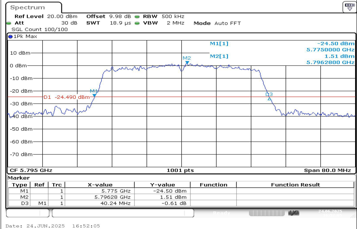
11AC40SISO-Ant1-5795
