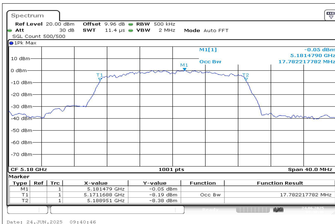
11AC20SISO-Ant1-5180
