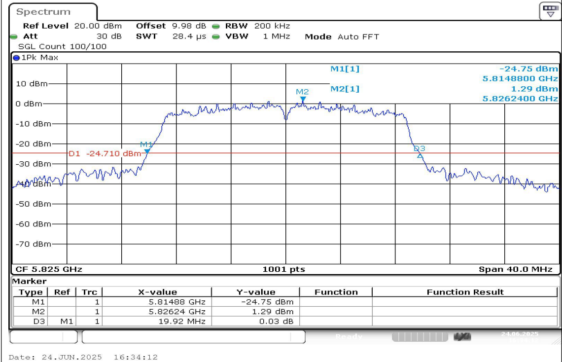
11N20SISO-Ant1-5825
