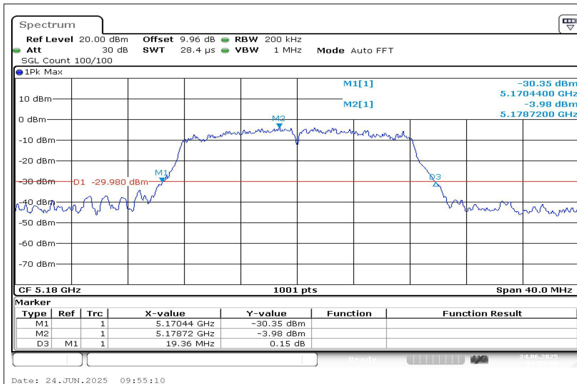
11A-Ant1-5180
