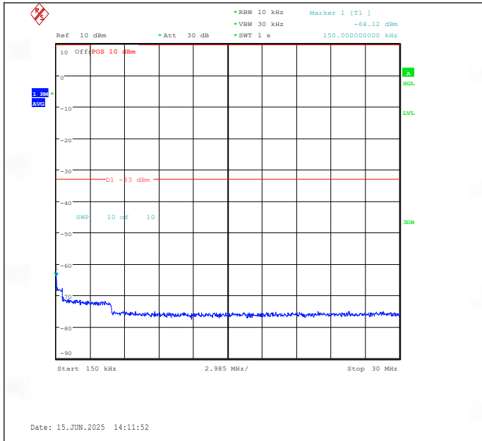
Band25-3MHz-16QAM-26675-1RB#0-0.15~30-PASS
