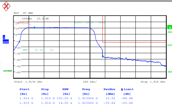
Band25-1.4MHz-QPSK-26683-1RB#0-PASS
