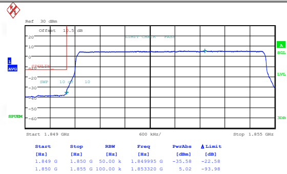
Band25-5MHz-16QAM-26065-1RB#0-PASS
