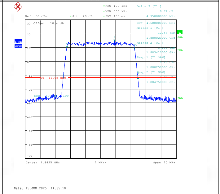
Band25-5MHz-16QAM-26365-25RB#0-PASS
