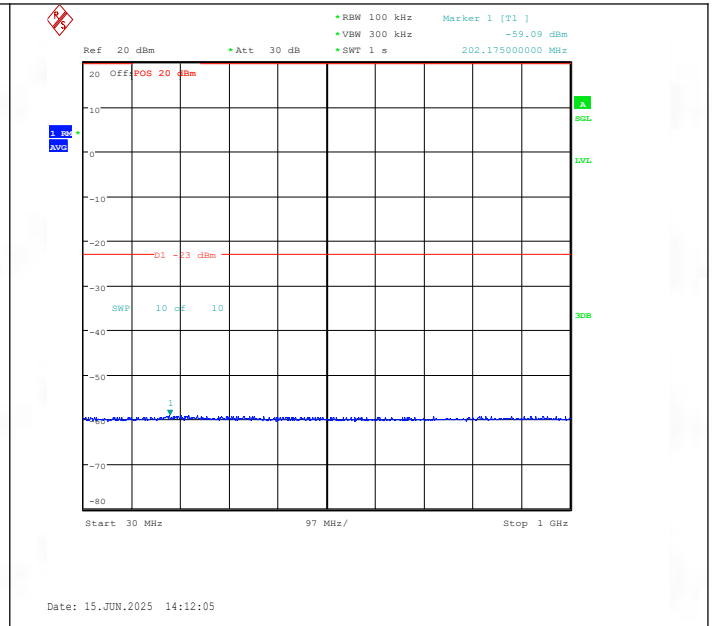
Band25-3MHz-16QAM-26675-1RB#0-30~1000-PASS
