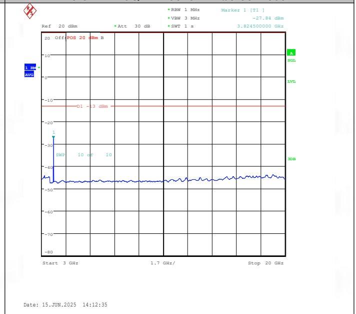
Band25-3MHz-16QAM-26675-1RB#0-3000~20000-PASS
