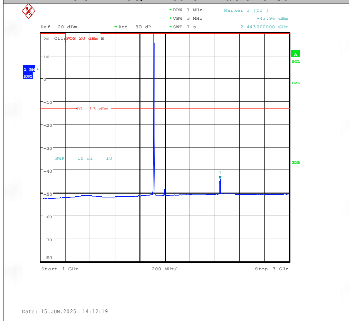
Band25-3MHz-16QAM-26675-1RB#0-1000~3000-PASS
