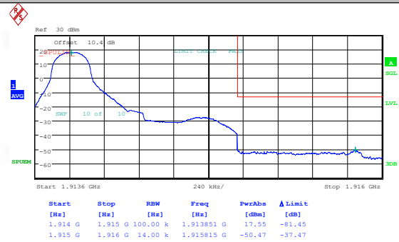
Band25-1.4MHz-QPSK-26683-1RB#5-PASS
