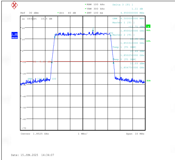
Band25-5MHz-QPSK-26065-25RB#0-PASS
