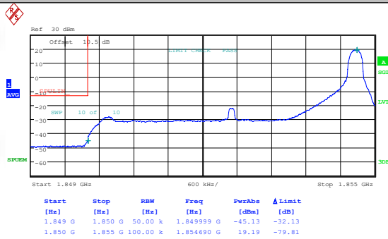
Band25-5MHz-QPSK-26065-25RB#0-PASS
