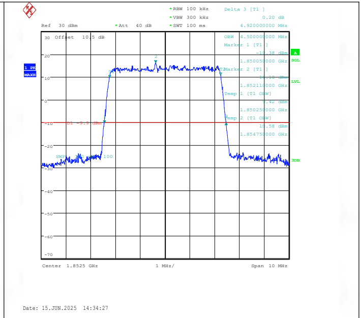
Band25-5MHz-16QAM-26065-25RB#0-PASS
