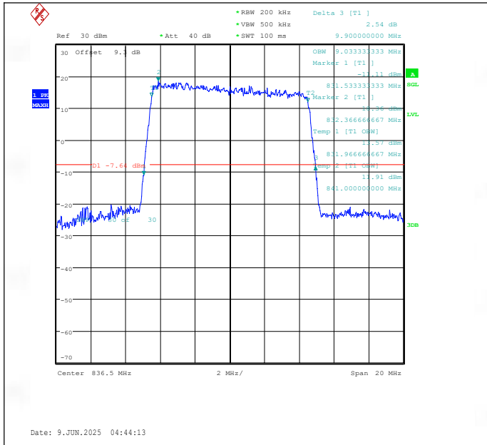
Band26(824-849)-10MHz-QPSK-26915-50RB#0-PASS
