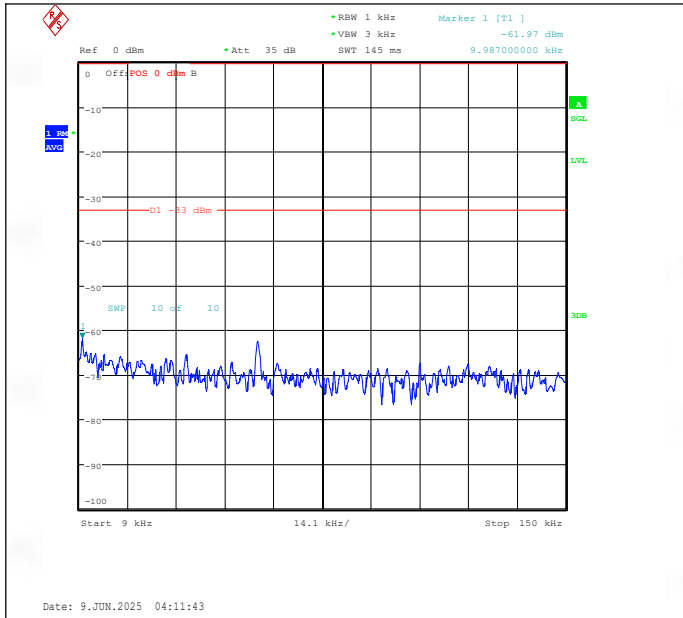
Band26(824-849)-5MHz-QPSK-26815-1RB#0-0.009~0.15-PASS
