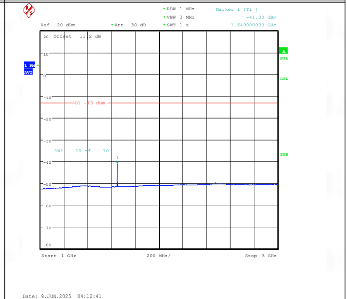
Band26(824-849)-5MHz-QPSK-26815-1RB#0-1000~3000-PASS
