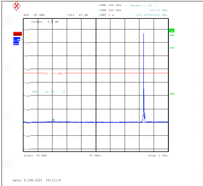
Band26(824-849)-5MHz-QPSK-26915-1RB#0-30~1000-PASS
