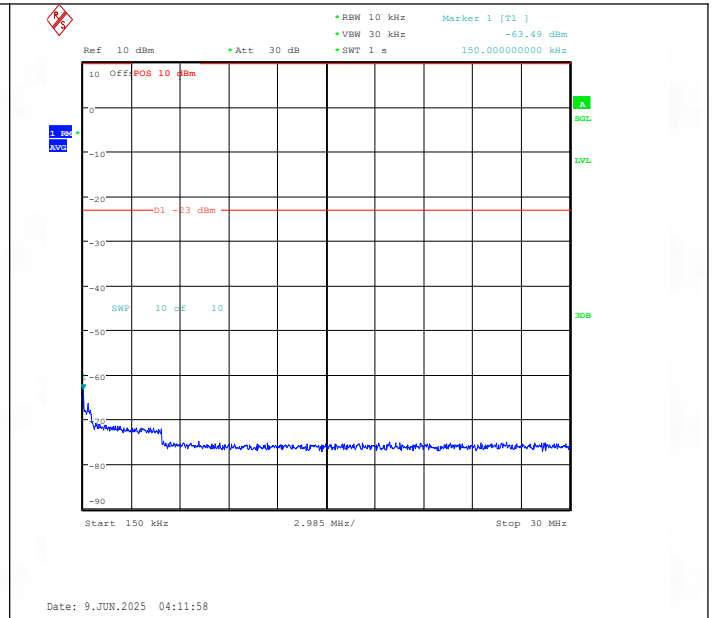
Band26(824-849)-5MHz-QPSK-26815-1RB#0-0.15~30-PASS
