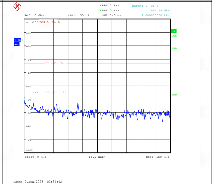
Band26(824-849)-3MHz-16QAM-26805-1RB#0-0.009~0.15-PASS
