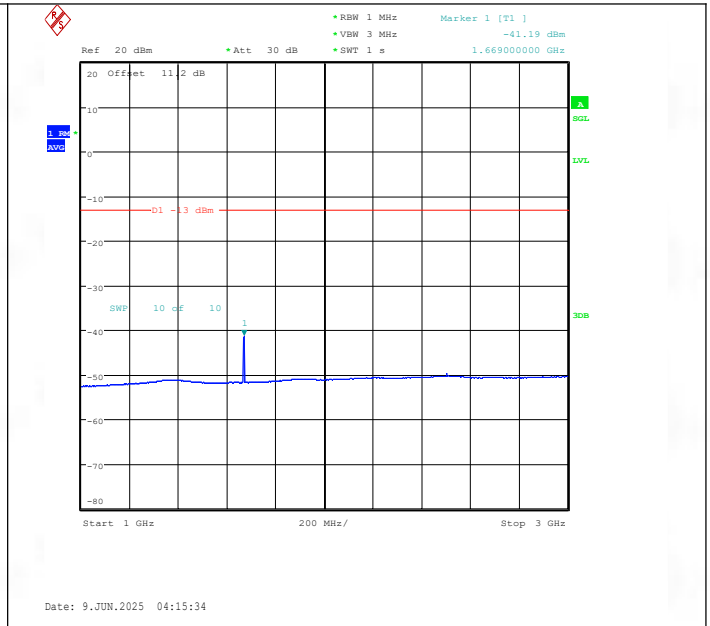
Band26(824-849)-5MHz-QPSK-26915-1RB#0-1000~3000-PASS
