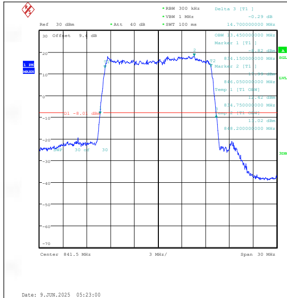
Band26(824-849)-15MHz-QPSK-26965-75RB#0-PASS
