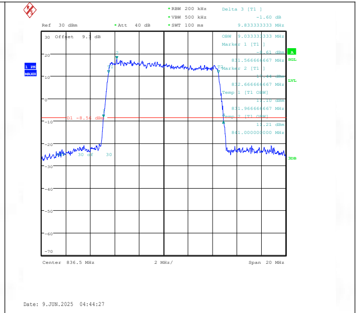
Band26(824-849)-10MHz-16QAM-26915-50RB#0-PASS
