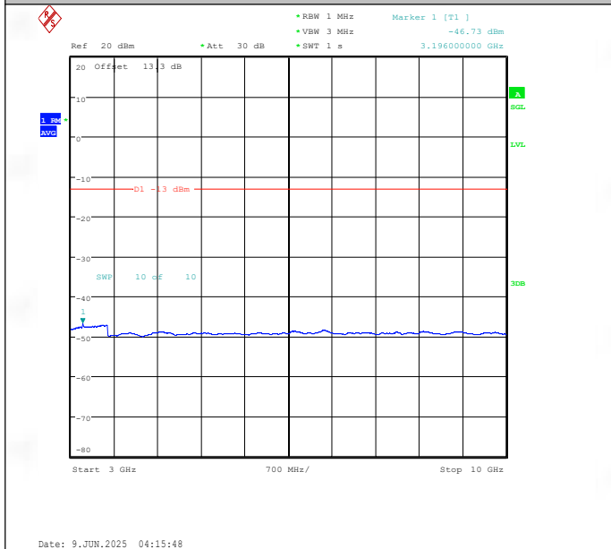
Band26(824-849)-5MHz-QPSK-26915-1RB#0-3000~10000-PASS
