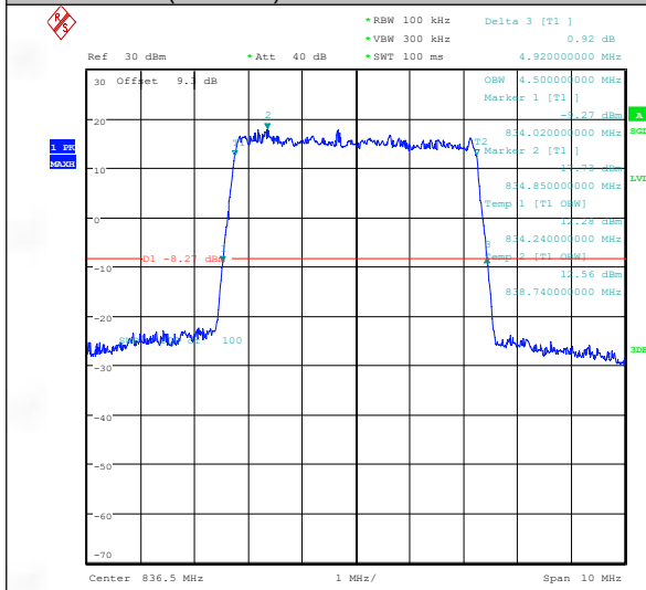
Band26(824-849)-5MHz-QPSK-26815-25RB#0-PASS
