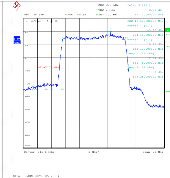
Band26(824-849)-15MHz-16QAM-26965-75RB#0-PASS
