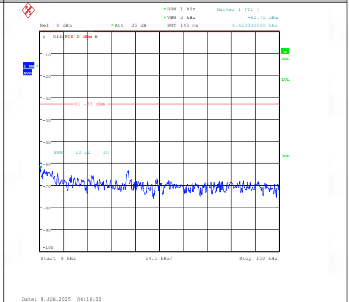
Band26(824-849)-5MHz-16QAM-26915-1RB#0-0.009~0.15-PASS
