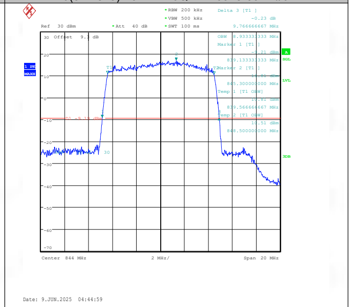
Band26(824-849)-10MHz-16QAM-26990-50RB#0-PASS
