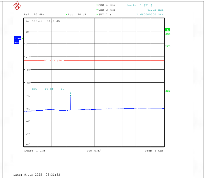
Band26(824-849)-15MHz-QPSK-26915-1RB#0-1000~3000-PASS
