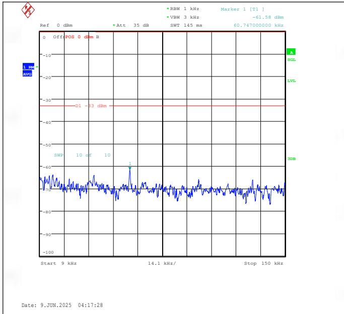
Band26(824-849)-5MHz-QPSK-27015-1RB#0-0.009~0.15-PASS
