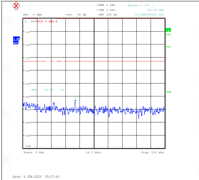
Band26(824-849)-15MHz-QPSK-26865-1RB#0-0.009~0.15-PASS
