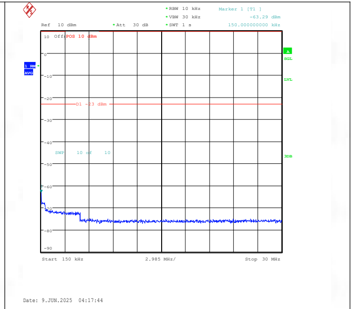
Band26(824-849)-5MHz-QPSK-27015-1RB#0-0.15~30-PASS
