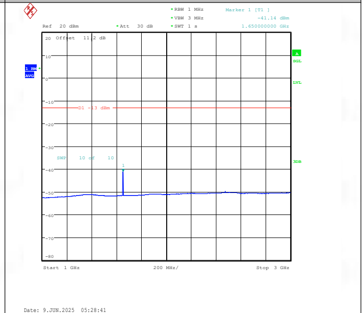
Band26(824-849)-15MHz-QPSK-26865-1RB#0-1000~3000-PASS
