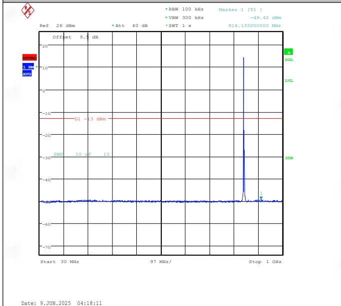
Band26(824-849)-5MHz-QPSK-27015-1RB#0-30~1000-PASS
