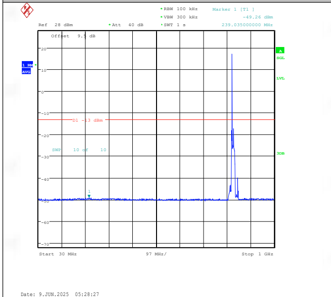
Band26(824-849)-15MHz-QPSK-26865-1RB#0-30~1000-PASS
