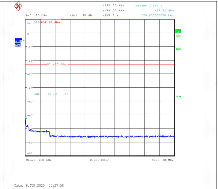
Band26(824-849)-15MHz-QPSK-26865-1RB#0-0.15~30-PASS
