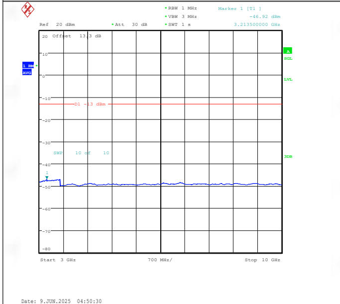
Band26(824-849)-10MHz-QPSK-26840-1RB#0-3000~10000-PASS
