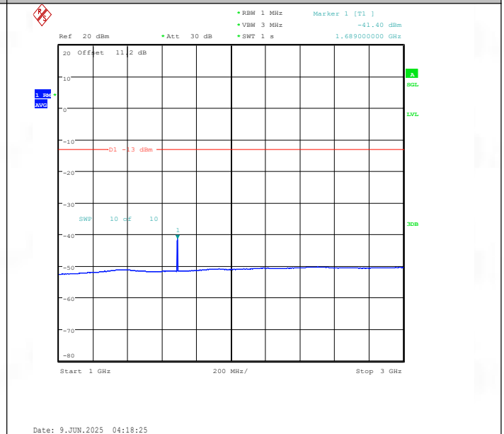
Band26(824-849)-5MHz-QPSK-27015-1RB#0-1000~3000-PASS
