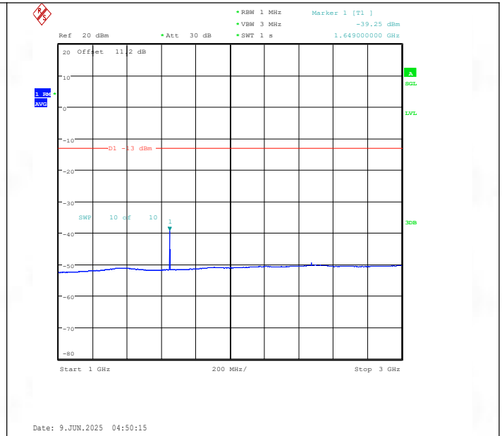
Band26(824-849)-10MHz-QPSK-26840-1RB#0-1000~3000-PASS
