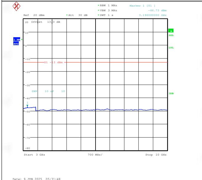
Band26(824-849)-15MHz-QPSK-26915-1RB#0-3000~10000-PASS
