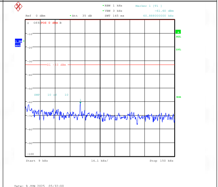
Band26(824-849)-15MHz-16QAM-26915-1RB#0-0.009~0.15-PASS
