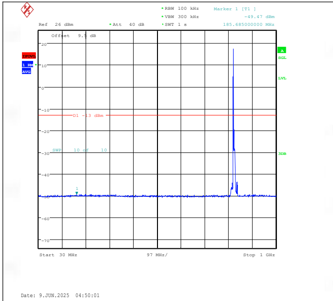
Band26(824-849)-10MHz-QPSK-26840-1RB#0-30~1000-PASS
