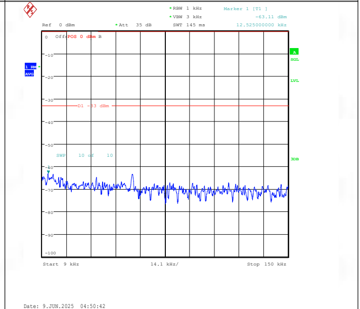
Band26(824-849)-10MHz-16QAM-26840-1RB#0-0.009~0.15-PASS
