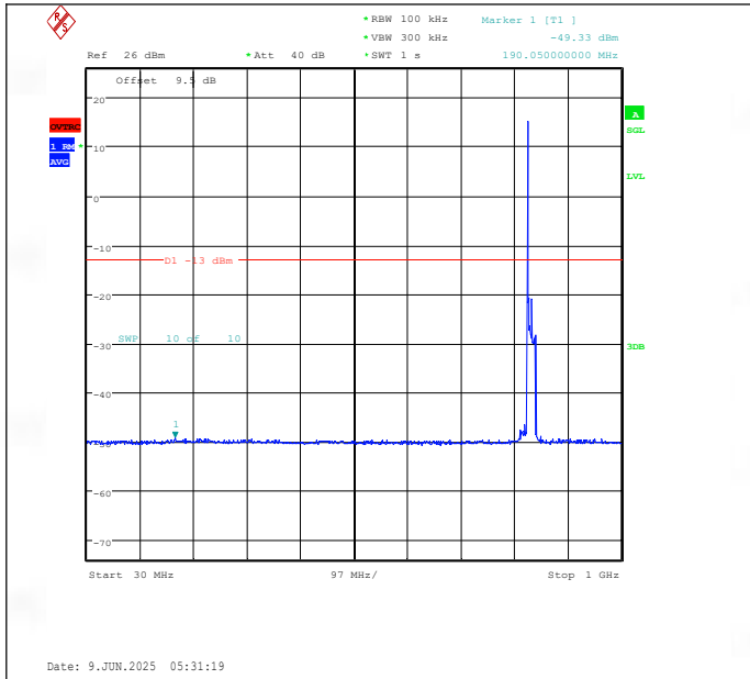
Band26(824-849)-15MHz-QPSK-26915-1RB#0-30~1000-PASS
