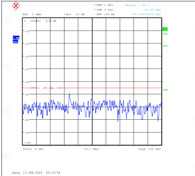
Band41(2535-2655)-15MHz-QPSK-40115-1RB#0-0.009~0.15-PASS
