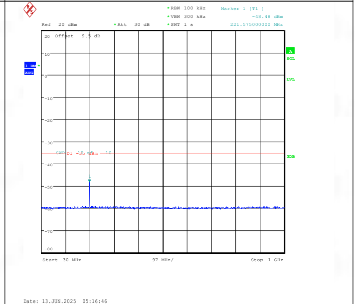
Band41(2535-2655)-15MHz-16QAM-40115-1RB#0-30~1000-PASS
