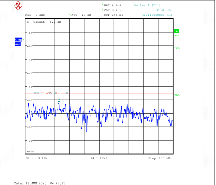
Band41(2535-2655)-10MHz-16QAM-41190-1RB#0-0.009~0.15-PASS
