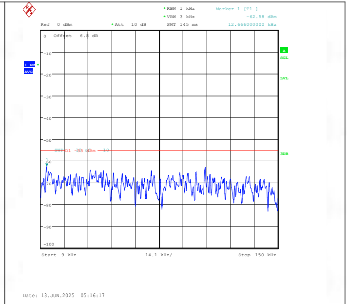
Band41(2535-2655)-15MHz-16QAM-40115-1RB#0-0.009~0.15-PASS
