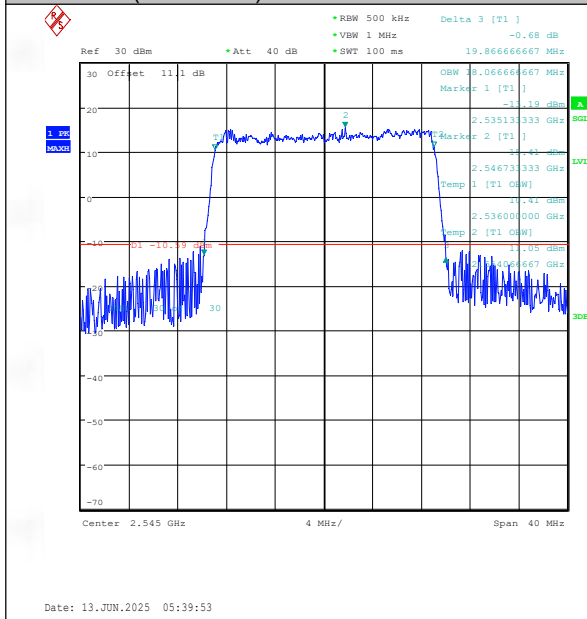
Band41(2535-2655)-20MHz-QPSK-40140-100RB#0-PASS
