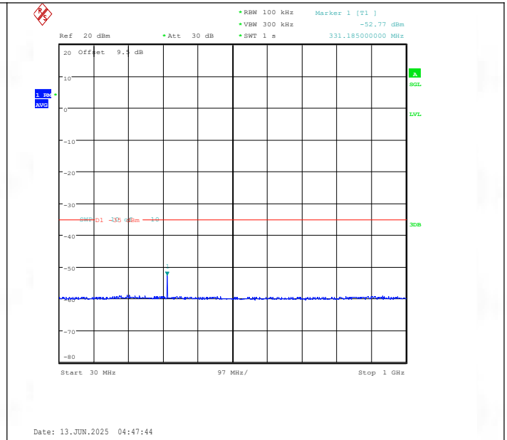
Band41(2535-2655)-10MHz-16QAM-41190-1RB#0-30~1000-PASS
