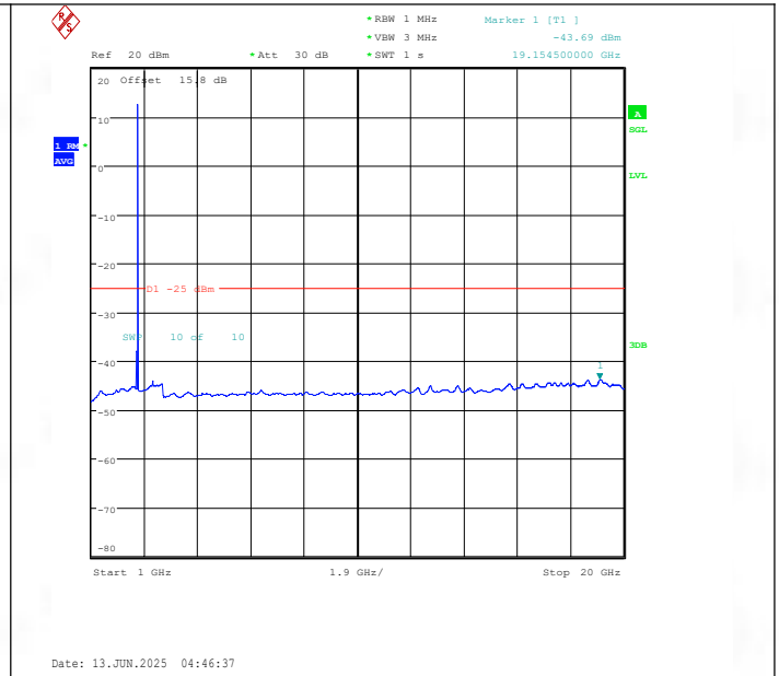
Band41(2535-2655)-10MHz-QPSK-41190-1RB#0-1000~20000-PASS
