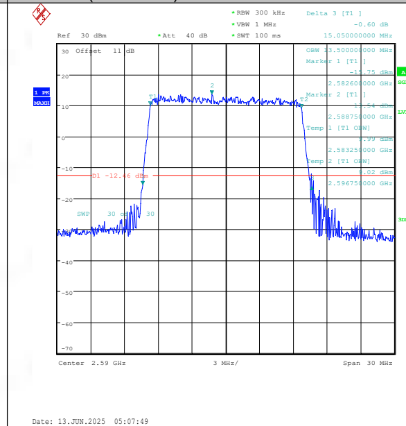
Band41(2535-2655)-15MHz-16QAM-40590-75RB#0-PASS
