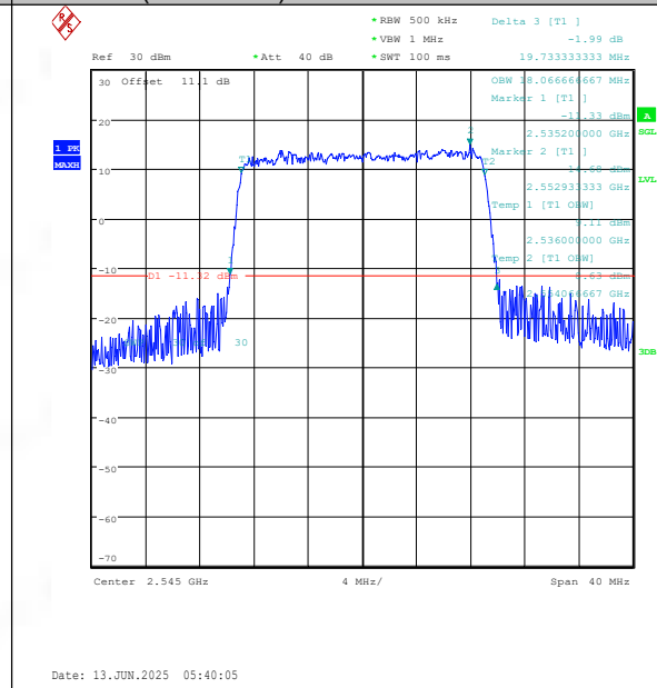
Band41(2535-2655)-20MHz-16QAM-40140-100RB#0-PASS
