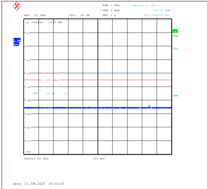
Band41(2535-2655)-15MHz-QPSK-40115-1RB#0-20000~27000-PASS
