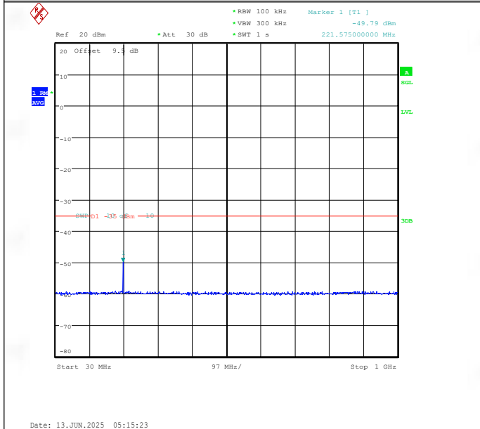
Band41(2535-2655)-15MHz-QPSK-40115-1RB#0-30~1000-PASS
