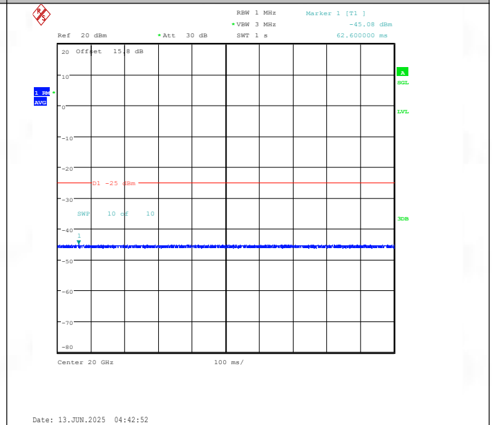
Band41(2535-2655)-10MHz-16QAM-40090-1RB#0-20000~27000-PASS
