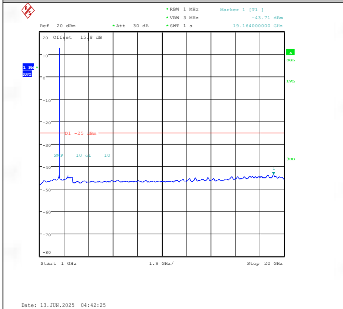
Band41(2535-2655)-10MHz-16QAM-40090-1RB#0-1000~20000-PASS
