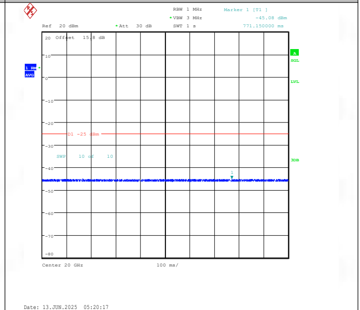
Band41(2535-2655)-15MHz-16QAM-40590-1RB#0-20000~27000-PASS
