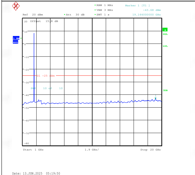
Band41(2535-2655)-15MHz-16QAM-40590-1RB#0-1000~20000-PASS
