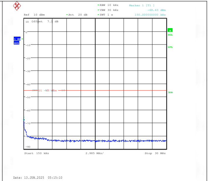
Band41(2535-2655)-15MHz-QPSK-40115-1RB#0-0.15~30-PASS
