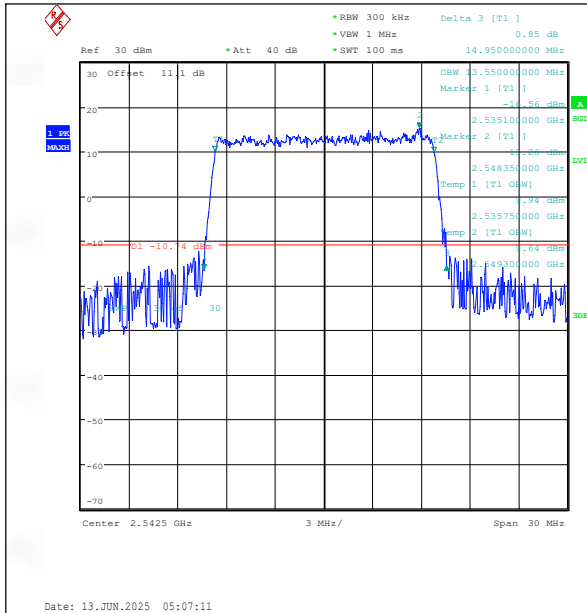
Band41(2535-2655)-15MHz-QPSK-40115-75RB#0-PASS
