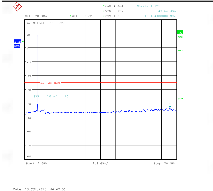
Band41(2535-2655)-10MHz-16QAM-41190-1RB#0-1000~20000-PASS
