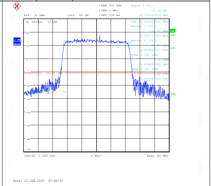
Band41(2535-2655)-20MHz-16QAM-41140-100RB#0-PASS
