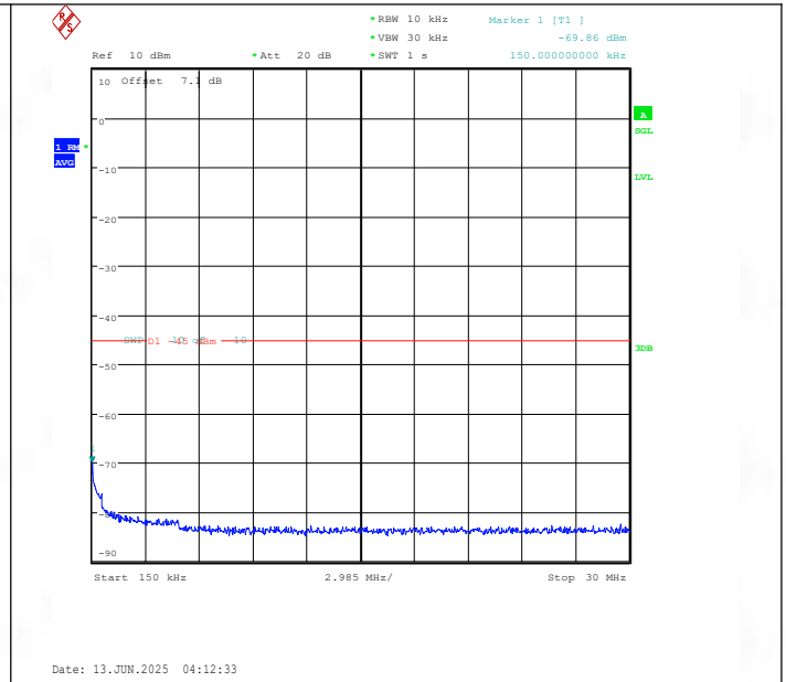
Band41(2535-2655)-5MHz-QPSK-41215-1RB#0-0.15~30-PASS
