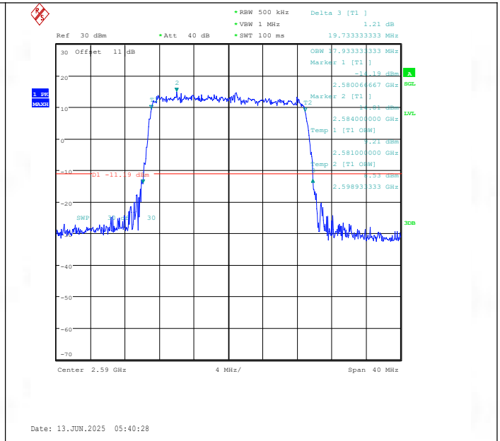
Band41(2535-2655)-20MHz-16QAM-40590-100RB#0-PASS
