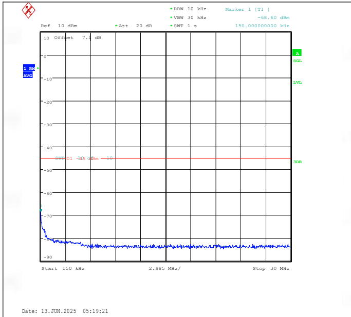
Band41(2535-2655)-15MHz-16QAM-40590-1RB#0-0.15~30-PASS
