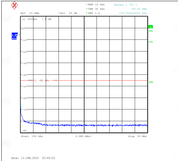
Band41(2535-2655)-20MHz-16QAM-40140-1RB#0-0.15~30-PASS
