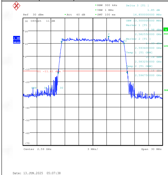
Band41(2535-2655)-15MHz-QPSK-40590-75RB#0-PASS
