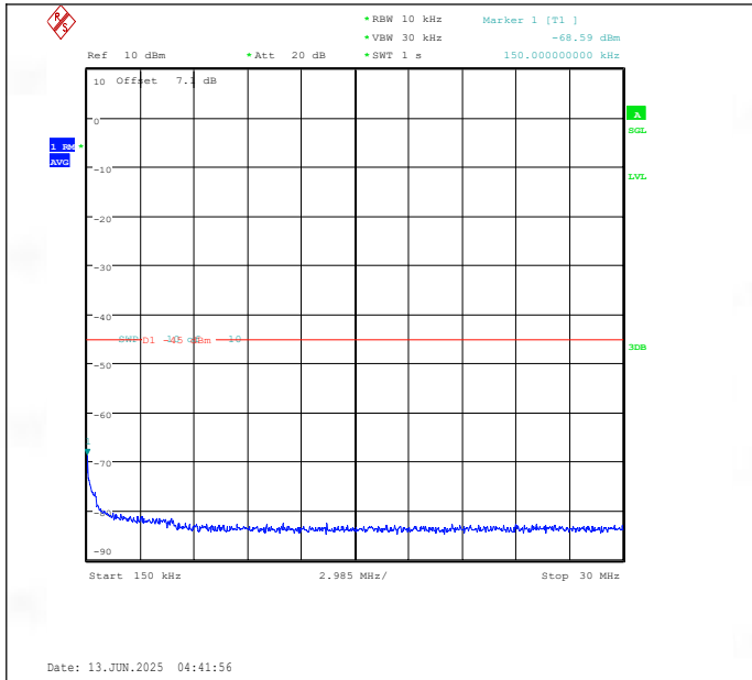
Band41(2535-2655)-10MHz-16QAM-40090-1RB#0-0.15~30-PASS
