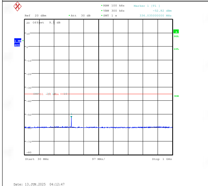
Band41(2535-2655)-5MHz-QPSK-41215-1RB#0-30~1000-PASS
