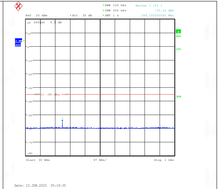
Band41(2535-2655)-15MHz-16QAM-40590-1RB#0-30~1000-PASS
