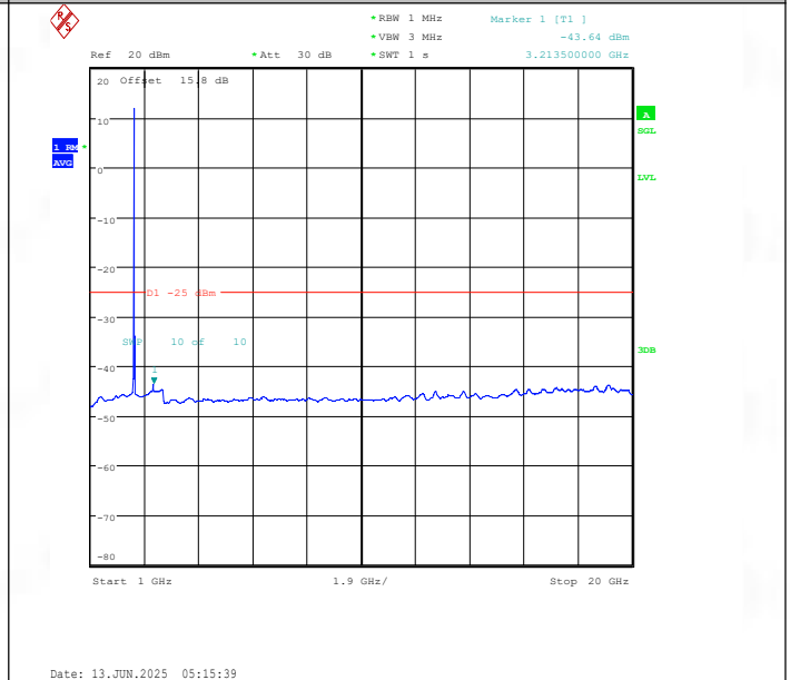
Band41(2535-2655)-15MHz-QPSK-40115-1RB#0-1000~20000-PASS
