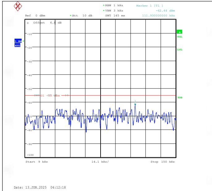
Band41(2535-2655)-5MHz-QPSK-41215-1RB#0-0.009~0.15-PASS
