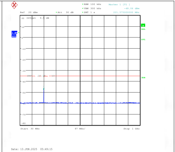
Band41(2535-2655)-20MHz-16QAM-40140-1RB#0-30~1000-PASS
