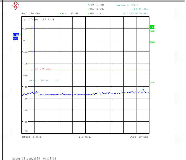
Band41(2535-2655)-5MHz-QPSK-41215-1RB#0-1000~20000-PASS
