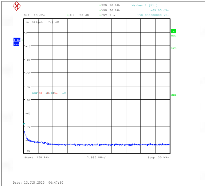
Band41(2535-2655)-10MHz-16QAM-41190-1RB#0-0.15~30-PASS
