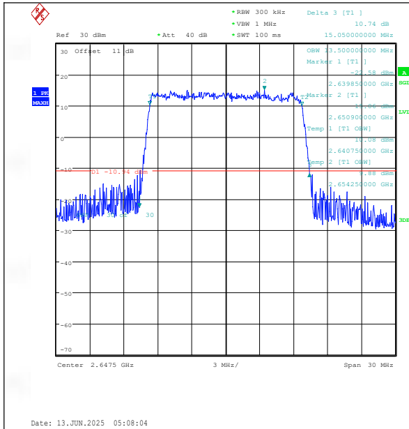
Band41(2535-2655)-15MHz-QPSK-41165-75RB#0-PASS
