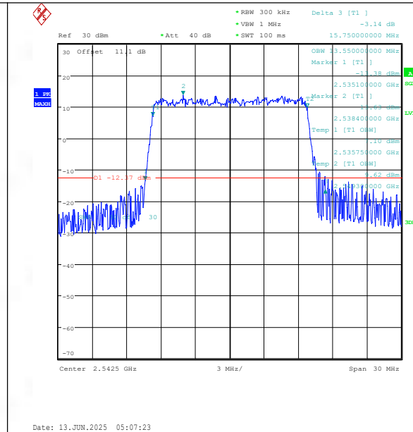
Band41(2535-2655)-15MHz-16QAM-40115-75RB#0-PASS
