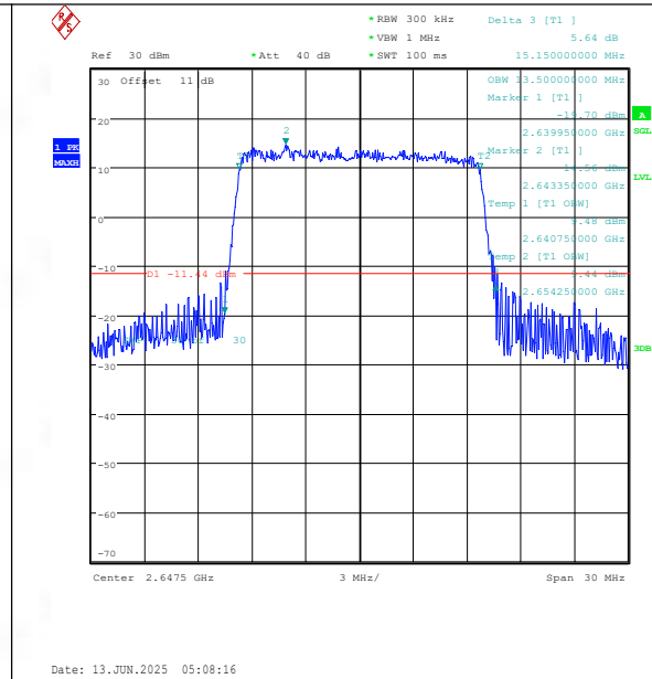
Band41(2535-2655)-15MHz-16QAM-41165-75RB#0-PASS
