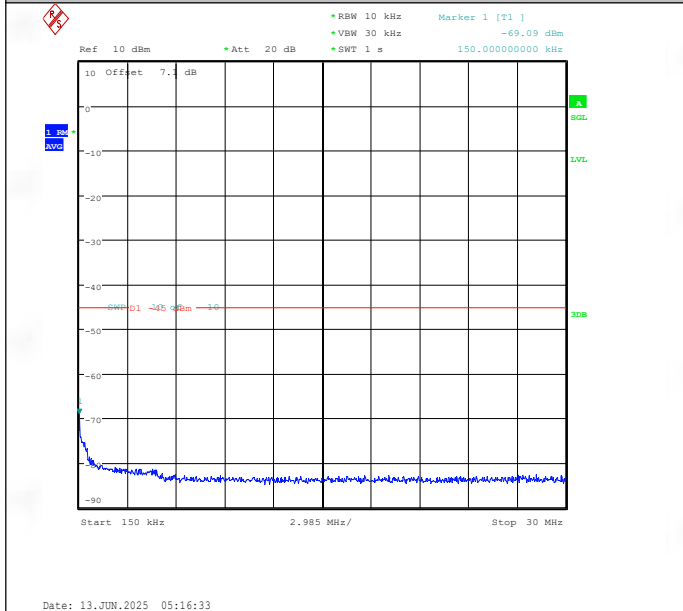
Band41(2535-2655)-15MHz-16QAM-40115-1RB#0-0.15~30-PASS
