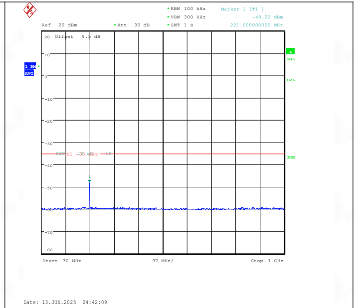
Band41(2535-2655)-10MHz-16QAM-40090-1RB#0-30~1000-PASS
