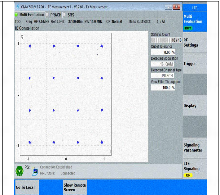
Band41(2535-2655)-15MHz-16QAM-41165-75RB#0-PASS
