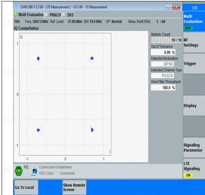
Band41(2535-2655)-15MHz-QPSK-41165-75RB#0-PASS
