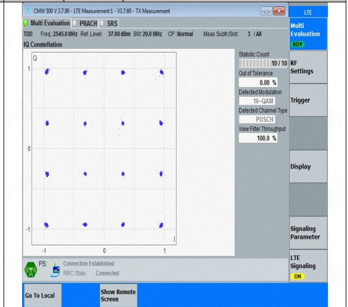
Band41(2535-2655)-20MHz-16QAM-40140-100RB#0-PASS
