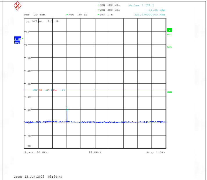
Band41(2535-2655)-20MHz-16QAM-41140-1RB#0-30~1000-PASS
