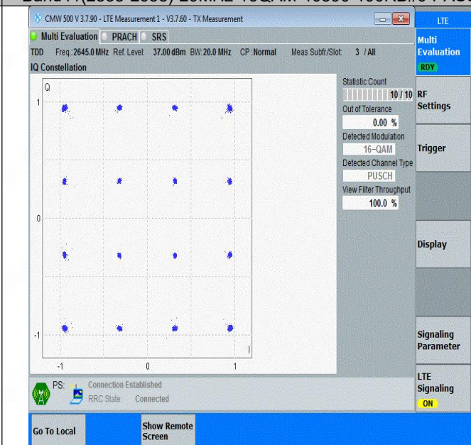
Band41(2535-2655)-20MHz-16QAM-41140-100RB#0-PASS
