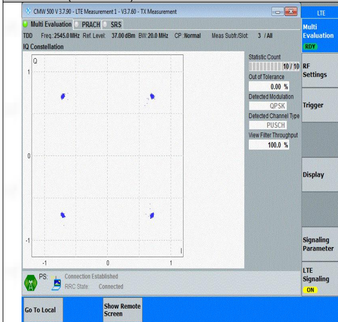
Band41(2535-2655)-20MHz-QPSK-40140-100RB#0-PASS
