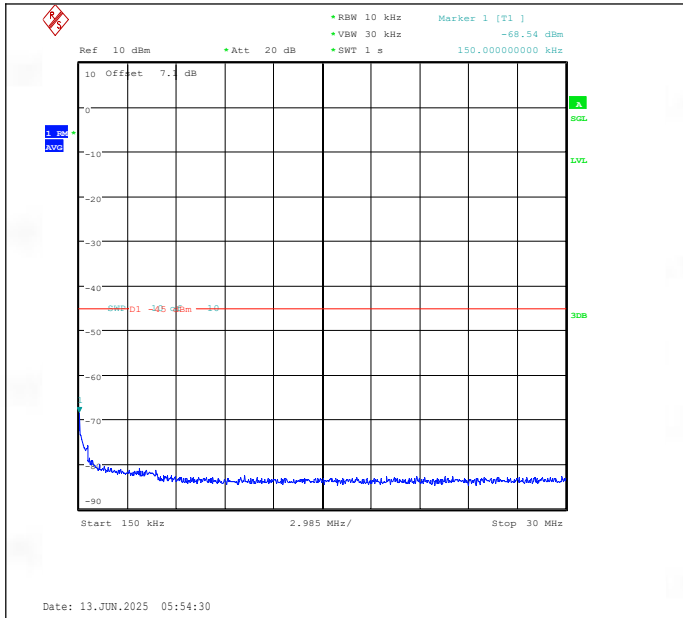
Band41(2535-2655)-20MHz-16QAM-41140-1RB#0-0.15~30-PASS
