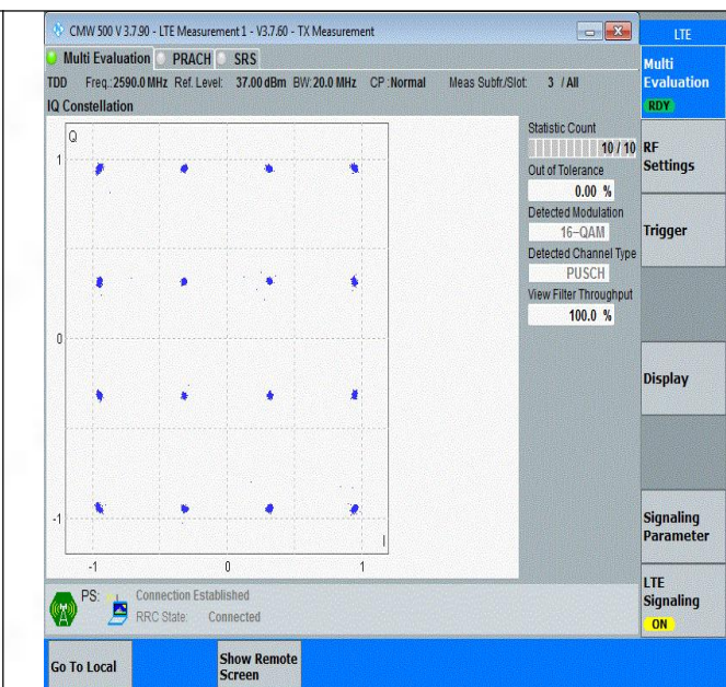
Band41(2535-2655)-20MHz-16QAM-40590-100RB#0-PASS
