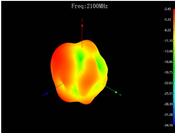
Ant1: 2100Mhz
