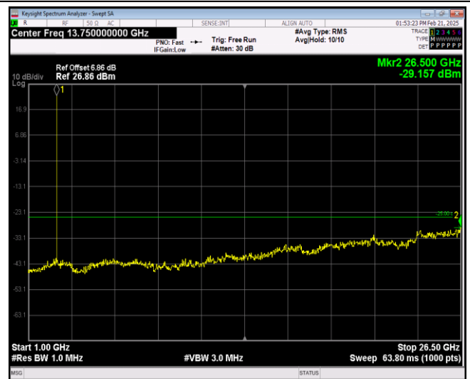
Band41-5MHz-16QAM-39675-1RB#0-Range2:1000~ 26500MHz
