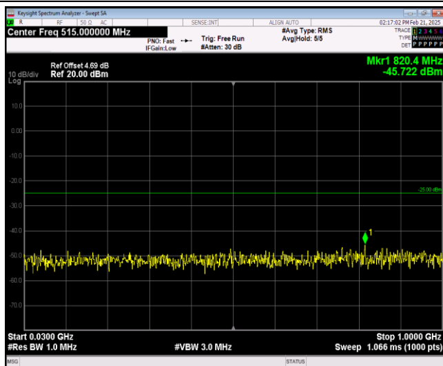
Band41-20MHz-16QAM-40620-1RB#0-Range1:30~1000MHz
