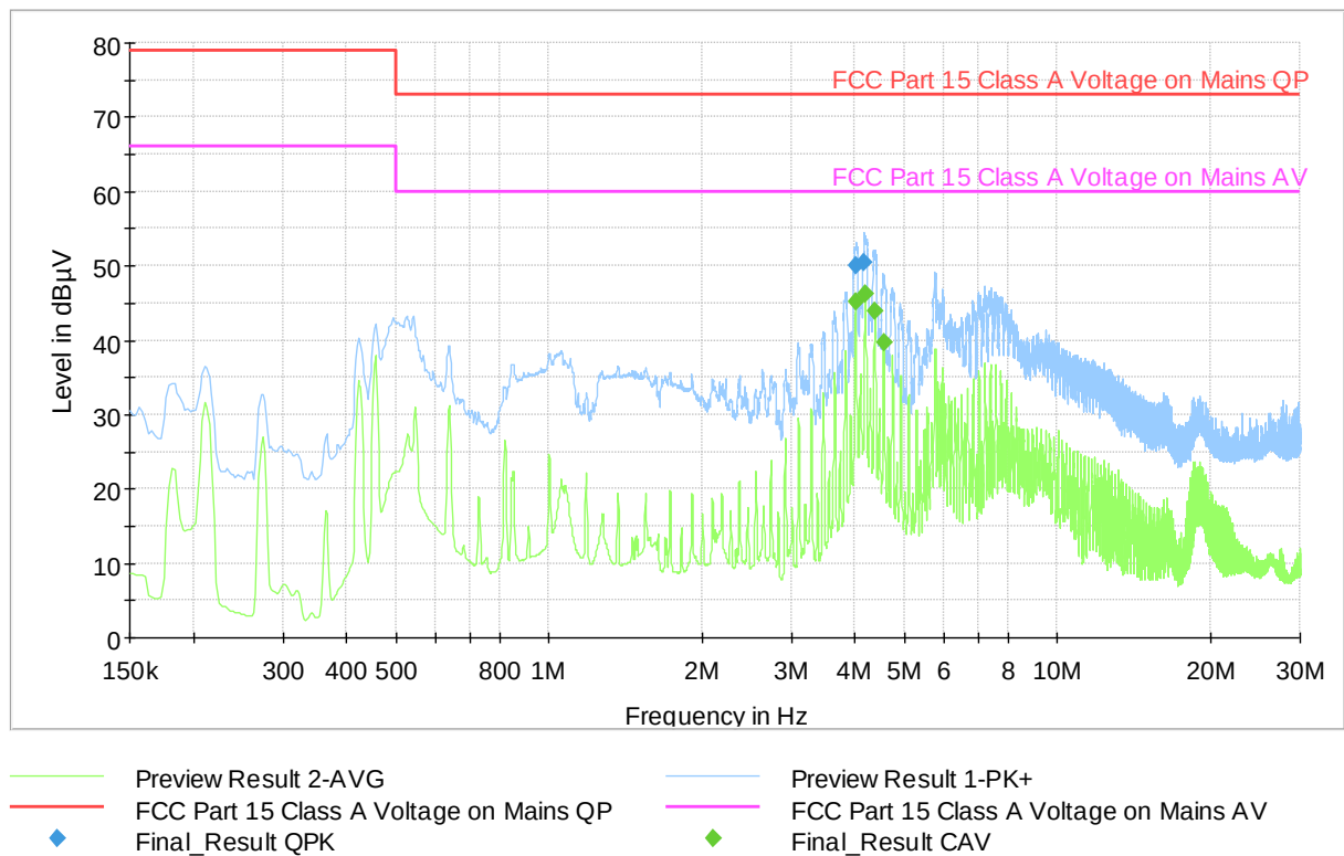
Figure 2: The measured curves with peak-detector and average detector
