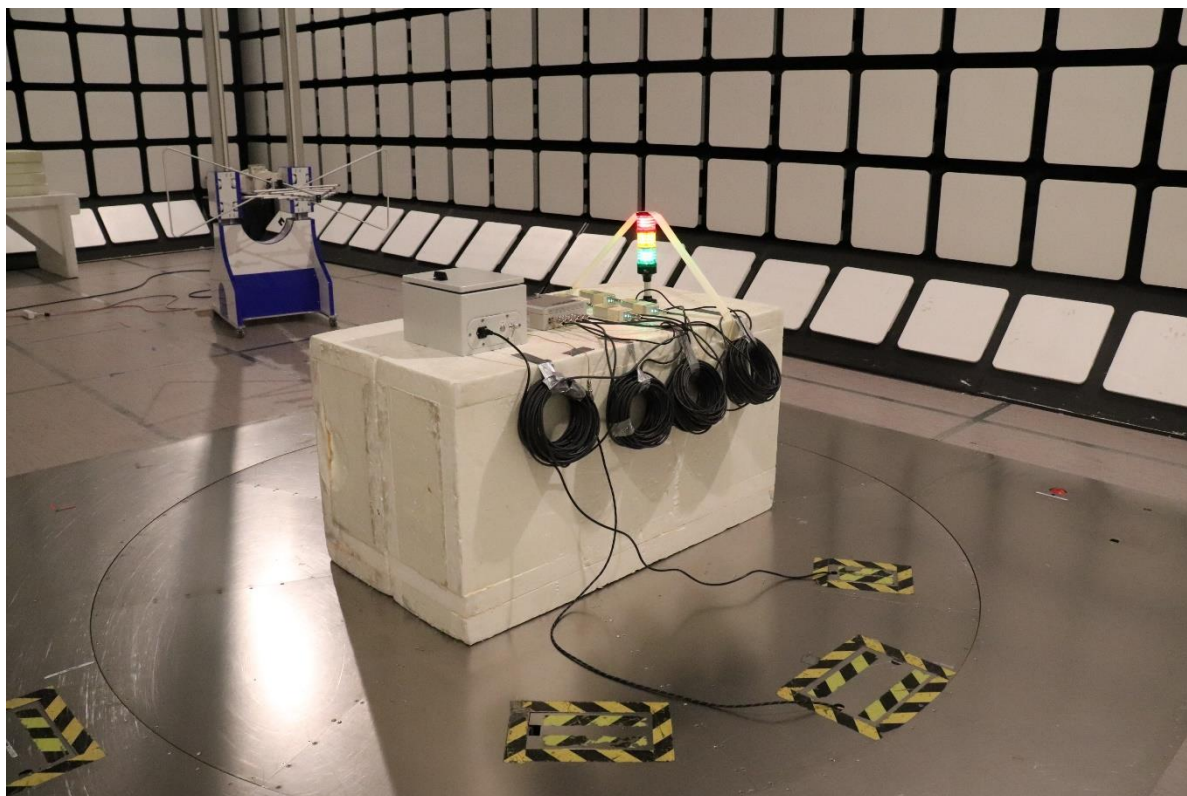
Photograph 9. Radiated Emissions 30 – 1000 MHz
