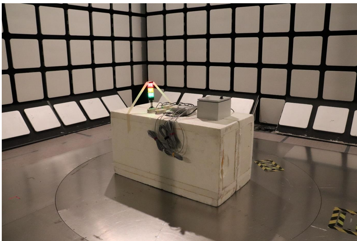
Photograph 10. Radiated Emissions 30 – 1000 MHz
