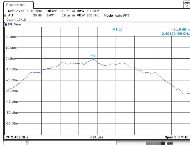
BLE_2M_Ant1_2402_0~Reference
