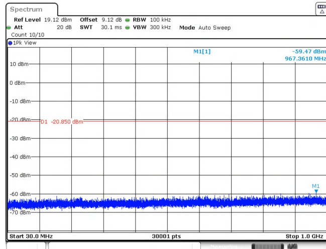
BLE_1M_Ant1_2402_30~1000
