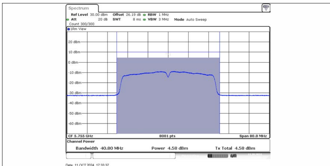
11AC40MIMO Ant2_5755
