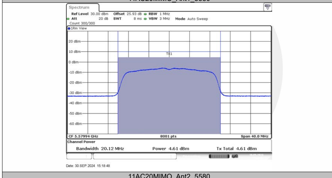
11AC20MIMO Ant2_5580
