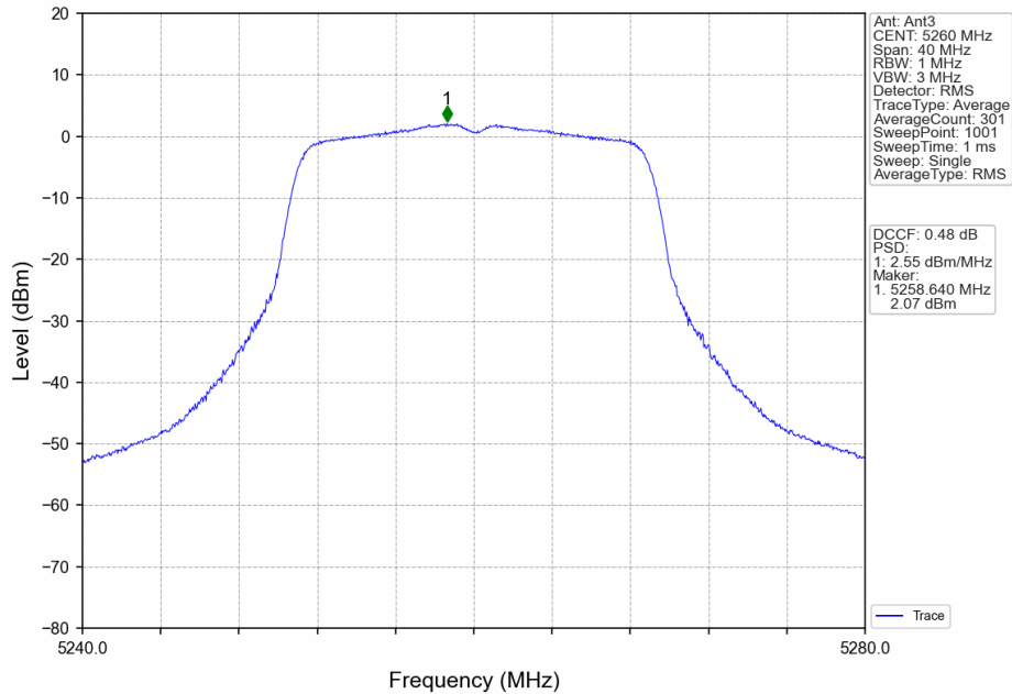
802.11ac(VHT20)_LCH_5260MHz_MIMO_NTNV
