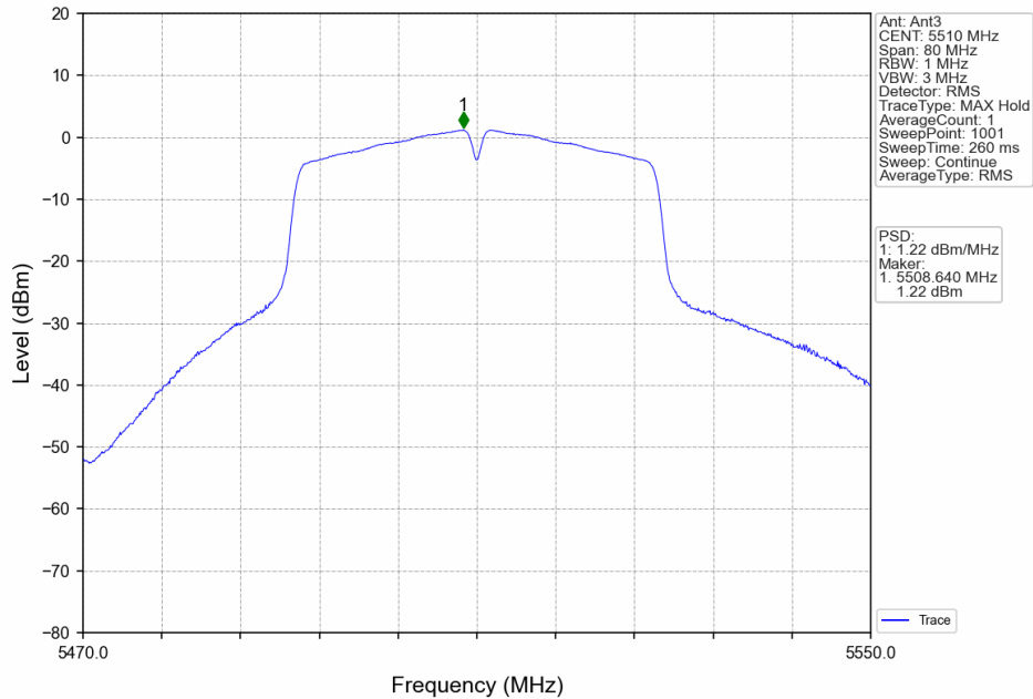
802.11ac(VHT40)_LCH_5510MHz_MIMO_NTNV
