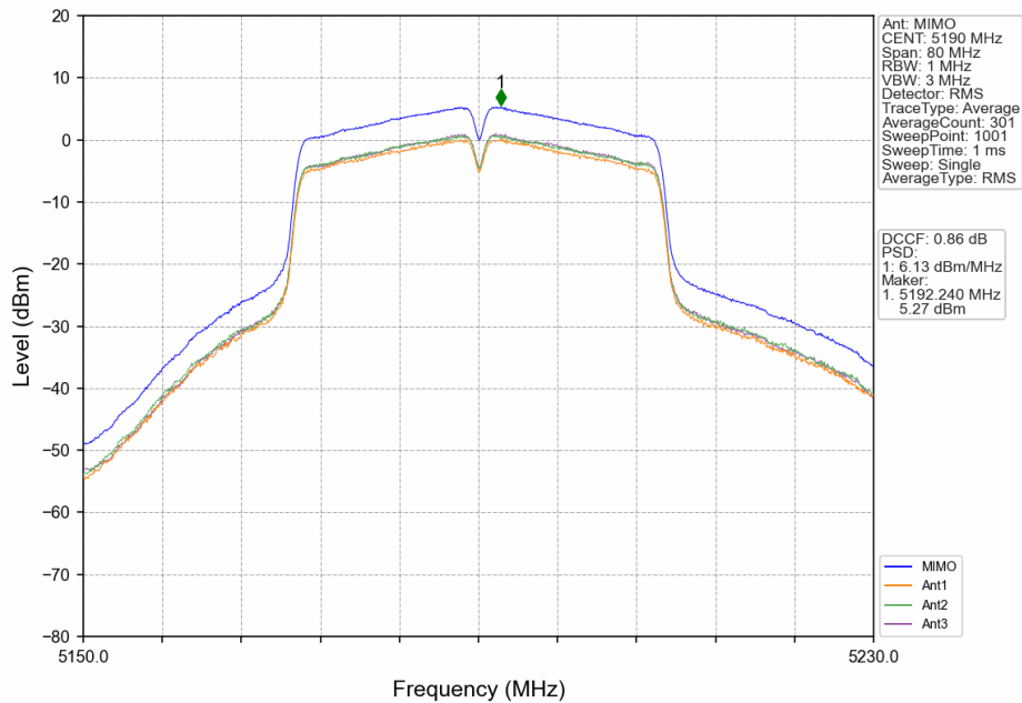
802.11ac(VHT40)_LCH_5190MHz_MIMO_NTNV
