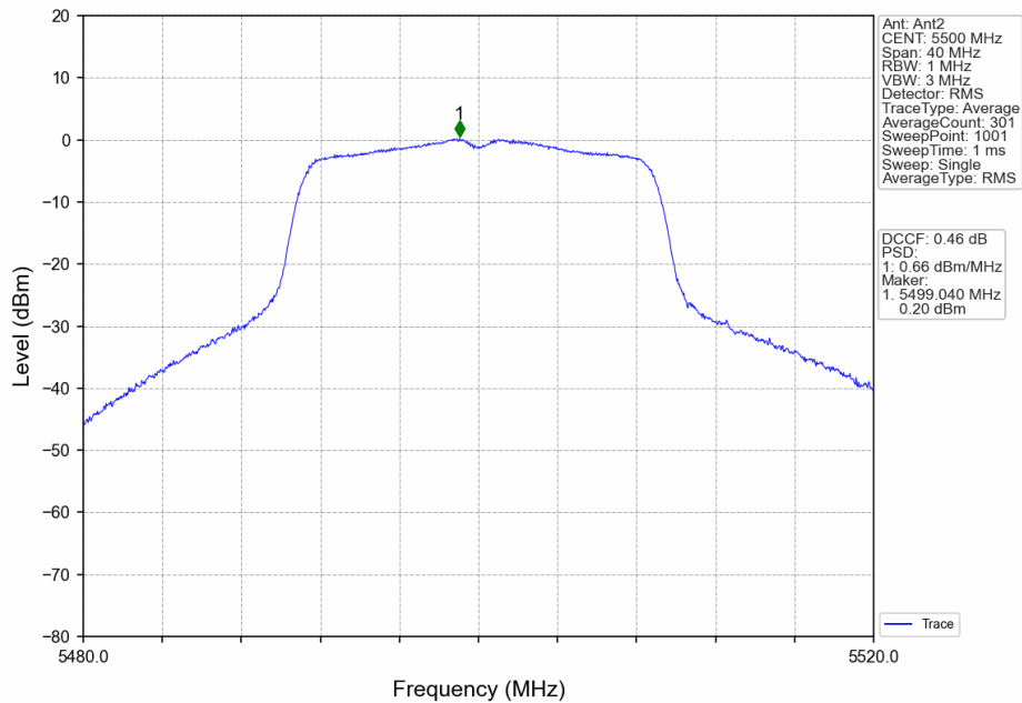
802.11ac(VHT20)_LCH_5500MHz_Ant2_NTNV
