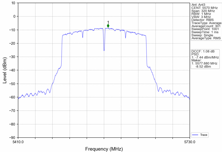
802.11ac(VHT160)_MCH_5570MHz_MIMO_NTNV
