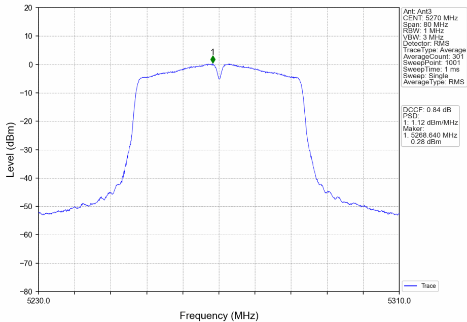
802.11ac(VHT40)_LCH_5270MHz_MIMO_NTNV
