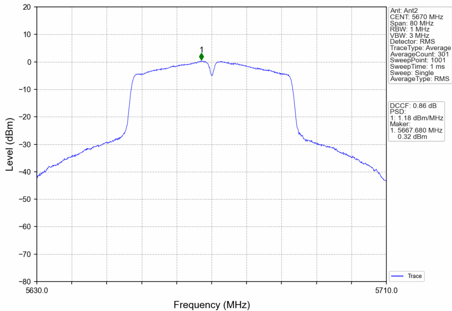
802.11ac(VHT40)_HCH_5670MHz_Ant2_NTNV
