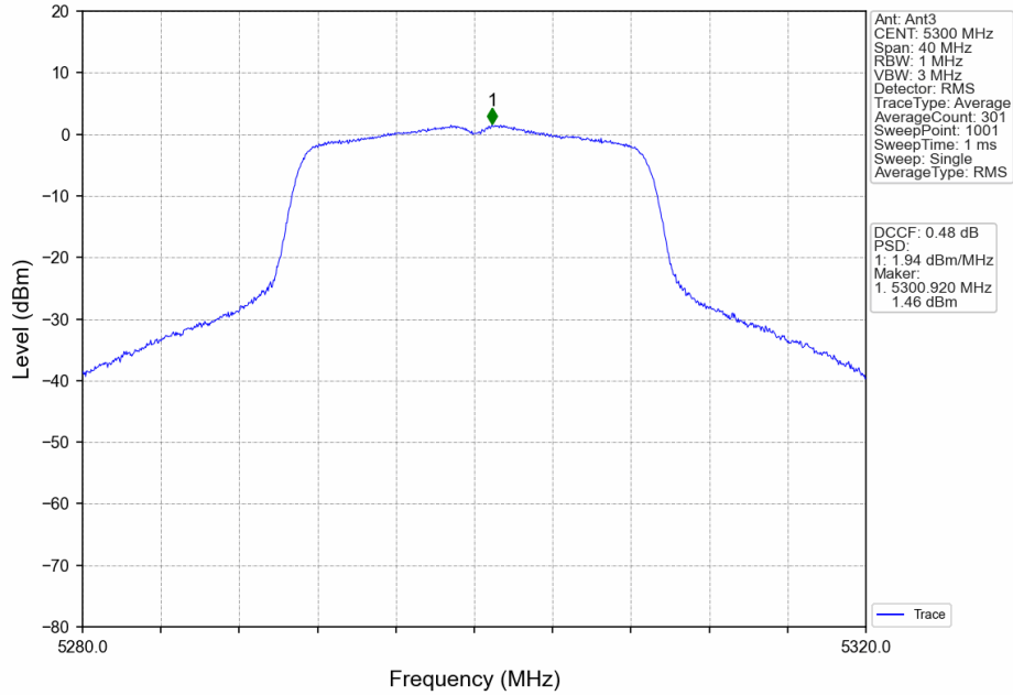
802.11ac(VHT20)_MCH_5300MHz_MIMO_NTNV
