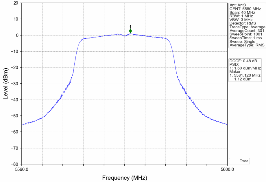
802.11ac(VHT20)_MCH_5580MHz_MIMO_NTNV
