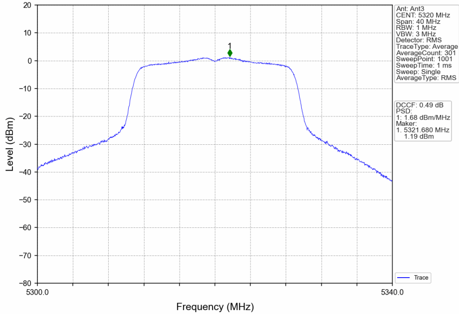
802.11ac(VHT20)_HCH_5320MHz_MIMO_NTNV
