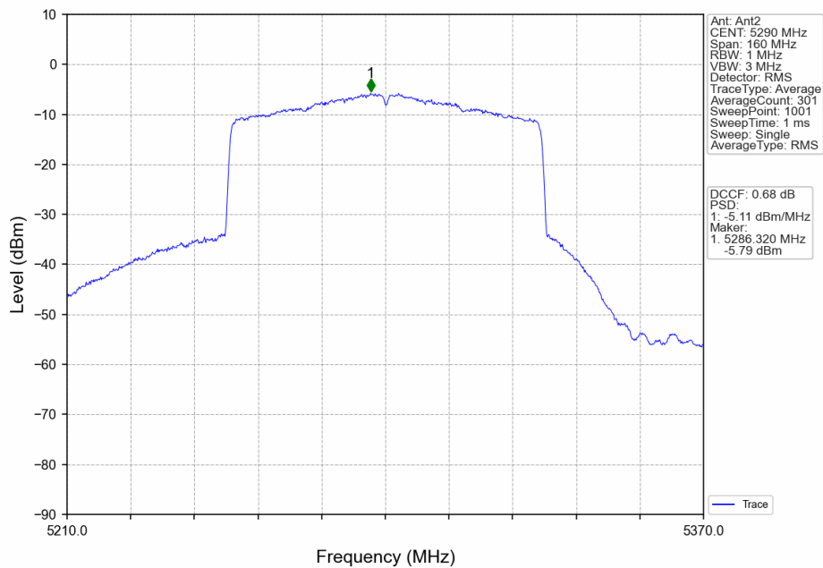
802.11ac(VHT80)_MCH_5290MHz_Ant2_NTNV
