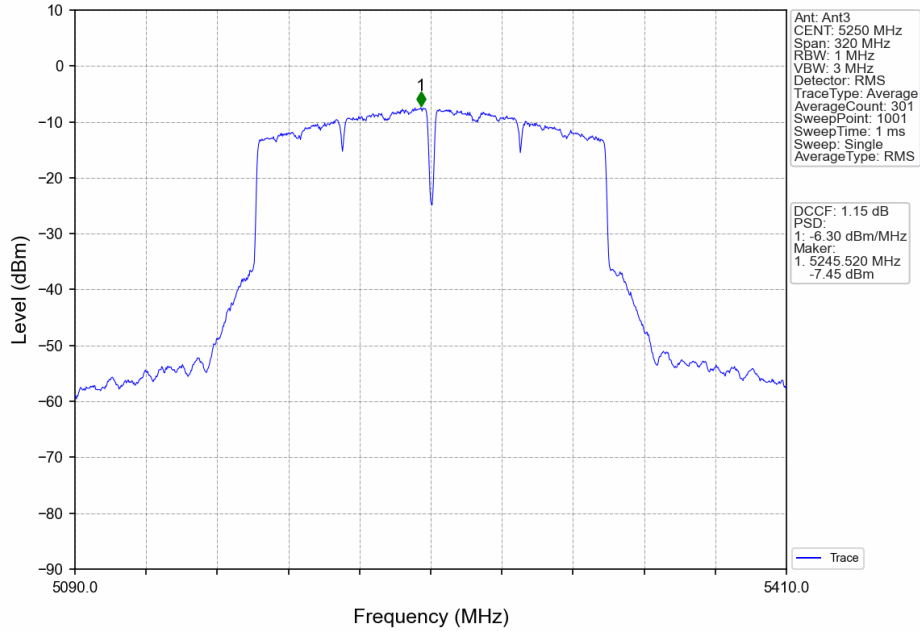
802.11ac(VHT160)_MCH_5250MHz_MIMO_NTNV
