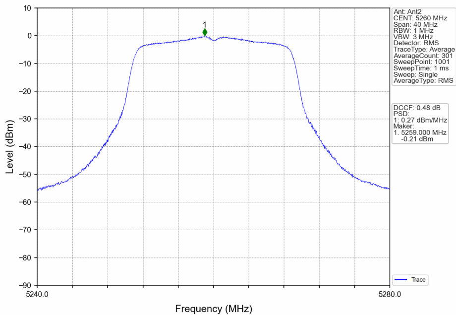
802.11ac(VHT20)_LCH_5260MHz_Ant2_NTNV
