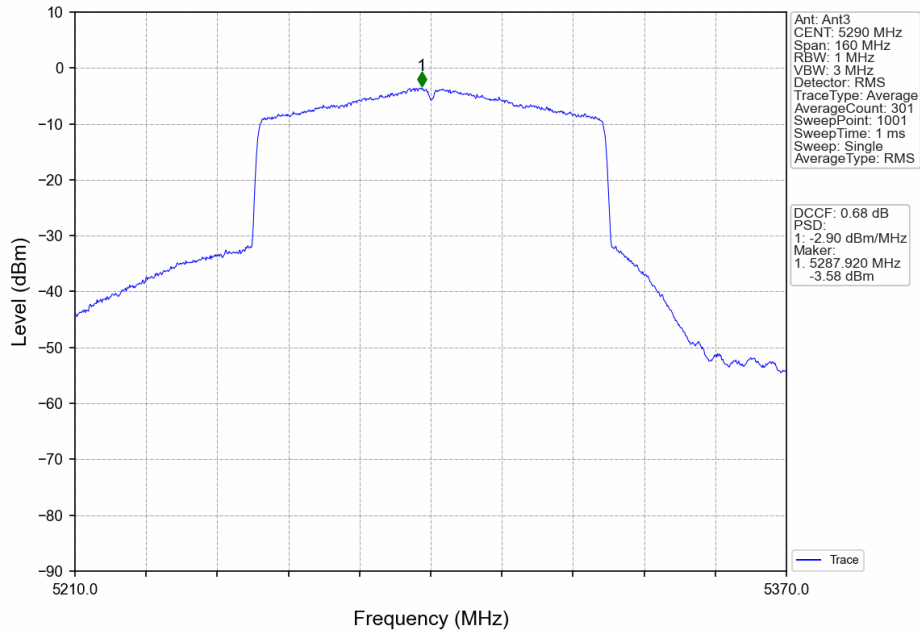
802.11ac(VHT80)_MCH_5290MHz_MIMO_NTNV
