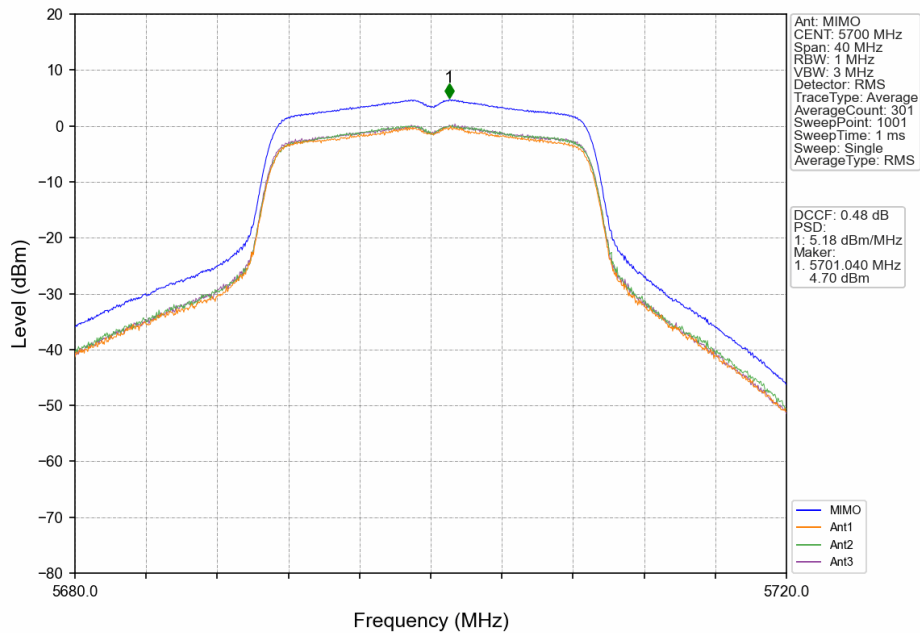
802.11ac(VHT20)_HCH_5700MHz_MIMO_NTNV
