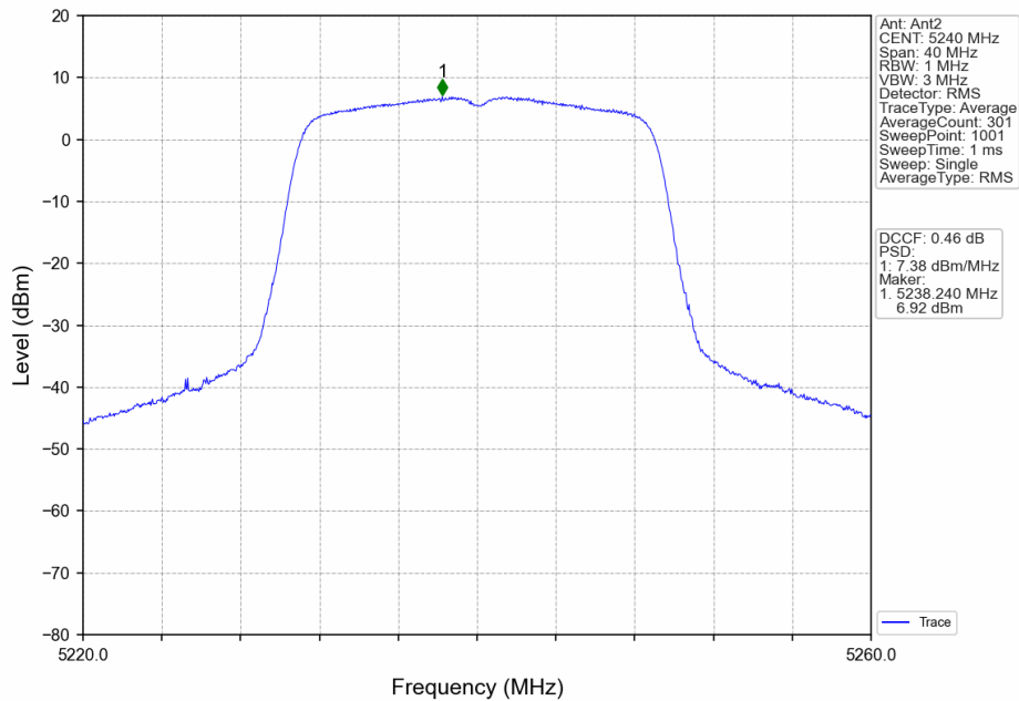
802.11ac(VHT20)_HCH_5240MHz_Ant2_NTNV
