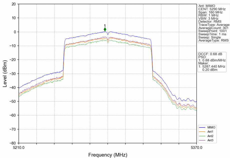
802.11ac(VHT80)_MCH_5290MHz_MIMO_NTNV
