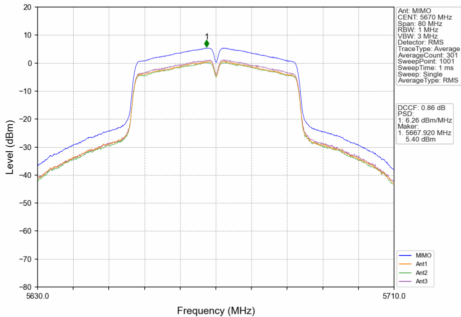
802.11ac(VHT40)_HCH_5670MHz_MIMO_NTNV
